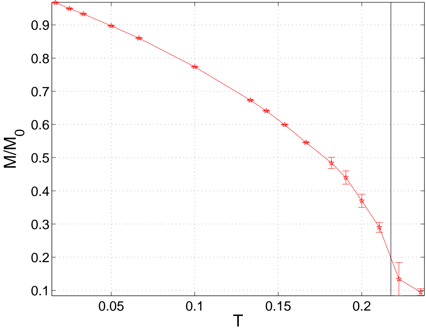
Cubic system with exponential coupling; l/a = .75
