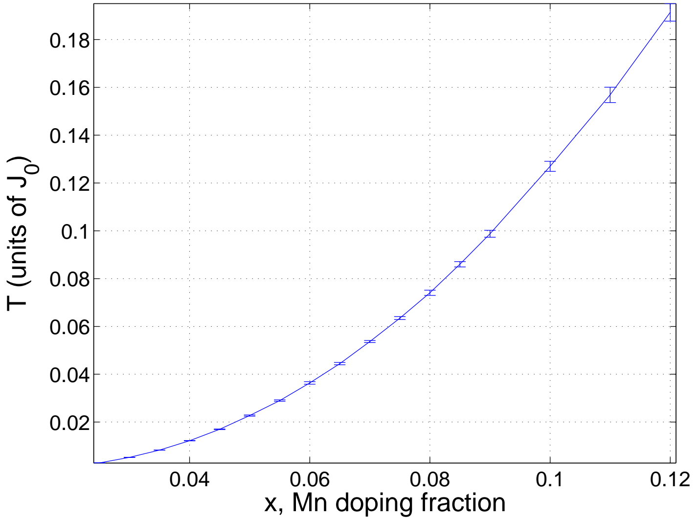
Curie Temperatures for n_c/n_i = .1 ; l/a = .5
