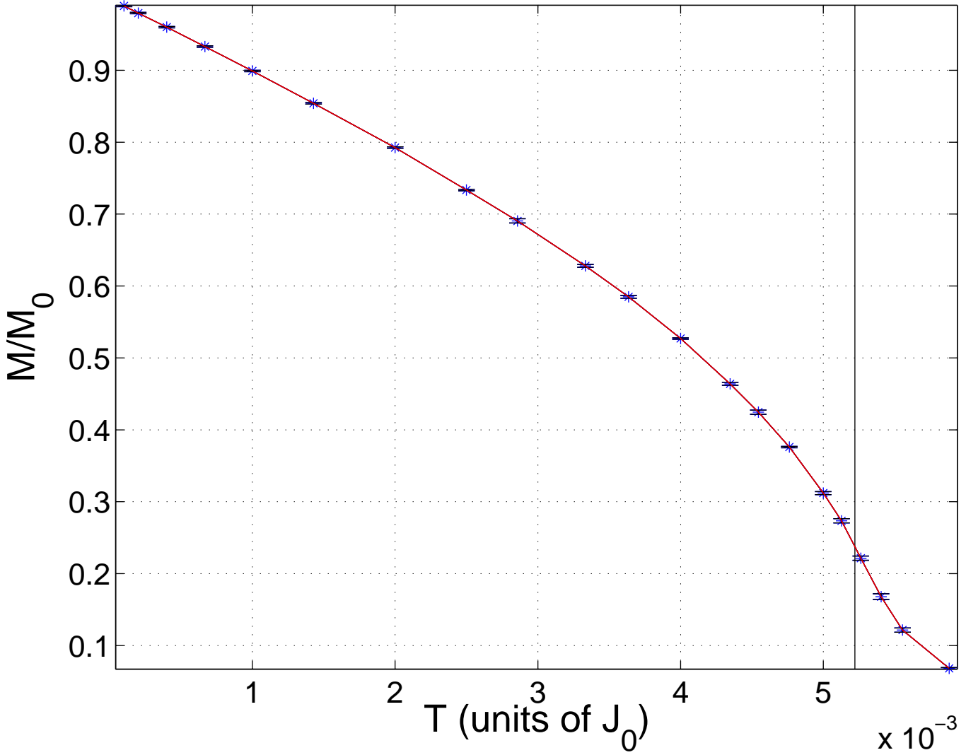
Magnetization for n_c/n_i=.1 , l/a = .5 , x = .03
