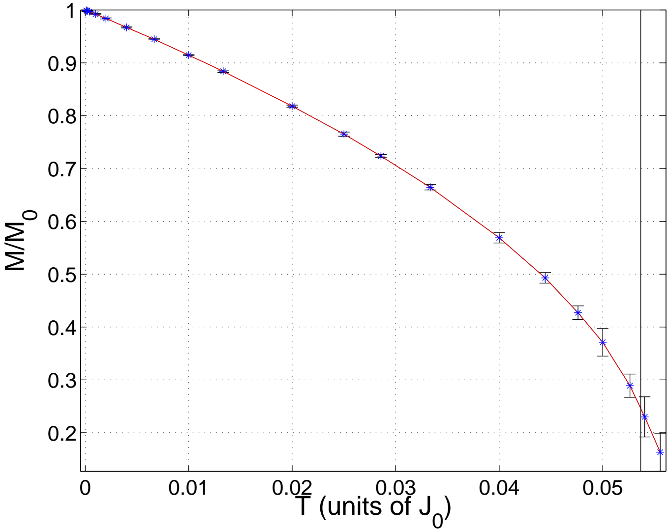
Magnetization for n_c/n_i=.1 , l/a = .5 , x = .07
