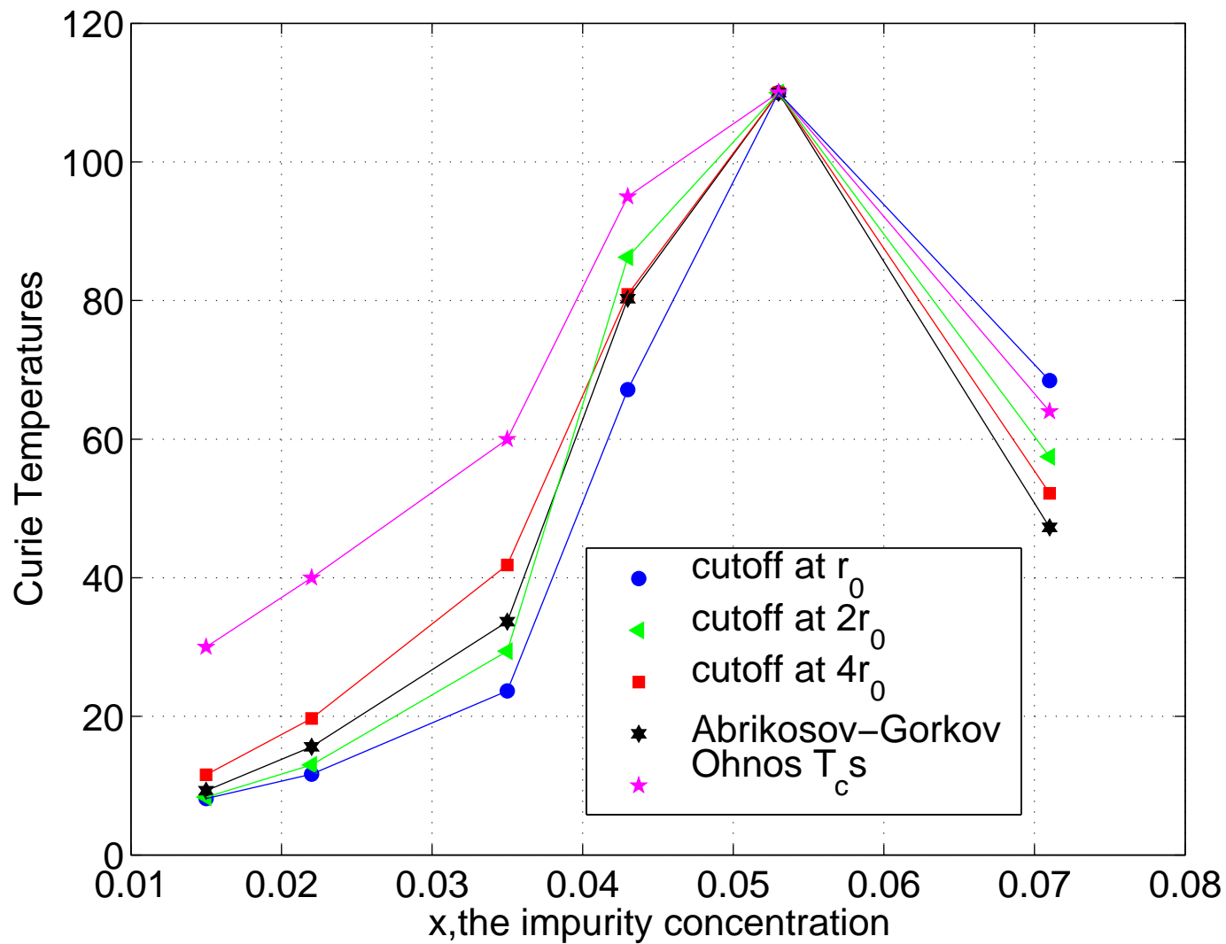
NORMALIZED T_c values [based on Ohnos experiments] (PRB 57,R2037[1998])
