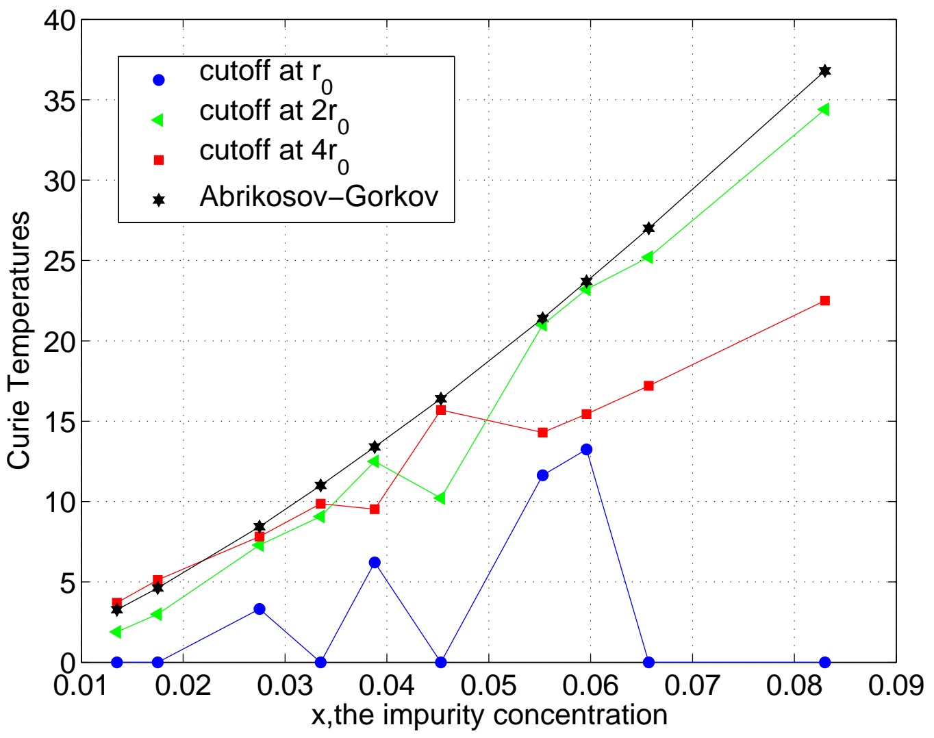
Calculated T_c values [based on Penn experiments] (PRB 66,012408[2002])
