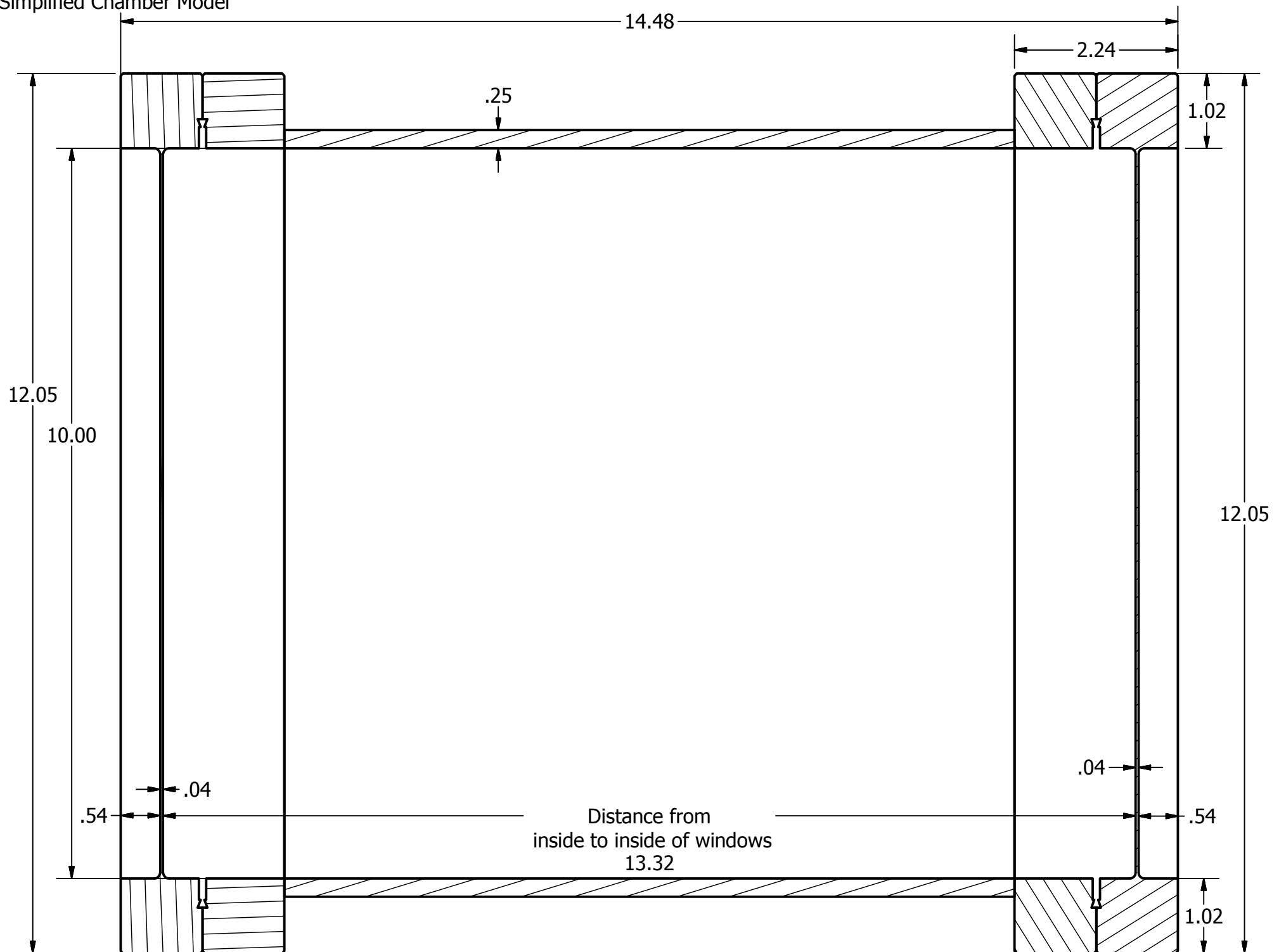
Simplified Chamber Model
