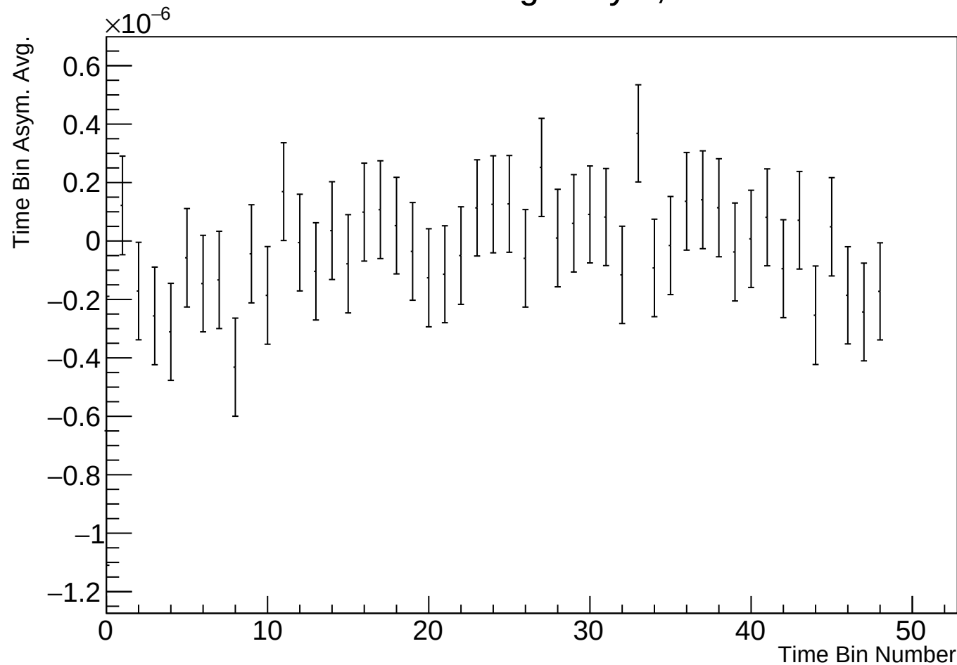
Time Bin Run Average Asym, r17784 w18
