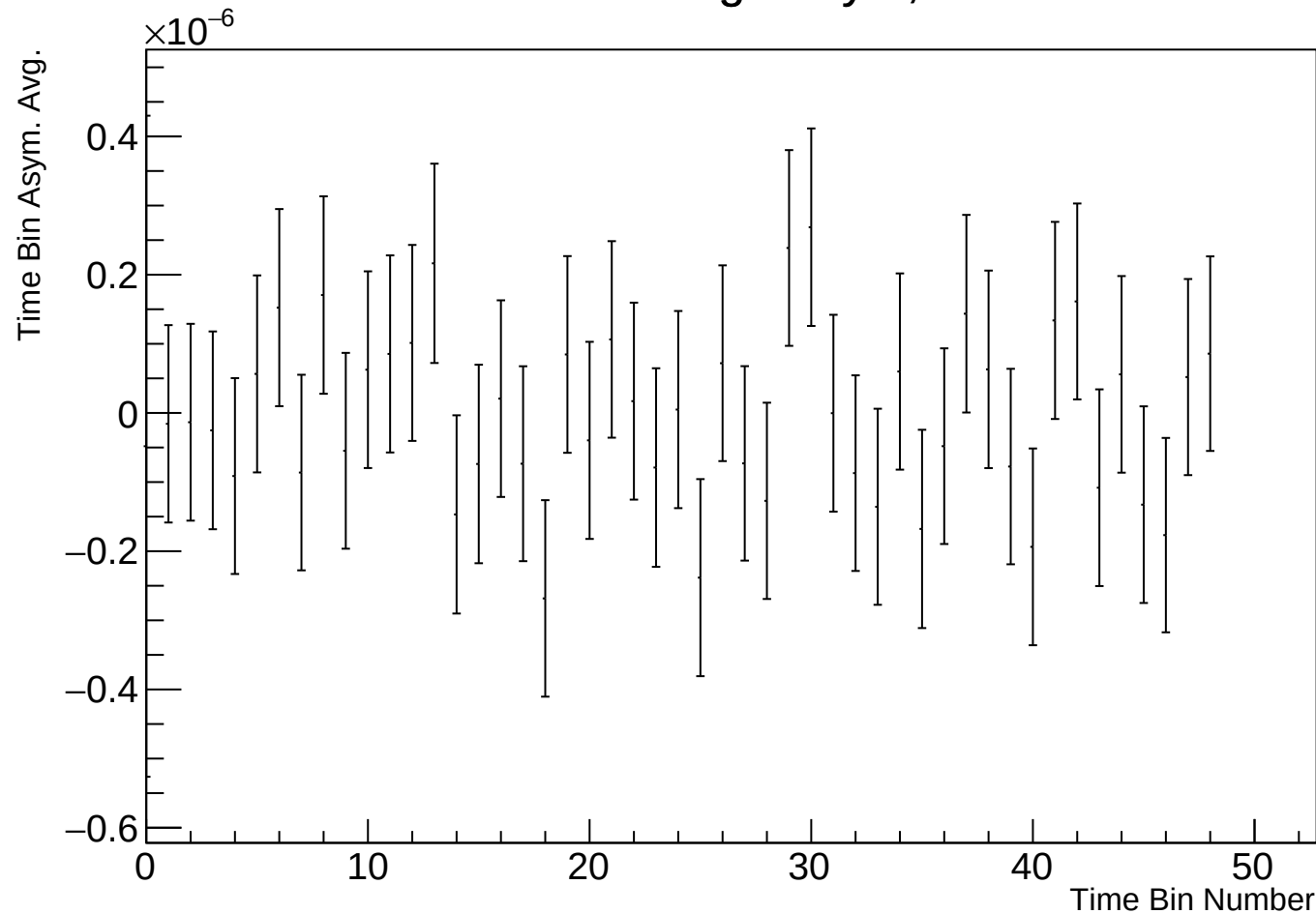
Time Bin Run Average Asym, r17784 w91
