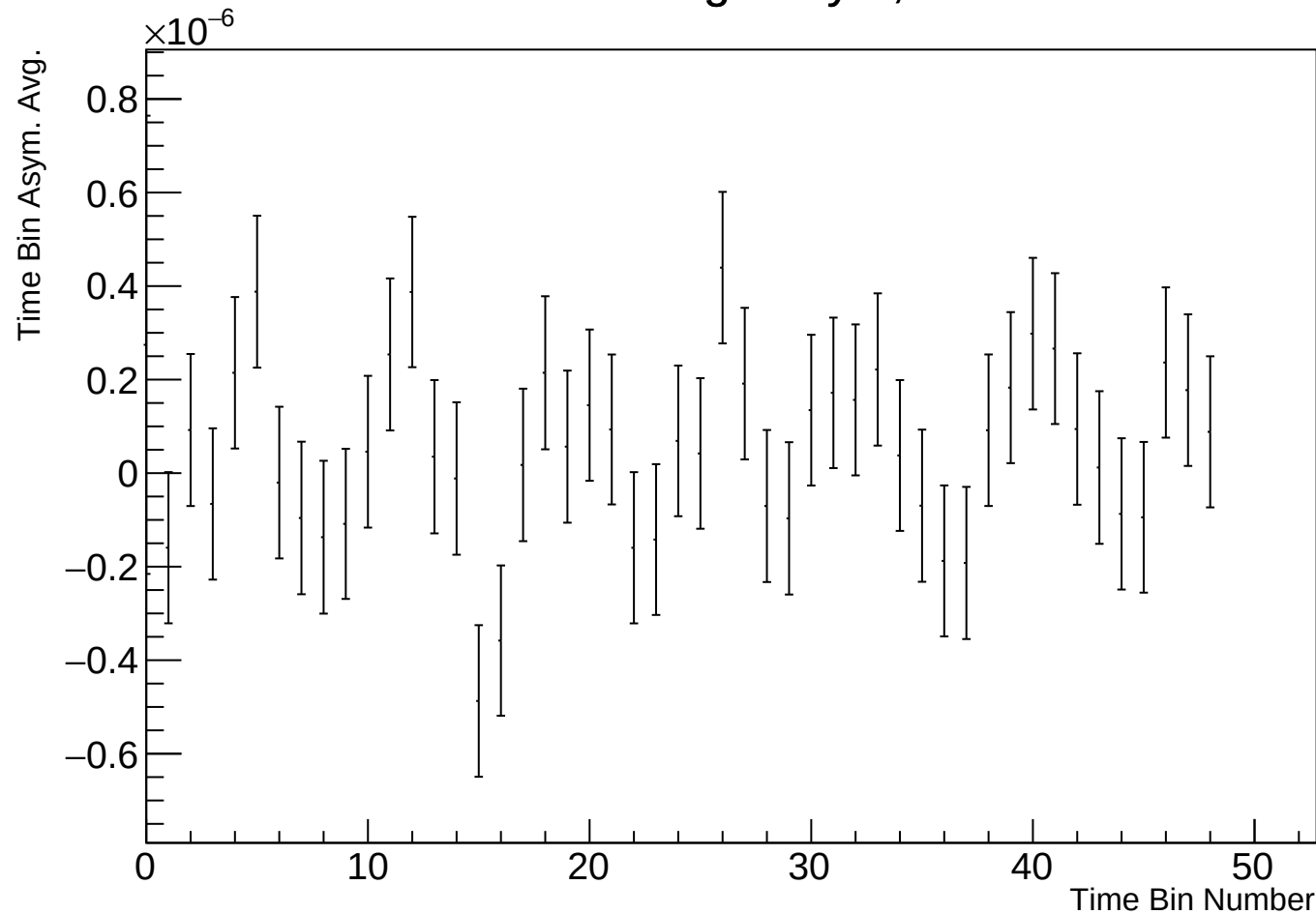
Time Bin Run Average Asym, r17784 w131
