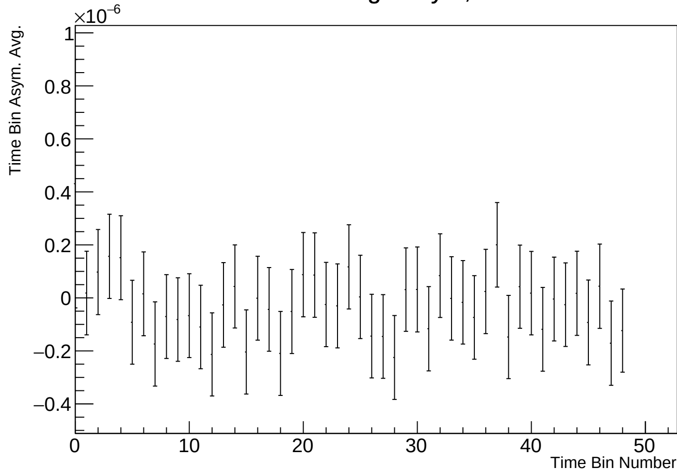
Time Bin Run Average Asym, r17784 w55
