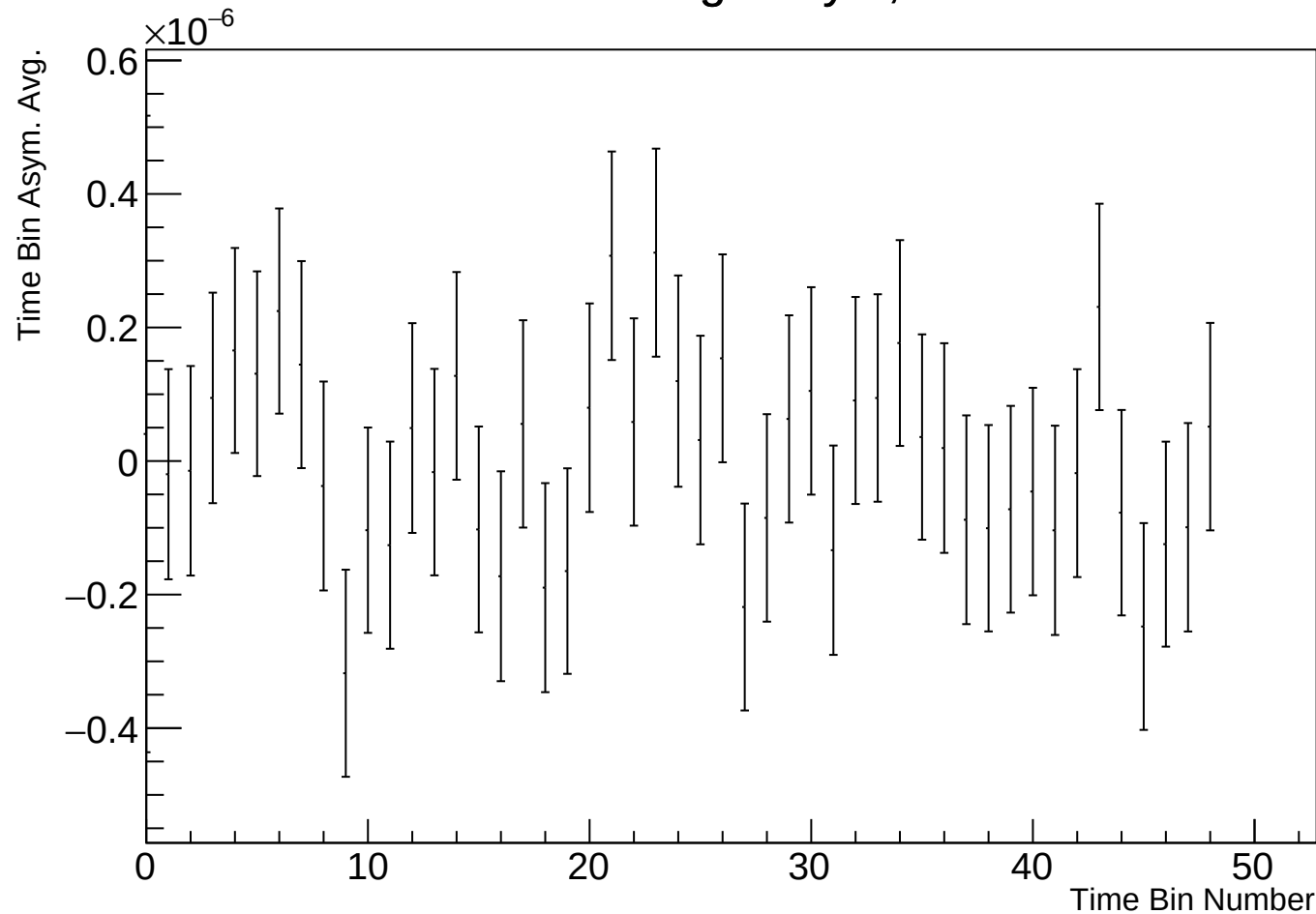
Time Bin Run Average Asym, r17784 w139
