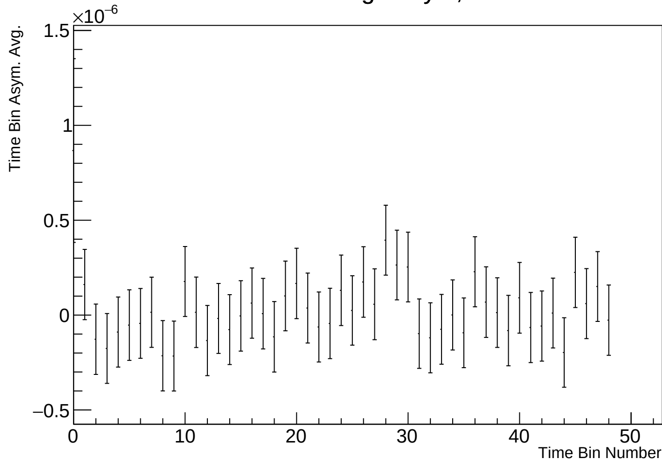
Time Bin Run Average Asym, r17784 w51
