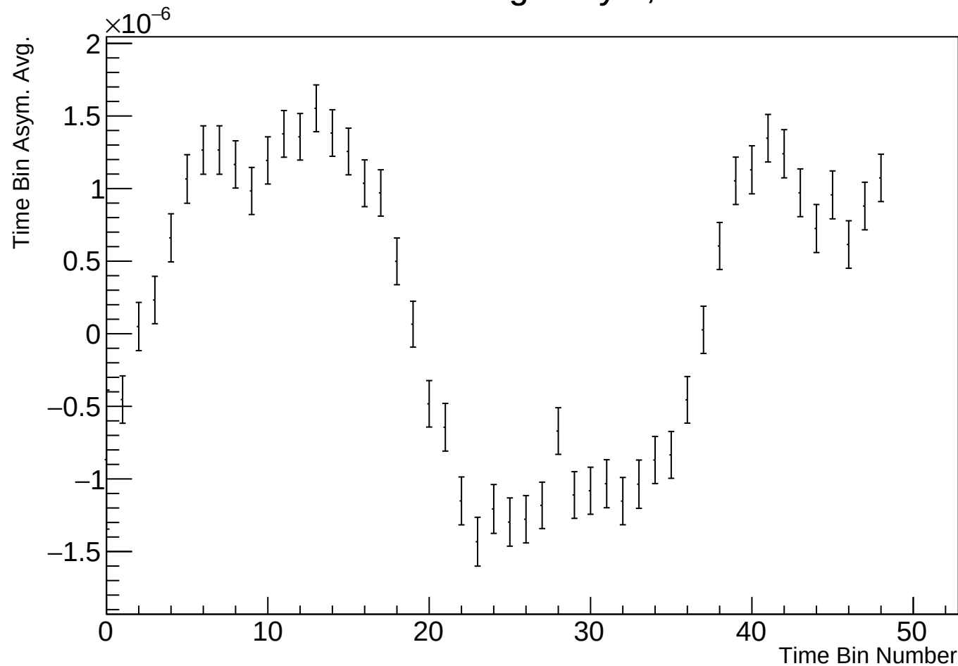
Time Bin Run Average Asym, r17784 w107
