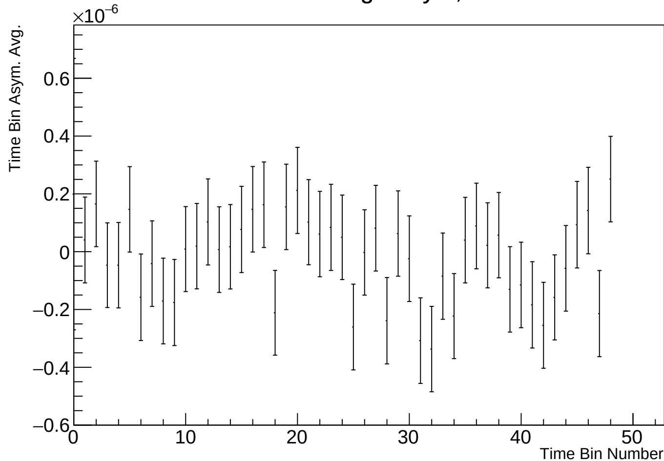
Time Bin Run Average Asym, r17784 w74
