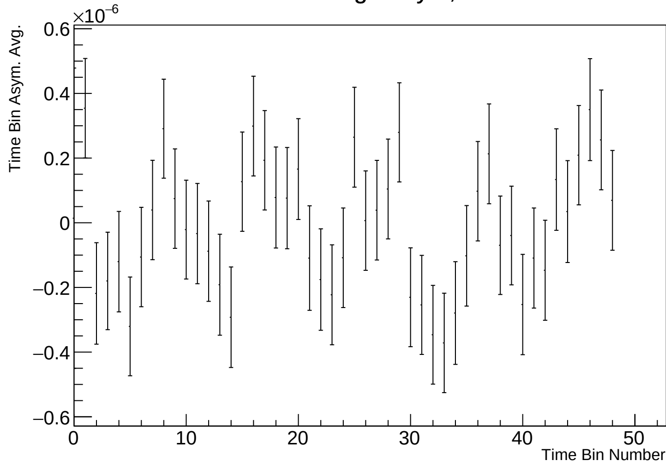
Time Bin Run Average Asym, r17784 w123
