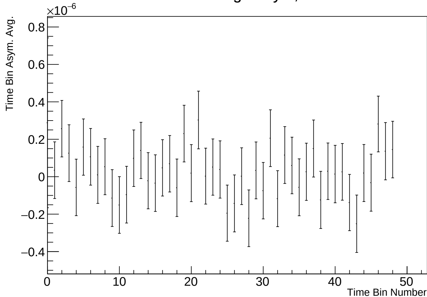
Time Bin Run Average Asym, r17784 w21
