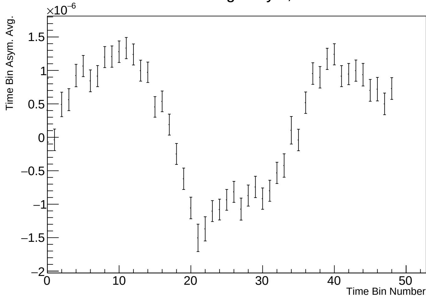
Time Bin Run Average Asym, r17784 w125
