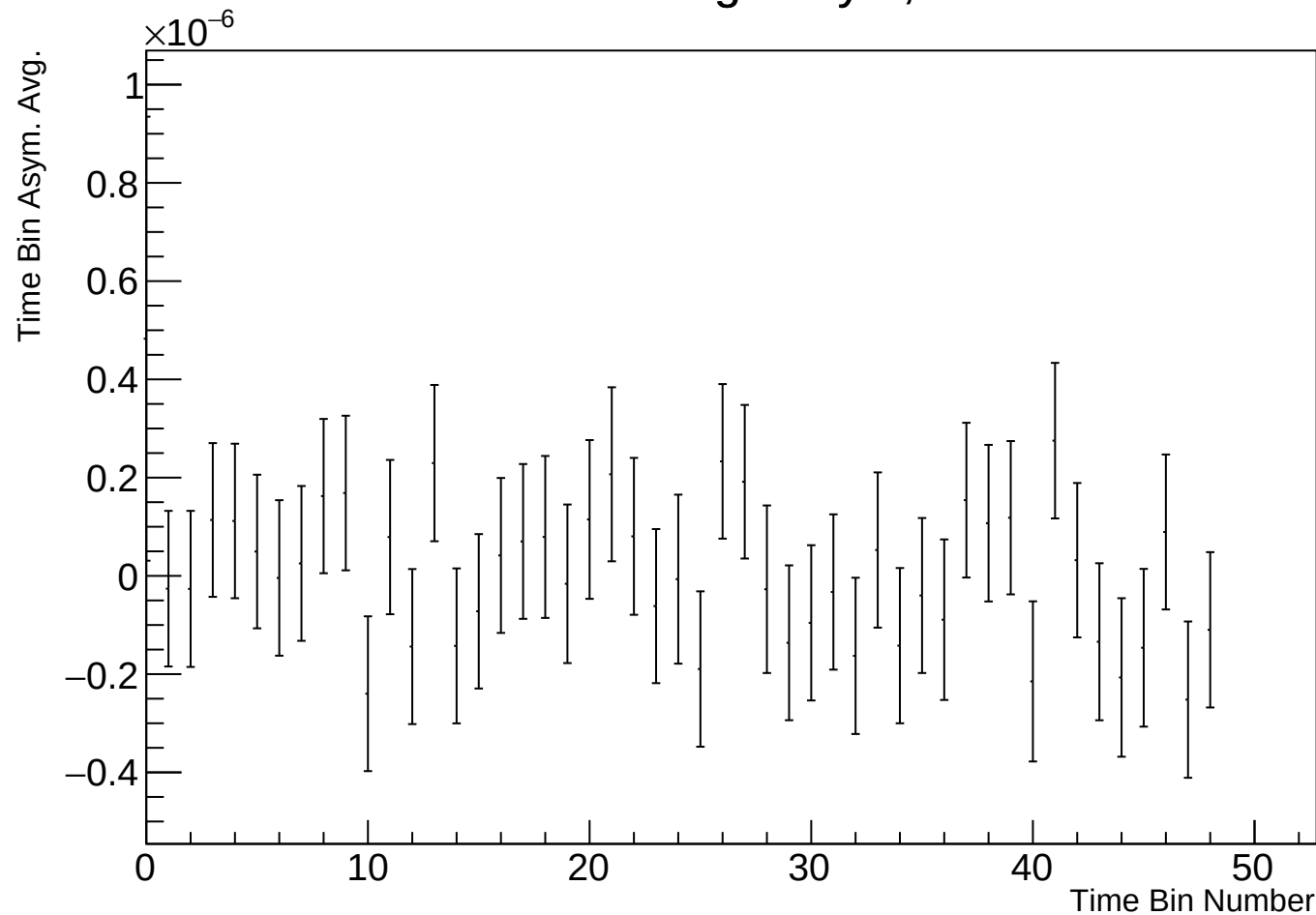
Time Bin Run Average Asym, r17784 w22
