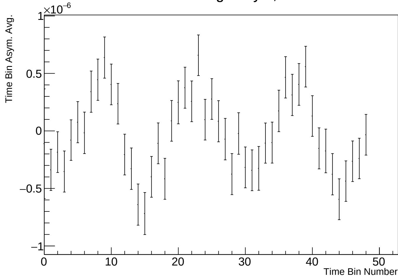
Time Bin Run Average Asym, r17784 w49
