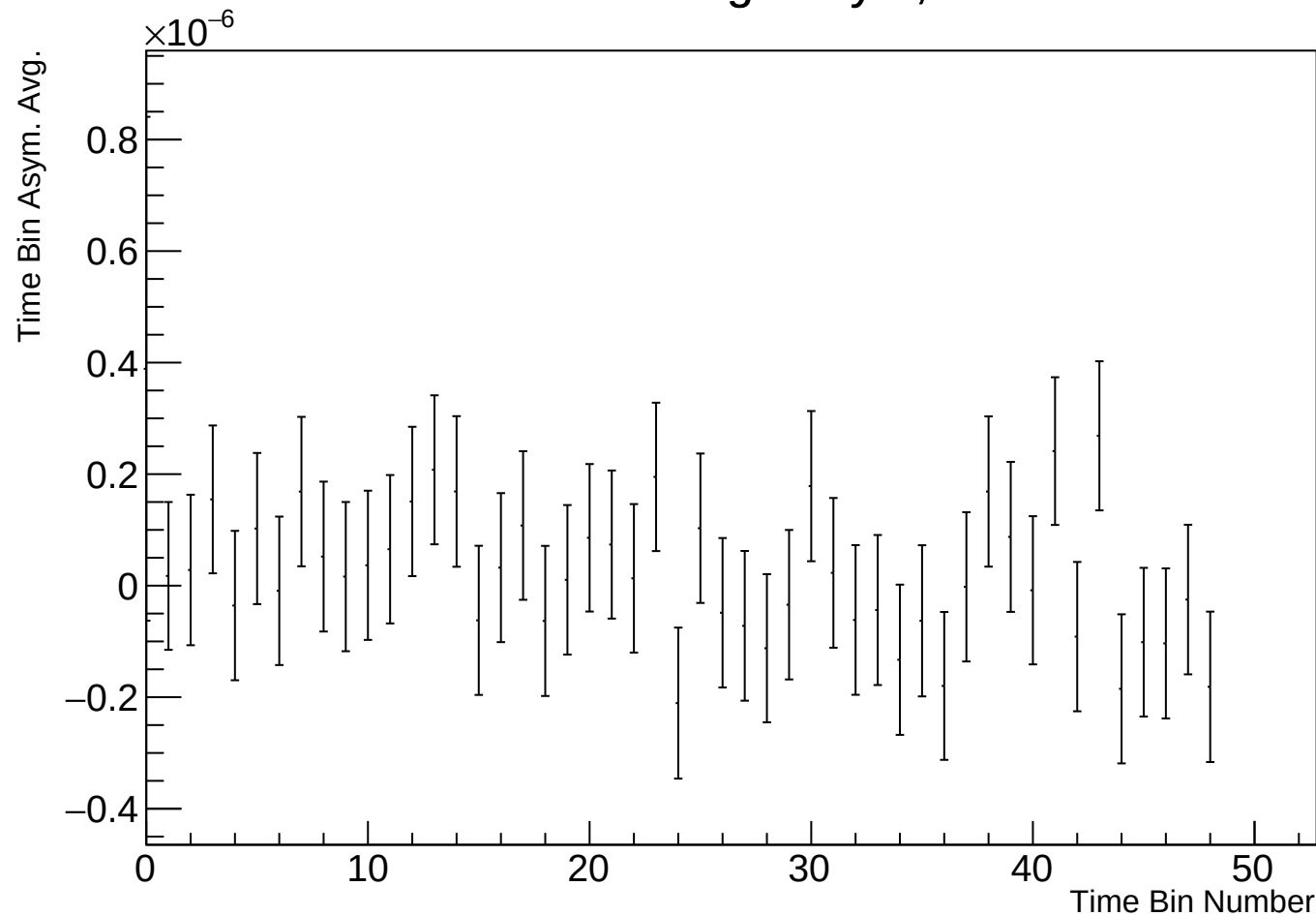
Time Bin Run Average Asym, r17784 w5
