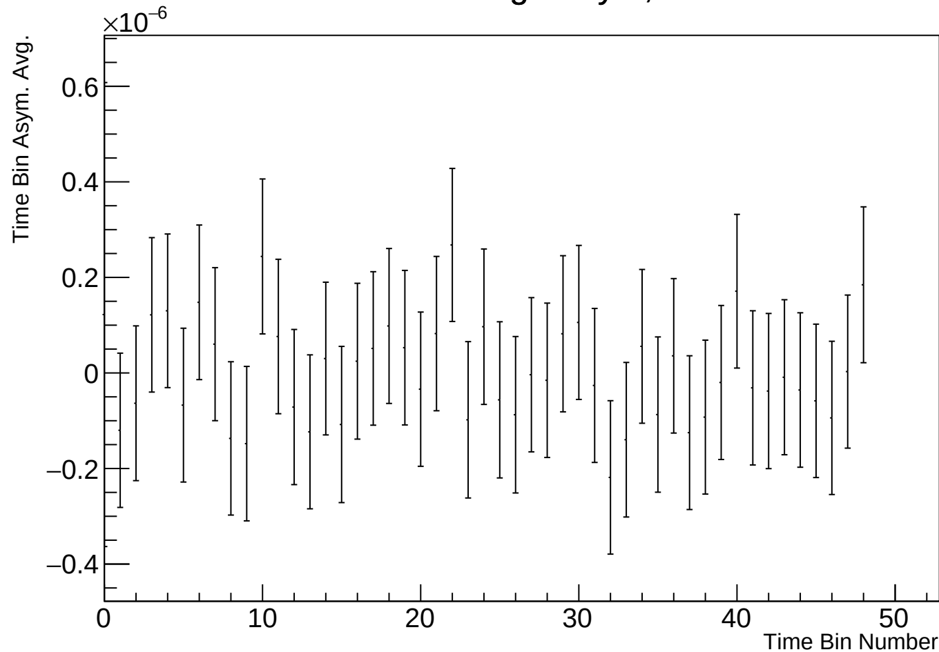
Time Bin Run Average Asym, r17784 w94
