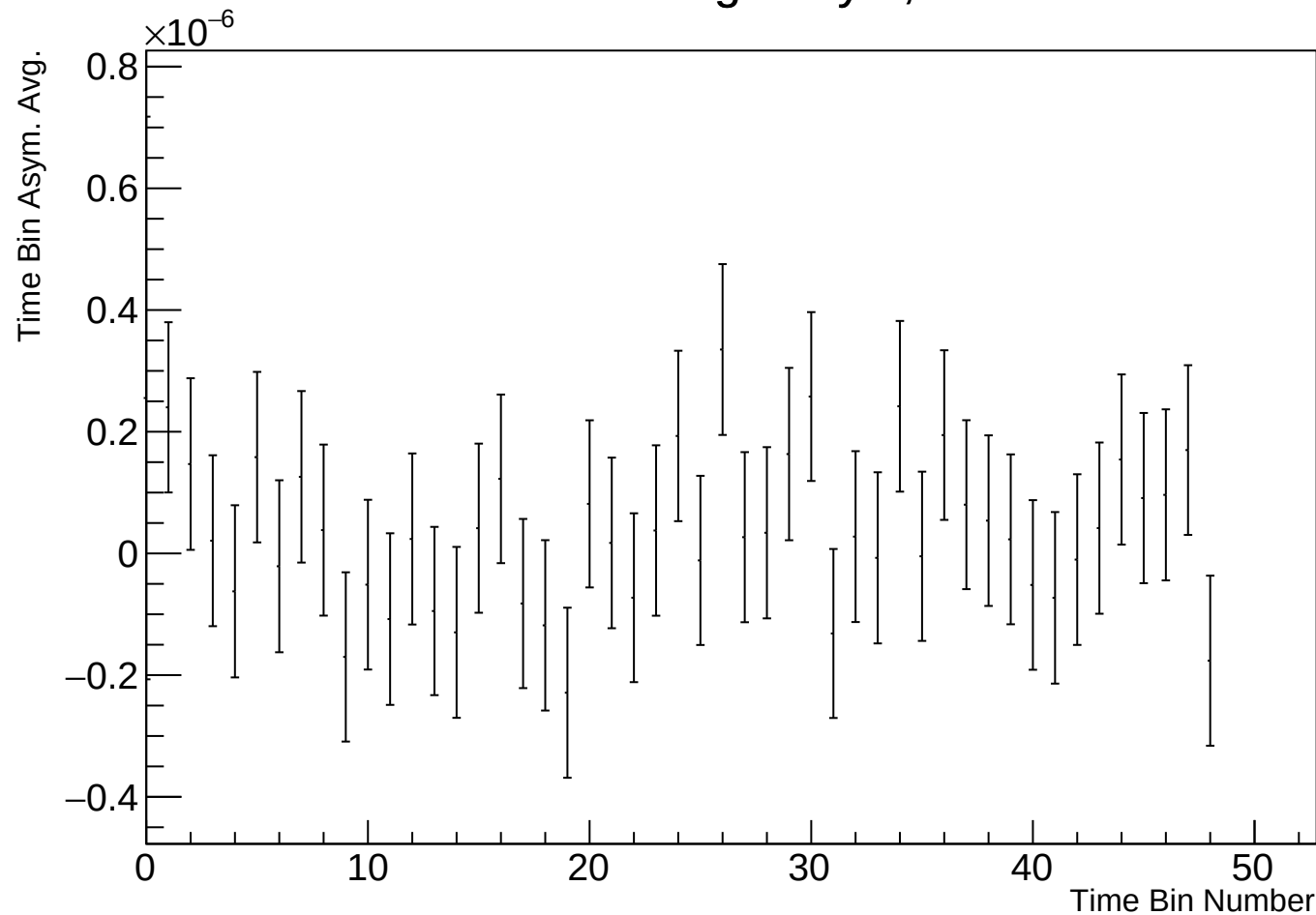
Time Bin Run Average Asym, r17784 w16
