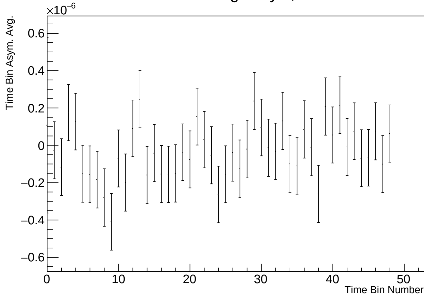
Time Bin Run Average Asym, r17784 w29
