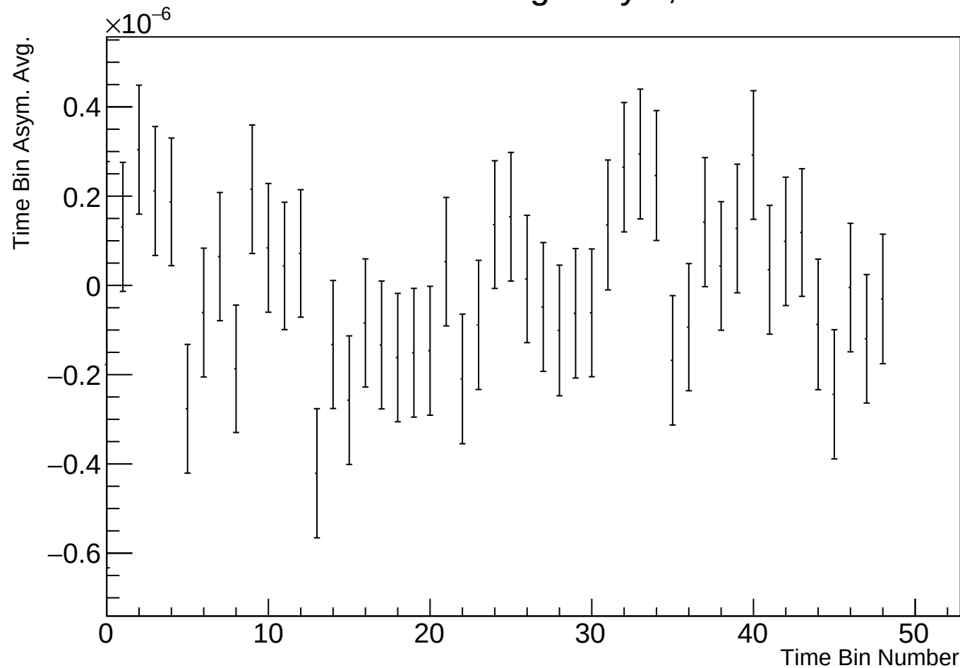
Time Bin Run Average Asym, r17784 w2
