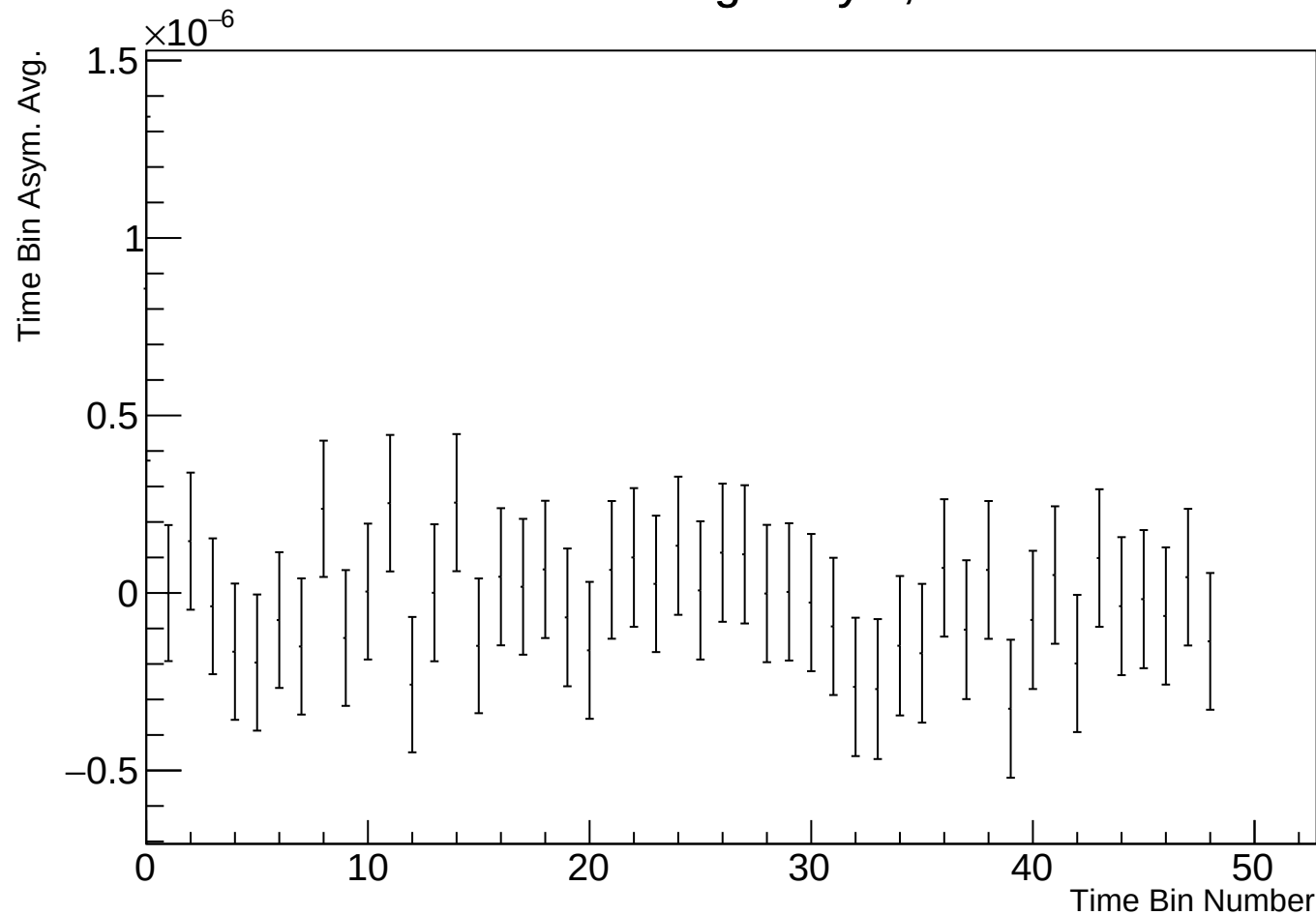
Time Bin Run Average Asym, r17784 w76
