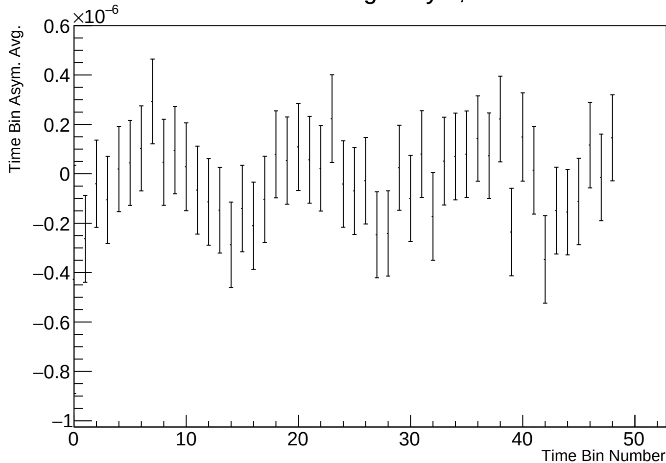
Time Bin Run Average Asym, r17784 w41
