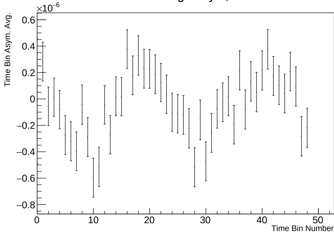
Time Bin Run Average Asym, r17784 w108
