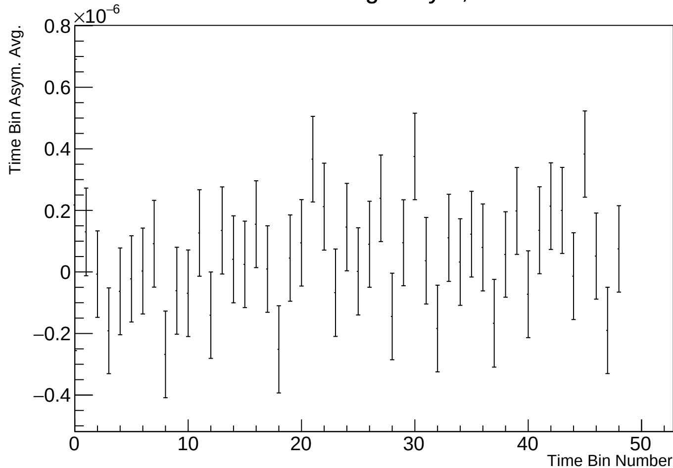
Time Bin Run Average Asym, r17784 w90
