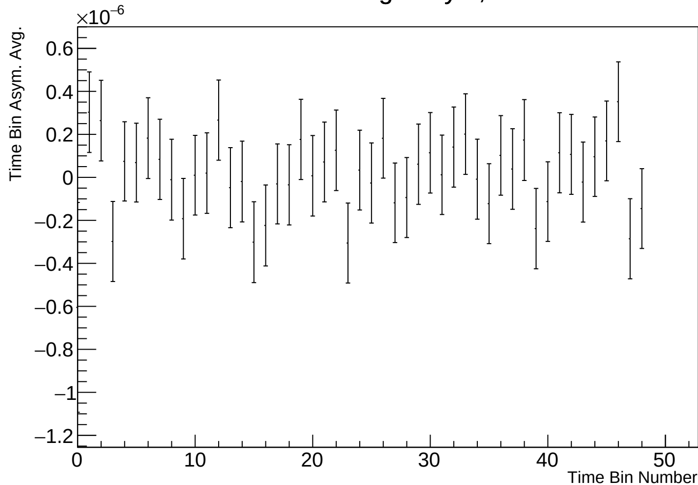
Time Bin Run Average Asym, r17784 w67
