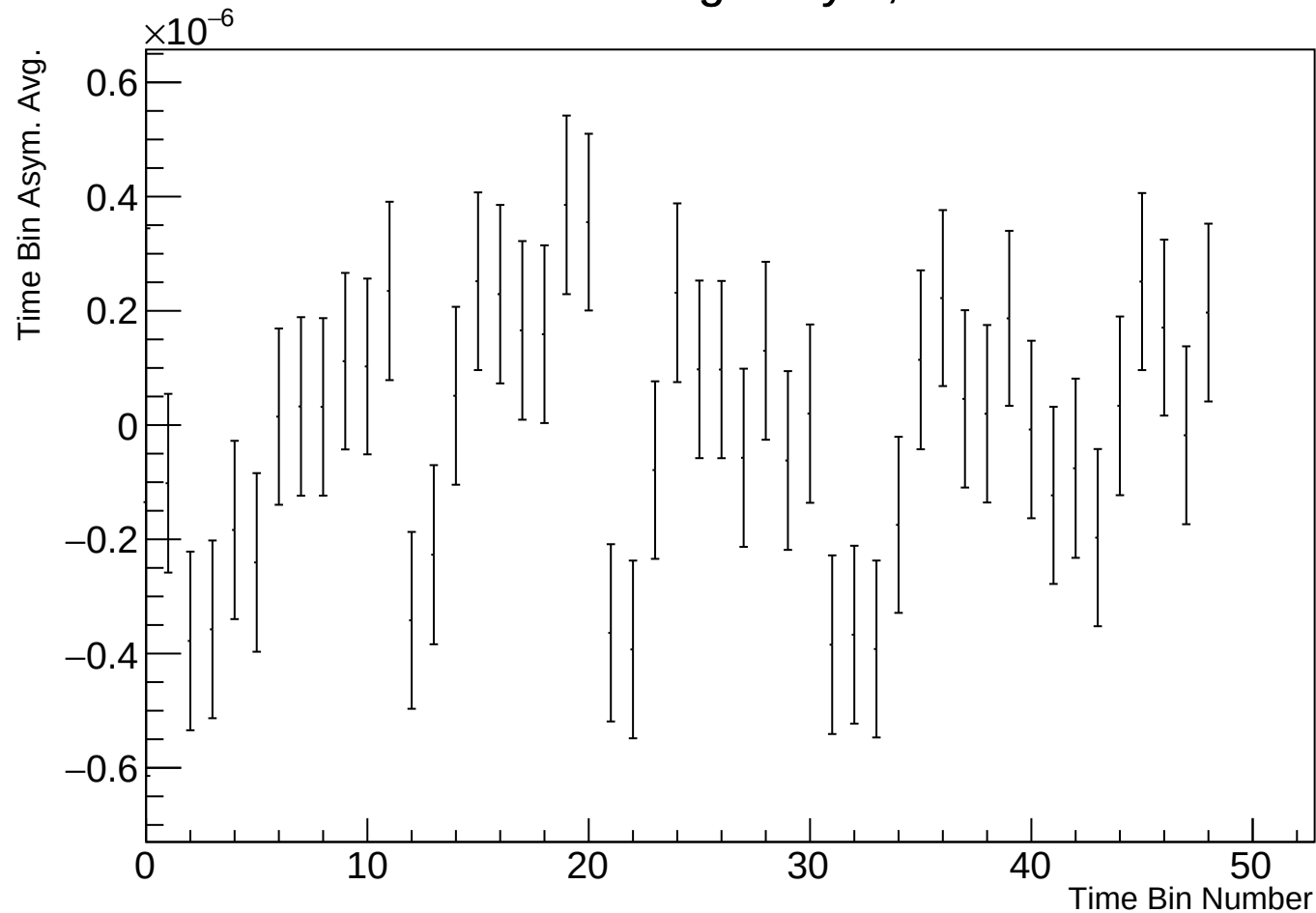
Time Bin Run Average Asym, r17784 w119
