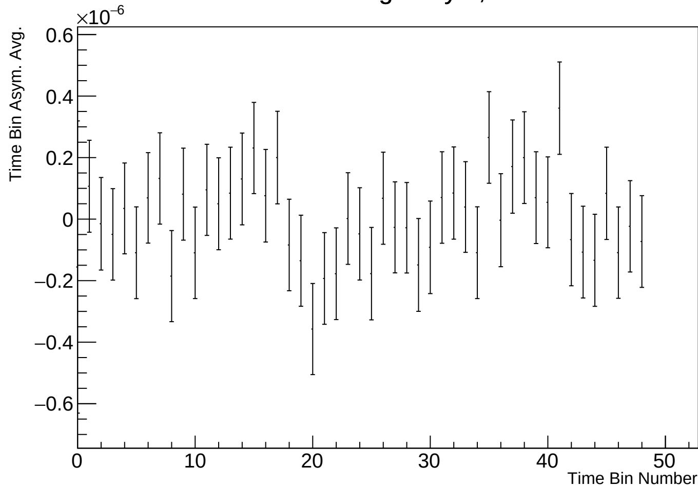
Time Bin Run Average Asym, r17784 w72
