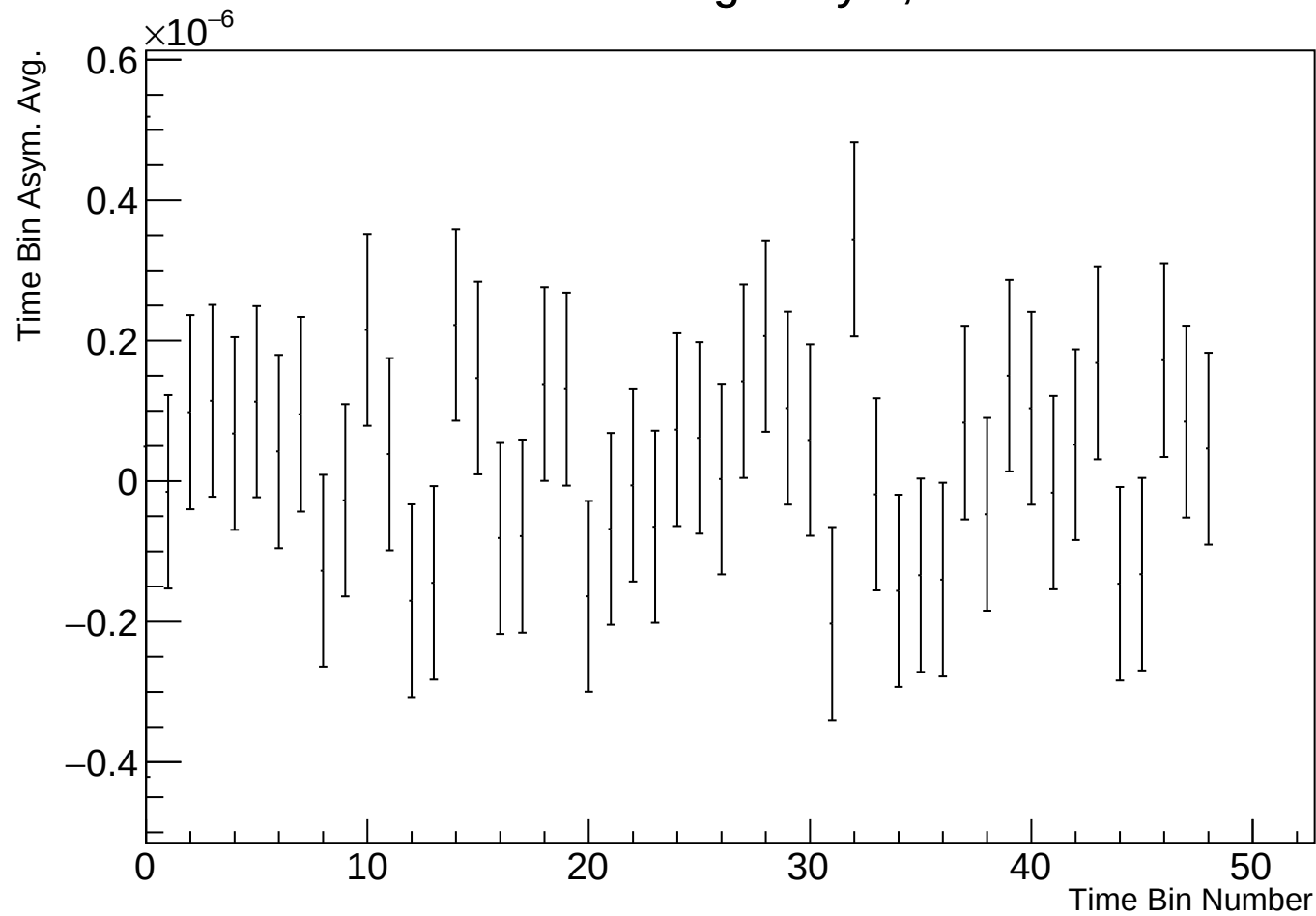
Time Bin Run Average Asym, r17784 w17
