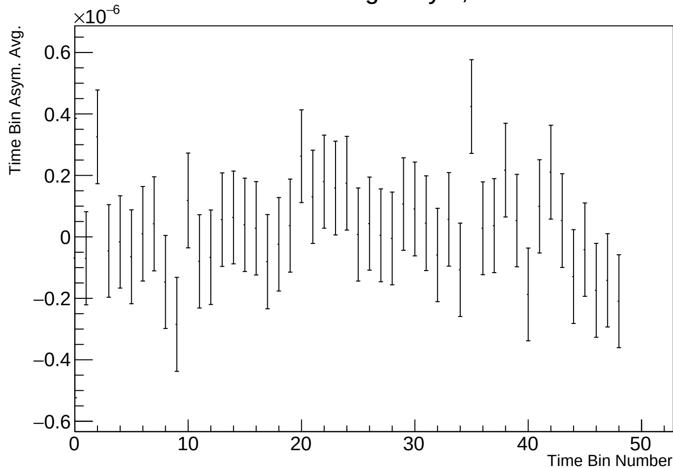
Time Bin Run Average Asym, r17784 w19
