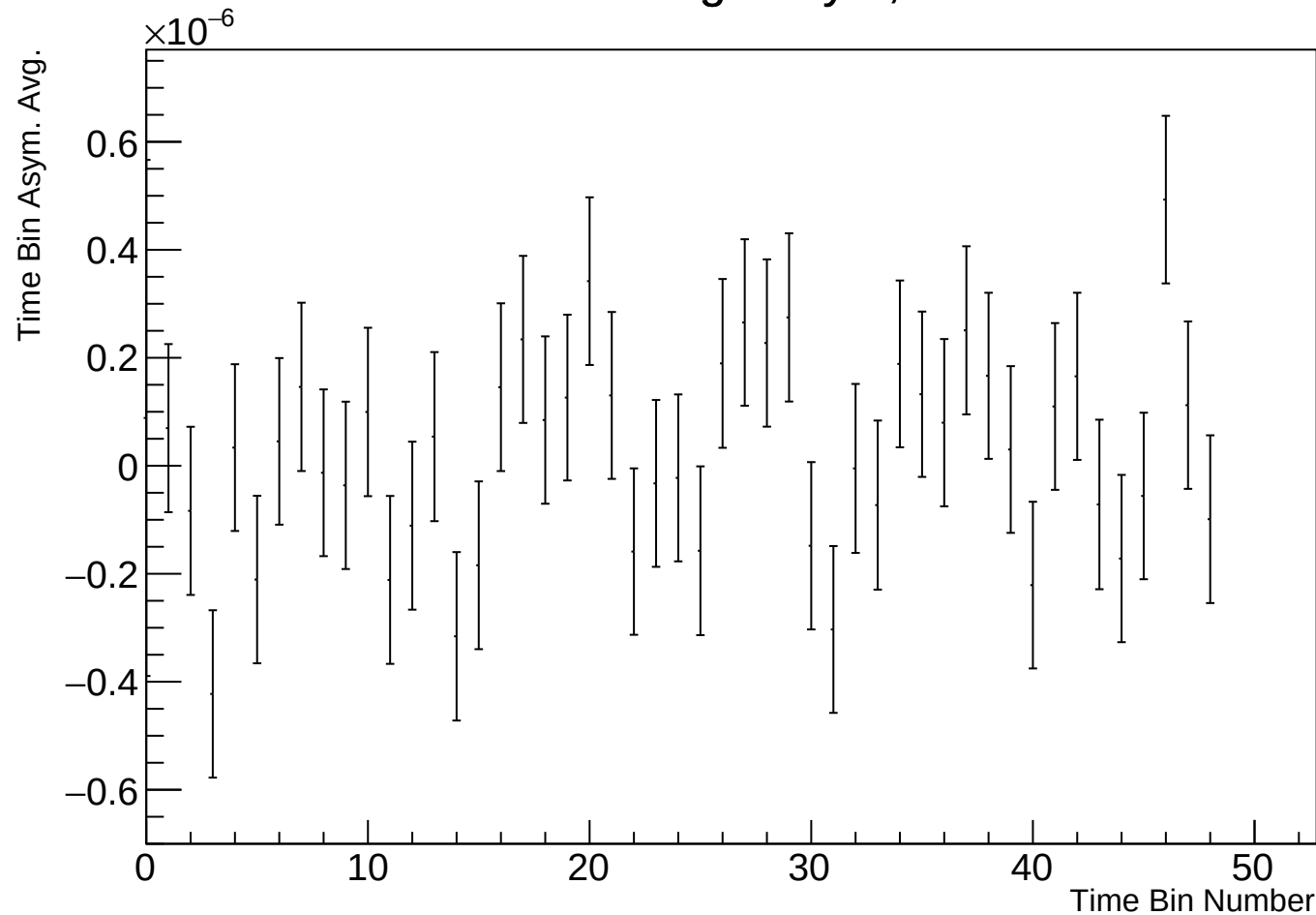
Time Bin Run Average Asym, r17784 w120
