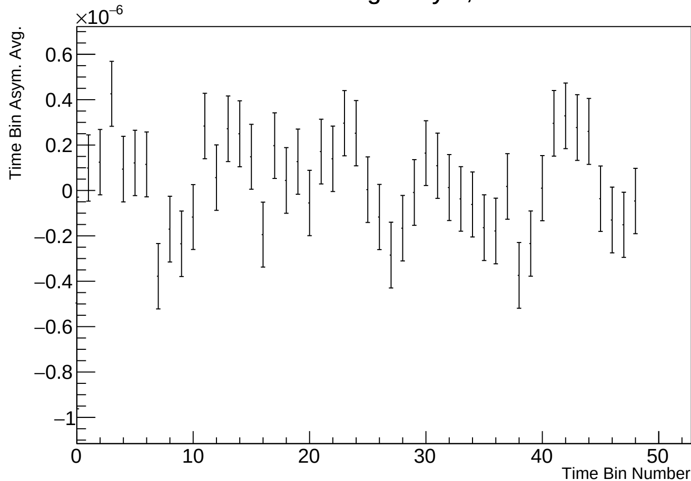
Time Bin Run Average Asym, r17784 w112
