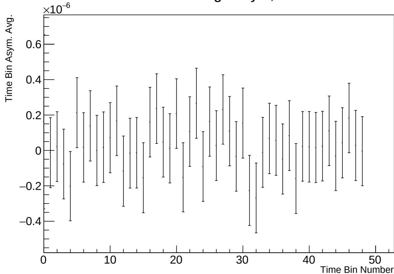
Time Bin Run Average Asym, r17784 w78
