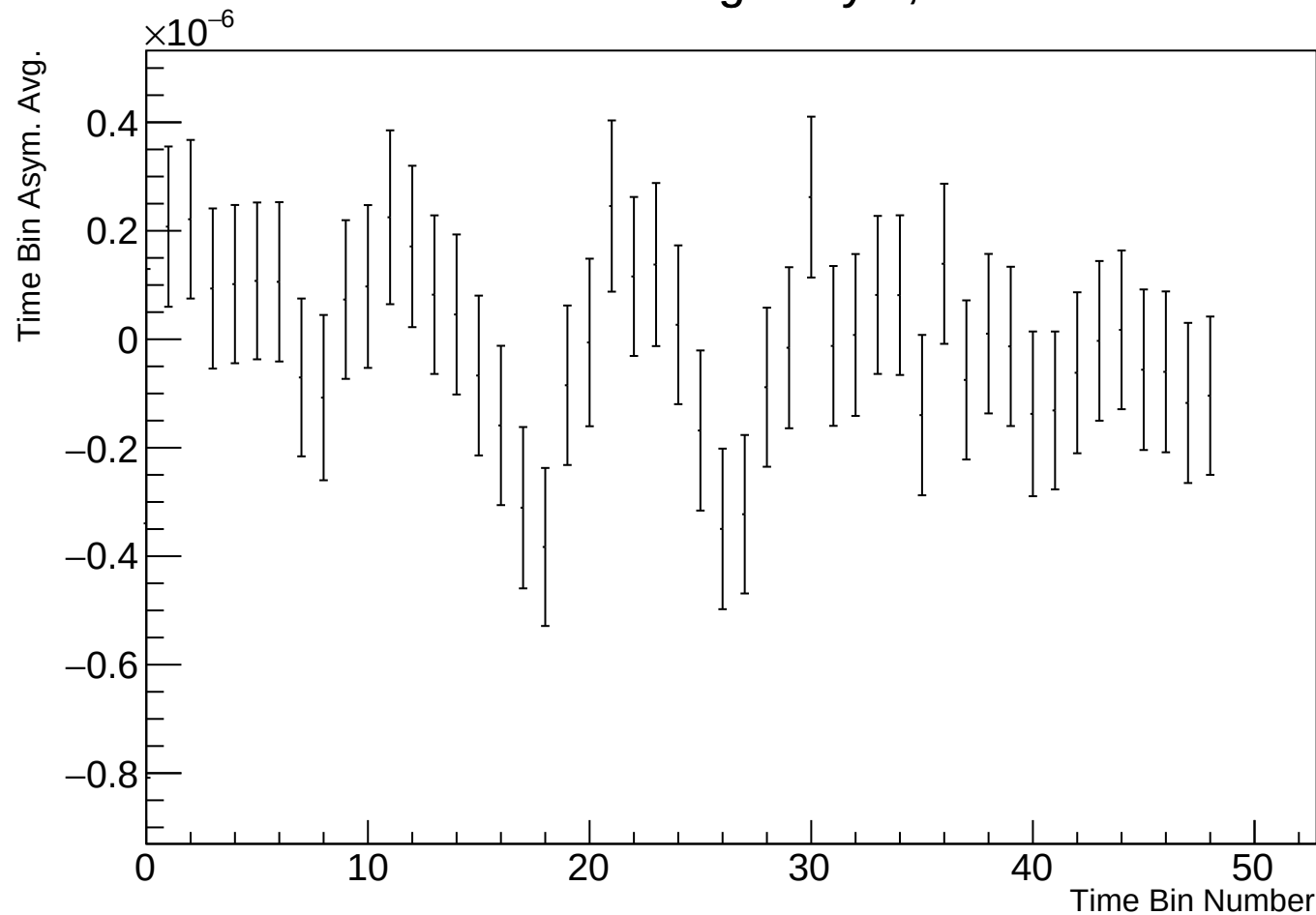
Time Bin Run Average Asym, r17784 w31
