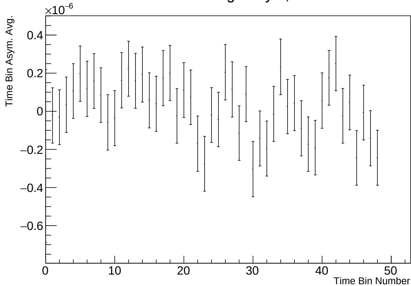
Time Bin Run Average Asym, r17784 w0
