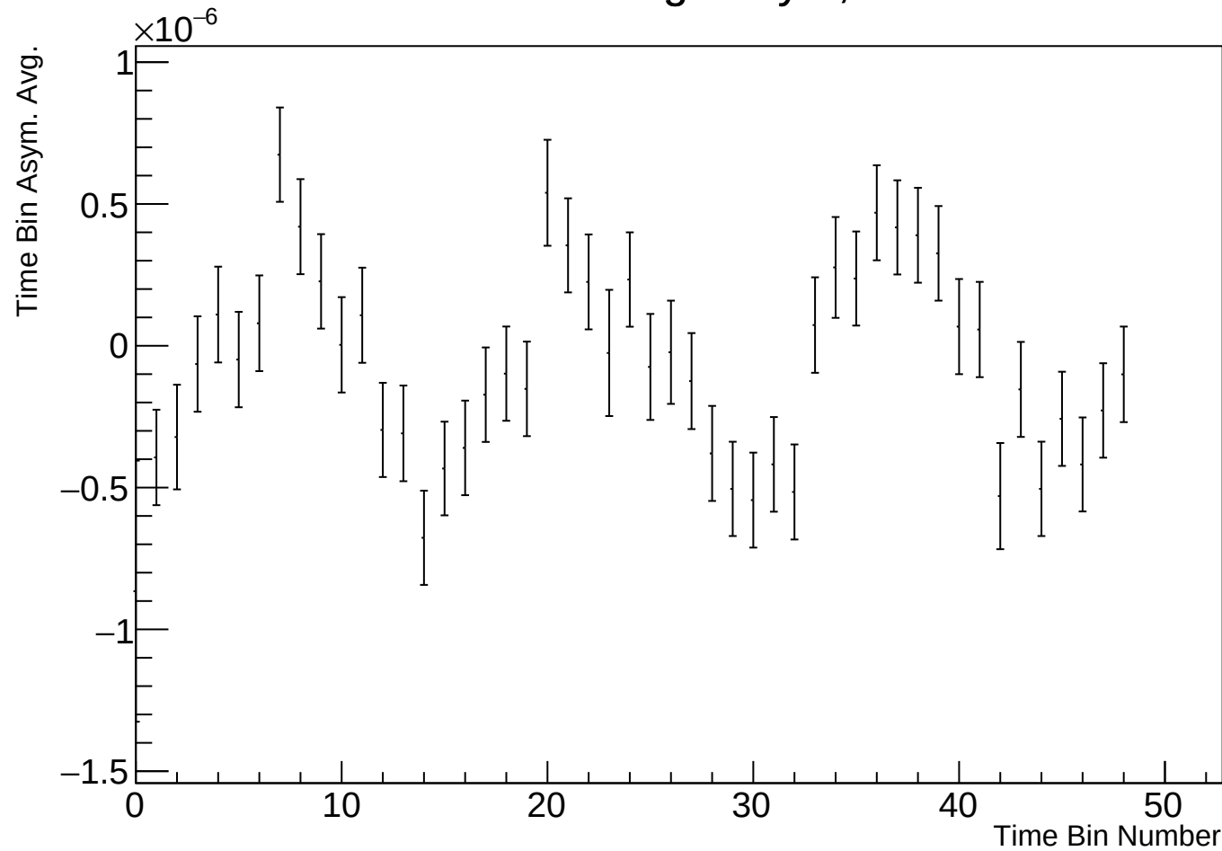
Time Bin Run Average Asym, r17784 w40
