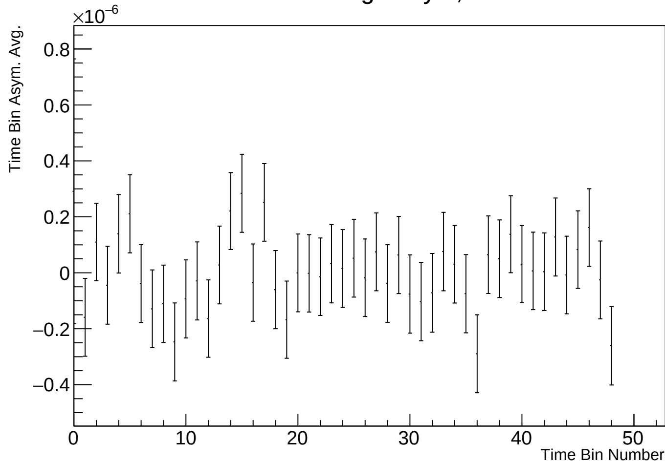
Time Bin Run Average Asym, r17784 w86
