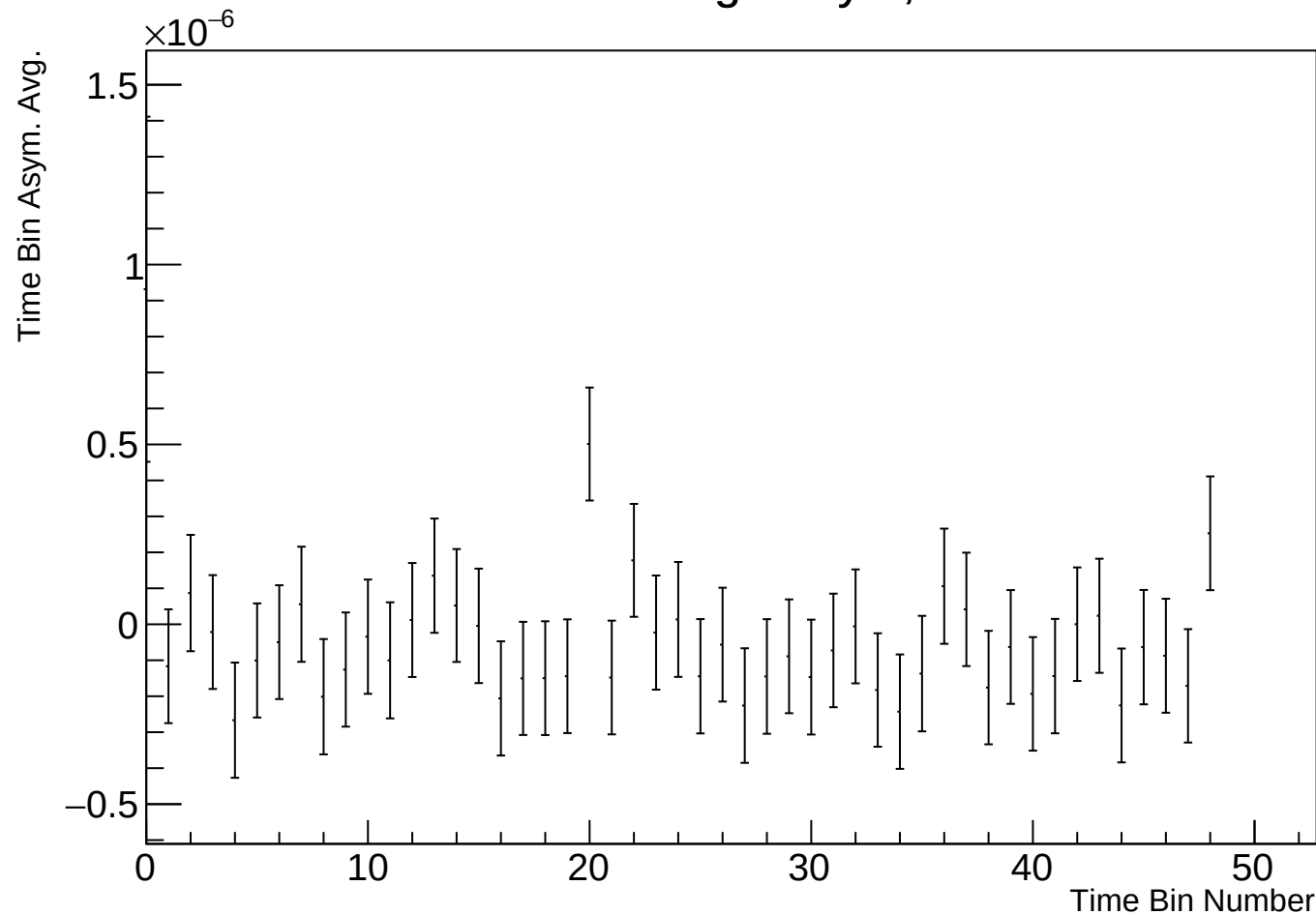
Time Bin Run Average Asym, r17784 w95
