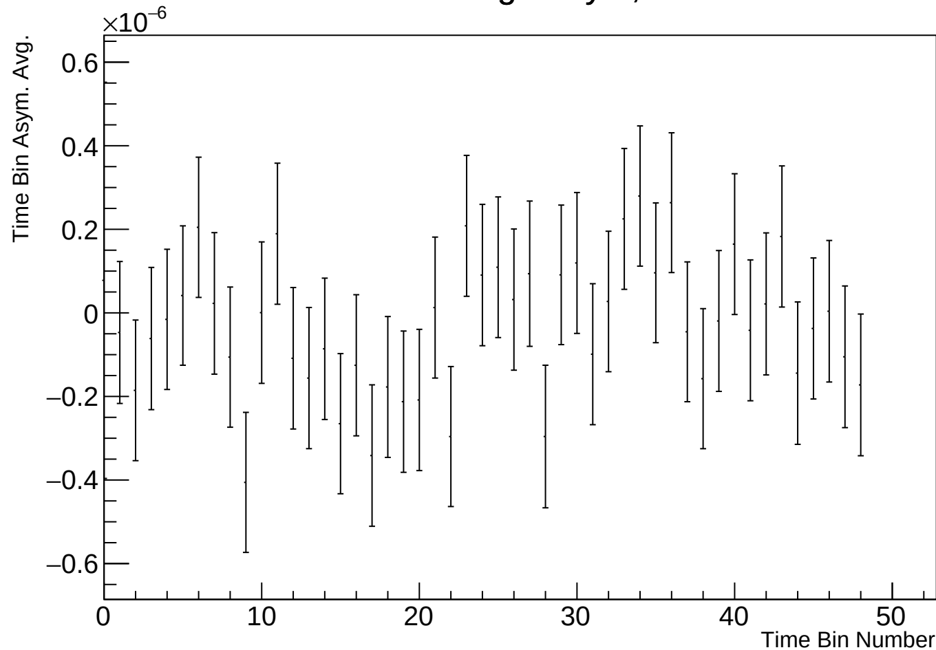
Time Bin Run Average Asym, r17784 w142
