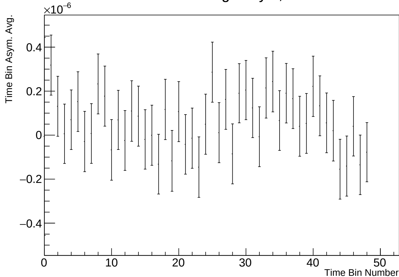
Time Bin Run Average Asym, r17784 w1
