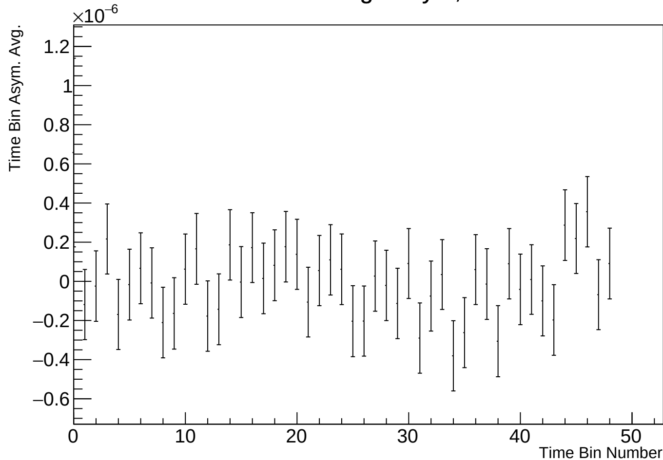
Time Bin Run Average Asym, r17784 w45
