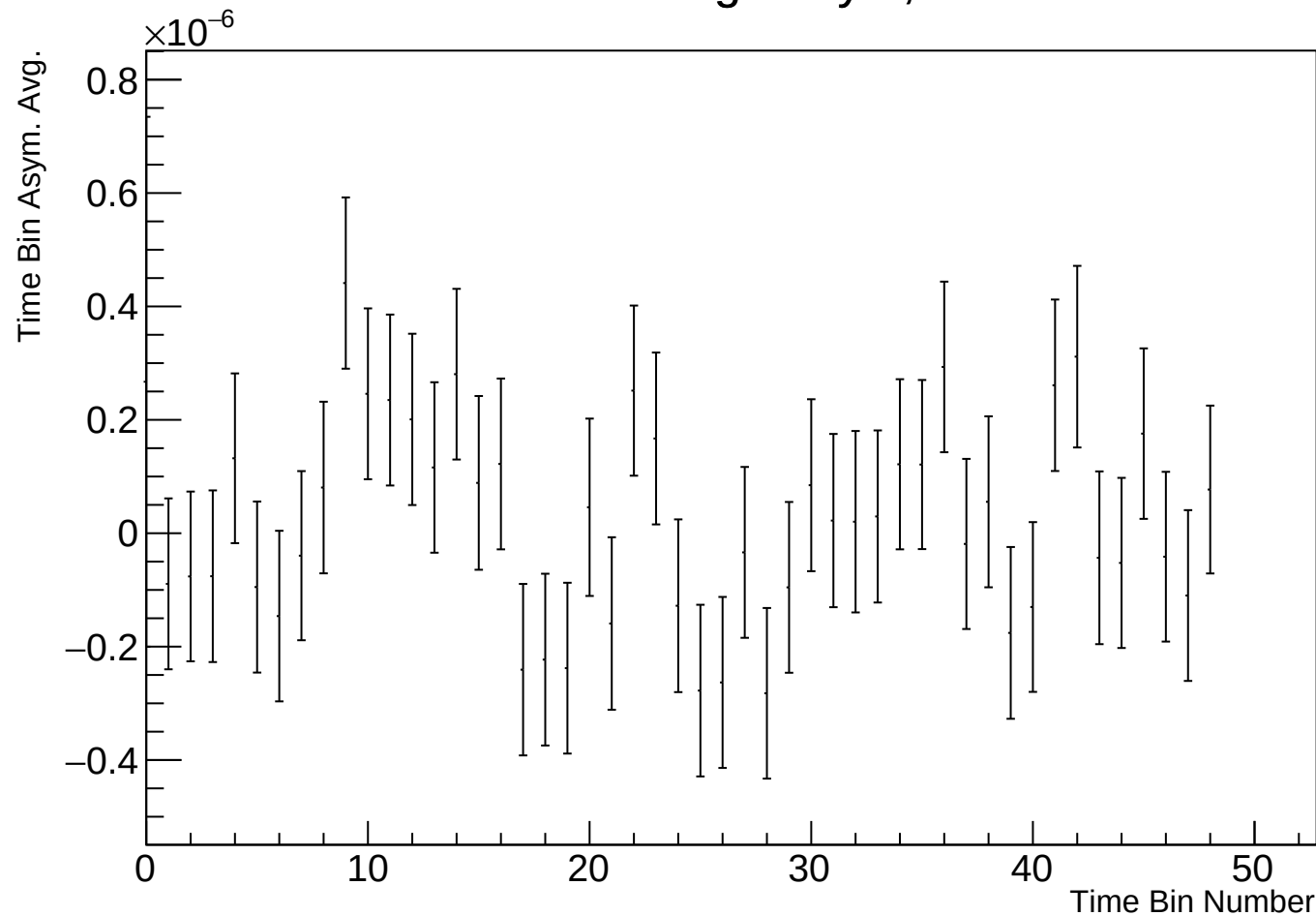
Time Bin Run Average Asym, r17784 w27
