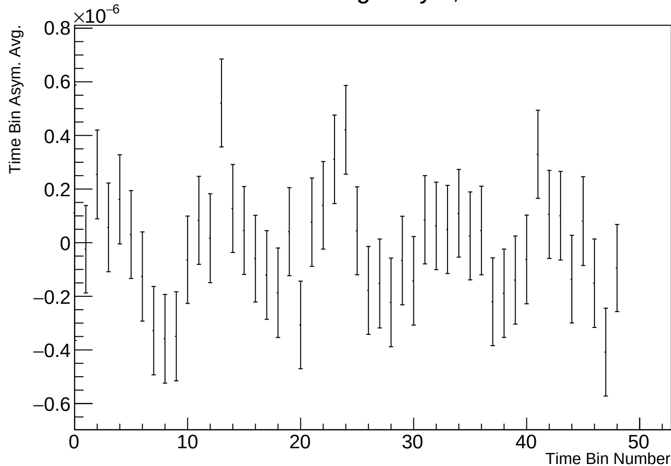
Time Bin Run Average Asym, r17784 w114
