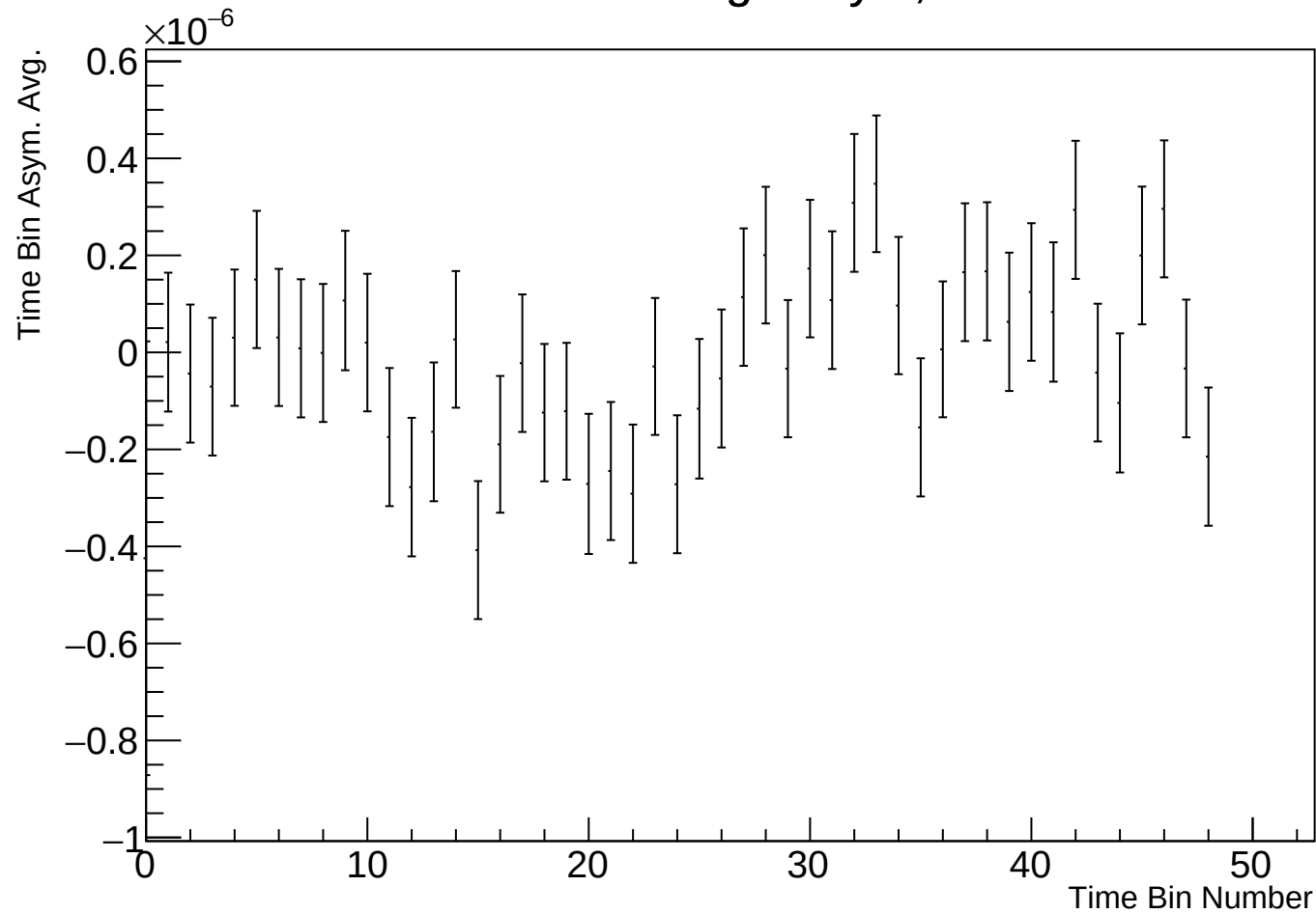
Time Bin Run Average Asym, r17784 w4
