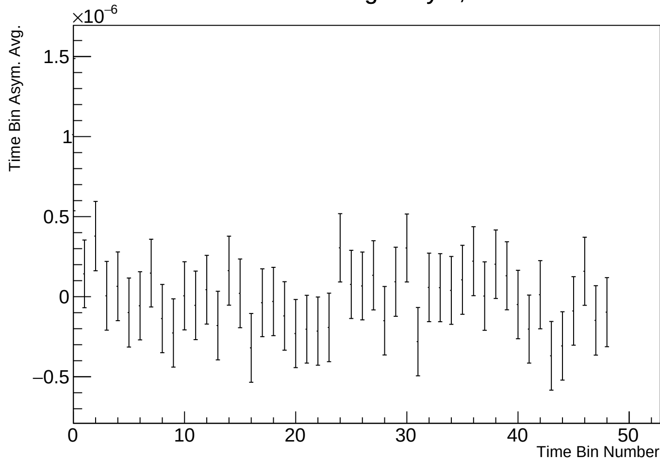
Time Bin Run Average Asym, r17784 w6
