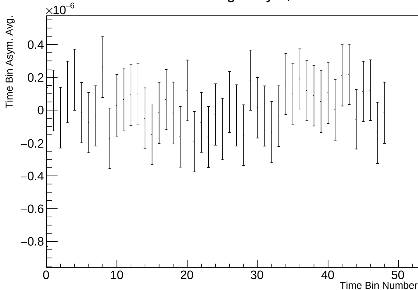
Time Bin Run Average Asym, r17784 w66
