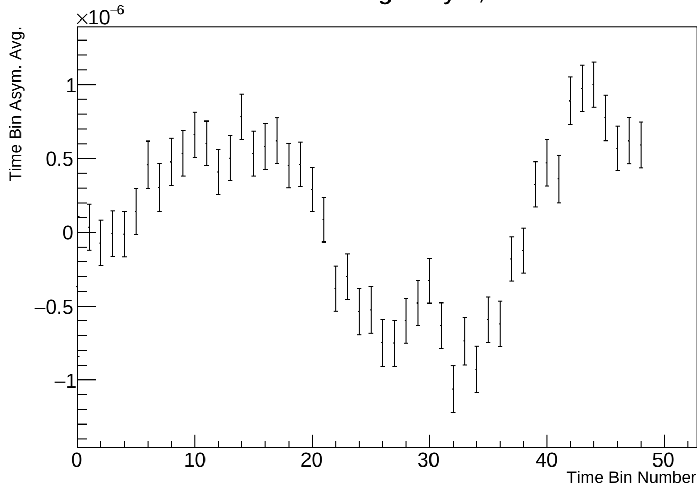
Time Bin Run Average Asym, r17784 w98
