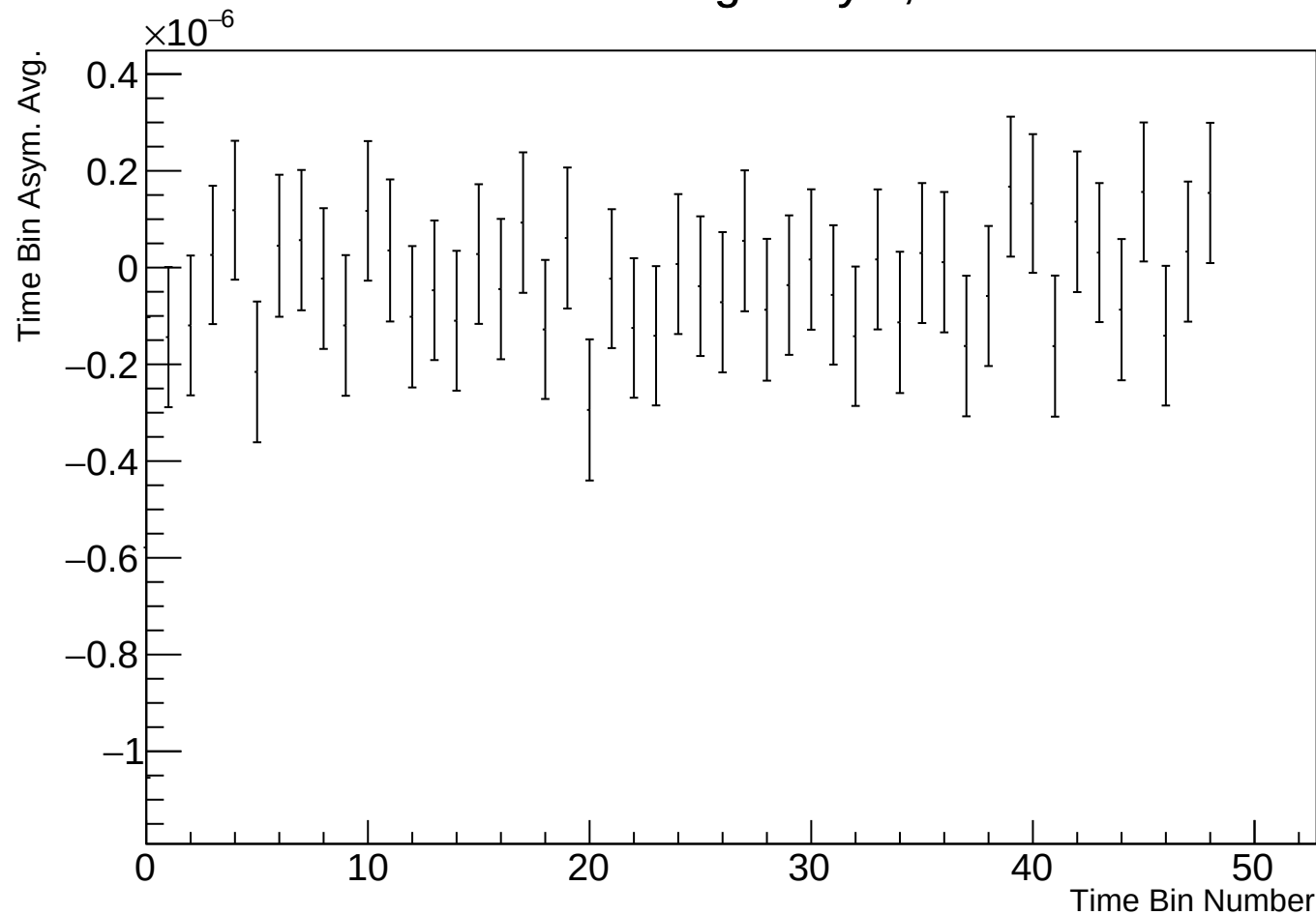
Time Bin Run Average Asym, r17784 w85
