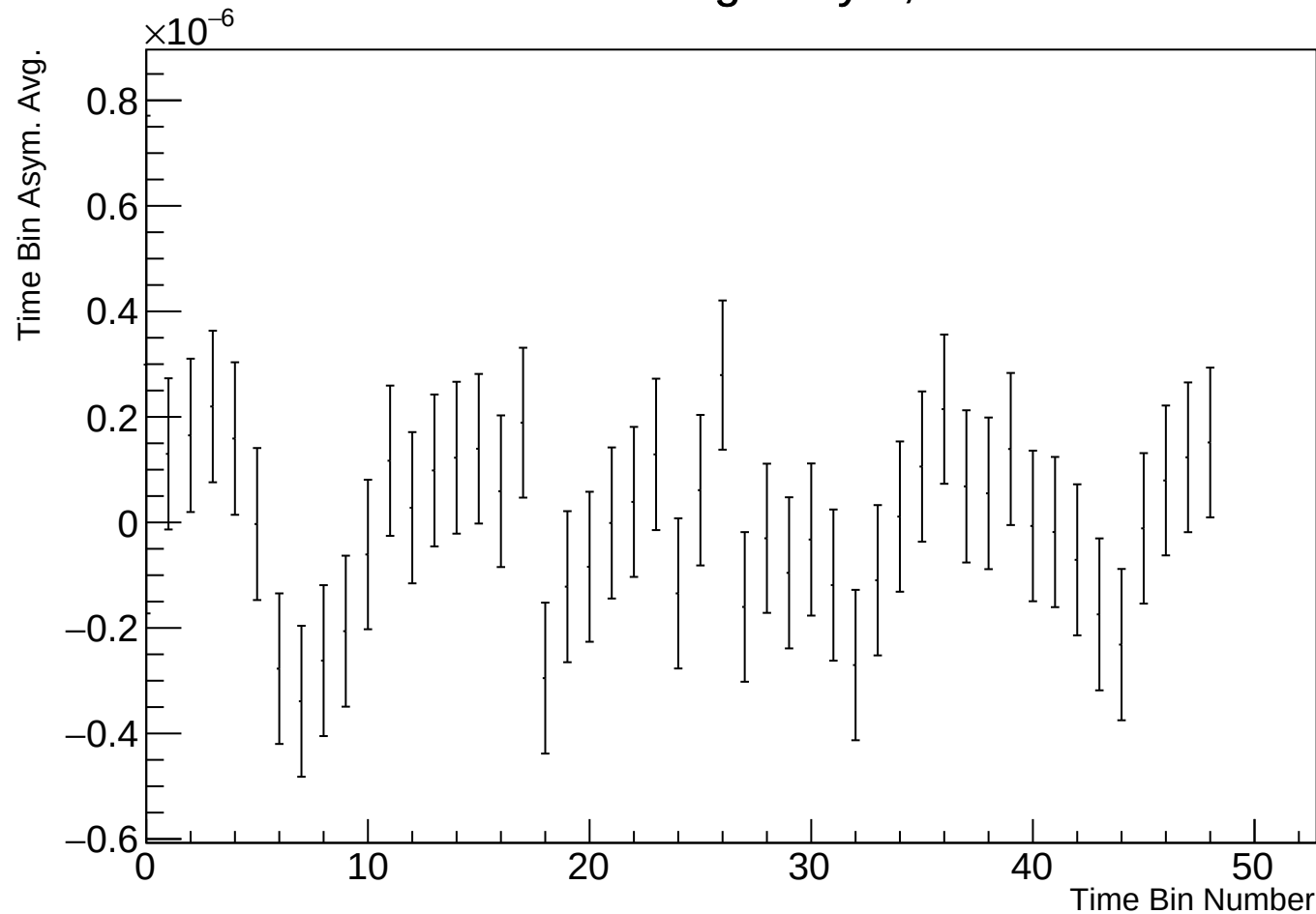
Time Bin Run Average Asym, r17784 w33
