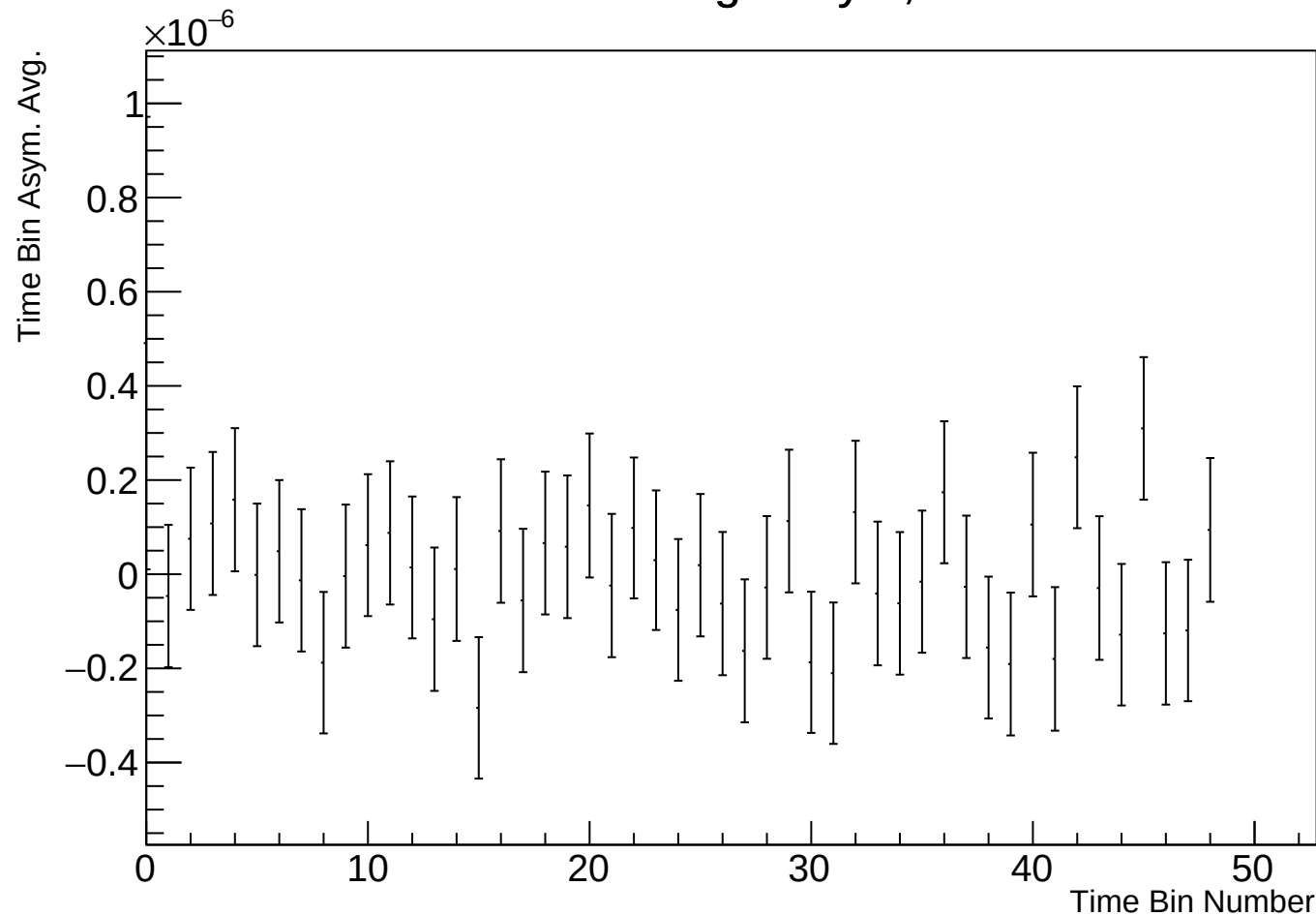
Time Bin Run Average Asym, r17784 w73
