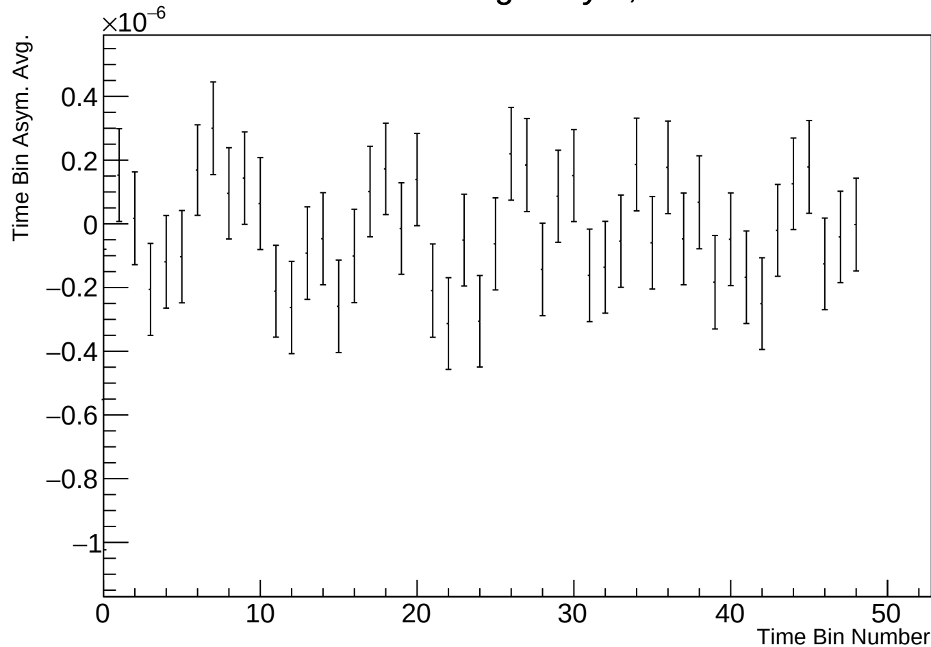
Time Bin Run Average Asym, r17784 w118
