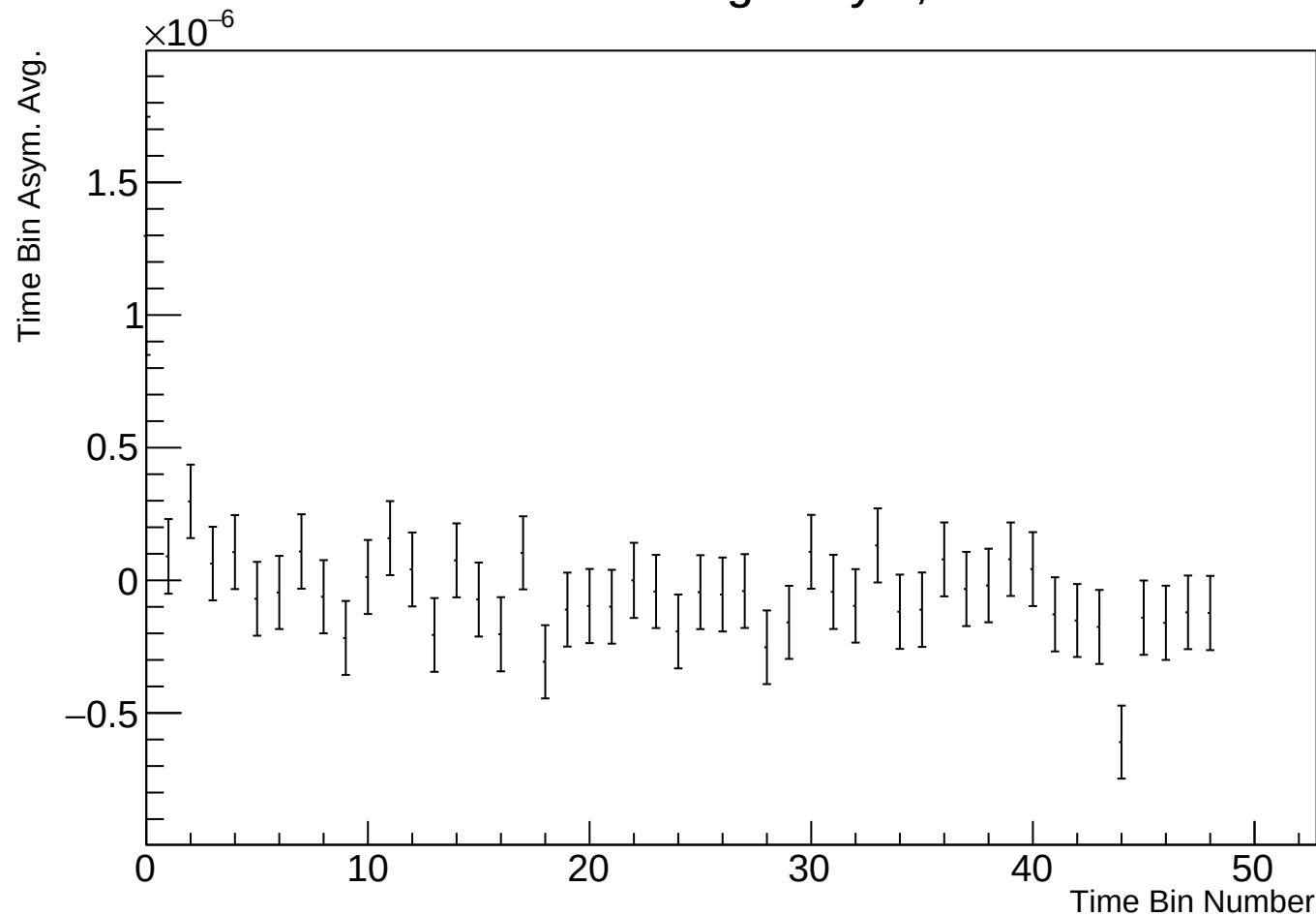
Time Bin Run Average Asym, r17784 w3
