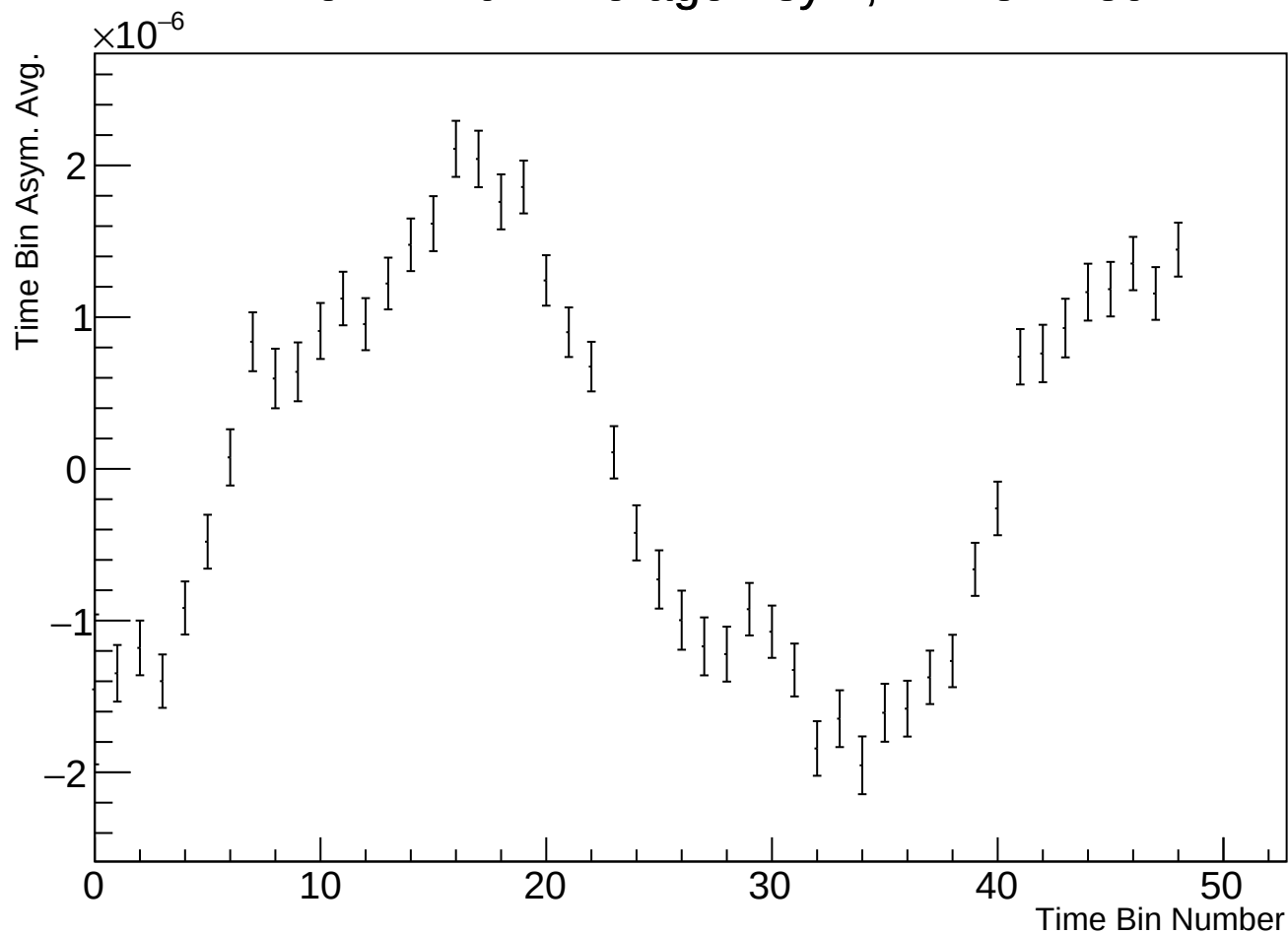
Time Bin Run Average Asym, r17784 w89
