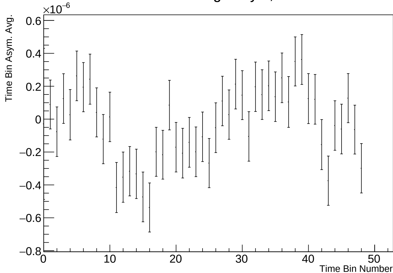
Time Bin Run Average Asym, r17784 w44
