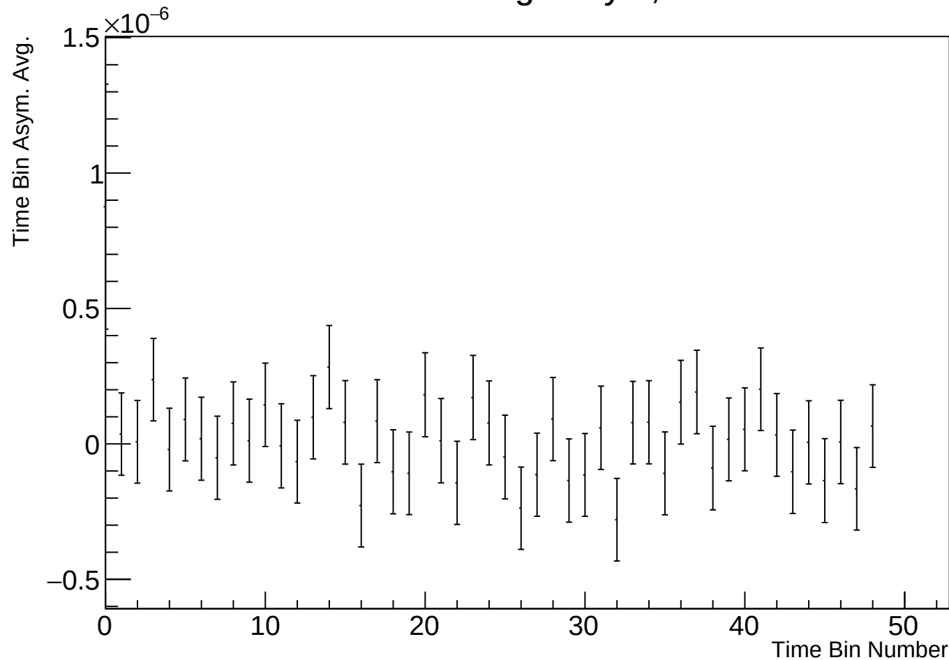
Time Bin Run Average Asym, r17784 w23
