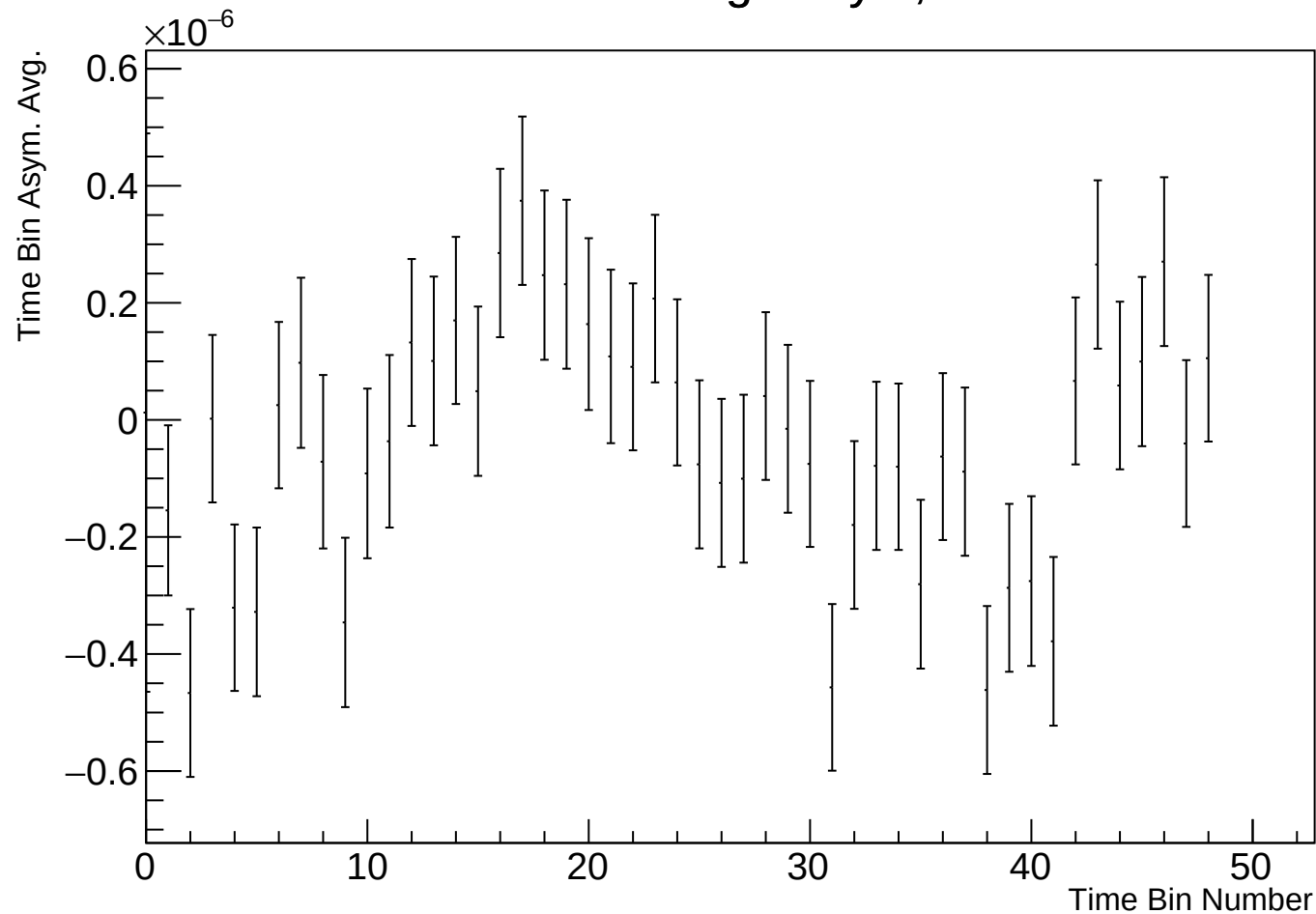
Time Bin Run Average Asym, r17784 w9
