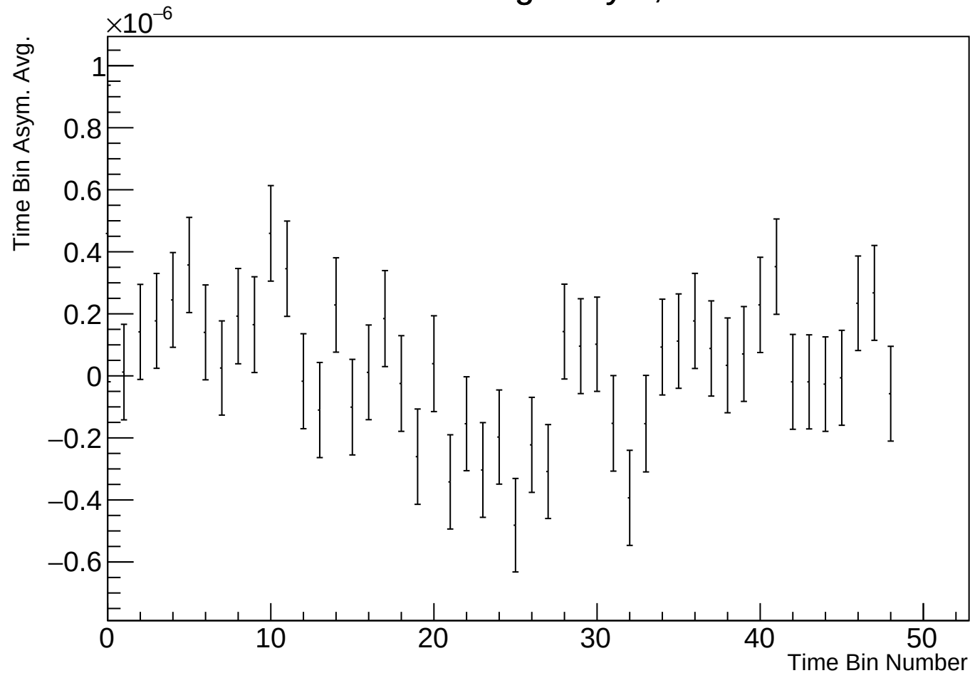
Time Bin Run Average Asym, r17784 w106
