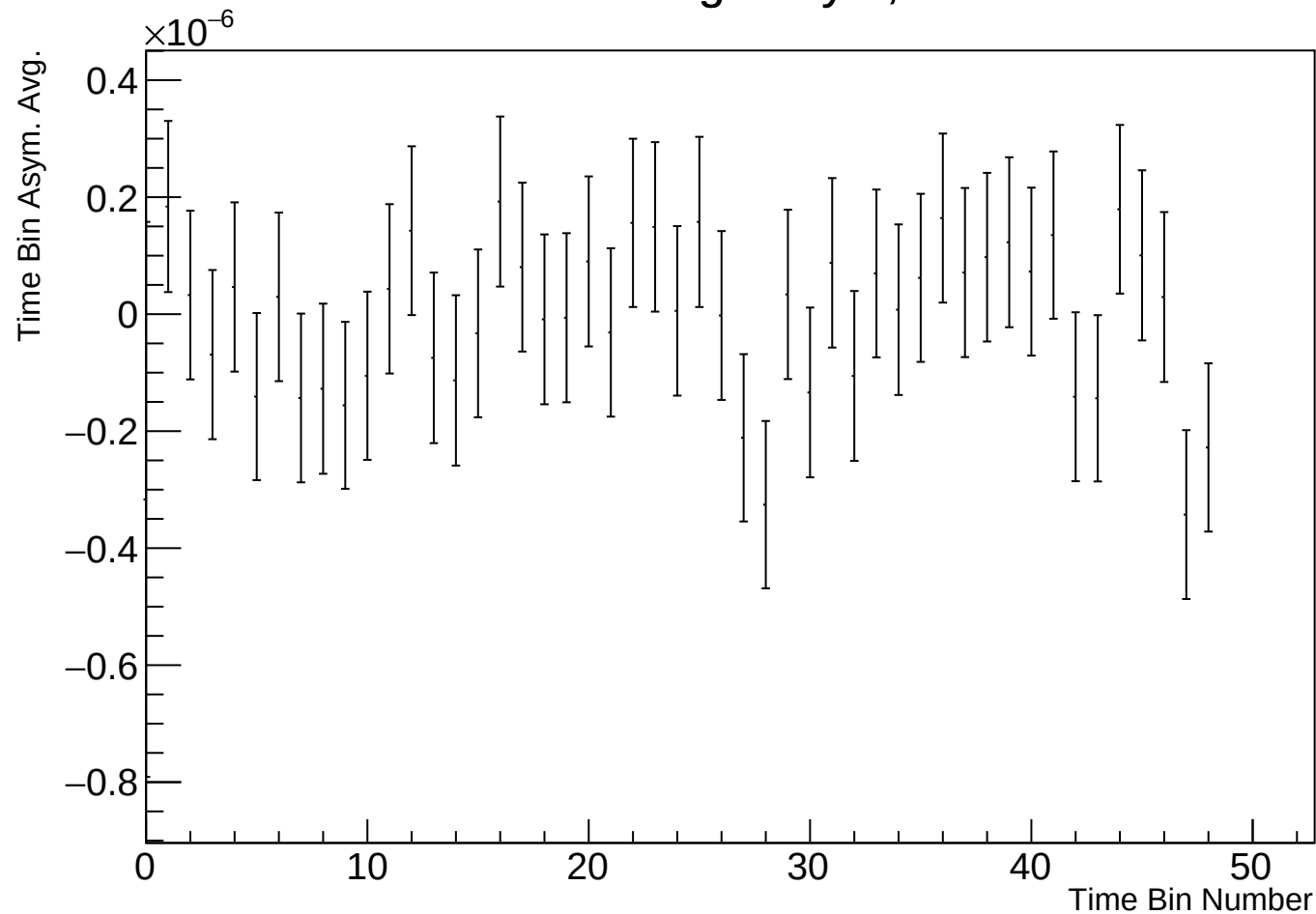
Time Bin Run Average Asym, r17784 w136
