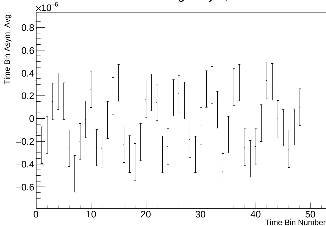
Time Bin Run Average Asym, r17784 w61
