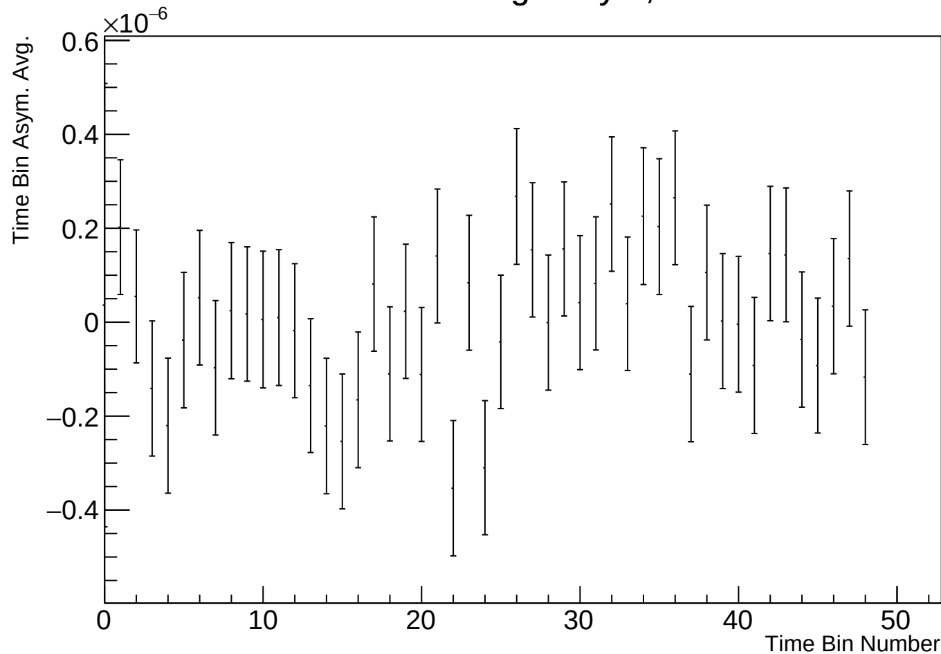
Time Bin Run Average Asym, r17784 w53
