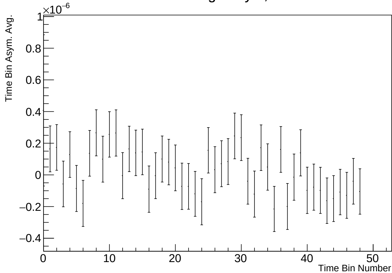
Time Bin Run Average Asym, r17784 w103
