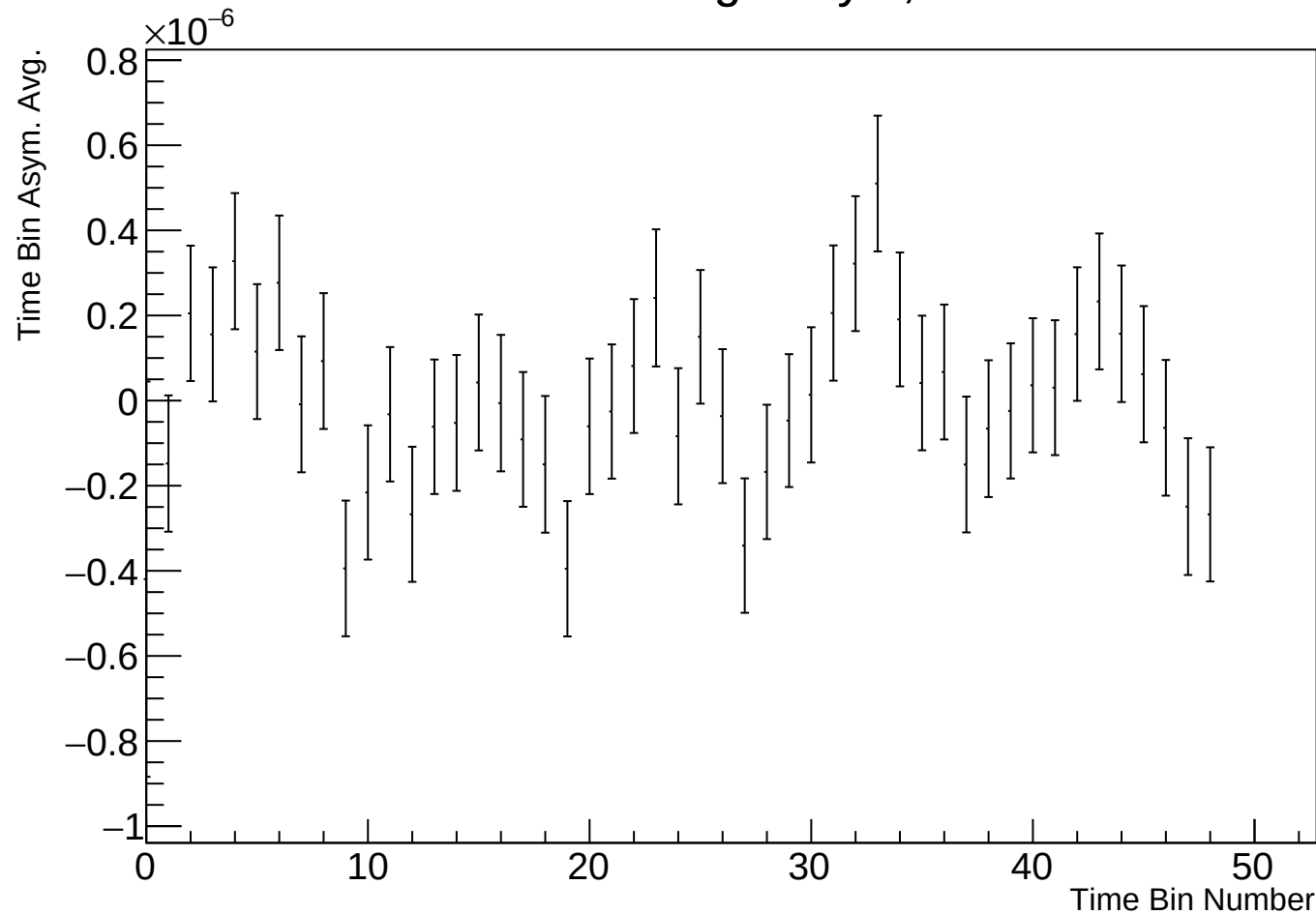
Time Bin Run Average Asym, r17784 w59
