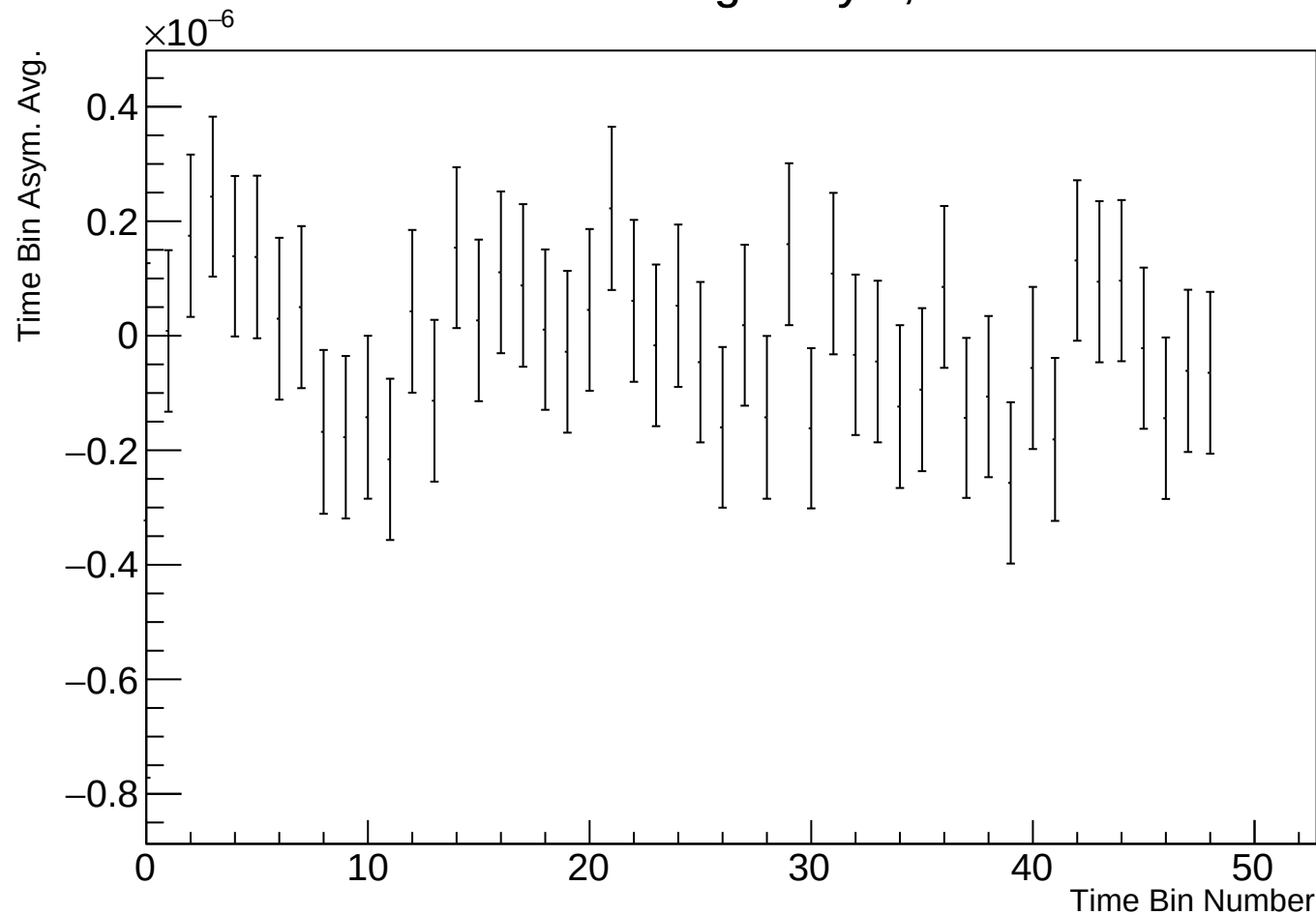
Time Bin Run Average Asym, r17784 w62
