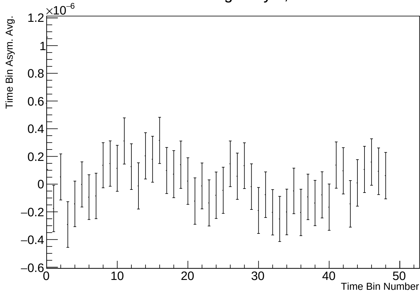
Time Bin Run Average Asym, r17784 w141
