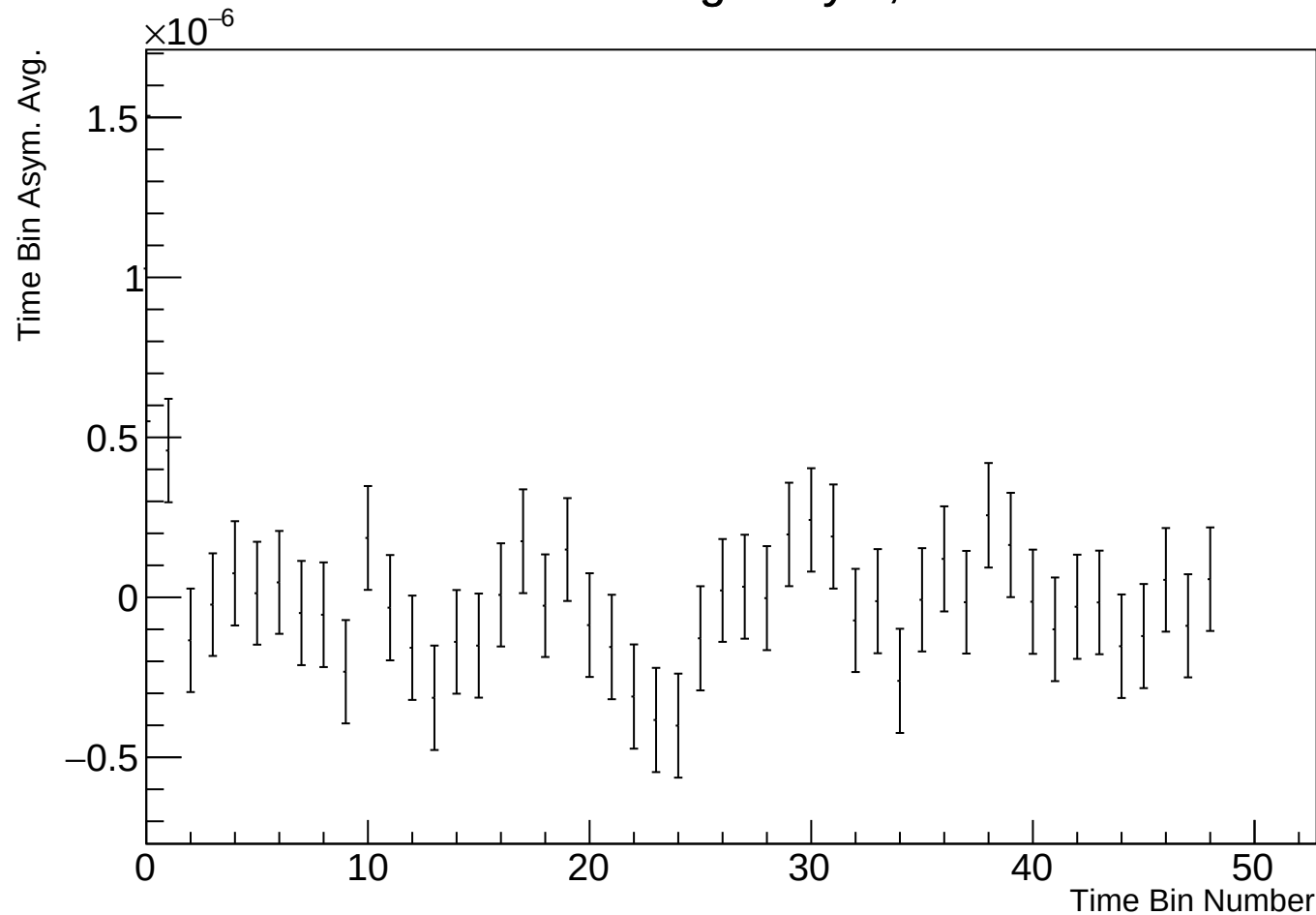
Time Bin Run Average Asym, r17784 w102
