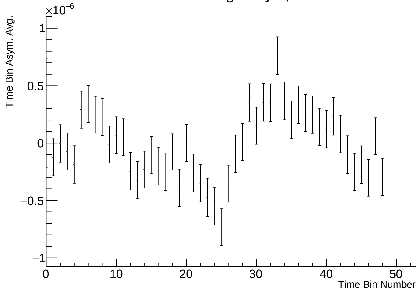
Time Bin Run Average Asym, r17784 w99
