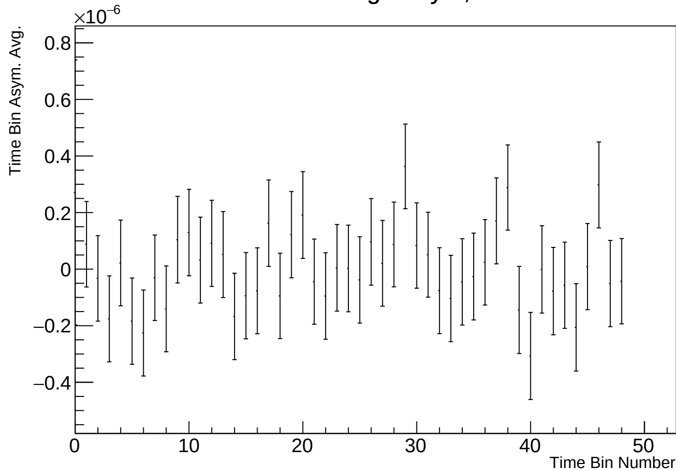
Time Bin Run Average Asym, r17784 w52
