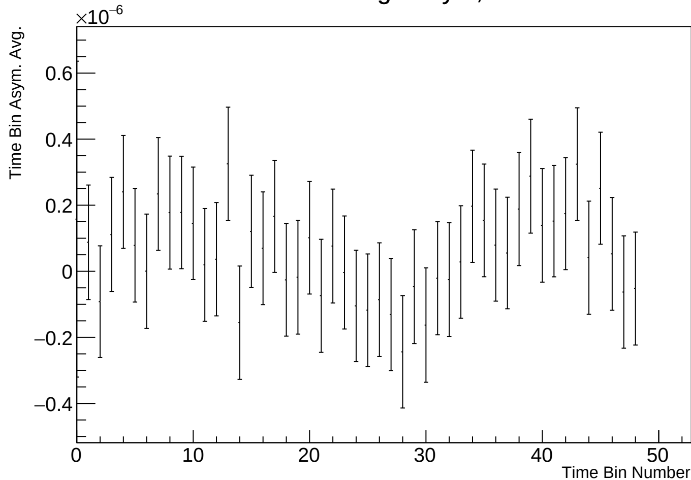
Time Bin Run Average Asym, r17784 w71
