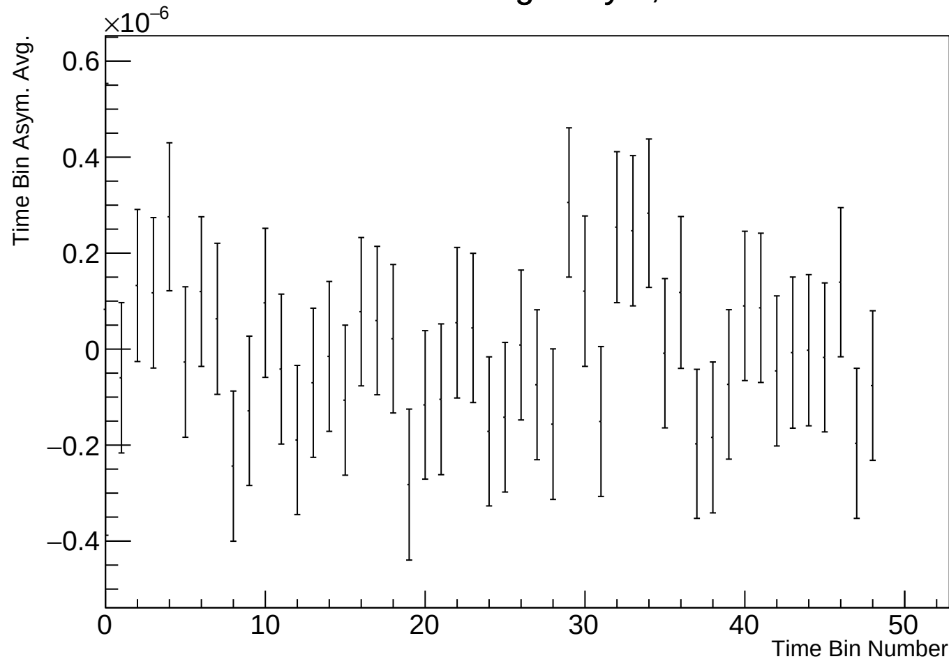
Time Bin Run Average Asym, r17784 w65
