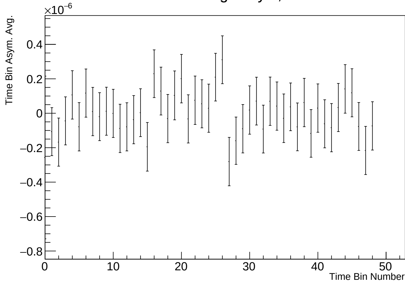
Time Bin Run Average Asym, r17784 w84
