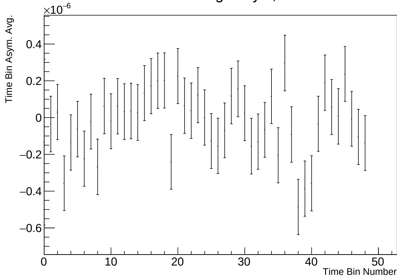
Time Bin Run Average Asym, r17784 w24
