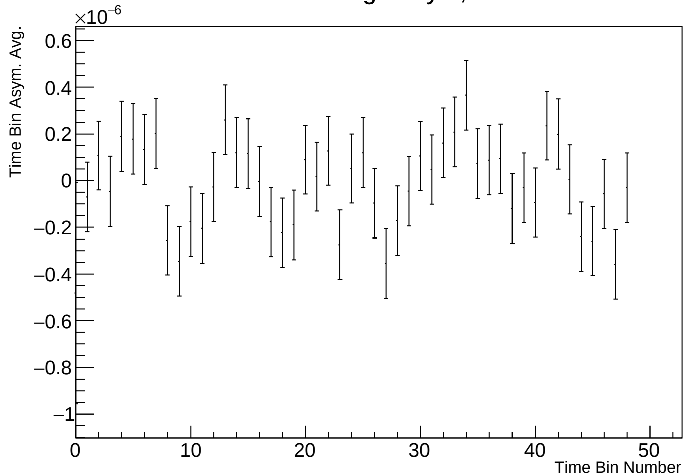
Time Bin Run Average Asym, r17784 w109
