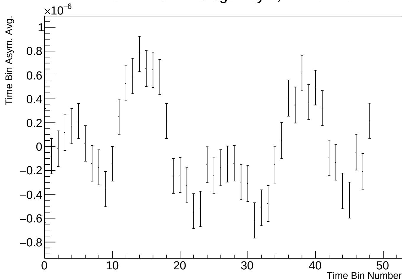
Time Bin Run Average Asym, r17784 w81
