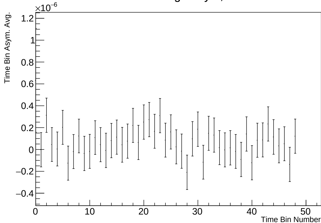
Time Bin Run Average Asym, r17784 w93
