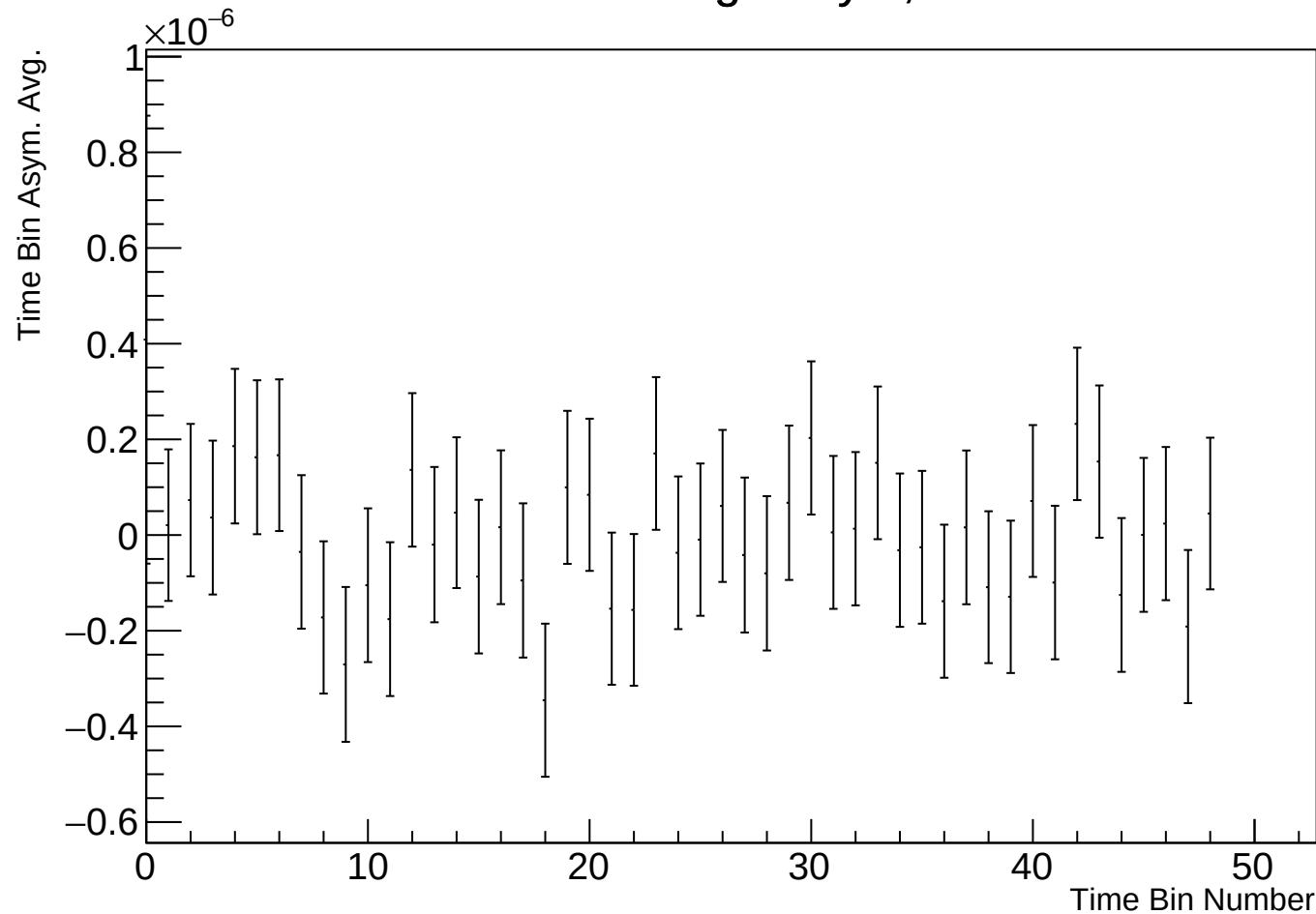
Time Bin Run Average Asym, r17784 w56
