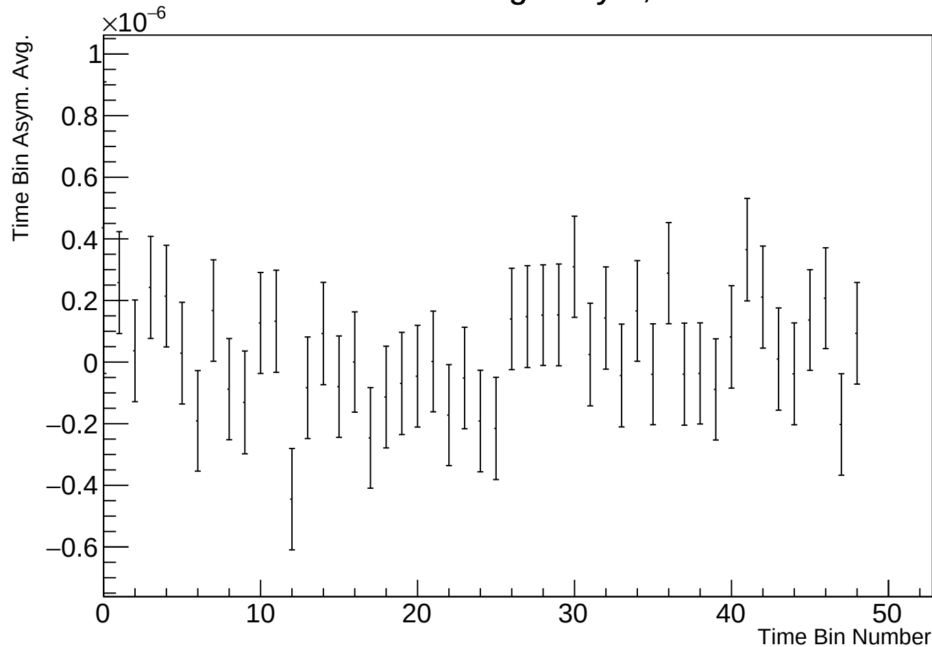
Time Bin Run Average Asym, r17784 w11
