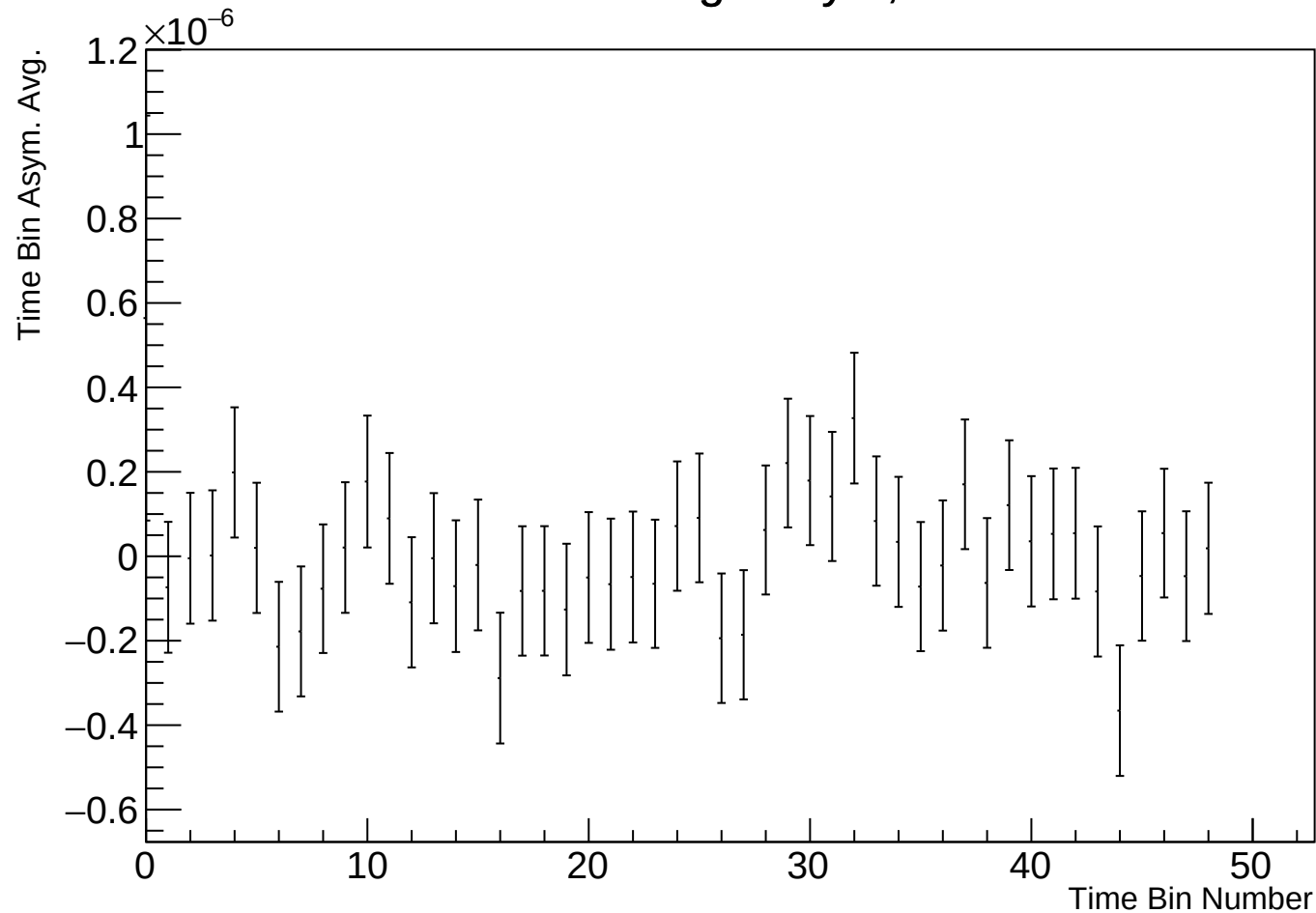
Time Bin Run Average Asym, r17784 w100
