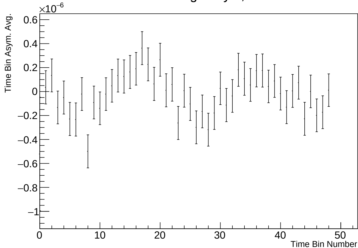
Time Bin Run Average Asym, r17784 w135
