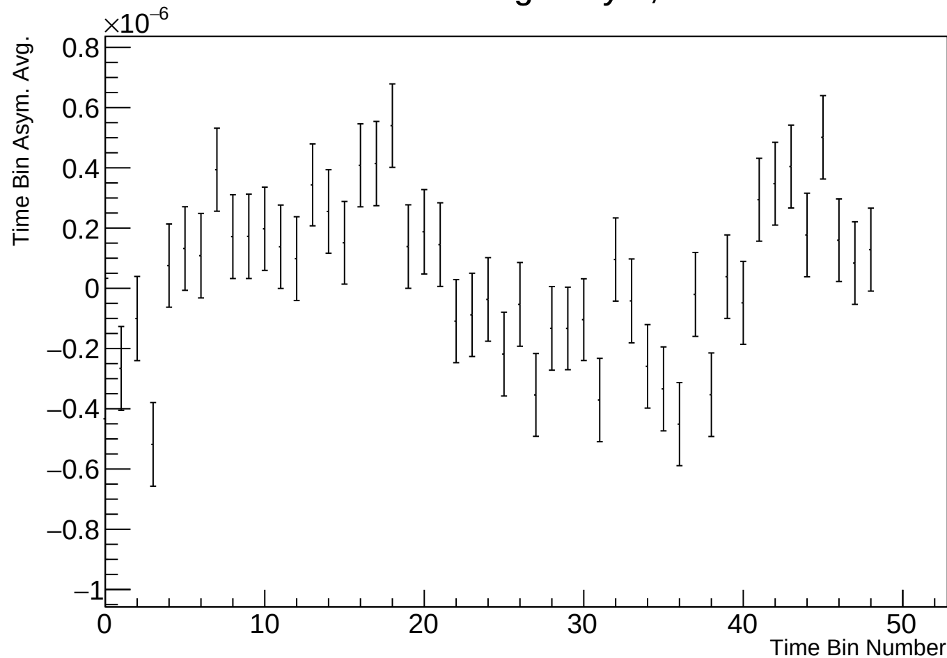
Time Bin Run Average Asym, r17784 w88
