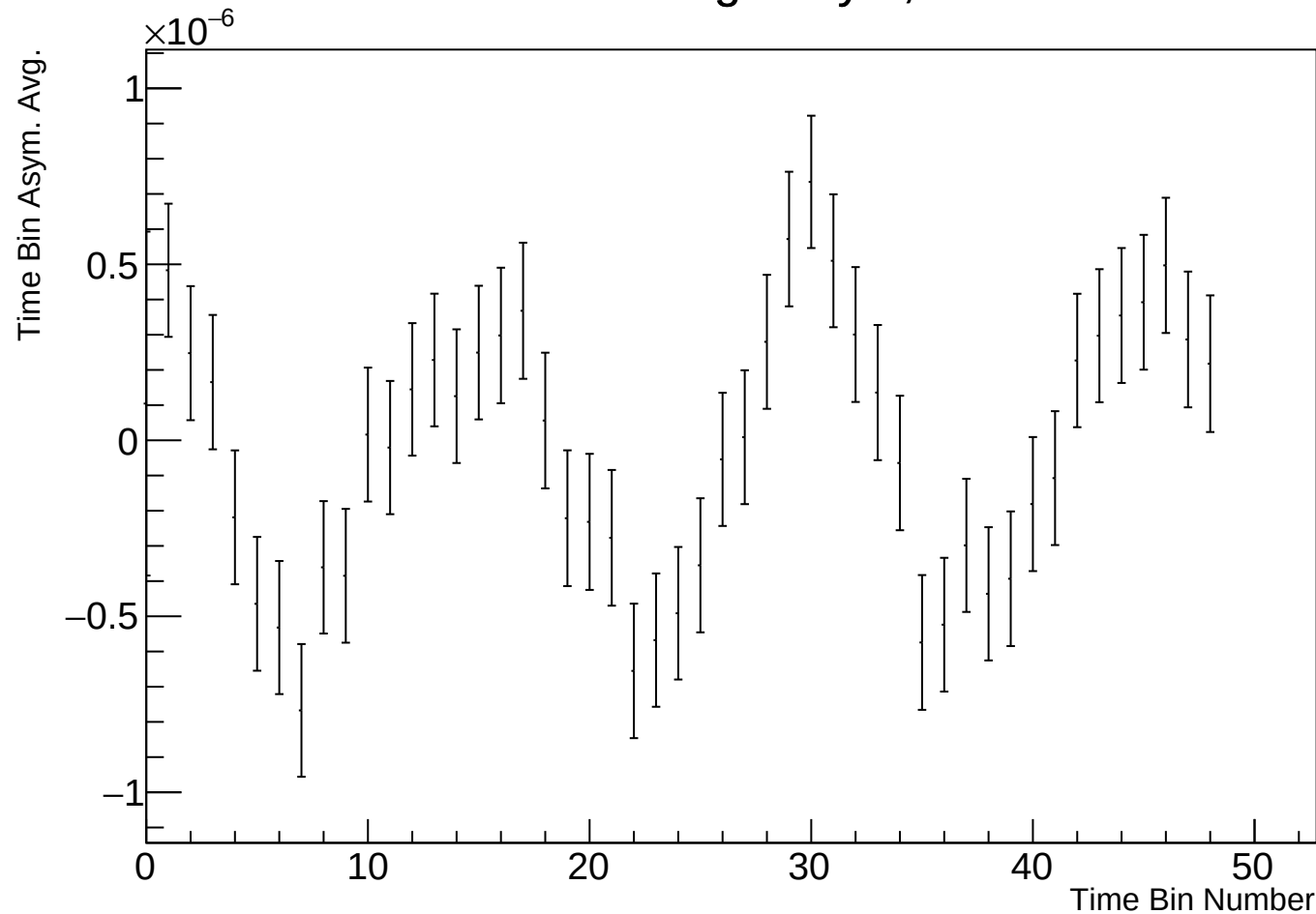
Time Bin Run Average Asym, r17784 w48
