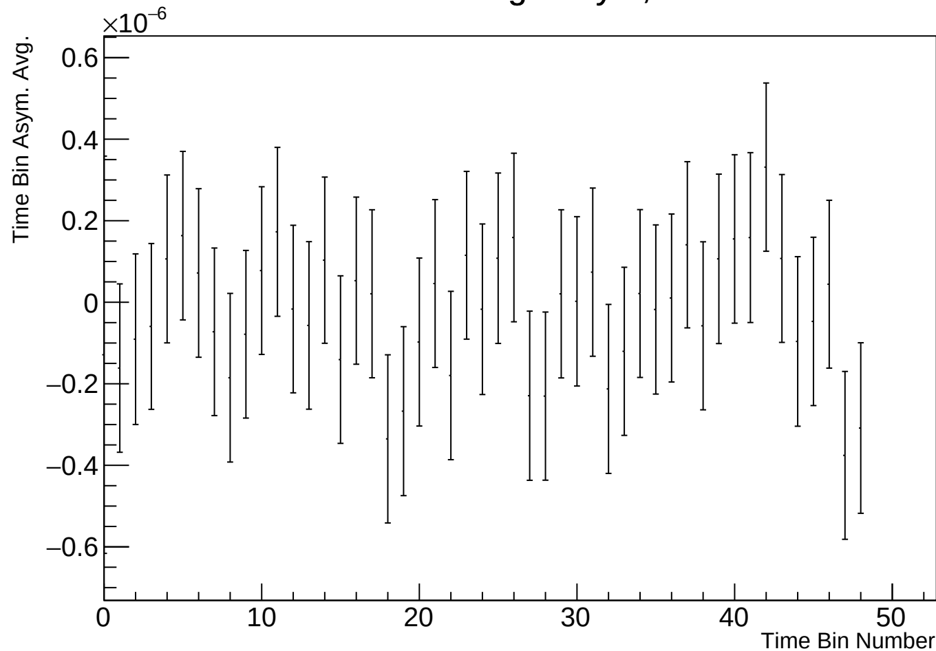
Time Bin Run Average Asym, r17784 w70
