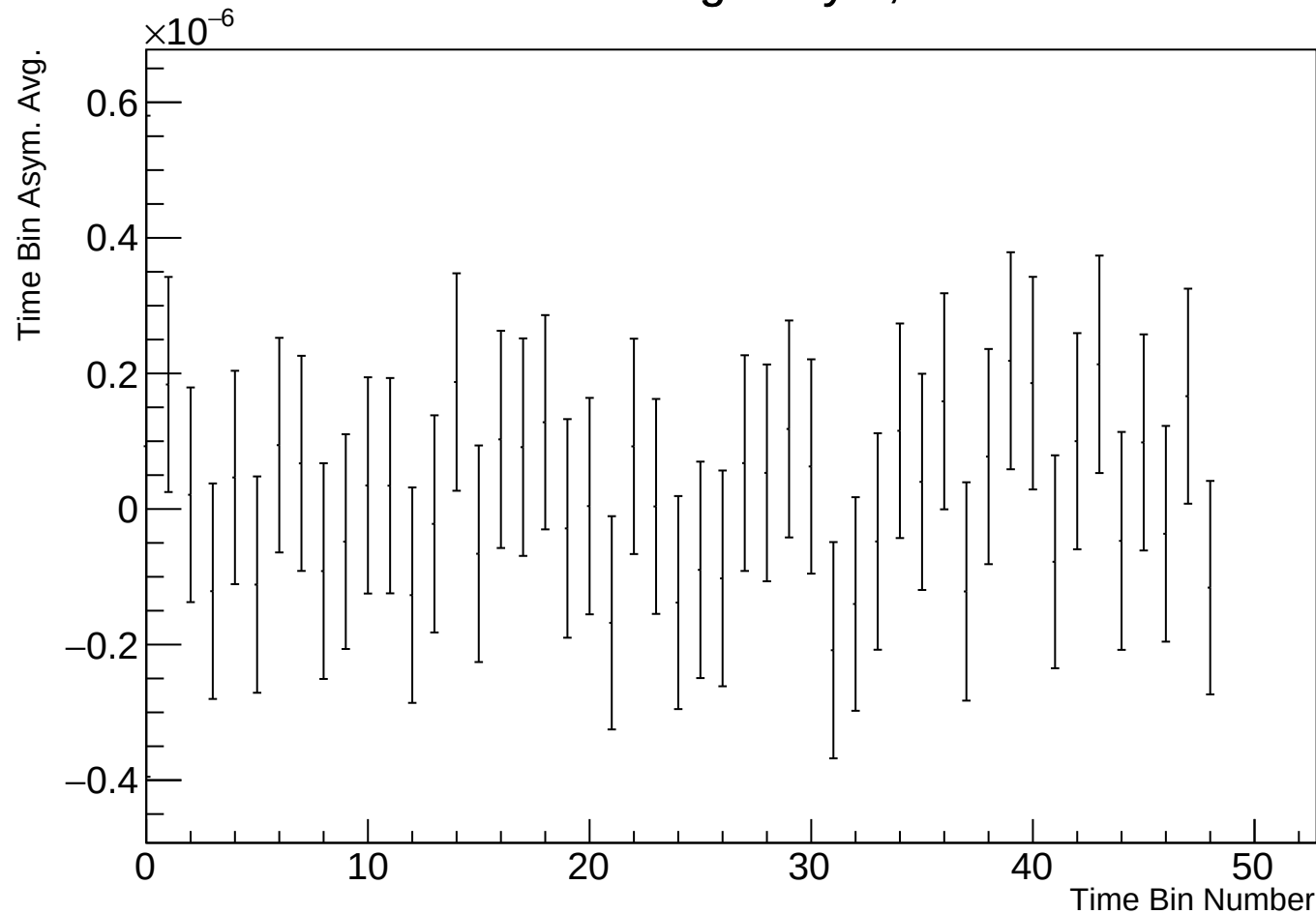
Time Bin Run Average Asym, r17784 w105
