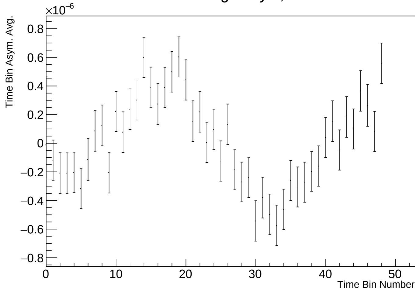
Time Bin Run Average Asym, r17784 w126
