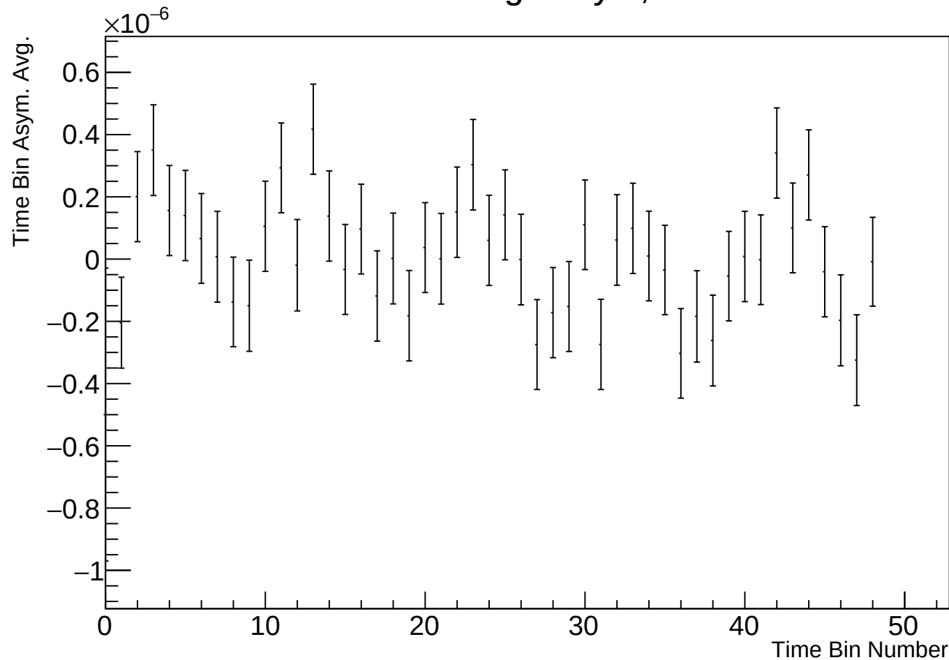
Time Bin Run Average Asym, r17784 w113
