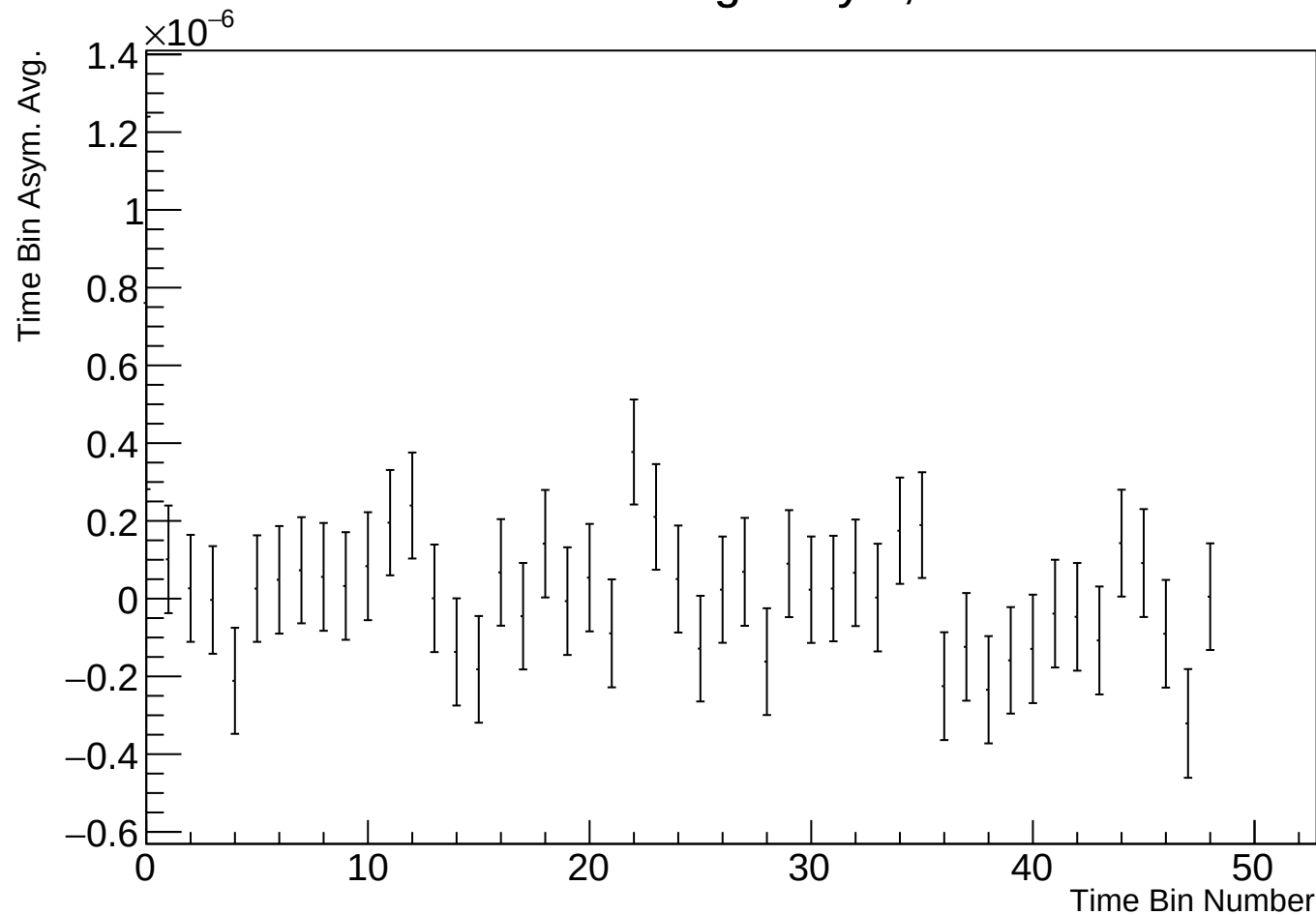
Time Bin Run Average Asym, r17784 w82
