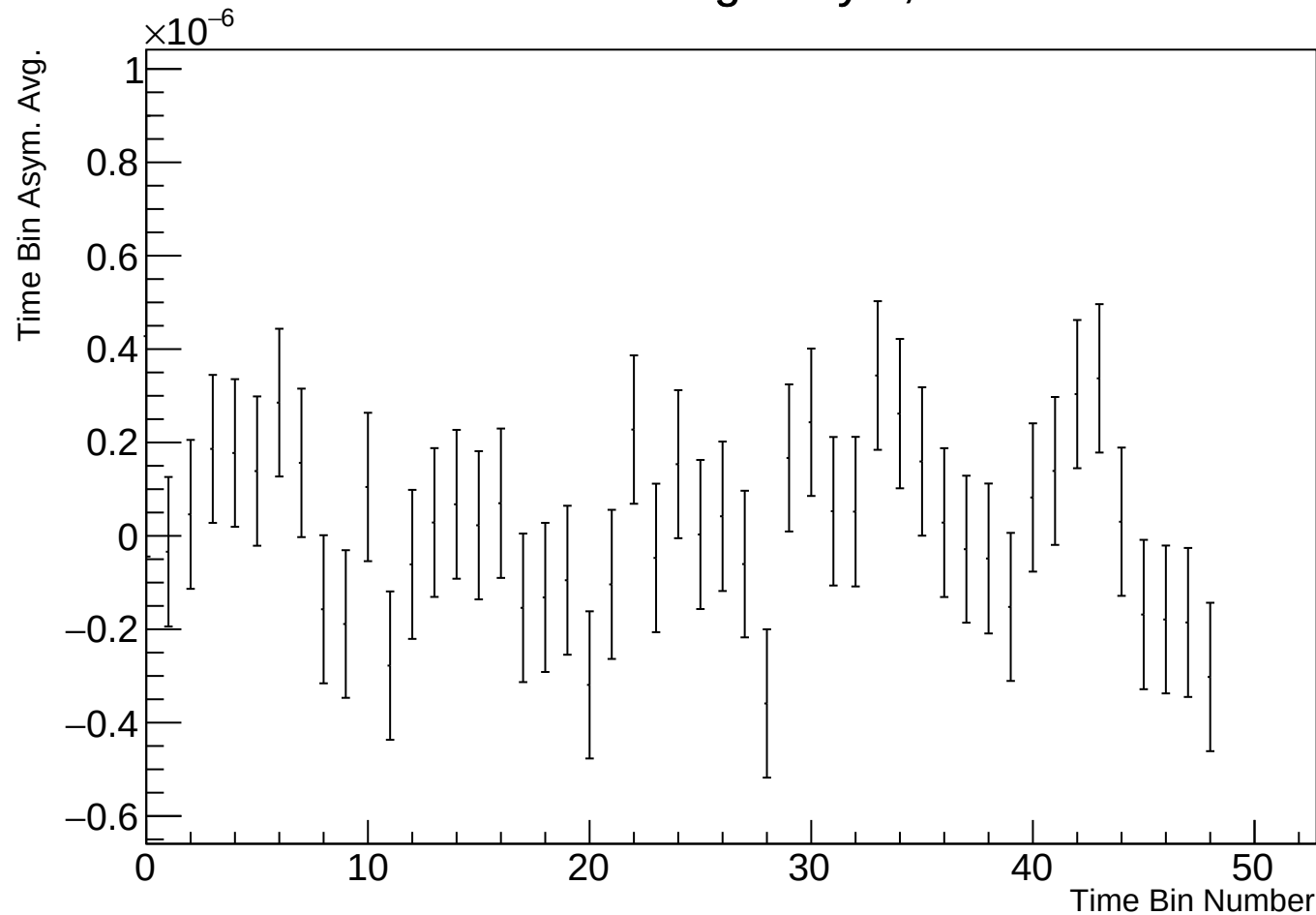
Time Bin Run Average Asym, r17784 w60
