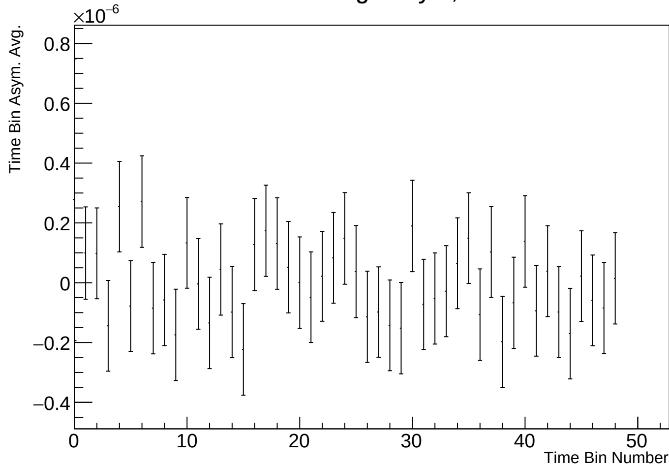
Time Bin Run Average Asym, r17784 w138
