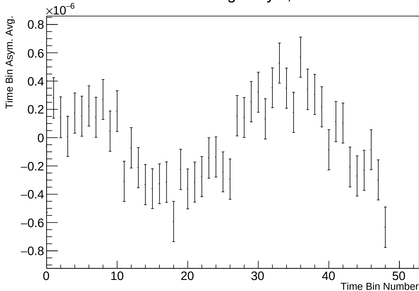
Time Bin Run Average Asym, r17784 w36
