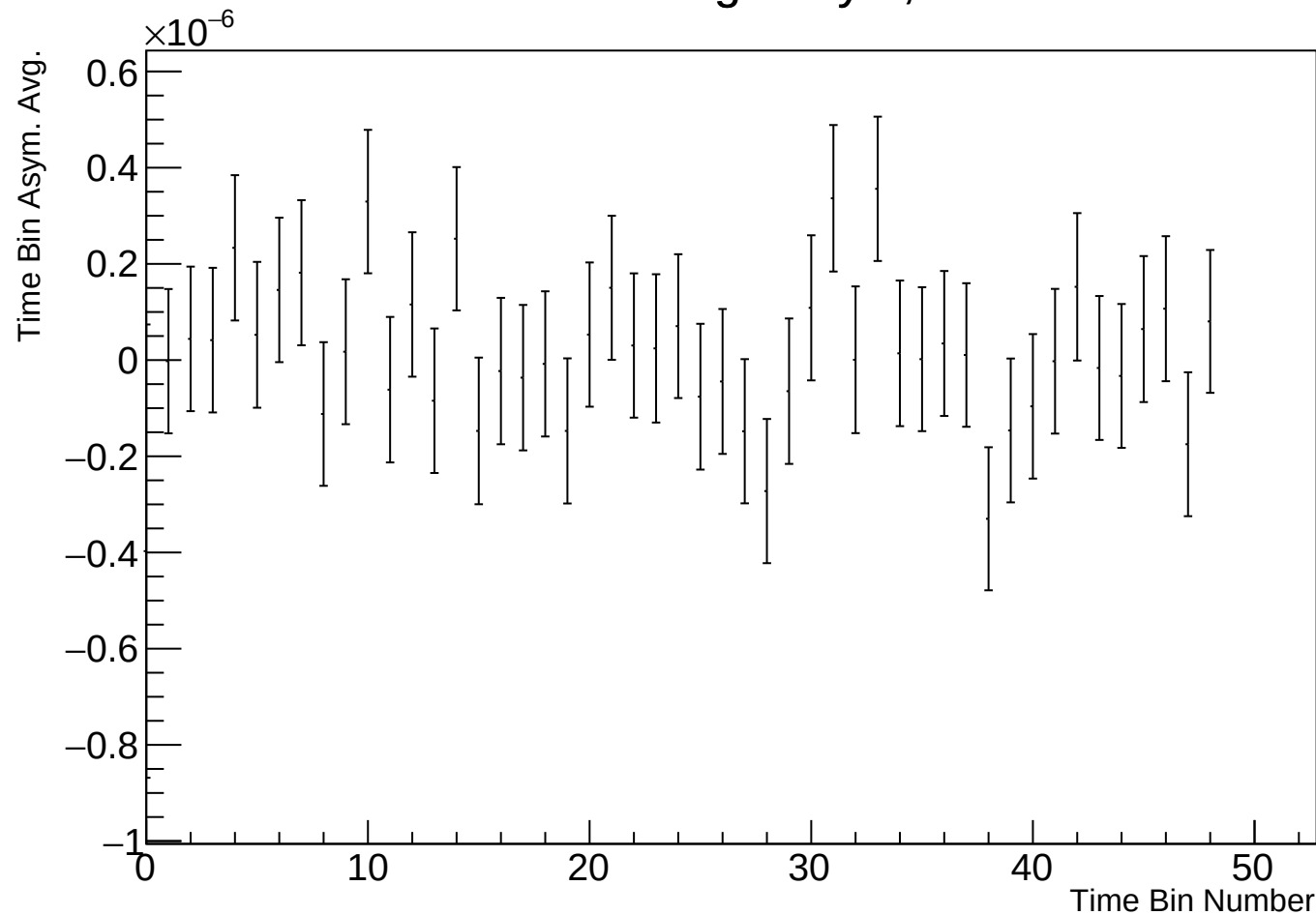
Time Bin Run Average Asym, r17784 w30
