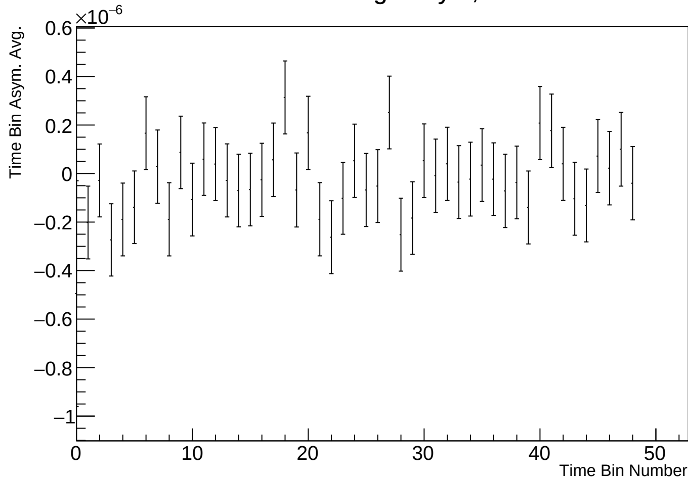
Time Bin Run Average Asym, r17784 w54
