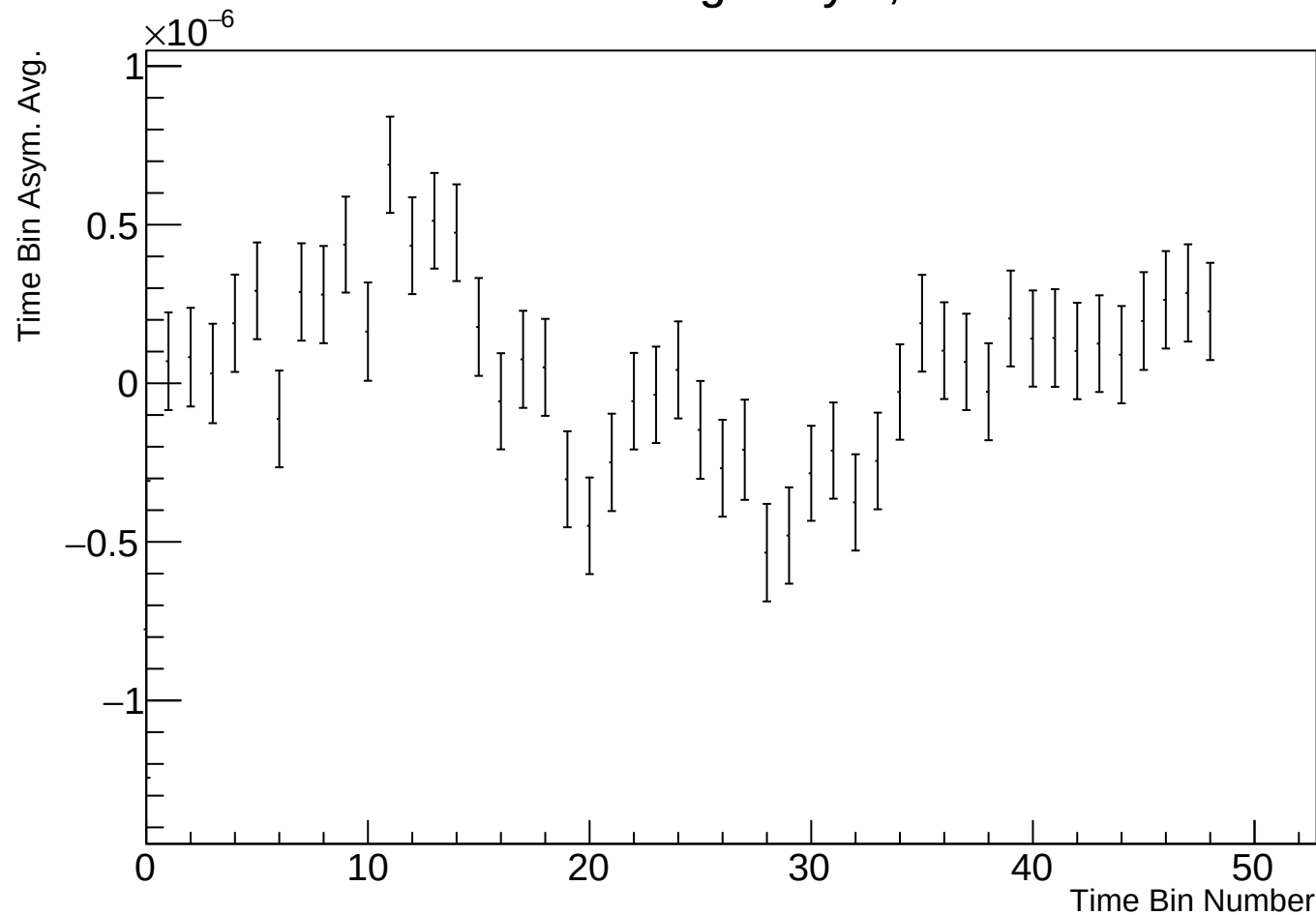
Time Bin Run Average Asym, r17784 w143
