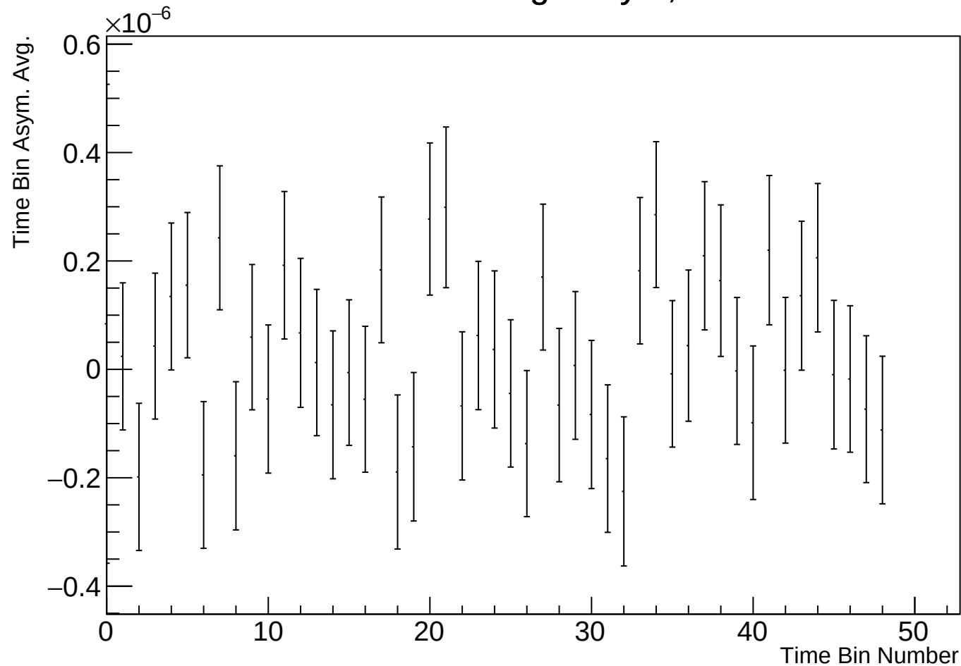
Time Bin Run Average Asym, r17784 w8
