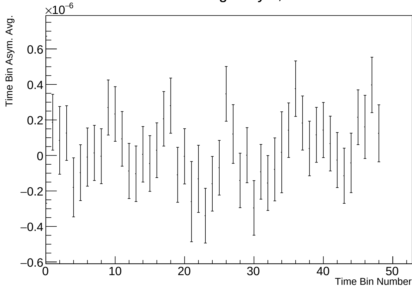
Time Bin Run Average Asym, r17784 w124
