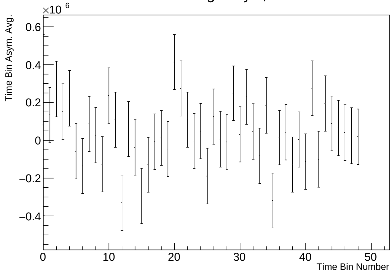
Time Bin Run Average Asym, r17784 w129
