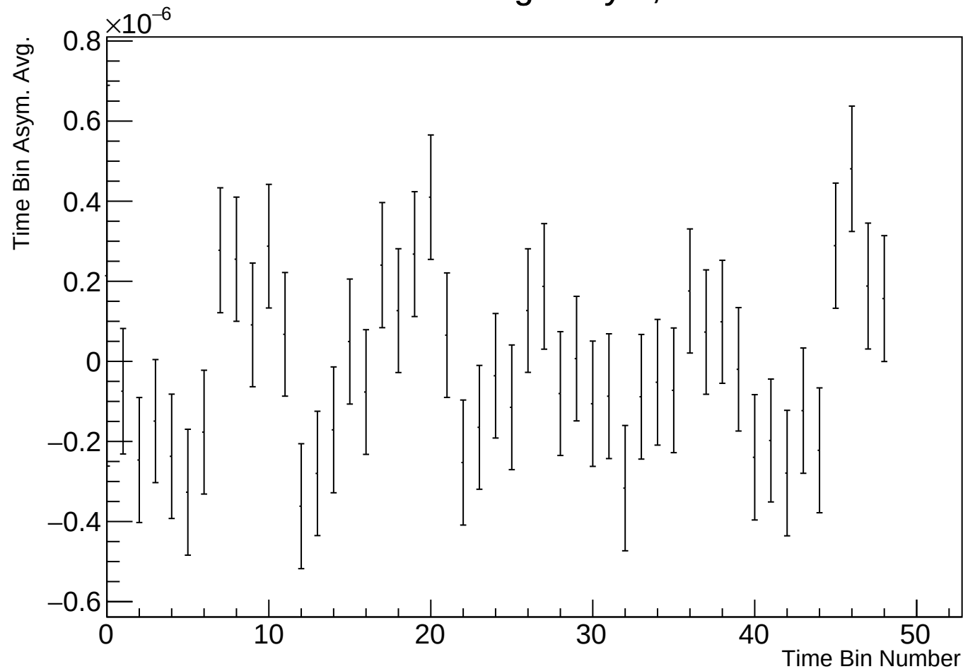
Time Bin Run Average Asym, r17784 w121
