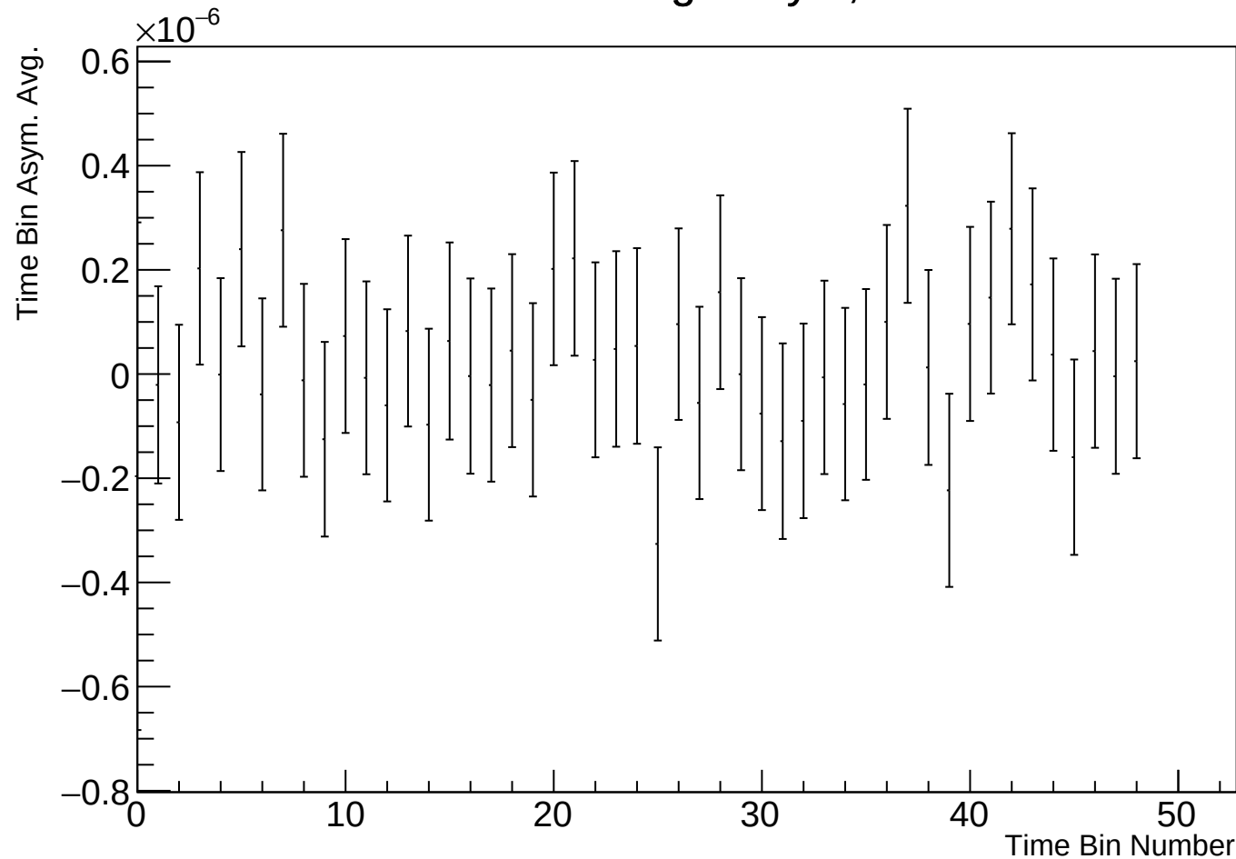
Time Bin Run Average Asym, r17784 w69
