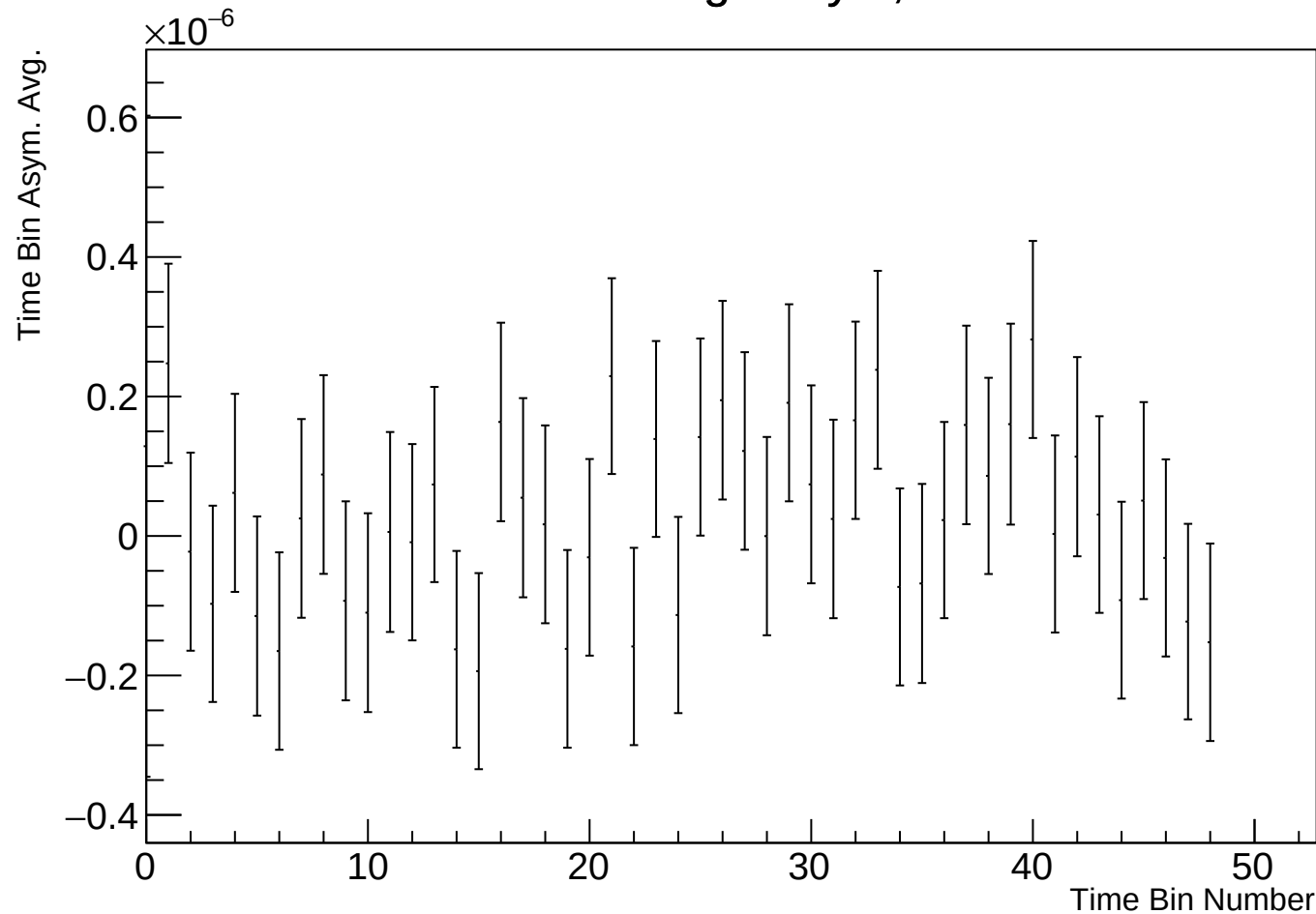
Time Bin Run Average Asym, r17784 w101
