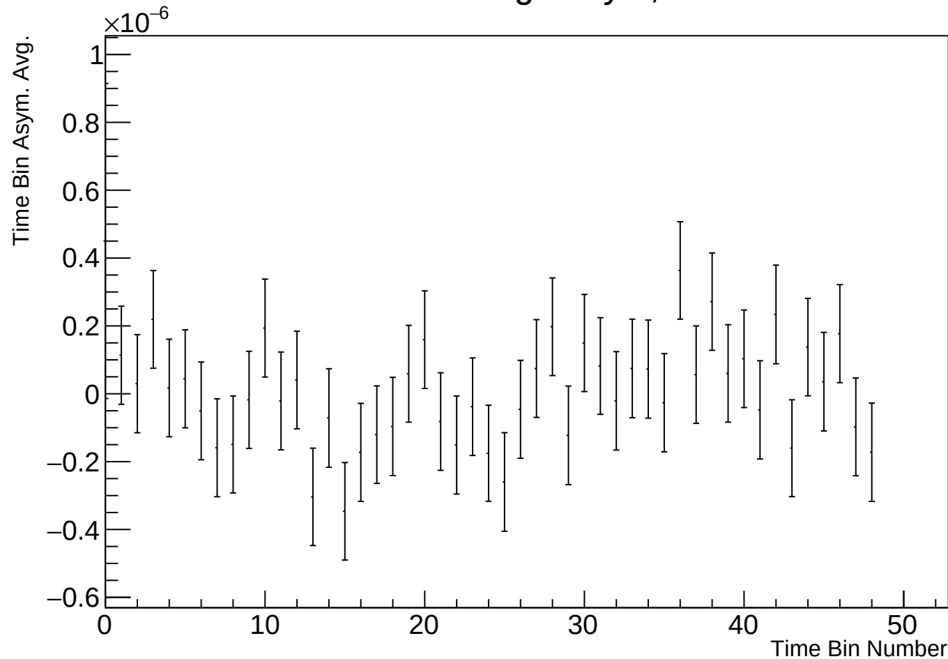
Time Bin Run Average Asym, r17784 w14
