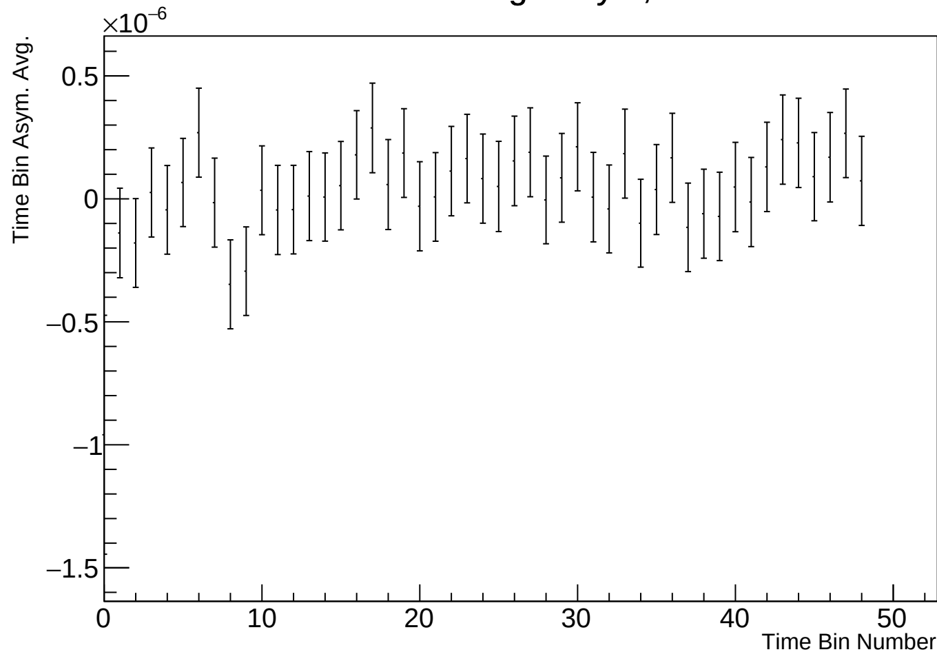
Time Bin Run Average Asym, r17784 w68
