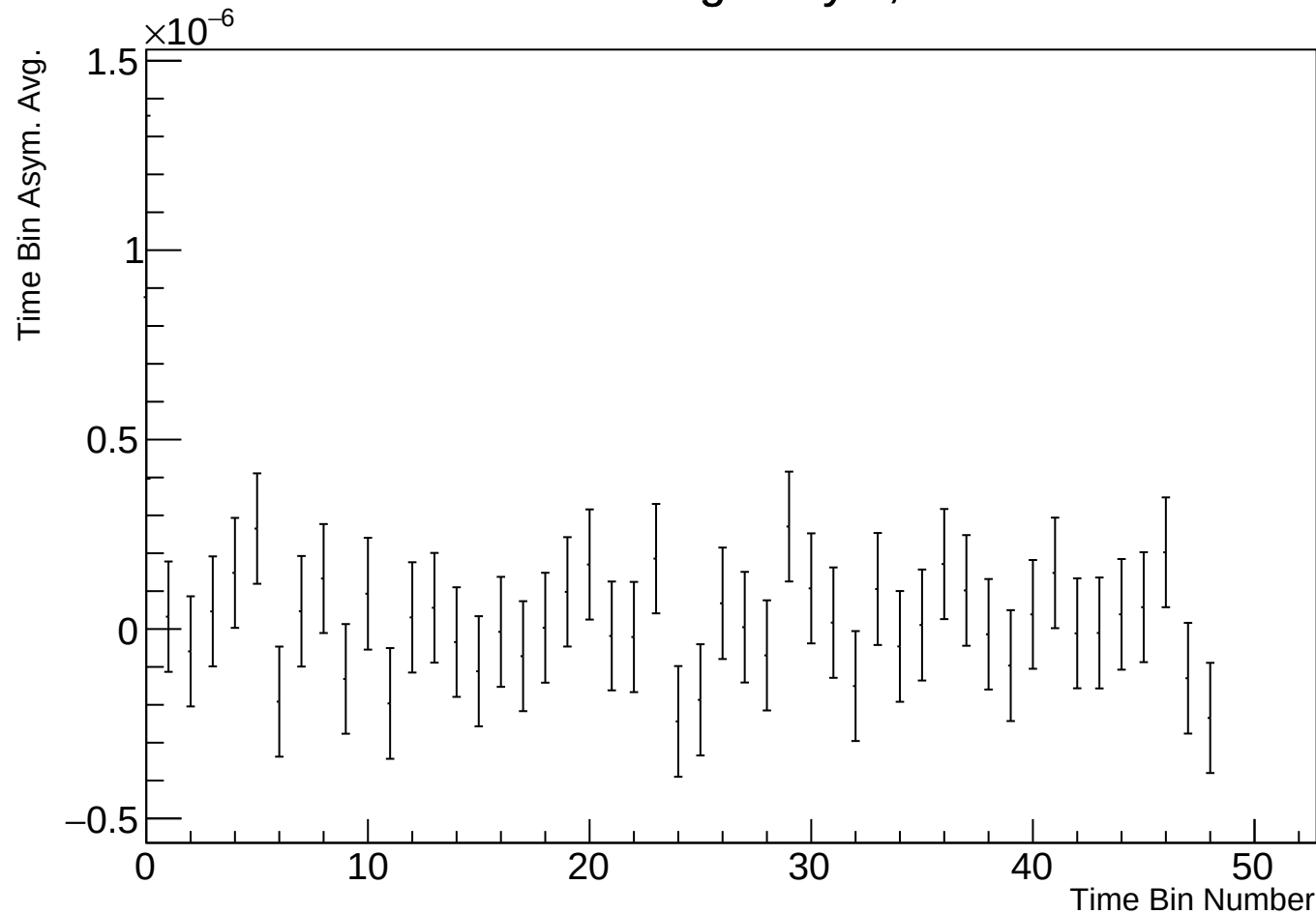
Time Bin Run Average Asym, r17784 w130
