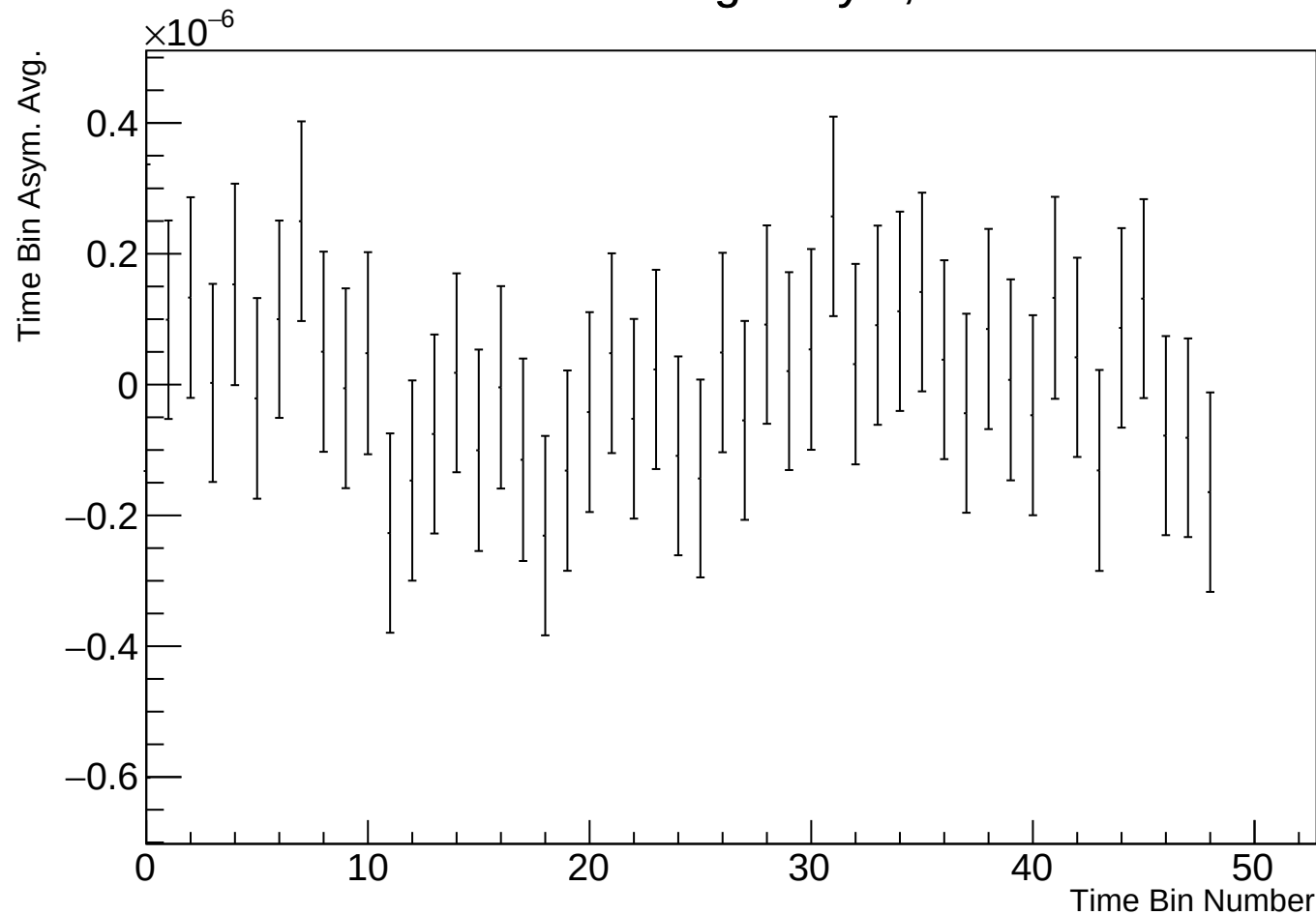
Time Bin Run Average Asym, r17784 w64
