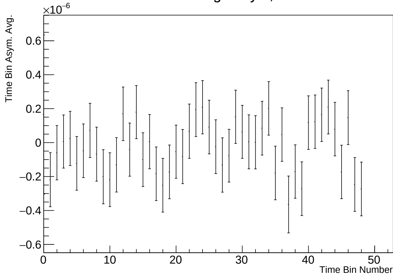
Time Bin Run Average Asym, r17784 w58
