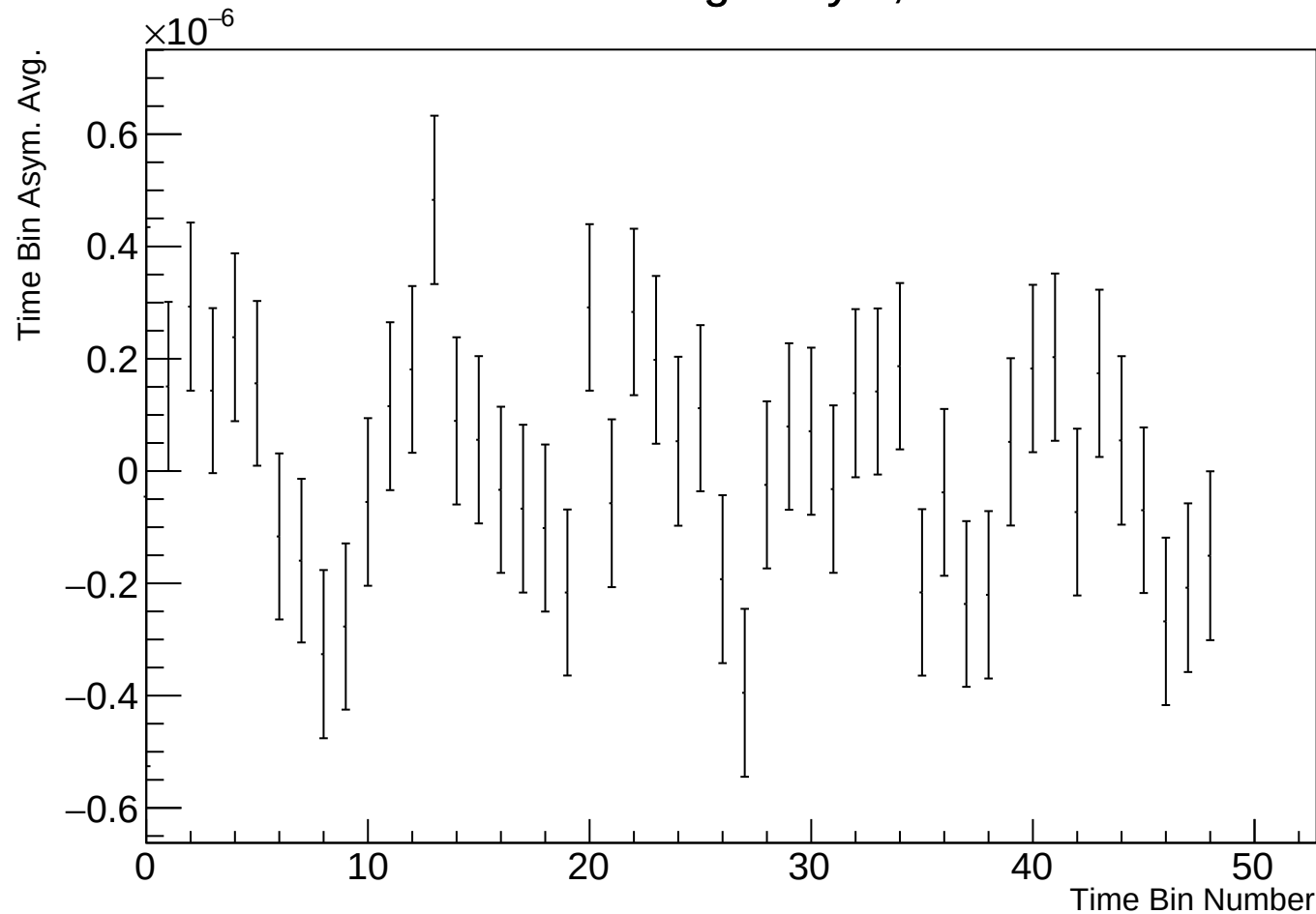
Time Bin Run Average Asym, r17784 w111
