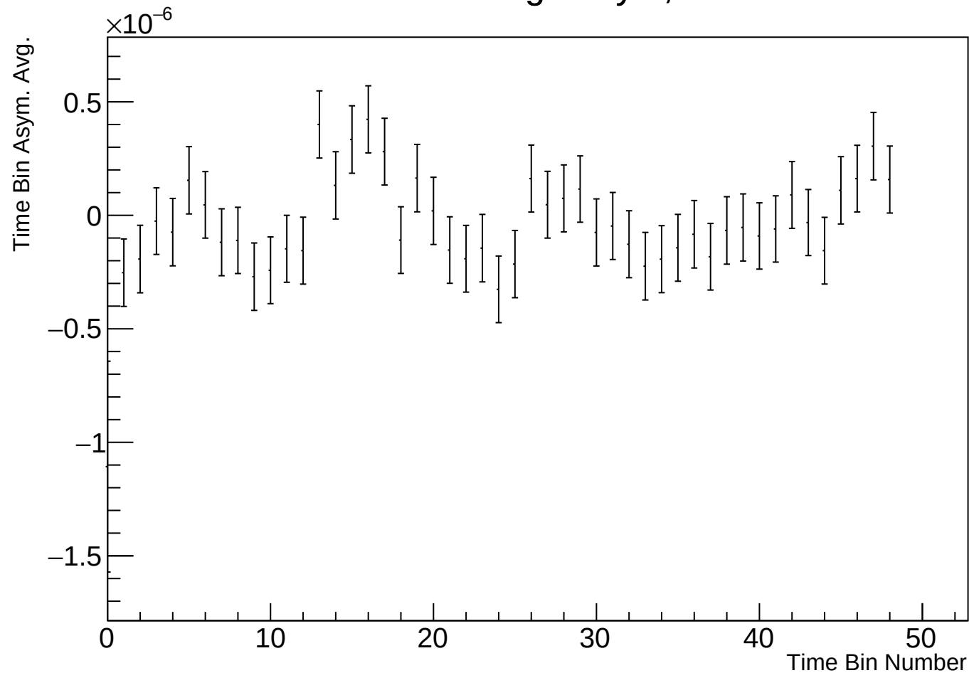
Time Bin Run Average Asym, r17784 w35
