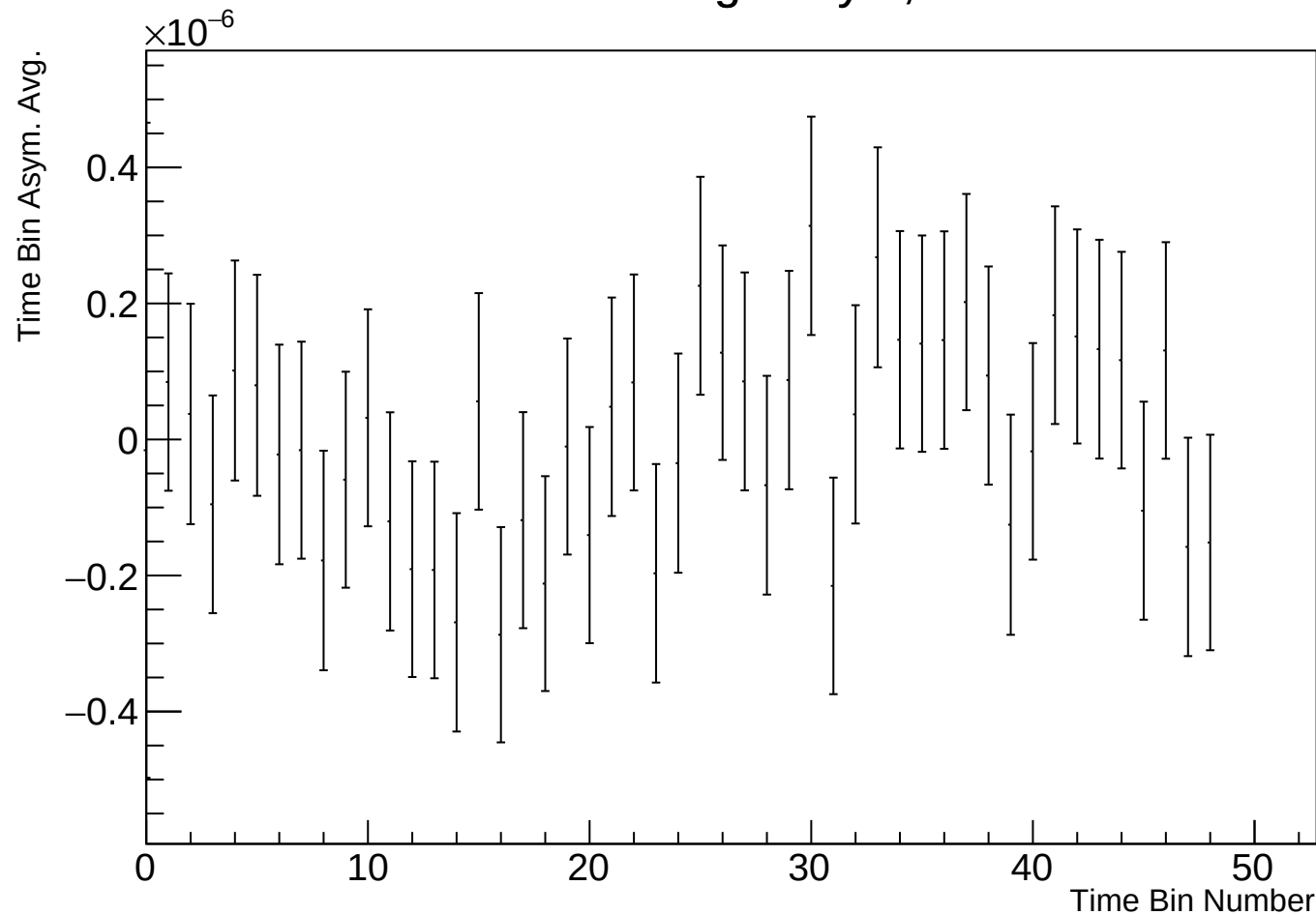
Time Bin Run Average Asym, r17784 w12
