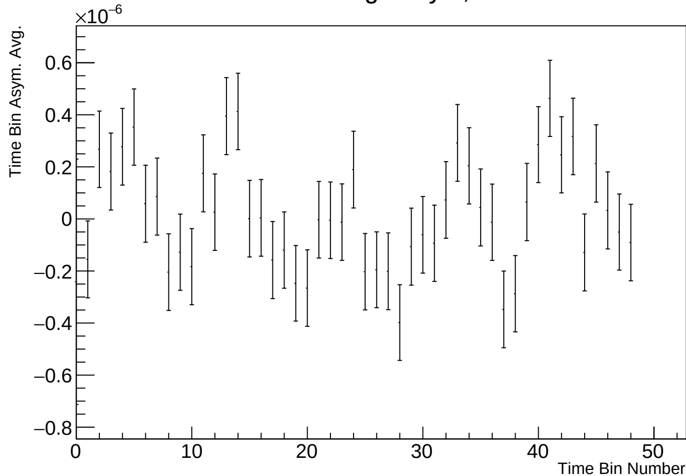
Time Bin Run Average Asym, r17784 w115
