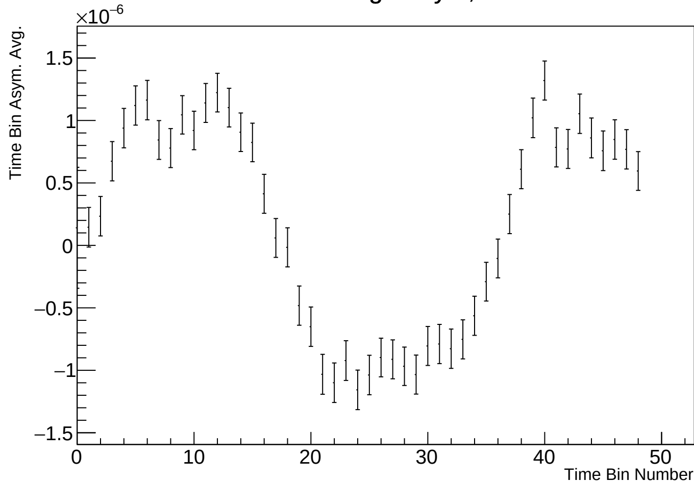
Time Bin Run Average Asym, r17784 w116
