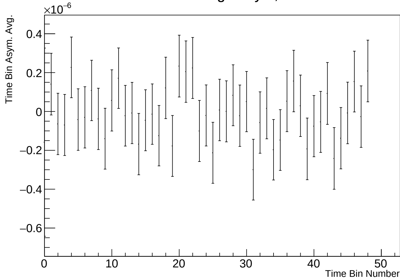
Time Bin Run Average Asym, r17784 w96
