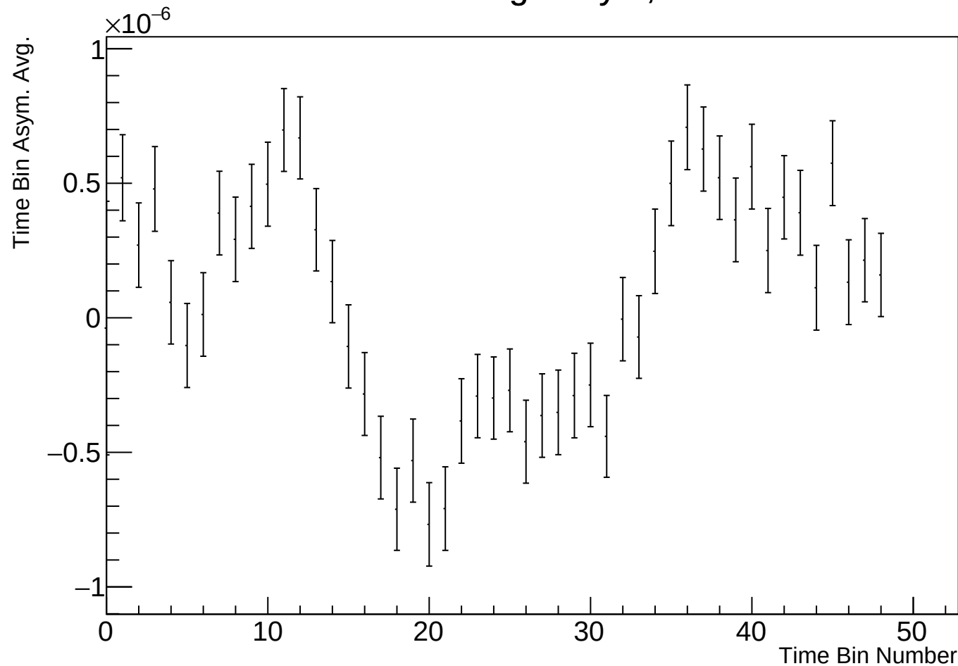
Time Bin Run Average Asym, r17784 w134
