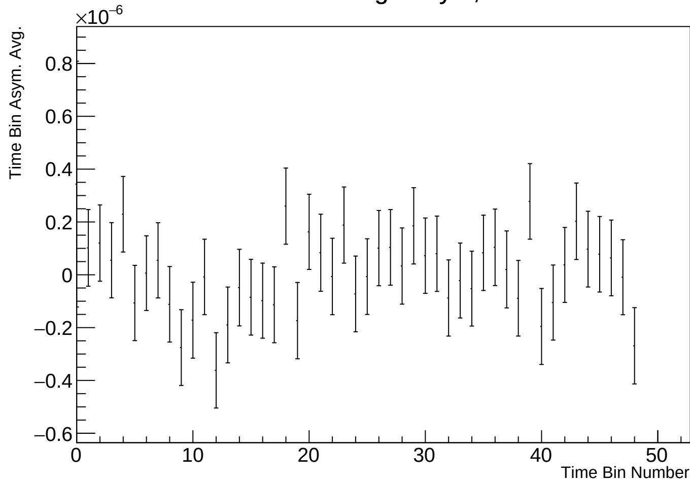
Time Bin Run Average Asym, r17784 w13
