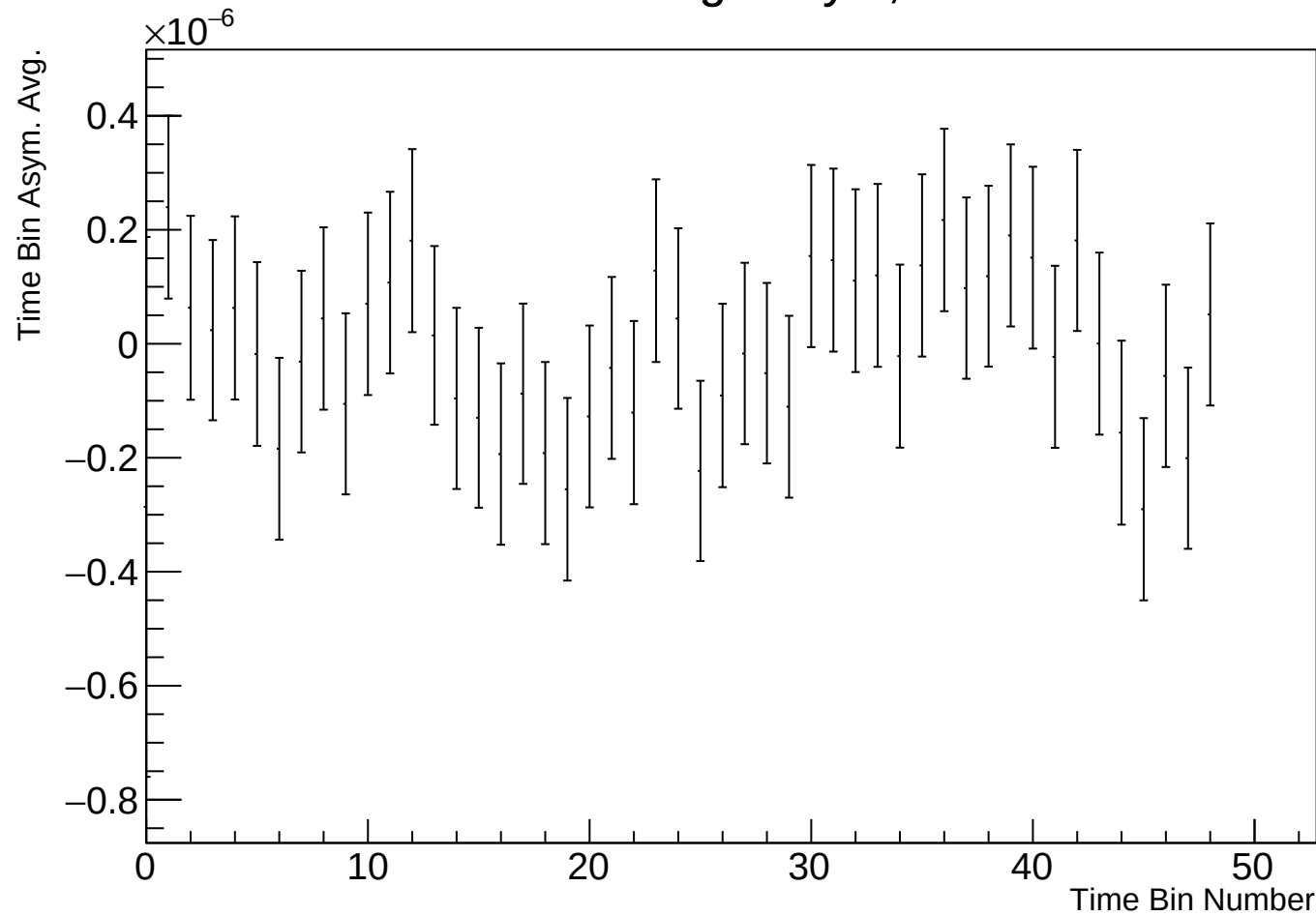
Time Bin Run Average Asym, r17784 w133
