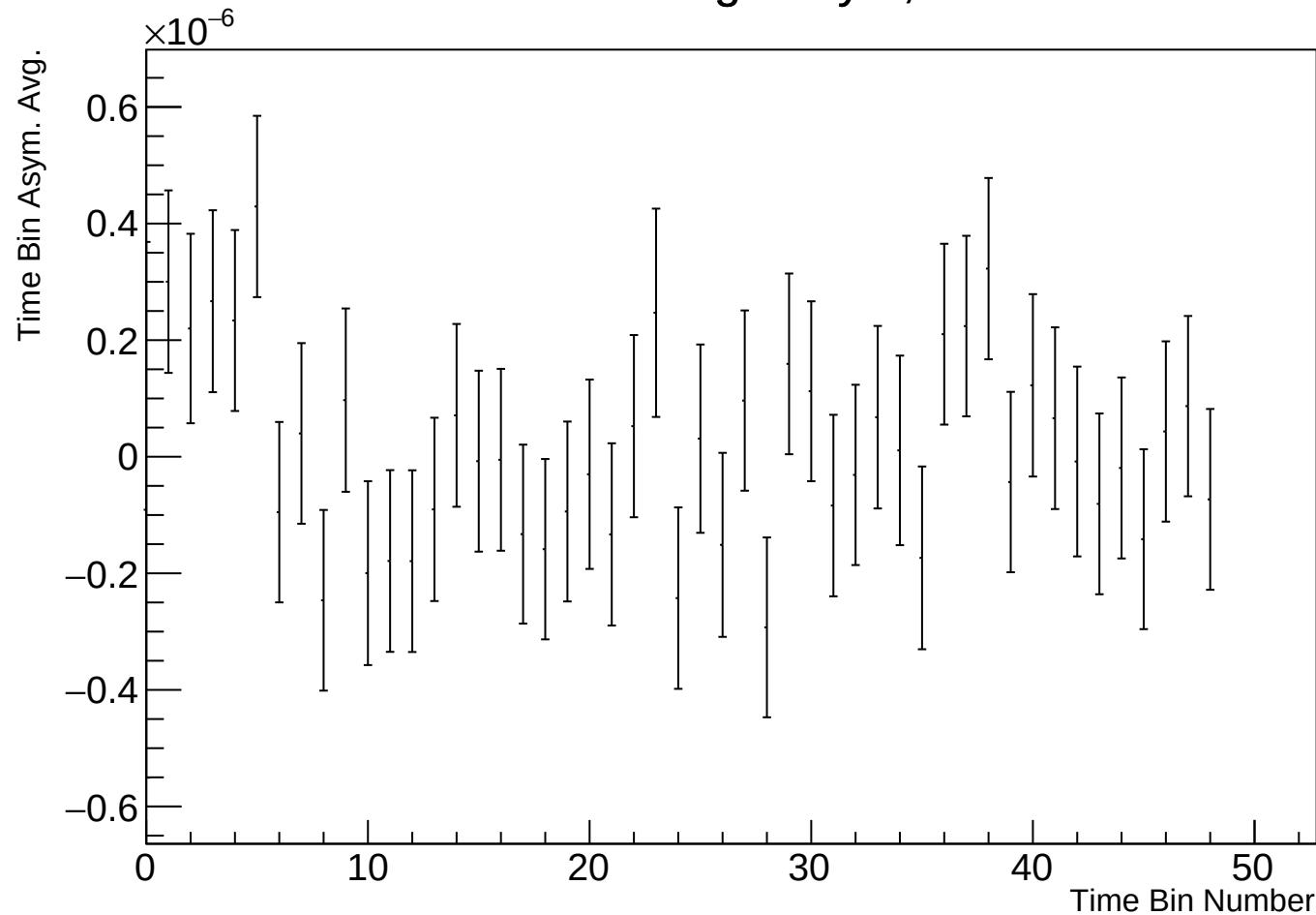
Time Bin Run Average Asym, r17784 w26
