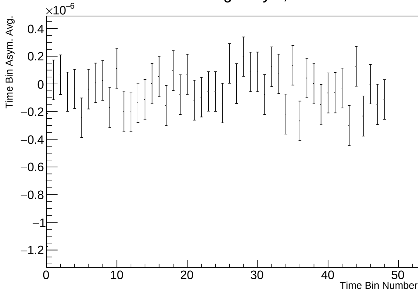
Time Bin Run Average Asym, r38100 w111
