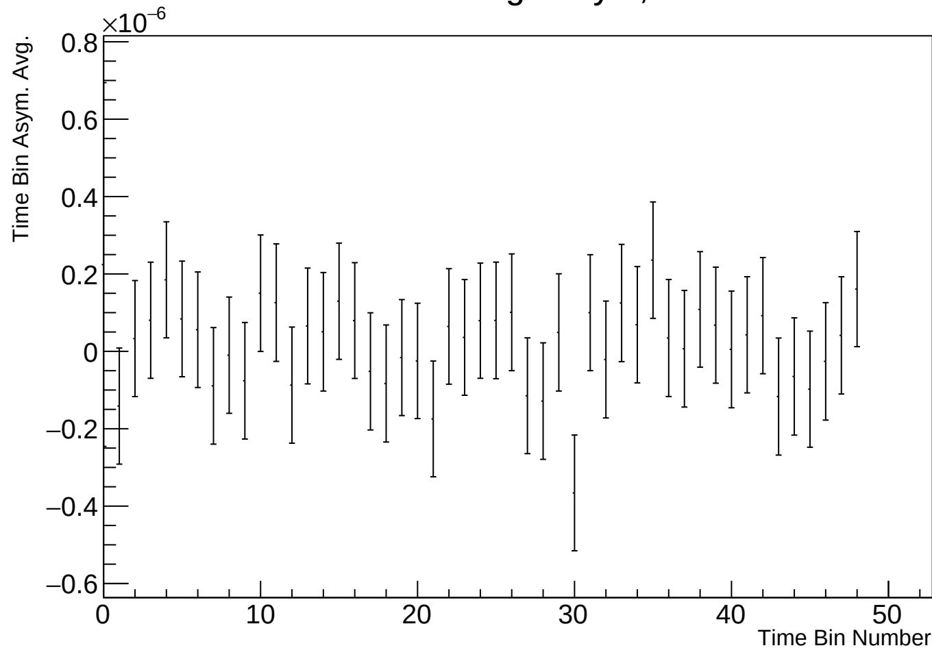
Time Bin Run Average Asym, r38100 w56
