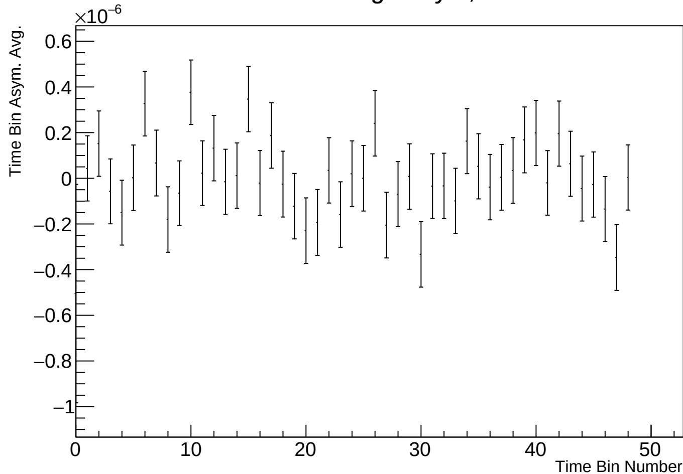
Time Bin Run Average Asym, r38100 w86
