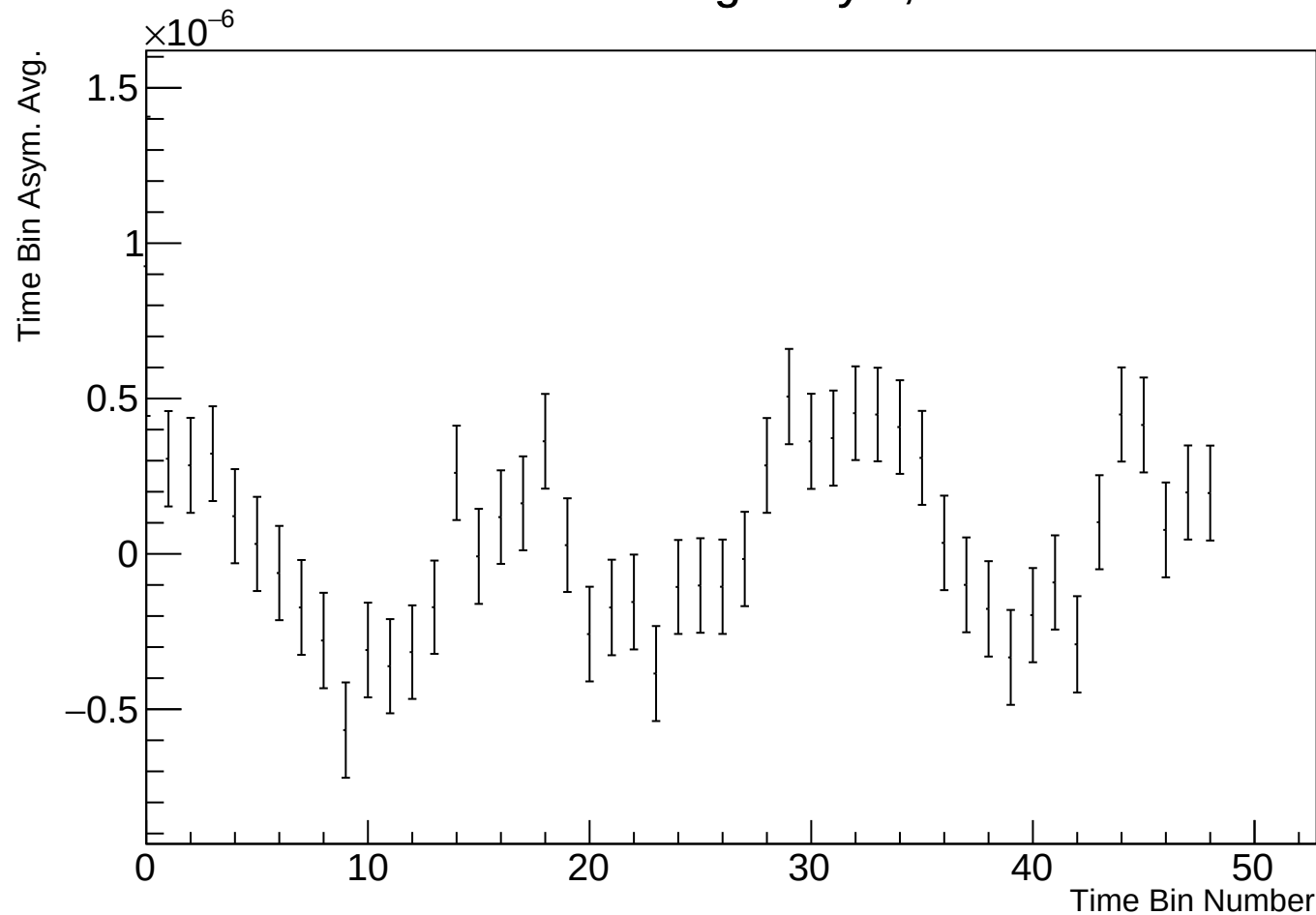
Time Bin Run Average Asym, r38100 w98
