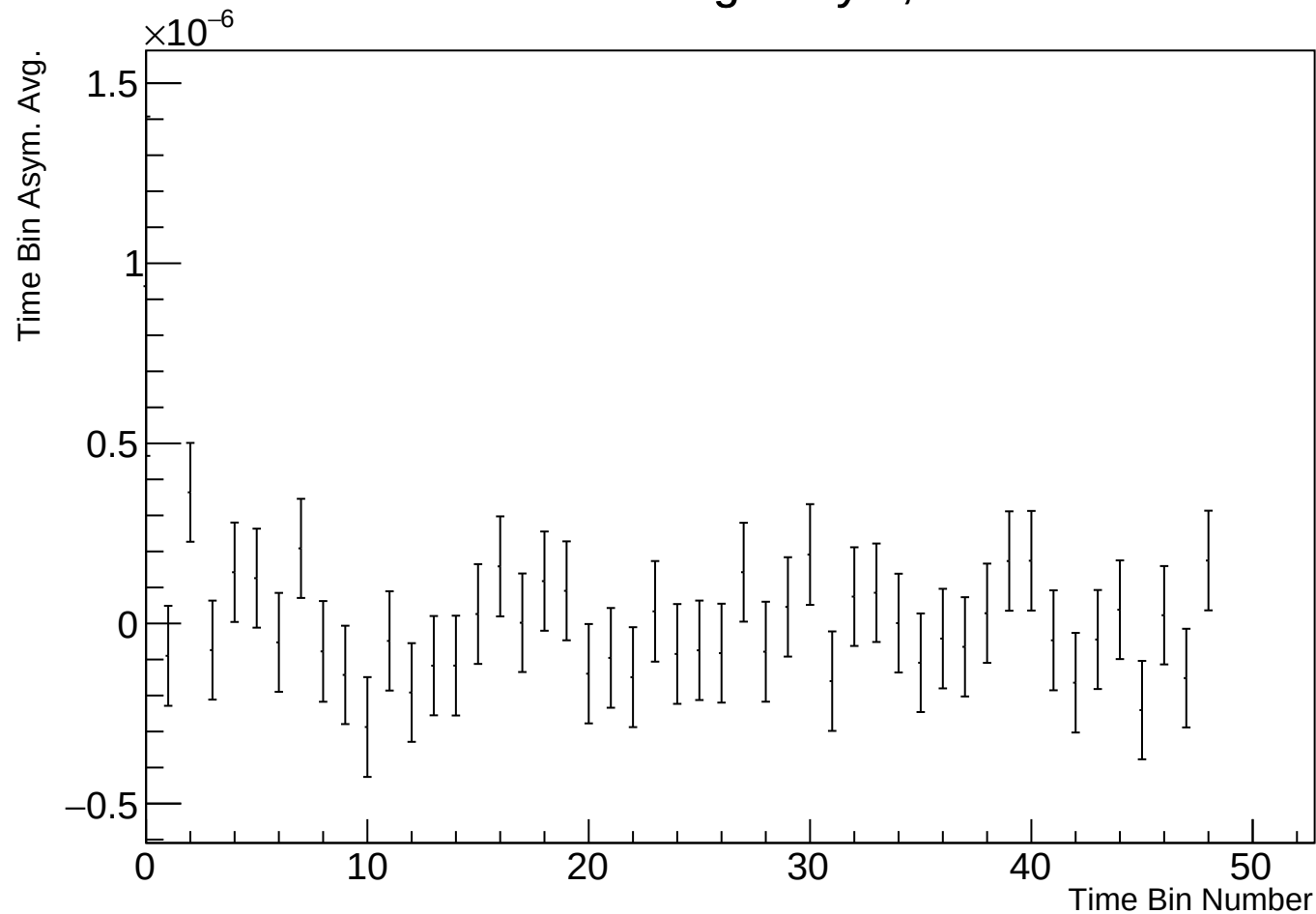
Time Bin Run Average Asym, r38100 w94
