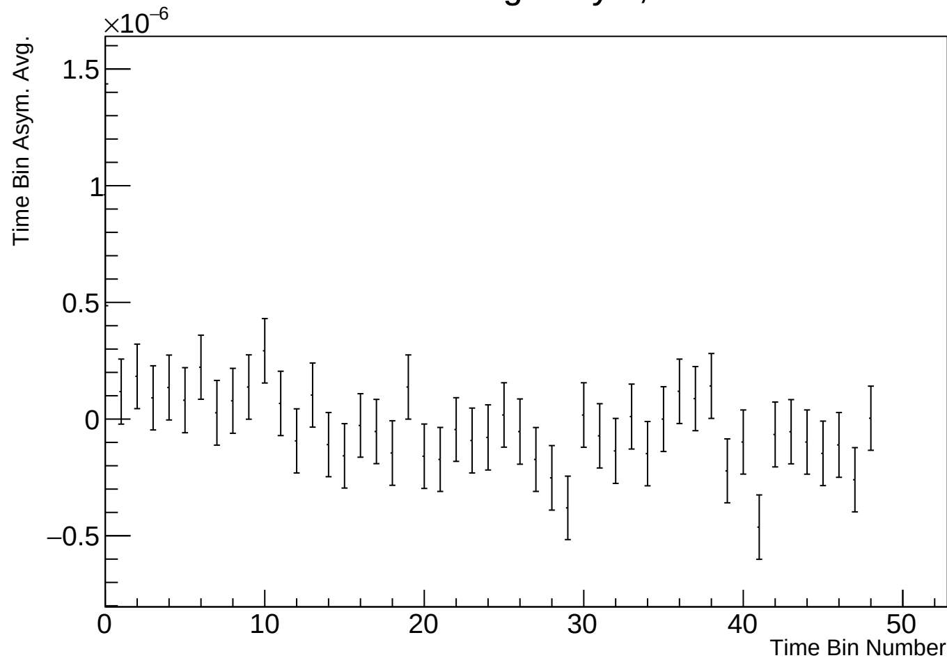
Time Bin Run Average Asym, r38100 w138
