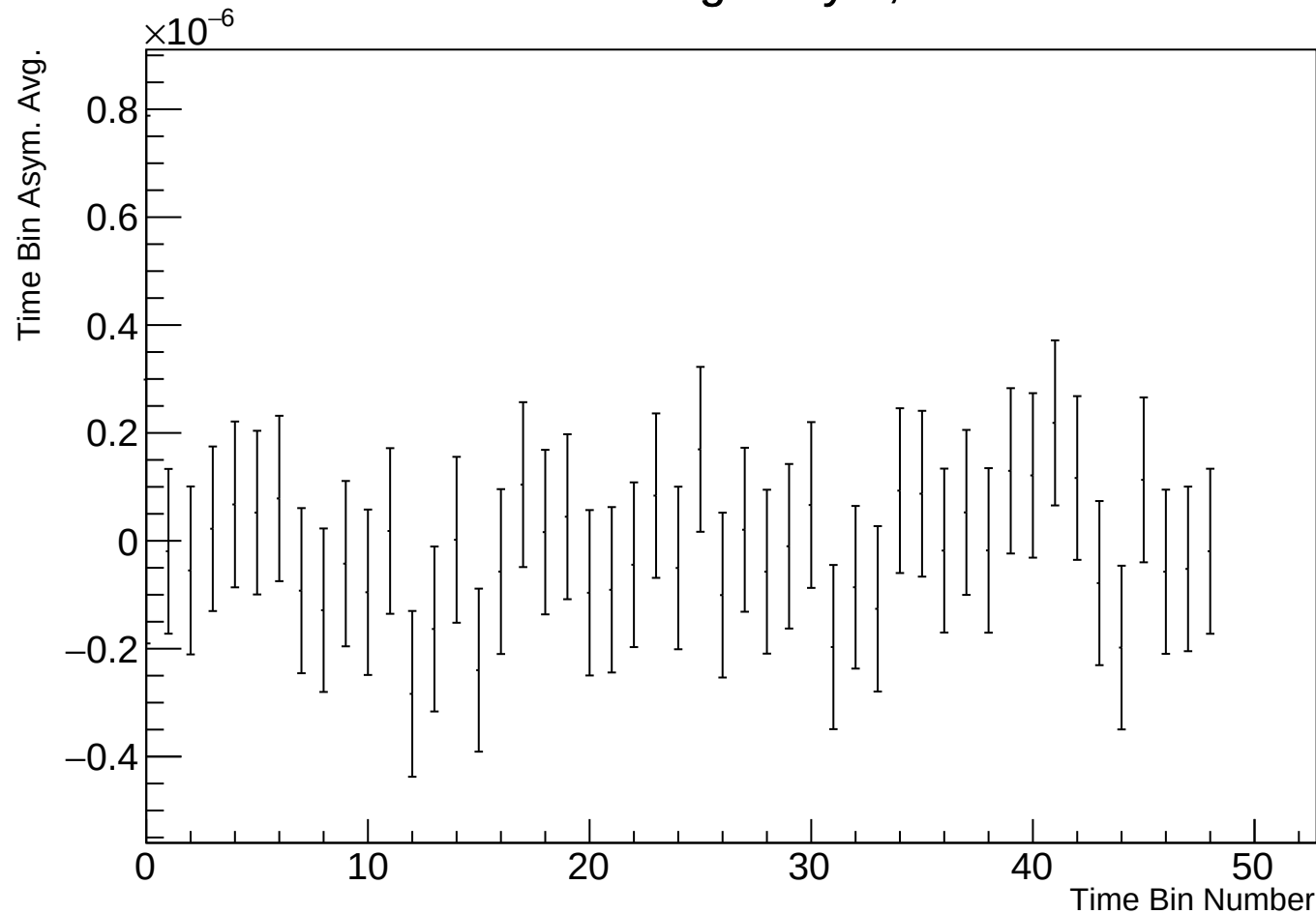
Time Bin Run Average Asym, r38100 w110
