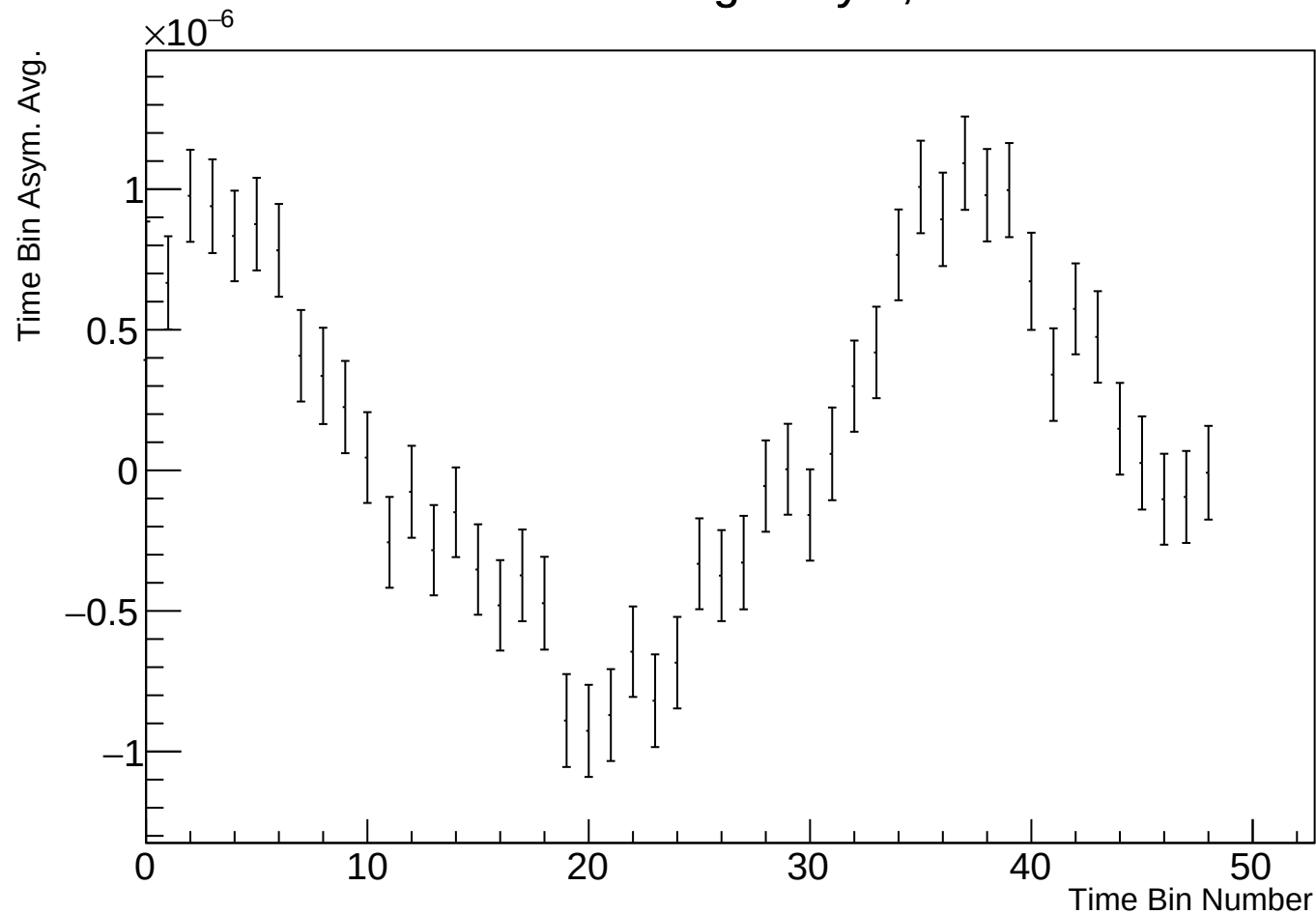
Time Bin Run Average Asym, r38100 w89
