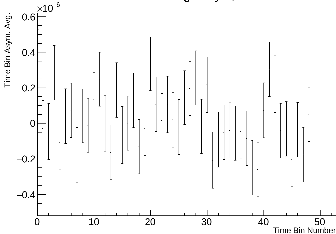
Time Bin Run Average Asym, r38100 w31
