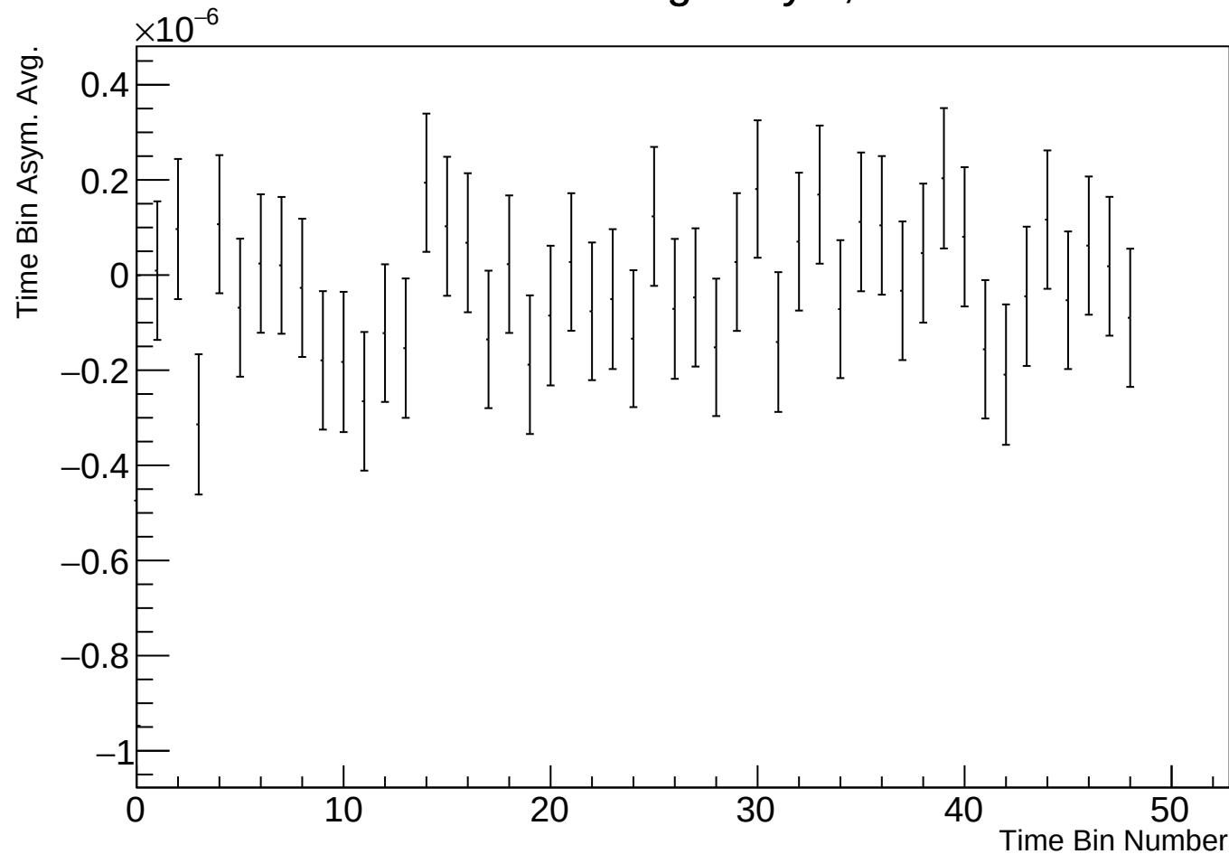
Time Bin Run Average Asym, r38100 w74
