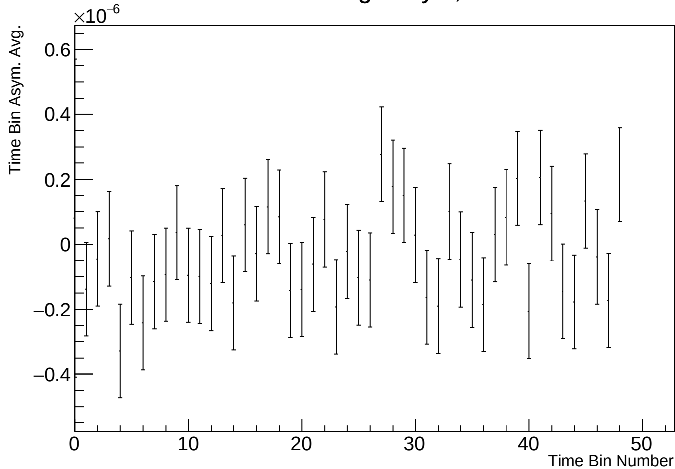
Time Bin Run Average Asym, r38100 w129
