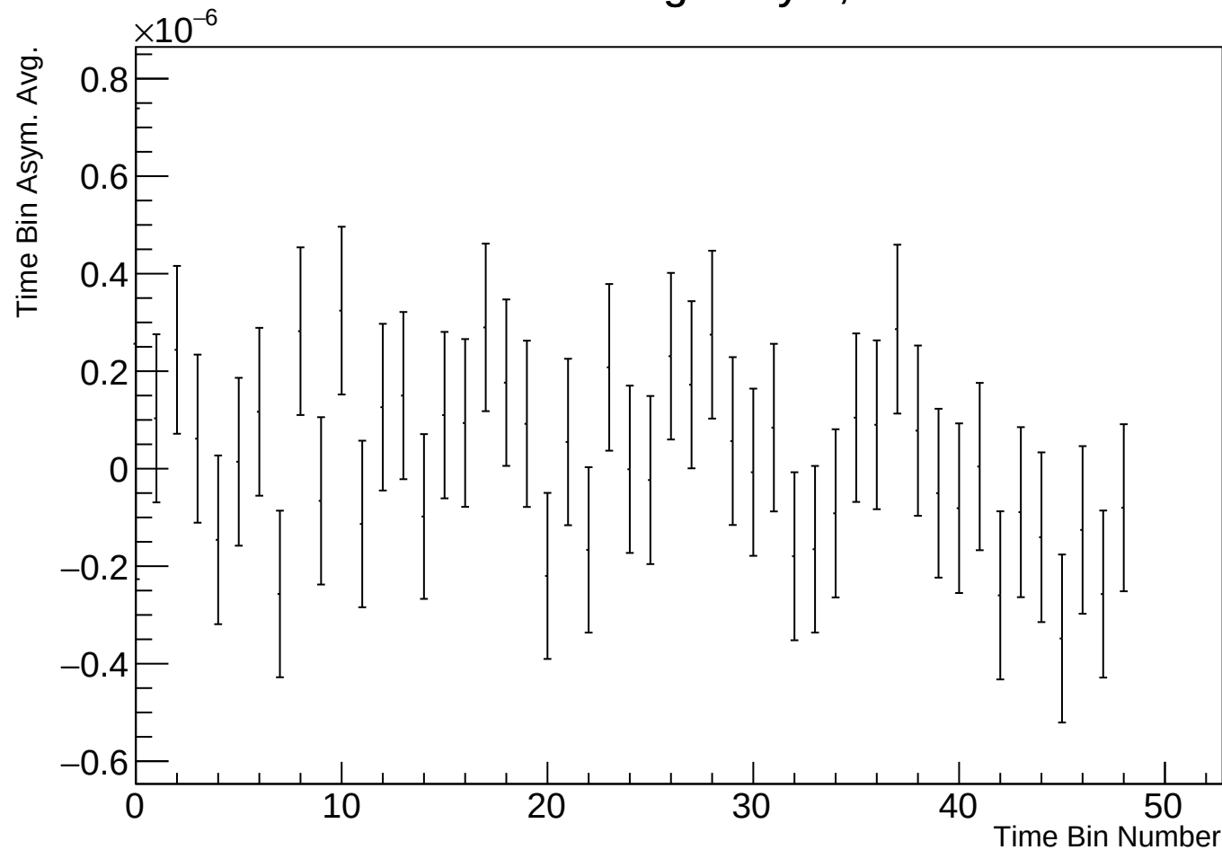
Time Bin Run Average Asym, r38100 w66
