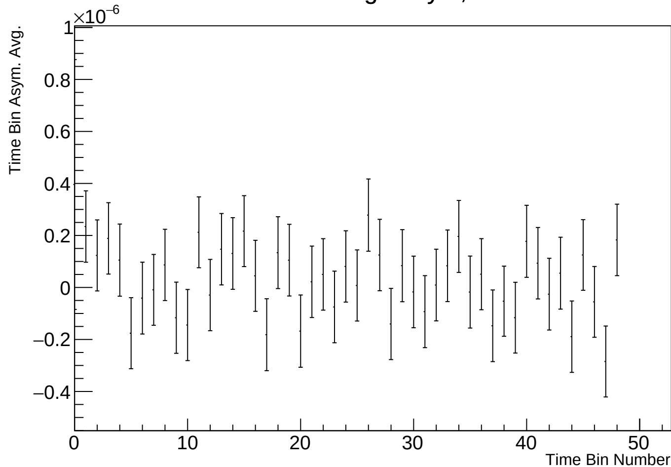
Time Bin Run Average Asym, r38100 w85
