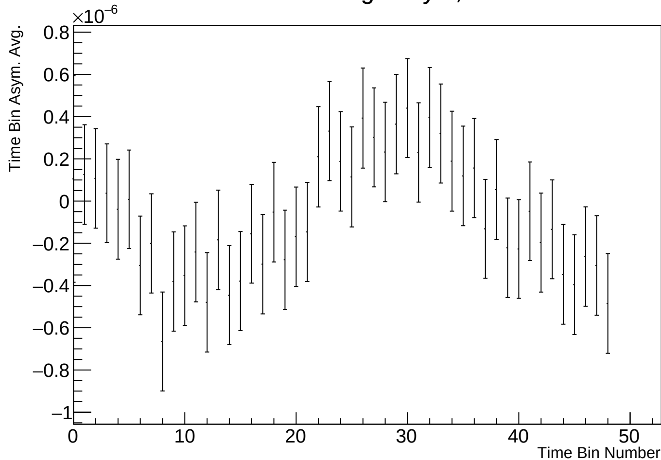
Time Bin Run Average Asym, r38100 w41
