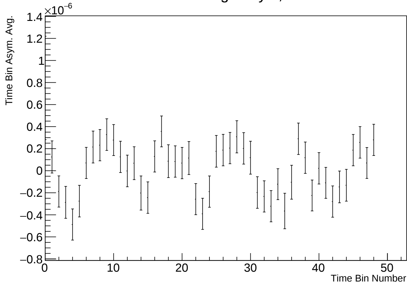
Time Bin Run Average Asym, r38314 w73
