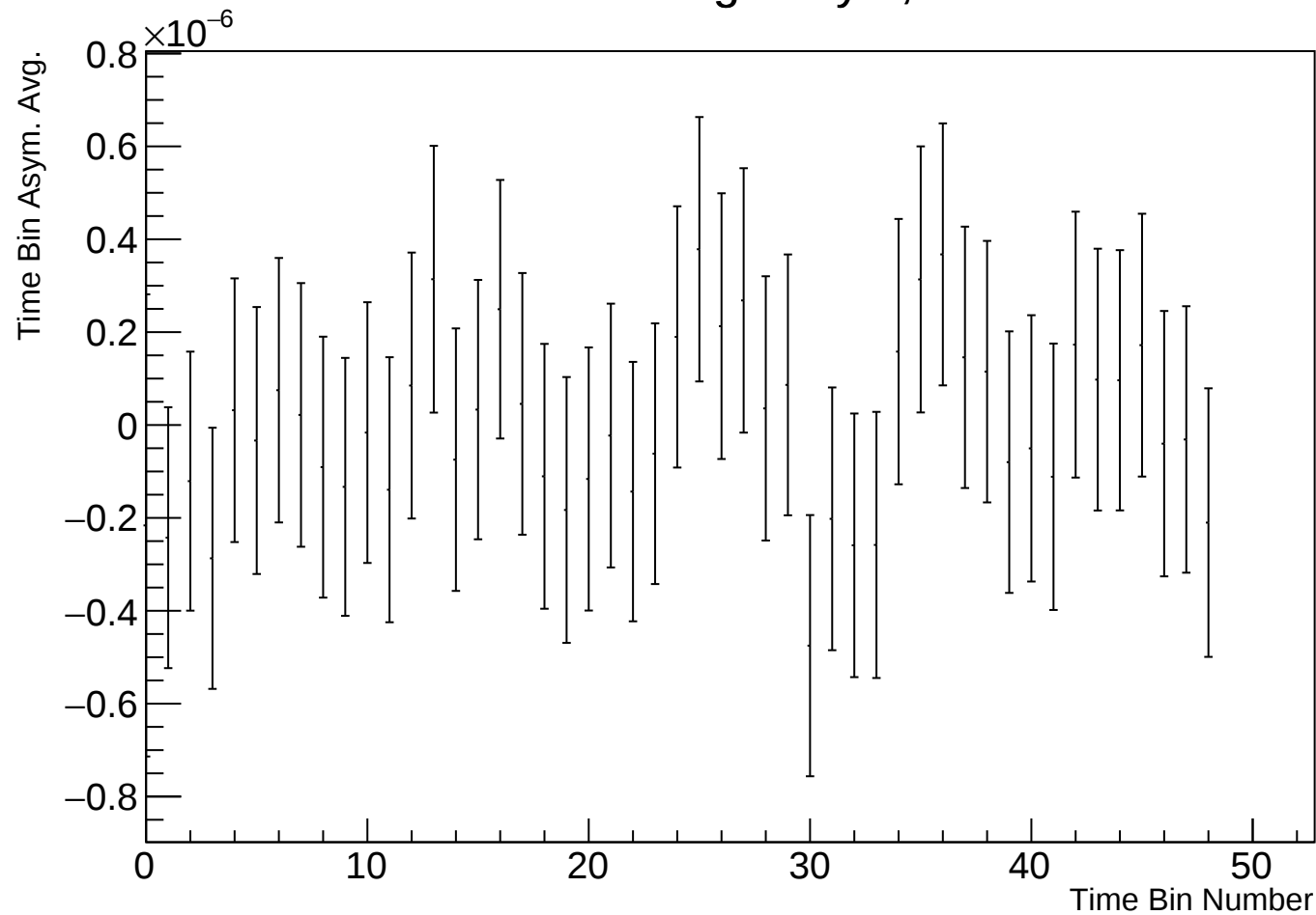
Time Bin Run Average Asym, r38314 w42
