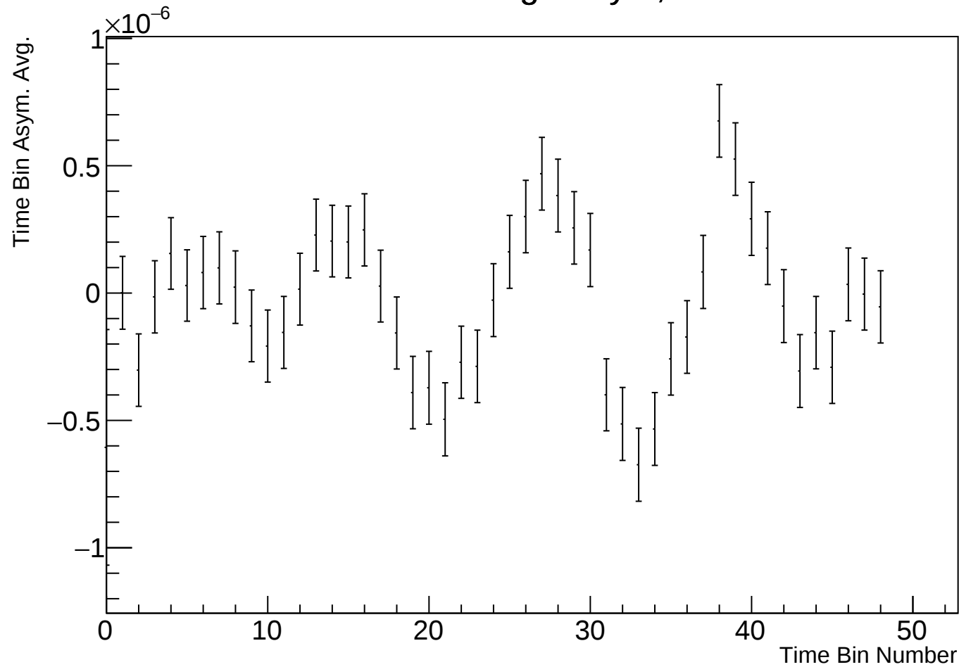
Time Bin Run Average Asym, r38314 w17
