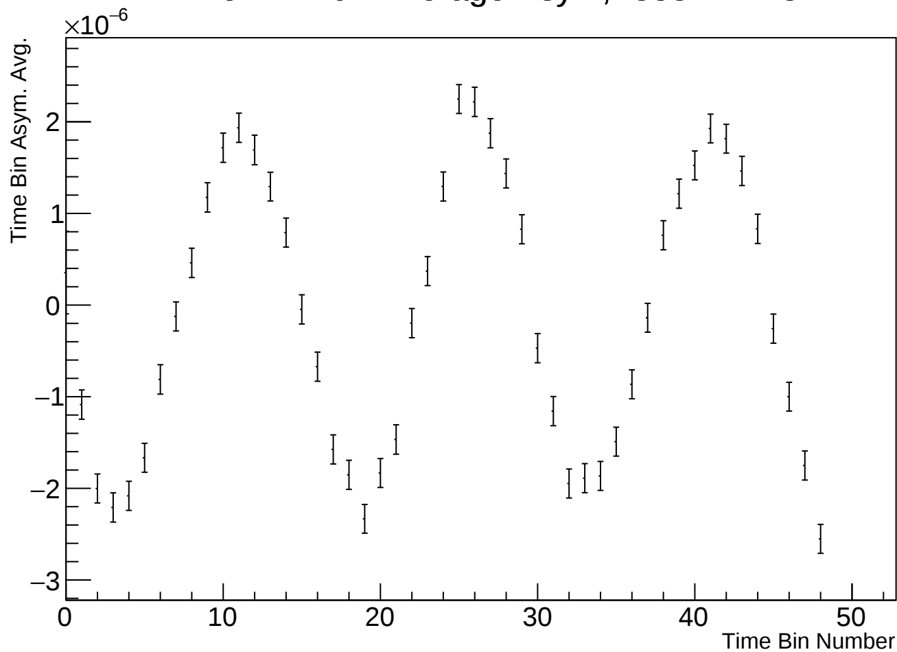
Time Bin Run Average Asym, r38314 w43
