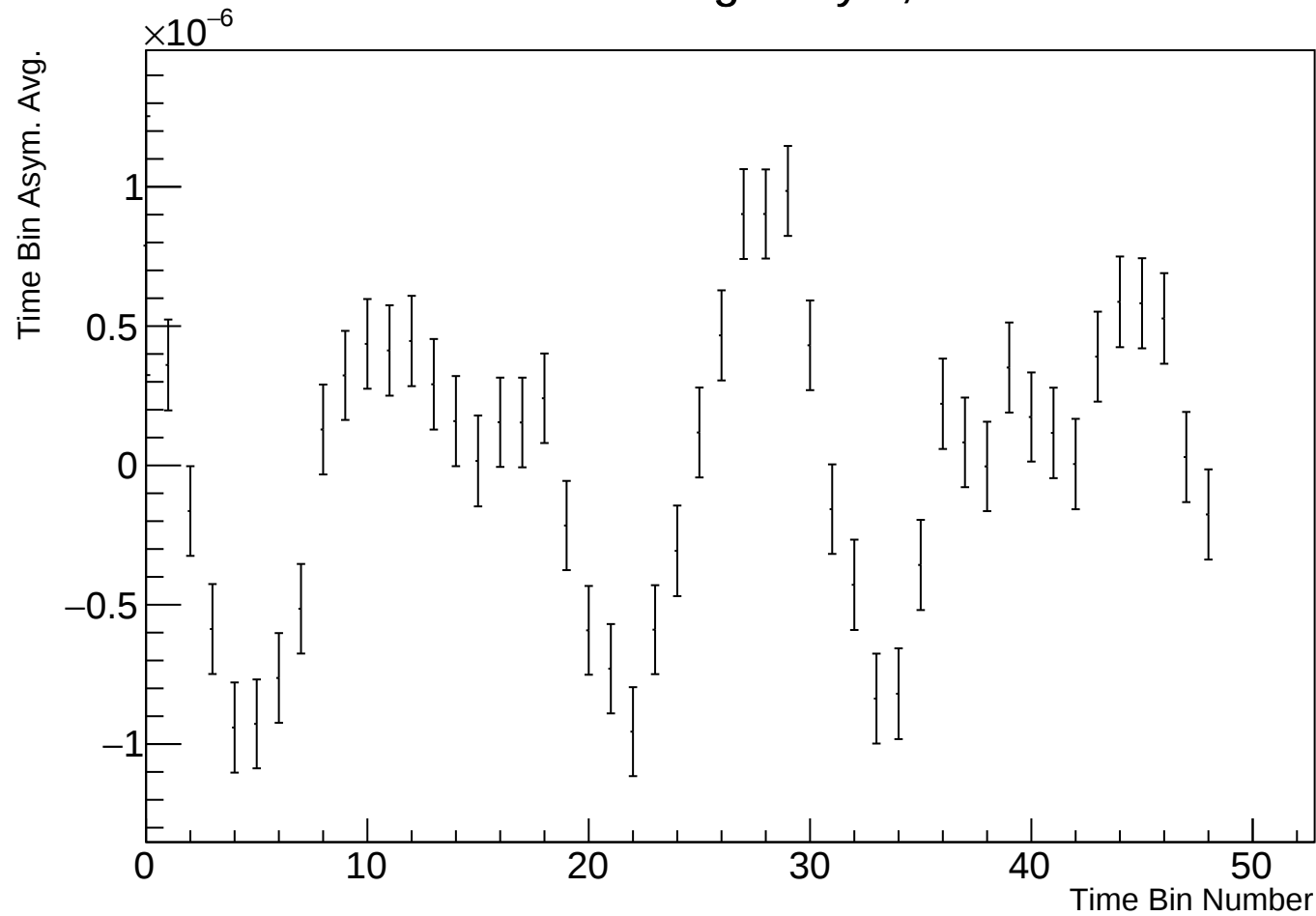
Time Bin Run Average Asym, r38314 w77
