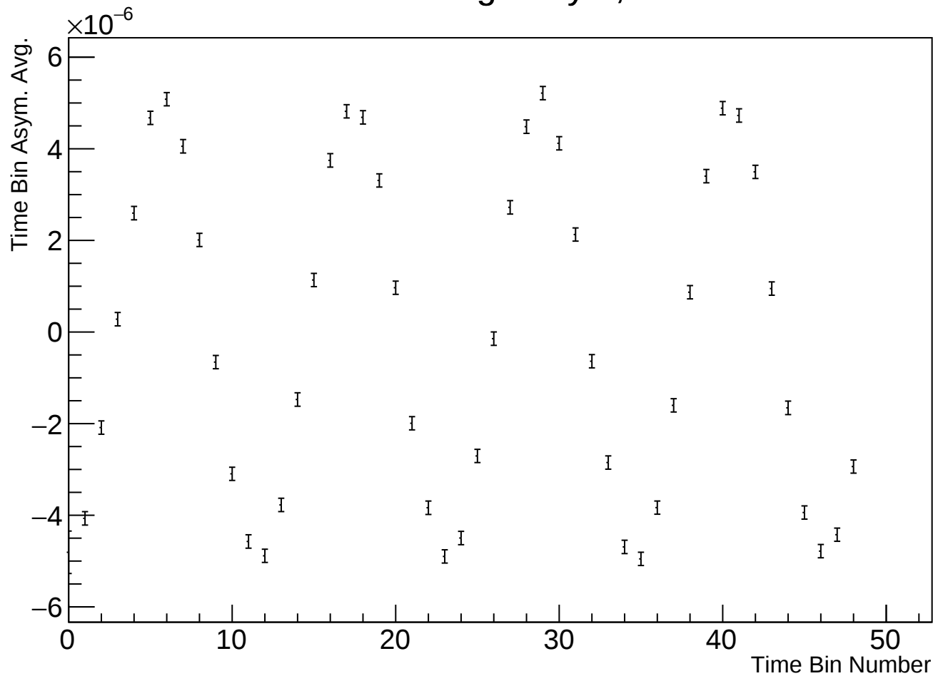
Time Bin Run Average Asym, r38314 w135
