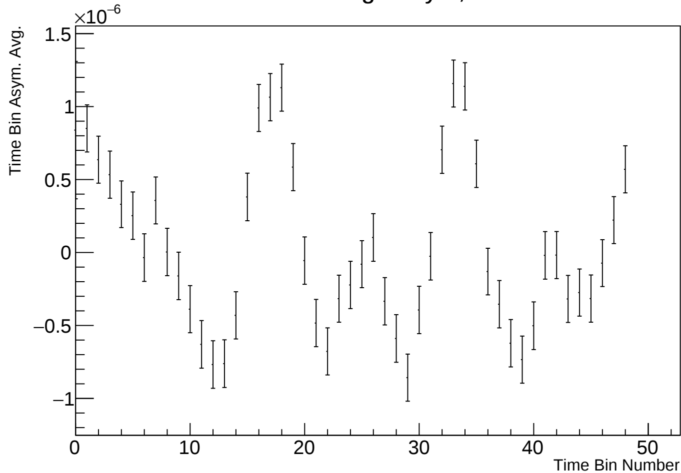
Time Bin Run Average Asym, r38314 w104
