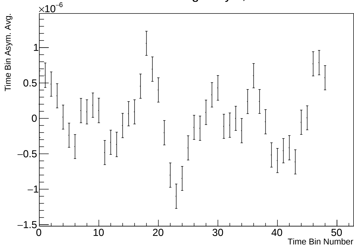
Time Bin Run Average Asym, r38314 w79
