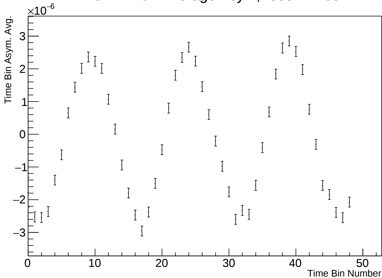
Time Bin Run Average Asym, r38314 w55
