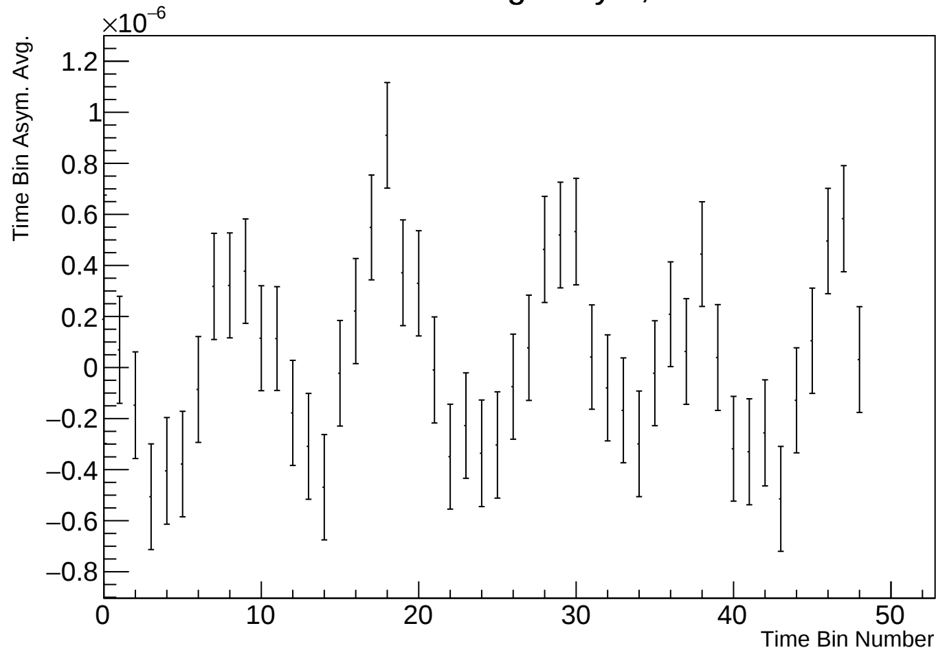
Time Bin Run Average Asym, r38314 w75
