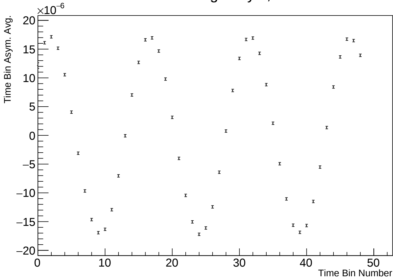
Time Bin Run Average Asym, r38314 w47
