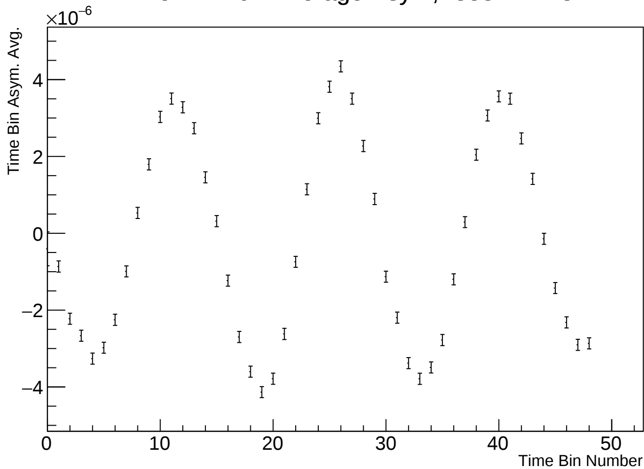
Time Bin Run Average Asym, r38314 w18
