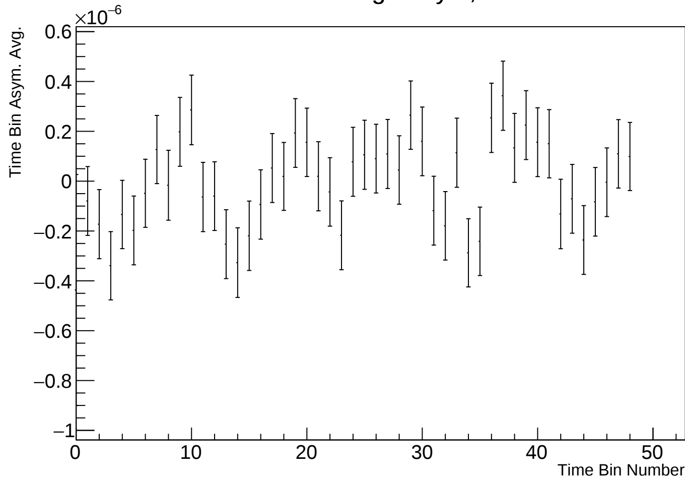
Time Bin Run Average Asym, r38314 w82
