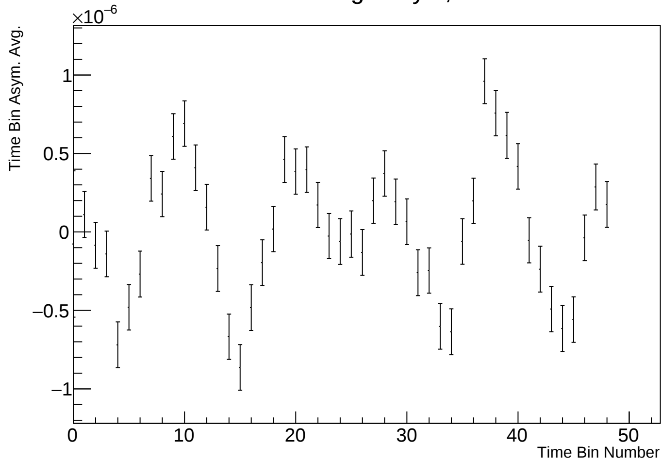
Time Bin Run Average Asym, r38314 w138
