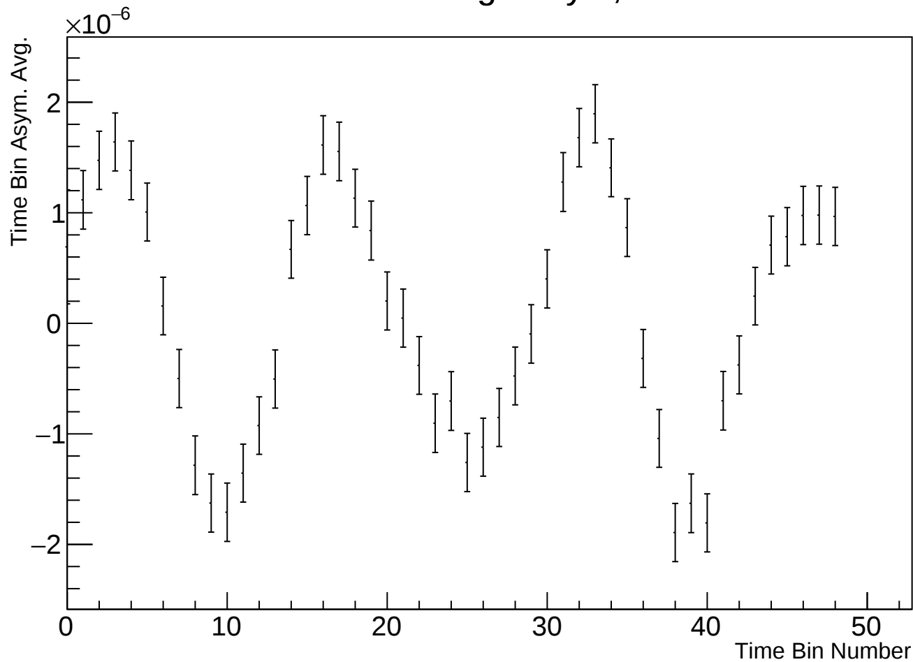
Time Bin Run Average Asym, r38314 w68
