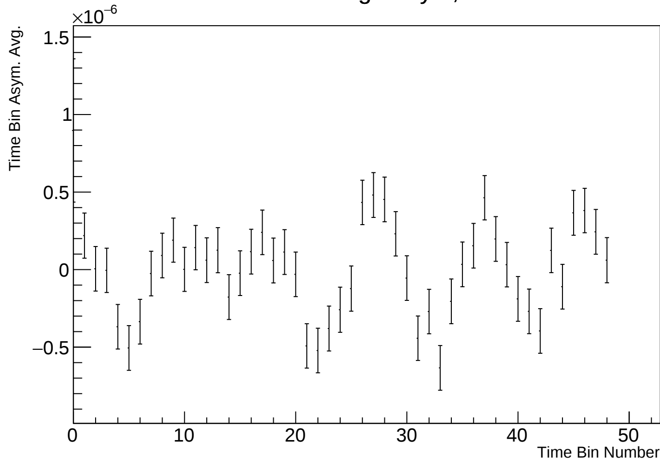
Time Bin Run Average Asym, r38314 w74
