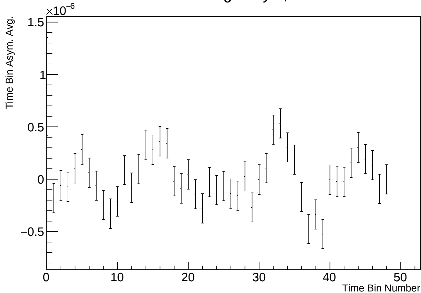
Time Bin Run Average Asym, r38314 w130
