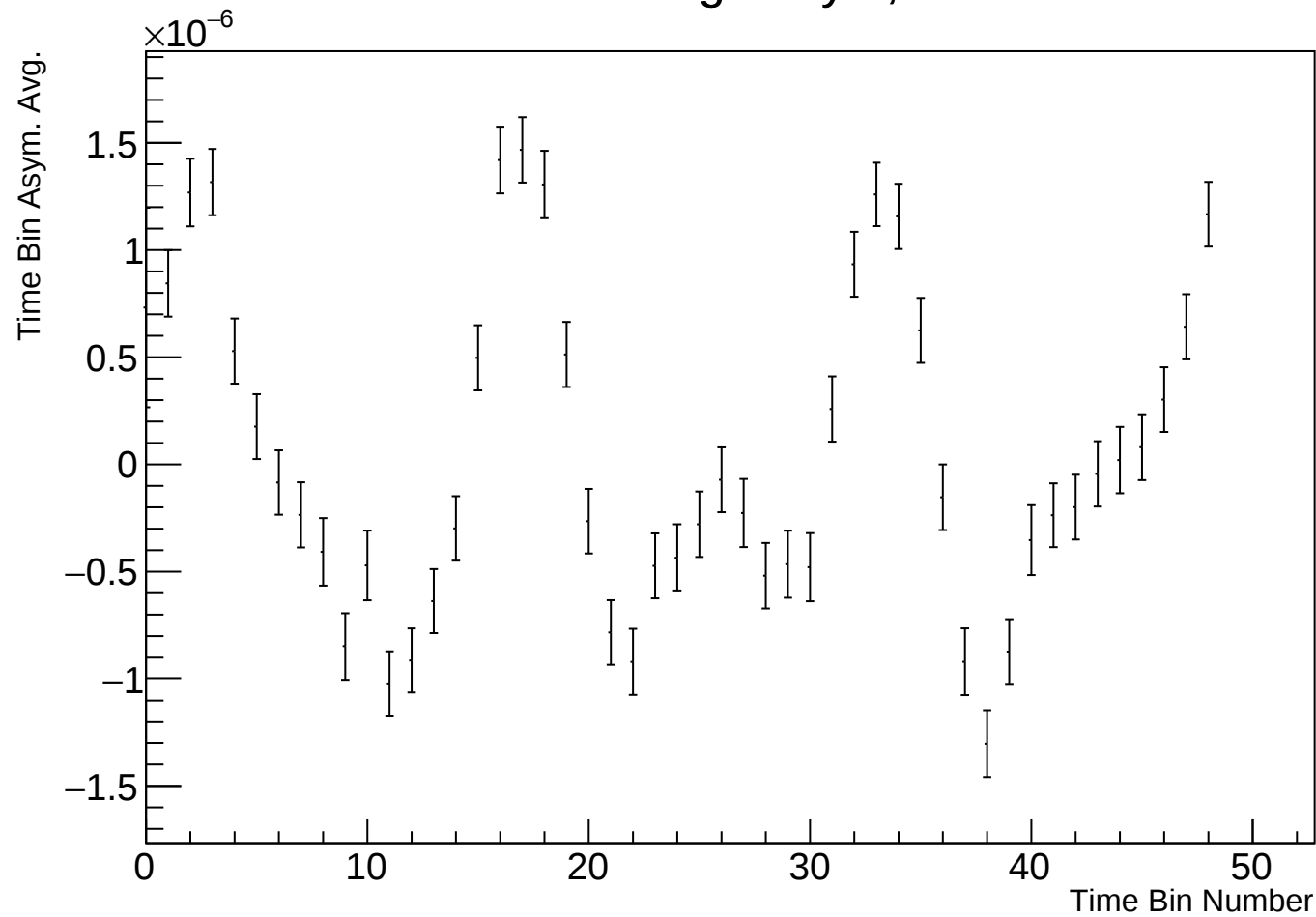
Time Bin Run Average Asym, r38314 w106
