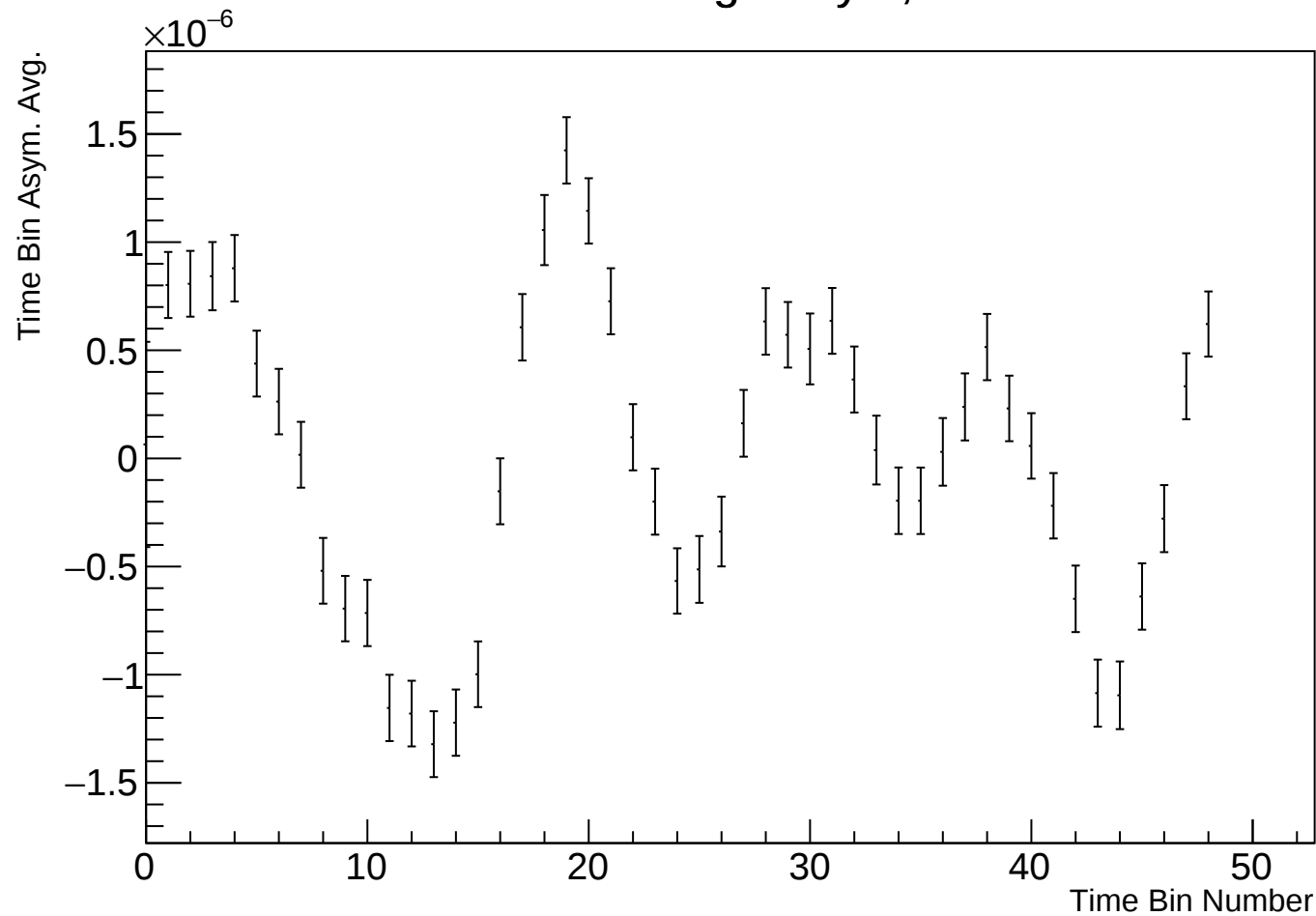
Time Bin Run Average Asym, r38314 w89
