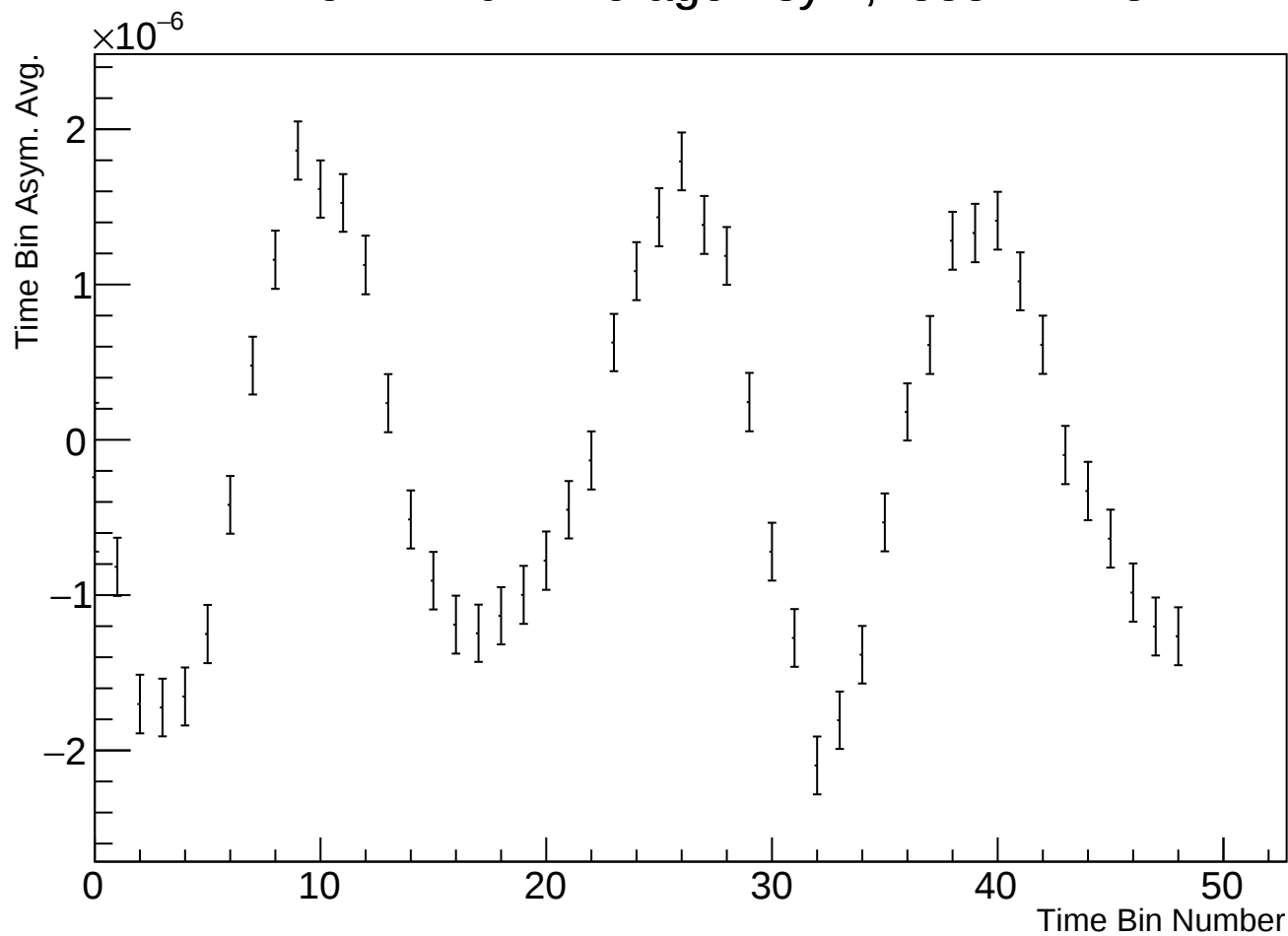
Time Bin Run Average Asym, r38314 w78
