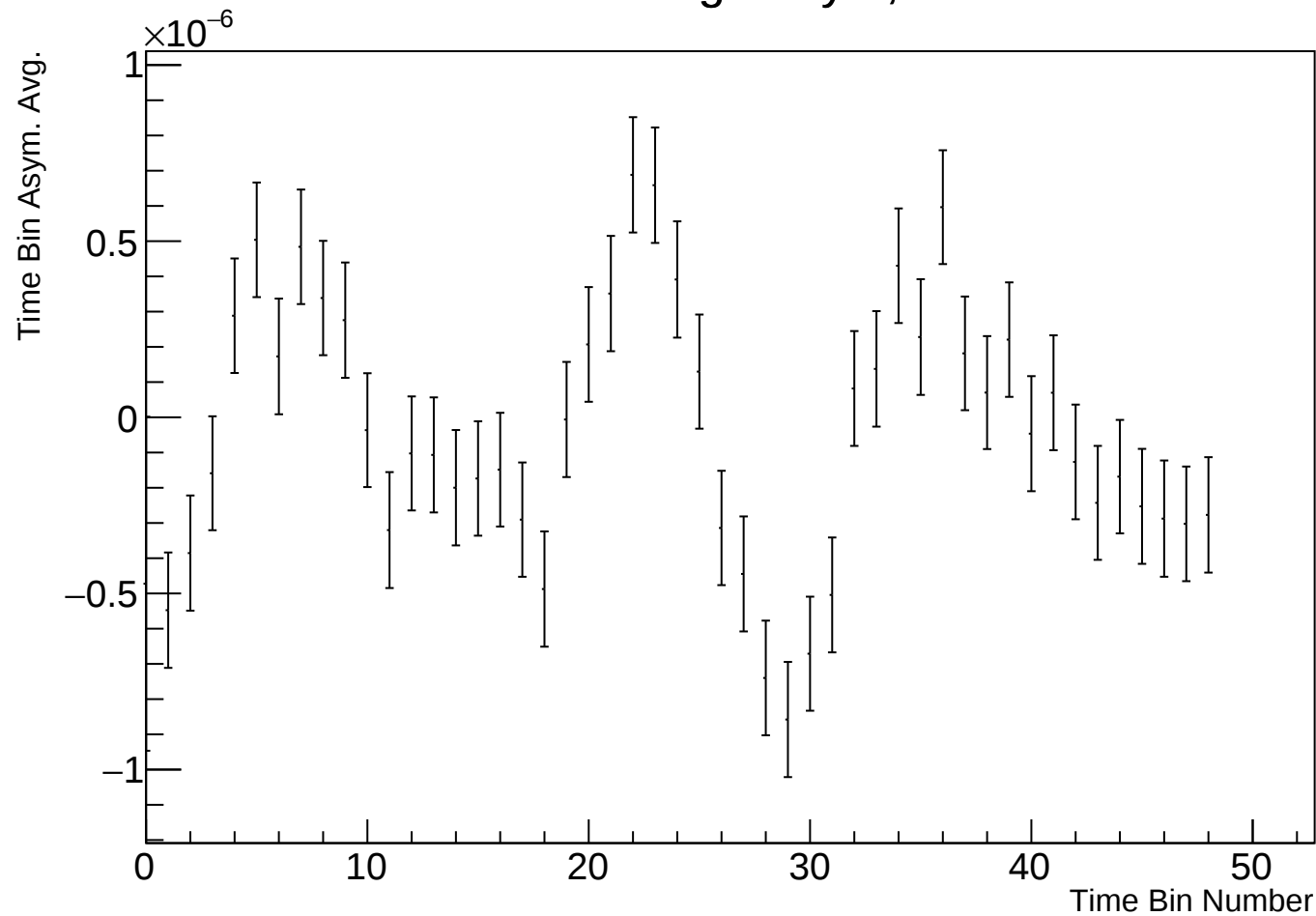
Time Bin Run Average Asym, r38314 w132
