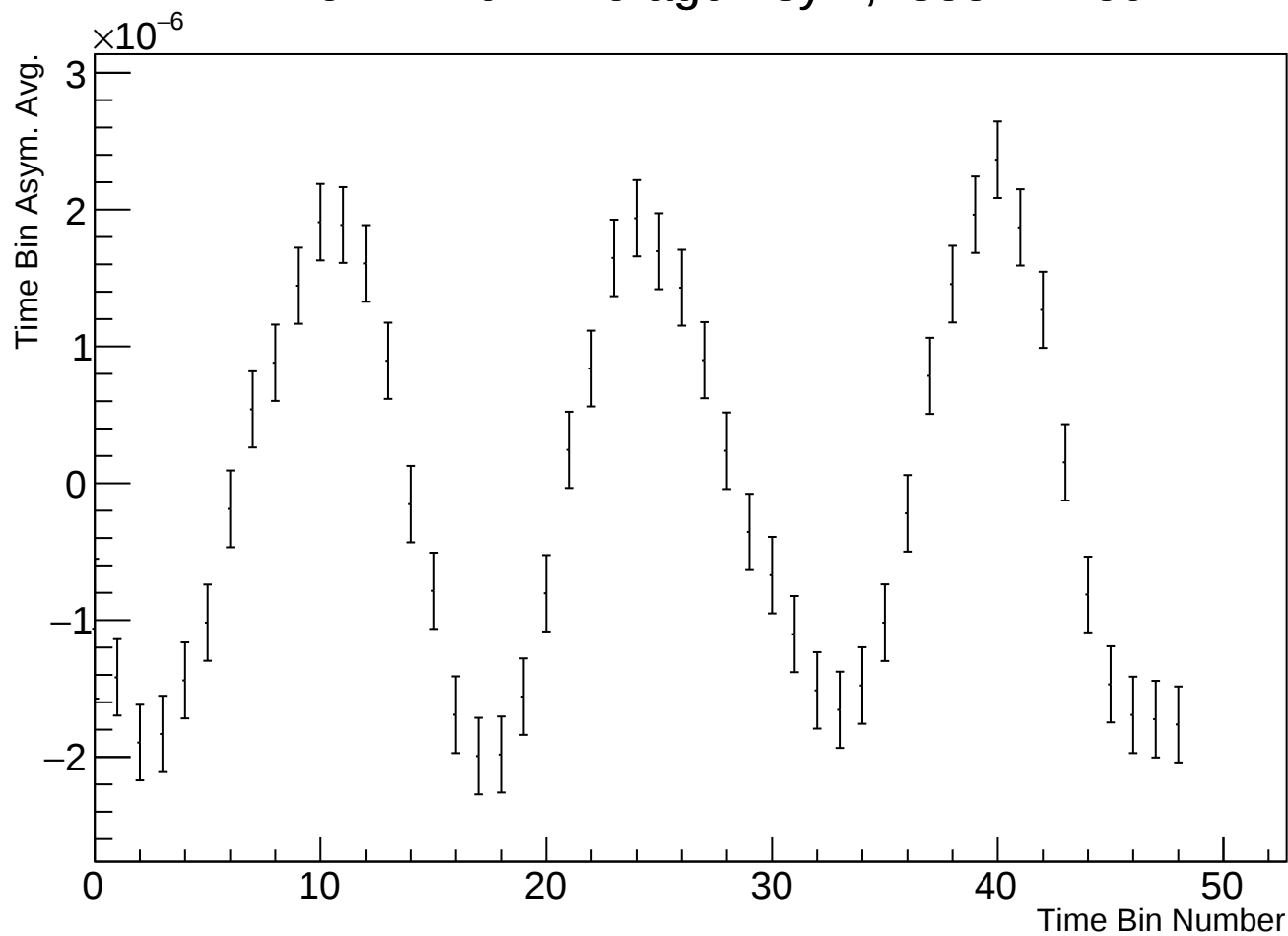
Time Bin Run Average Asym, r38314 w59
