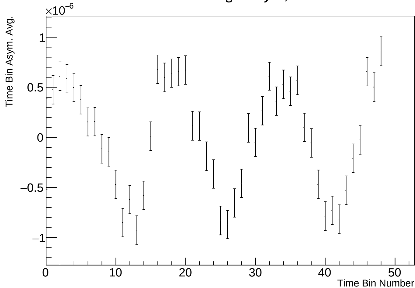
Time Bin Run Average Asym, r38314 w53
