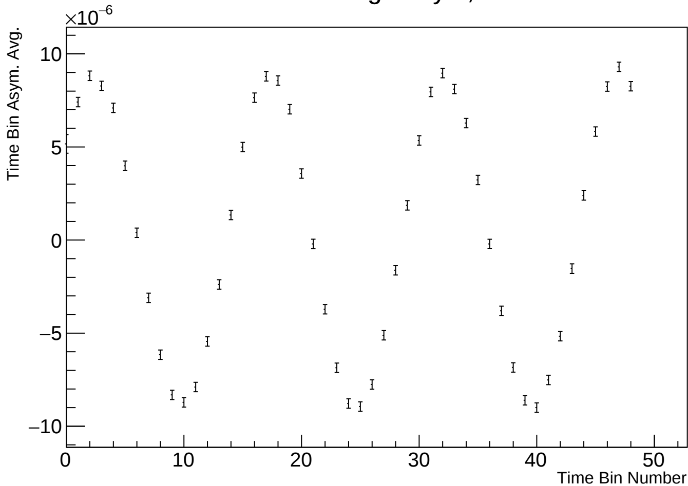
Time Bin Run Average Asym, r38314 w48
