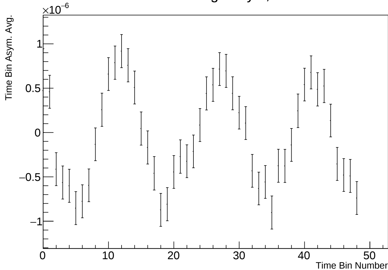
Time Bin Run Average Asym, r38314 w28
