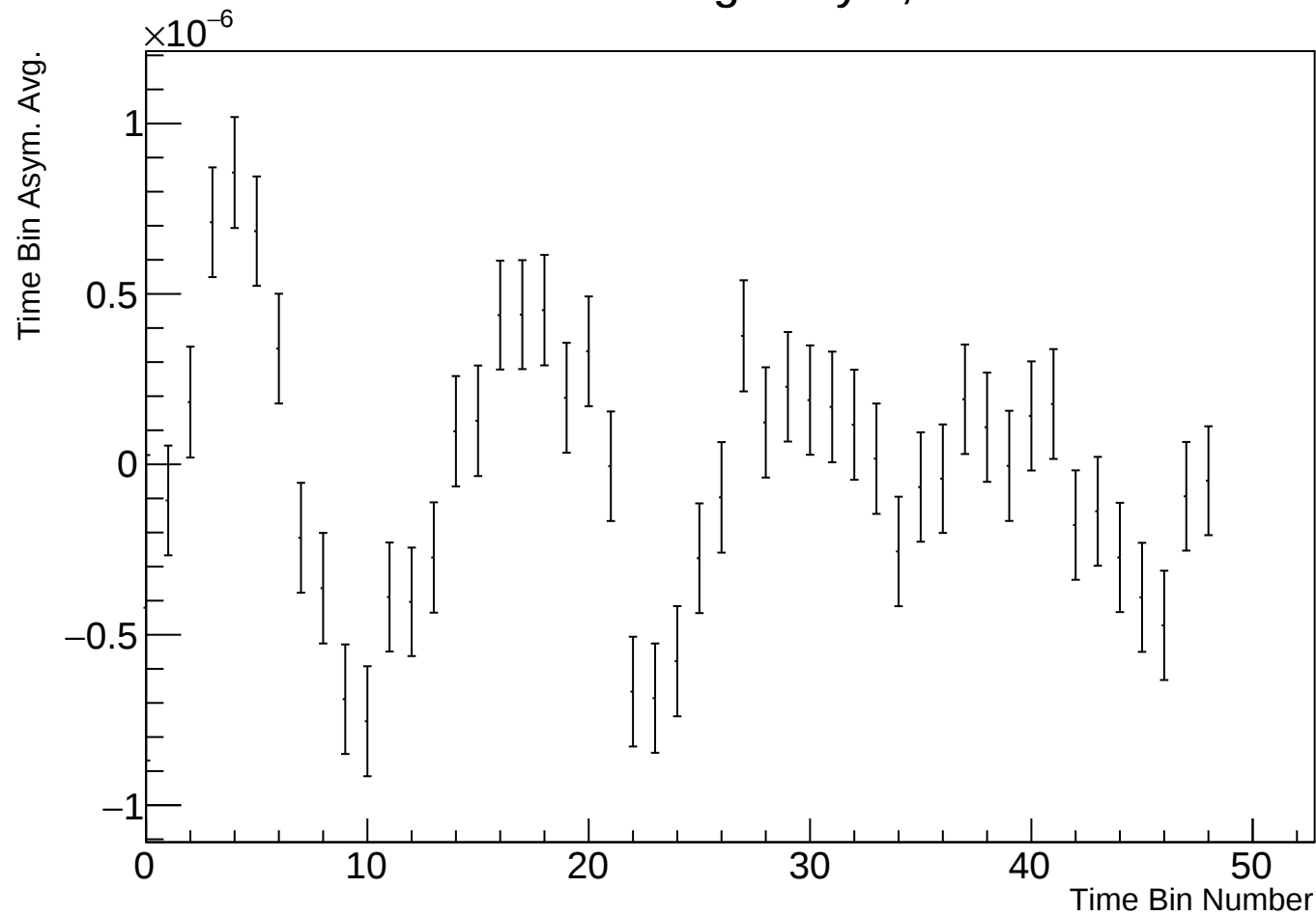
Time Bin Run Average Asym, r38314 w24
