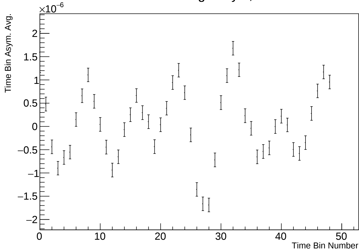
Time Bin Run Average Asym, r38314 w6
