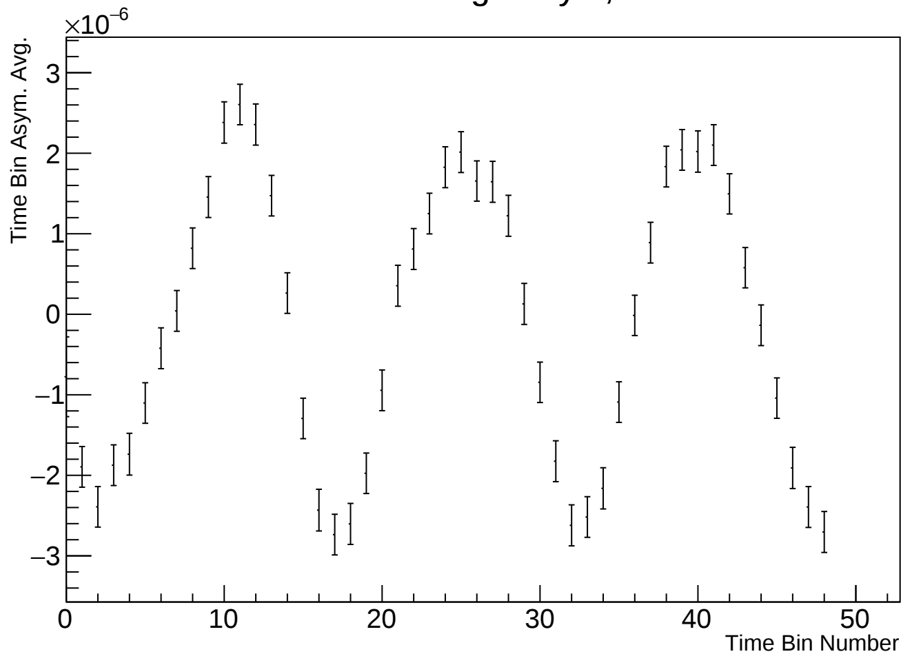
Time Bin Run Average Asym, r38314 w58
