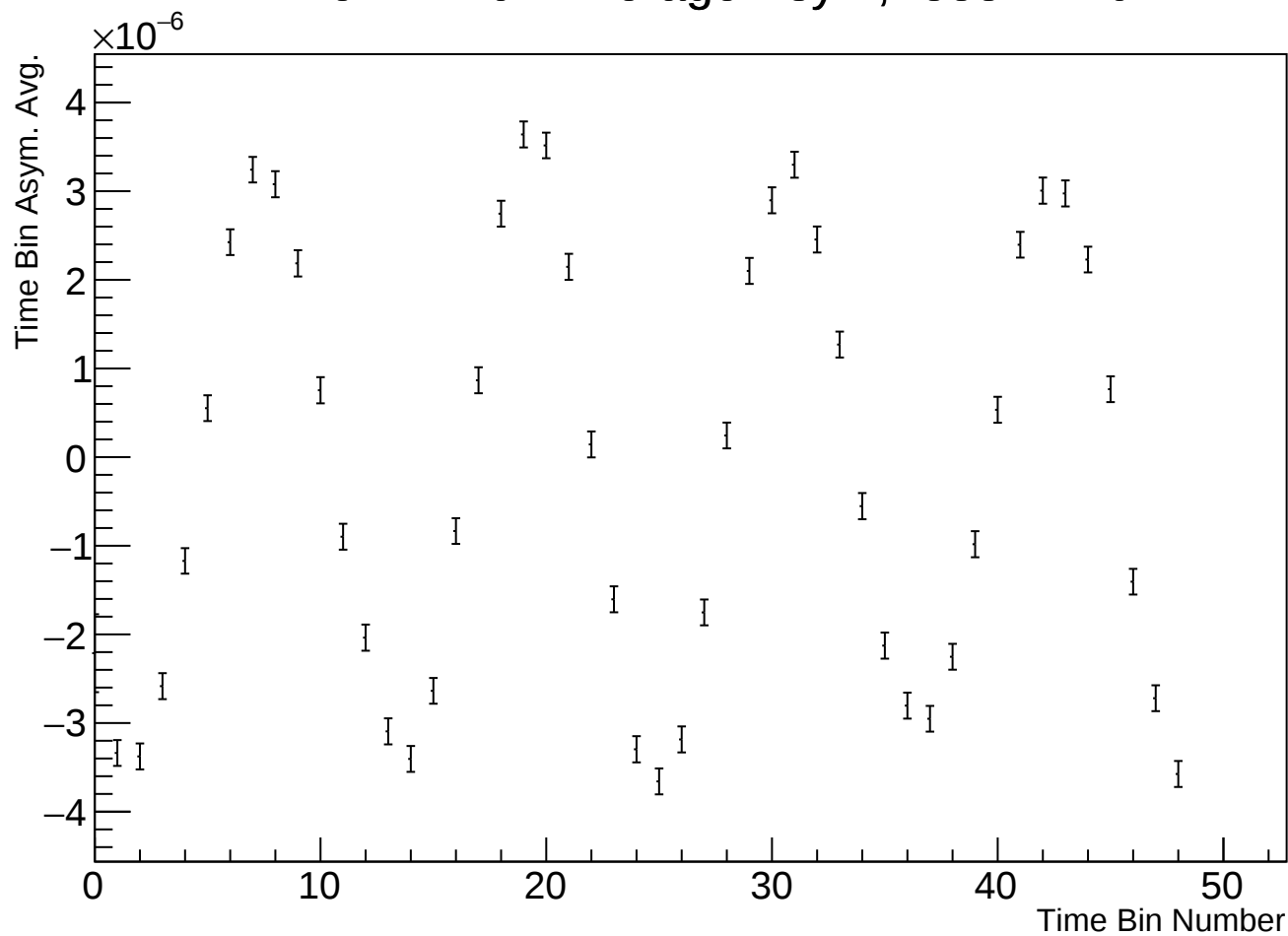
Time Bin Run Average Asym, r38314 w0
