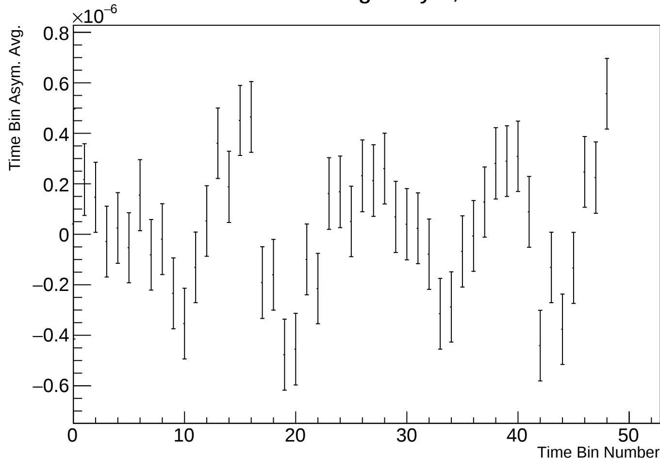
Time Bin Run Average Asym, r38314 w16
