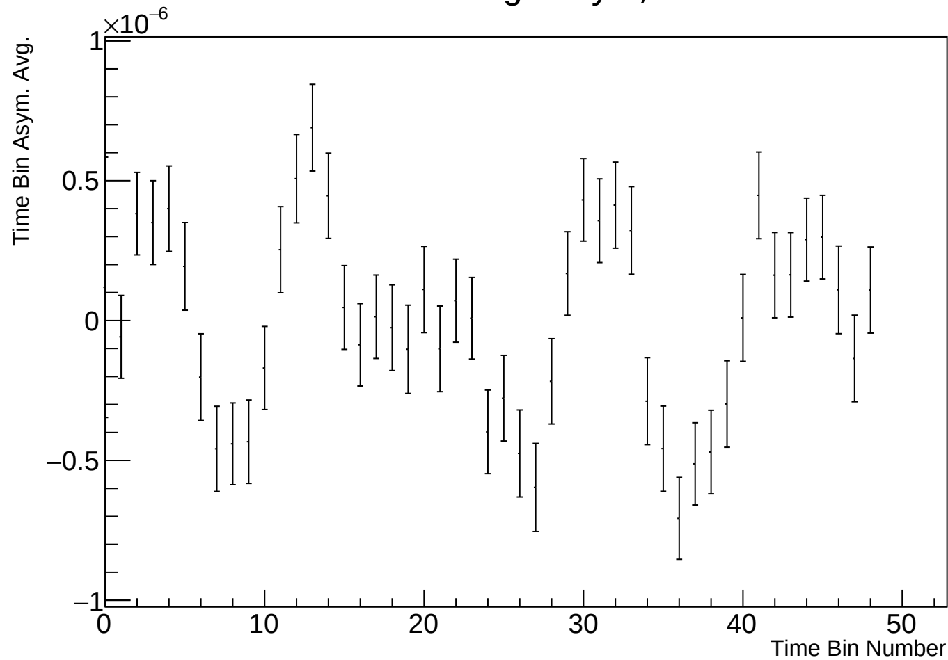
Time Bin Run Average Asym, r38314 w115
