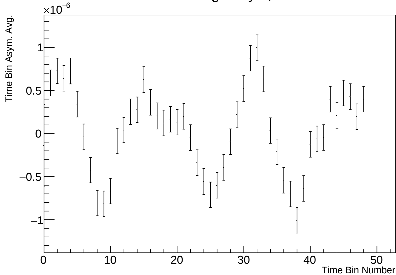
Time Bin Run Average Asym, r38314 w111
