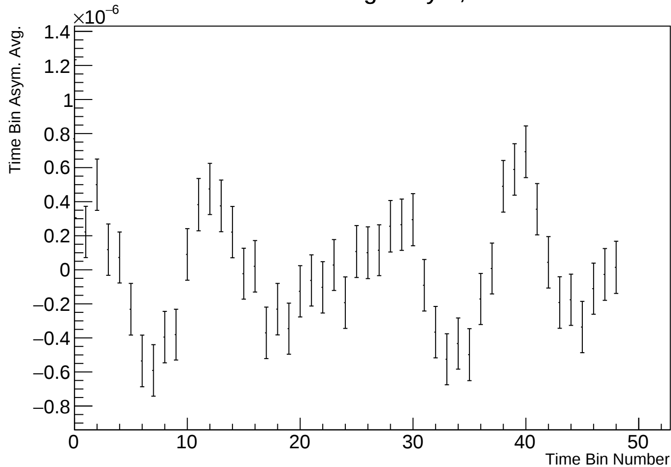
Time Bin Run Average Asym, r38314 w34
