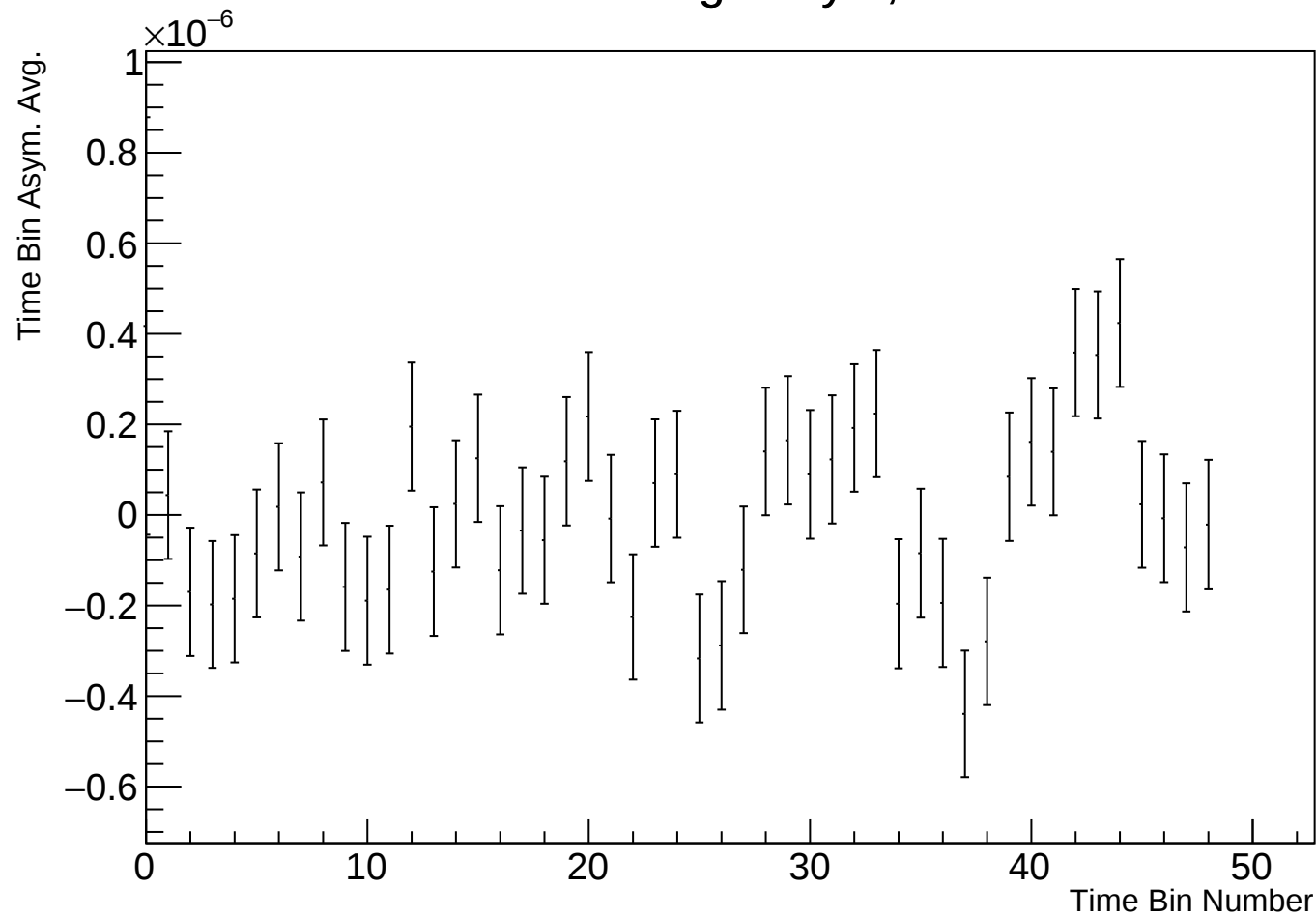
Time Bin Run Average Asym, r38314 w134
