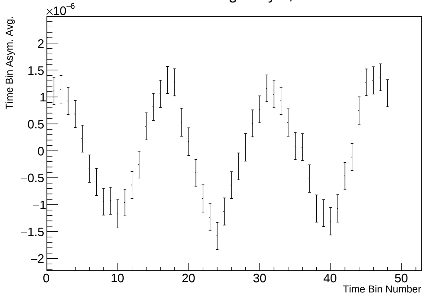
Time Bin Run Average Asym, r38314 w49
