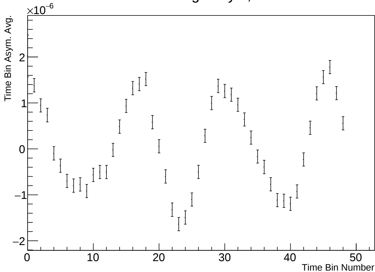
Time Bin Run Average Asym, r38314 w122
