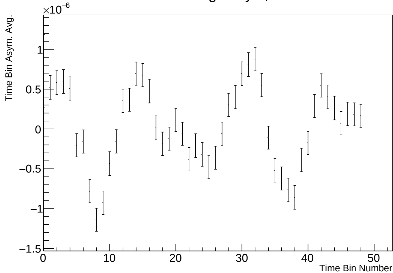
Time Bin Run Average Asym, r38314 w114
