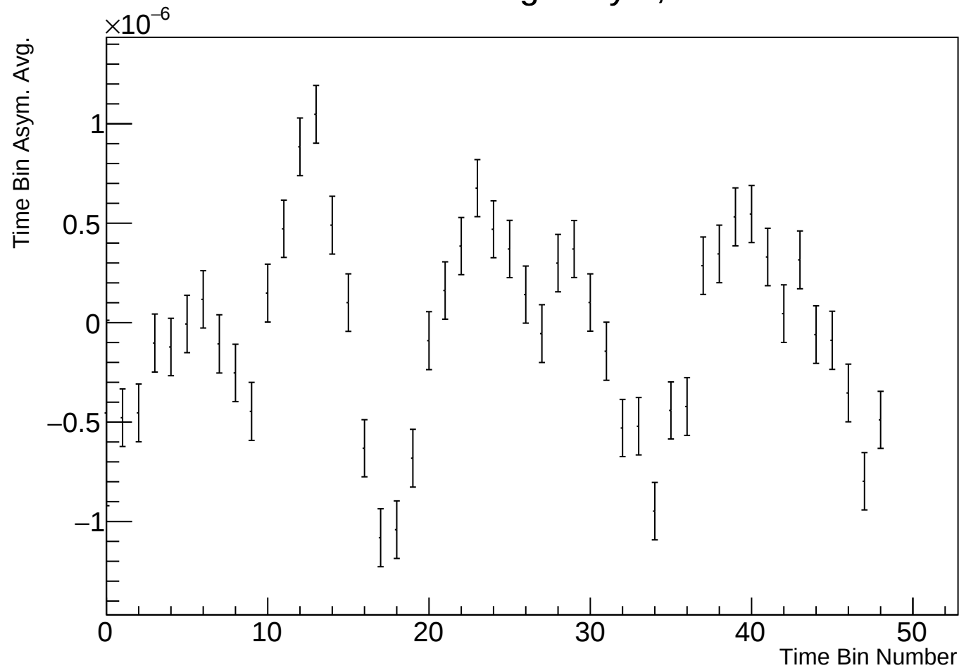
Time Bin Run Average Asym, r38314 w97
