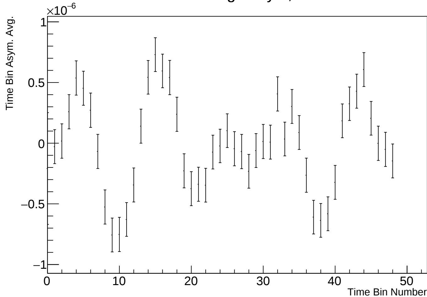
Time Bin Run Average Asym, r38314 w137
