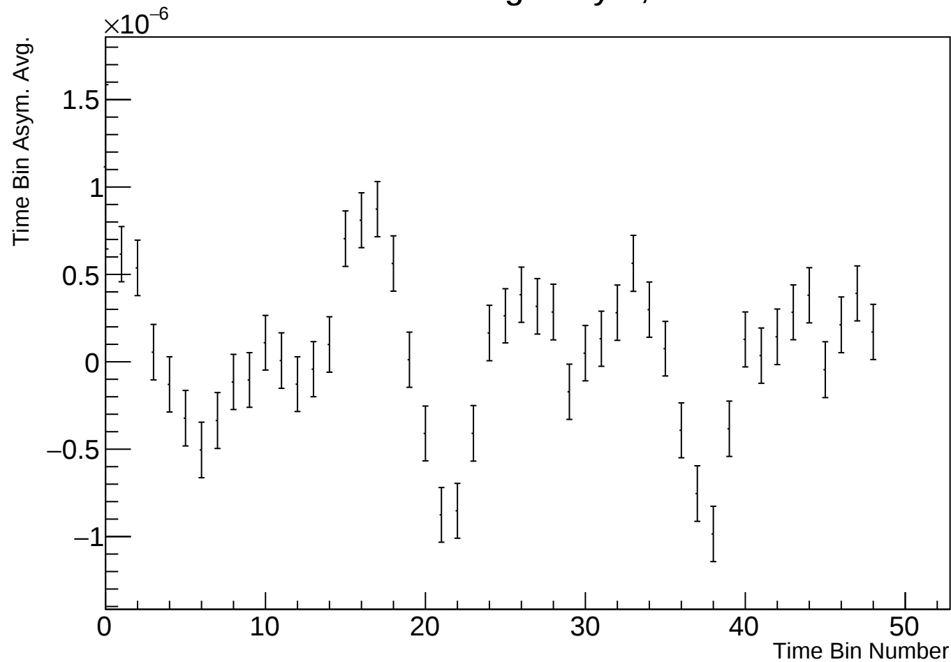
Time Bin Run Average Asym, r38314 w100
