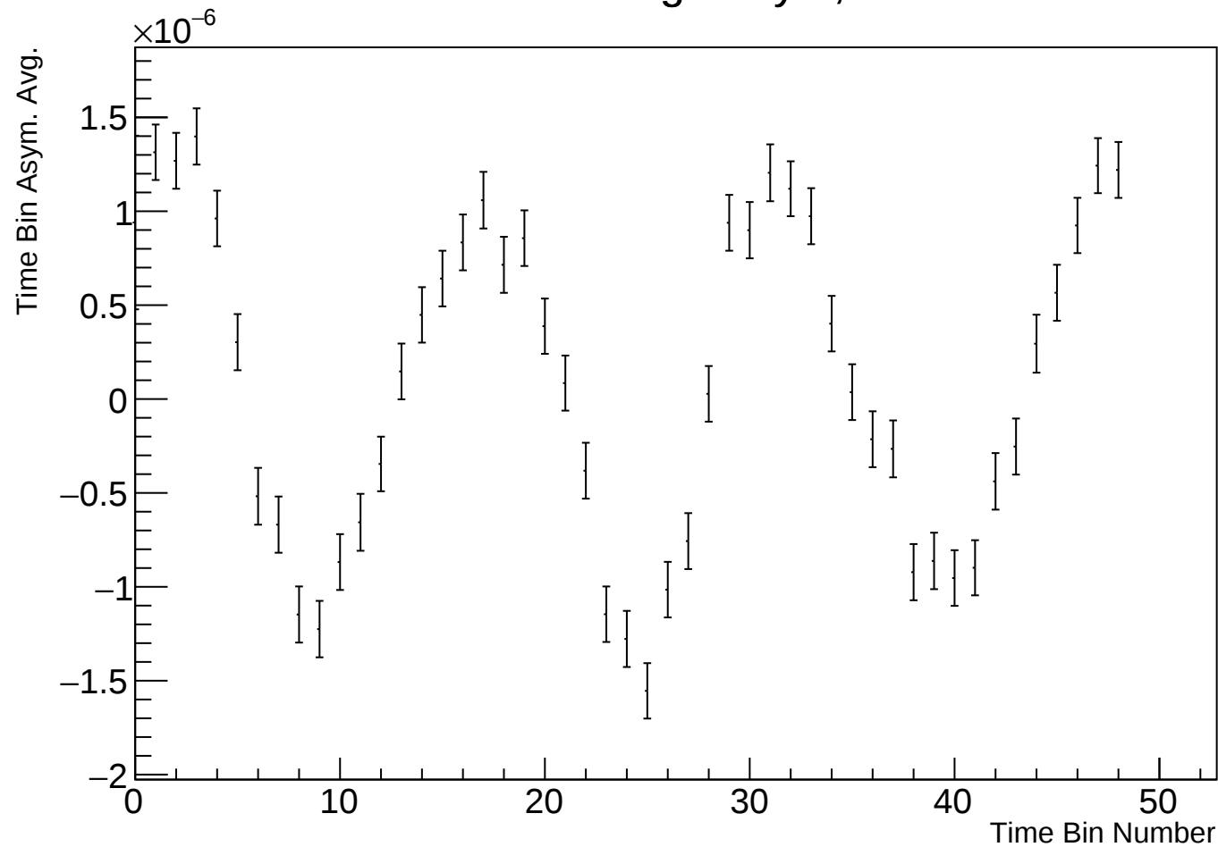
Time Bin Run Average Asym, r38314 w30
