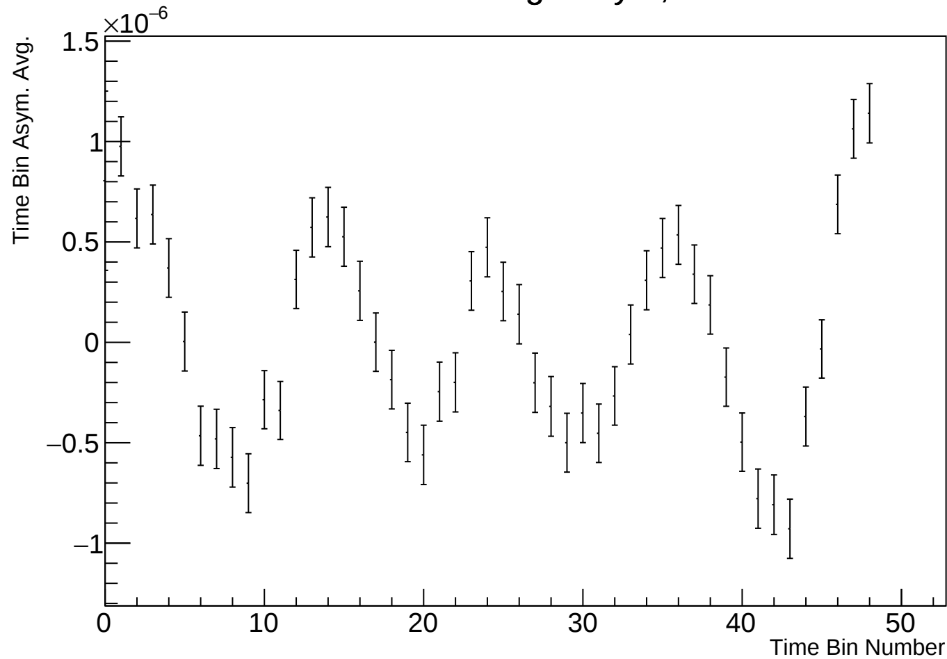
Time Bin Run Average Asym, r38314 w1
