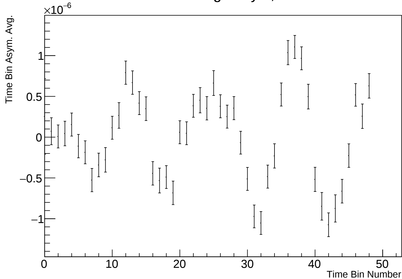
Time Bin Run Average Asym, r38314 w143
