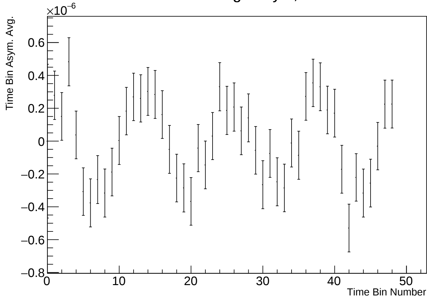
Time Bin Run Average Asym, r38314 w81
