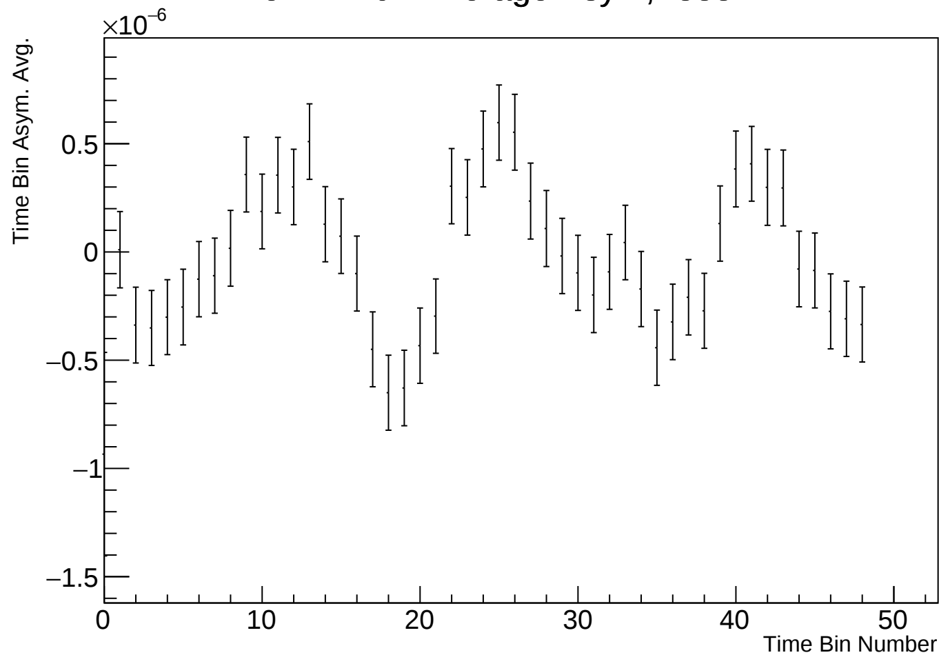
Time Bin Run Average Asym, r38314 w71
