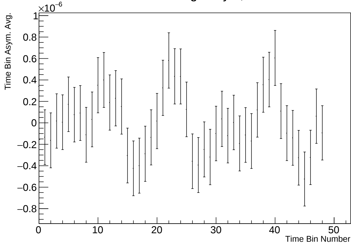
Time Bin Run Average Asym, r38314 w60
