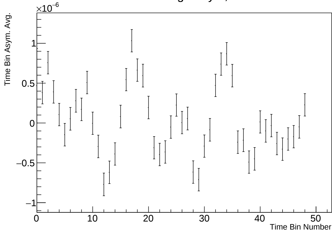
Time Bin Run Average Asym, r38314 w101
