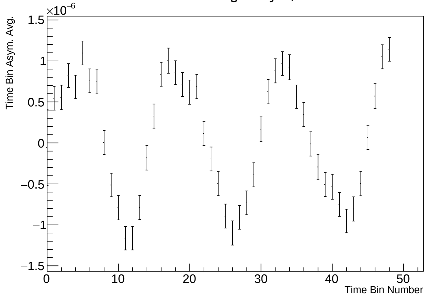
Time Bin Run Average Asym, r38314 w13
