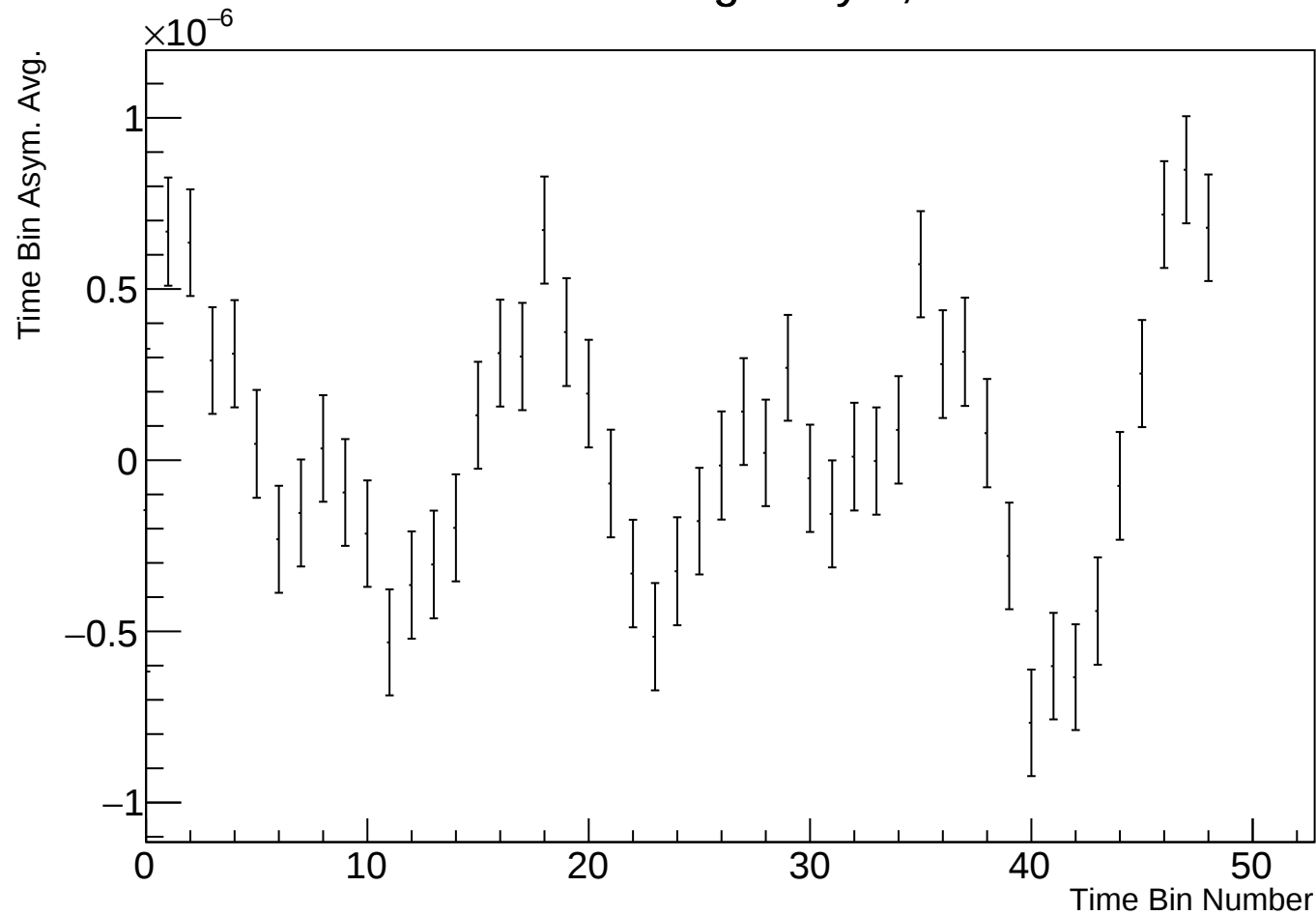
Time Bin Run Average Asym, r38314 w80
