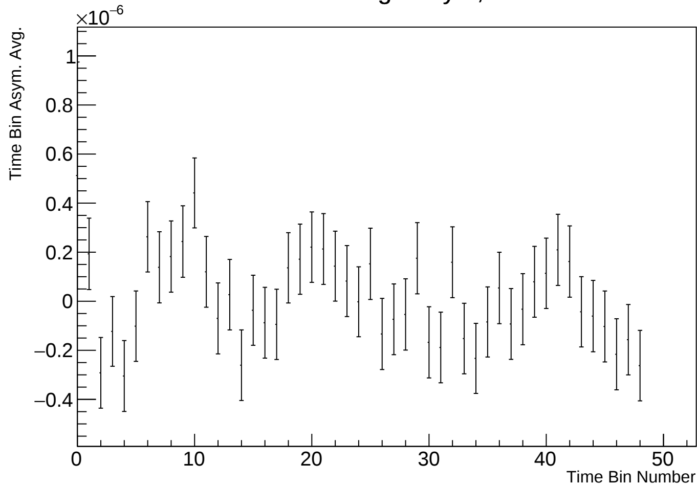
Time Bin Run Average Asym, r38314 w84
