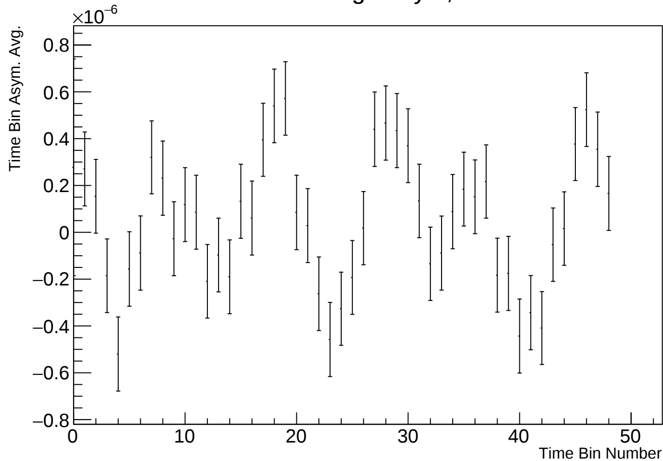
Time Bin Run Average Asym, r38314 w120
