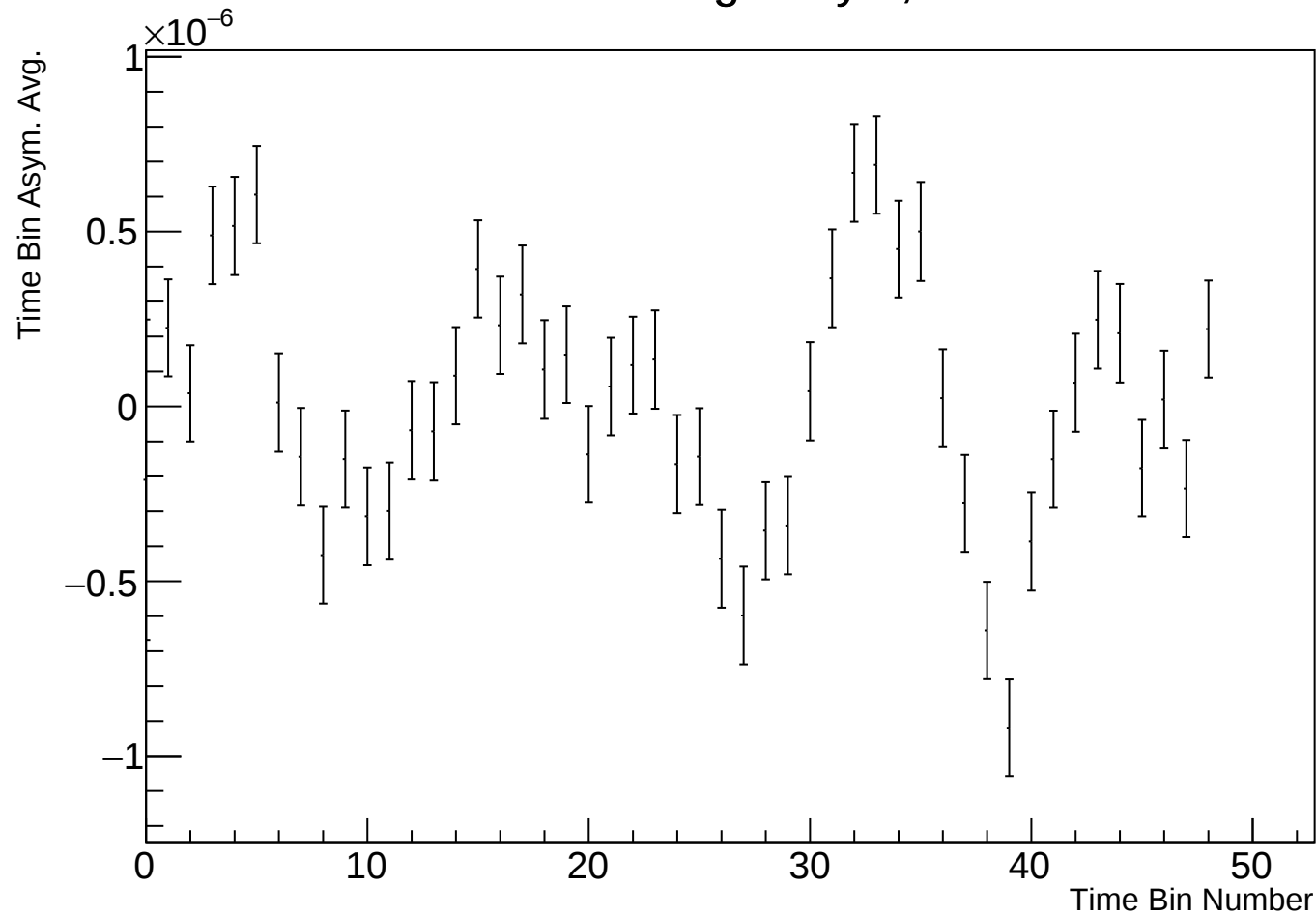
Time Bin Run Average Asym, r38314 w65
