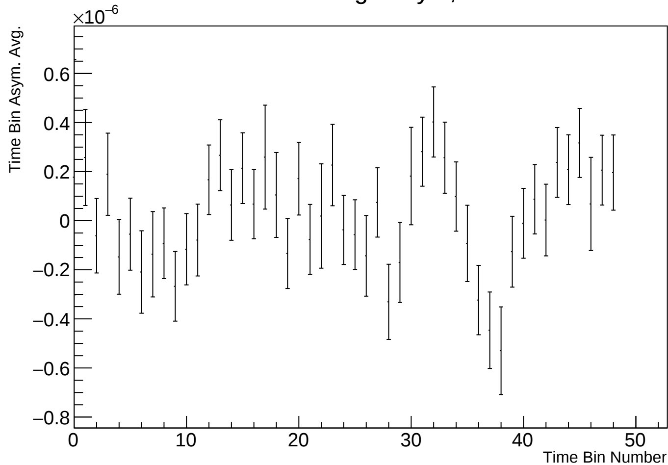
Time Bin Run Average Asym, r38314 w108
