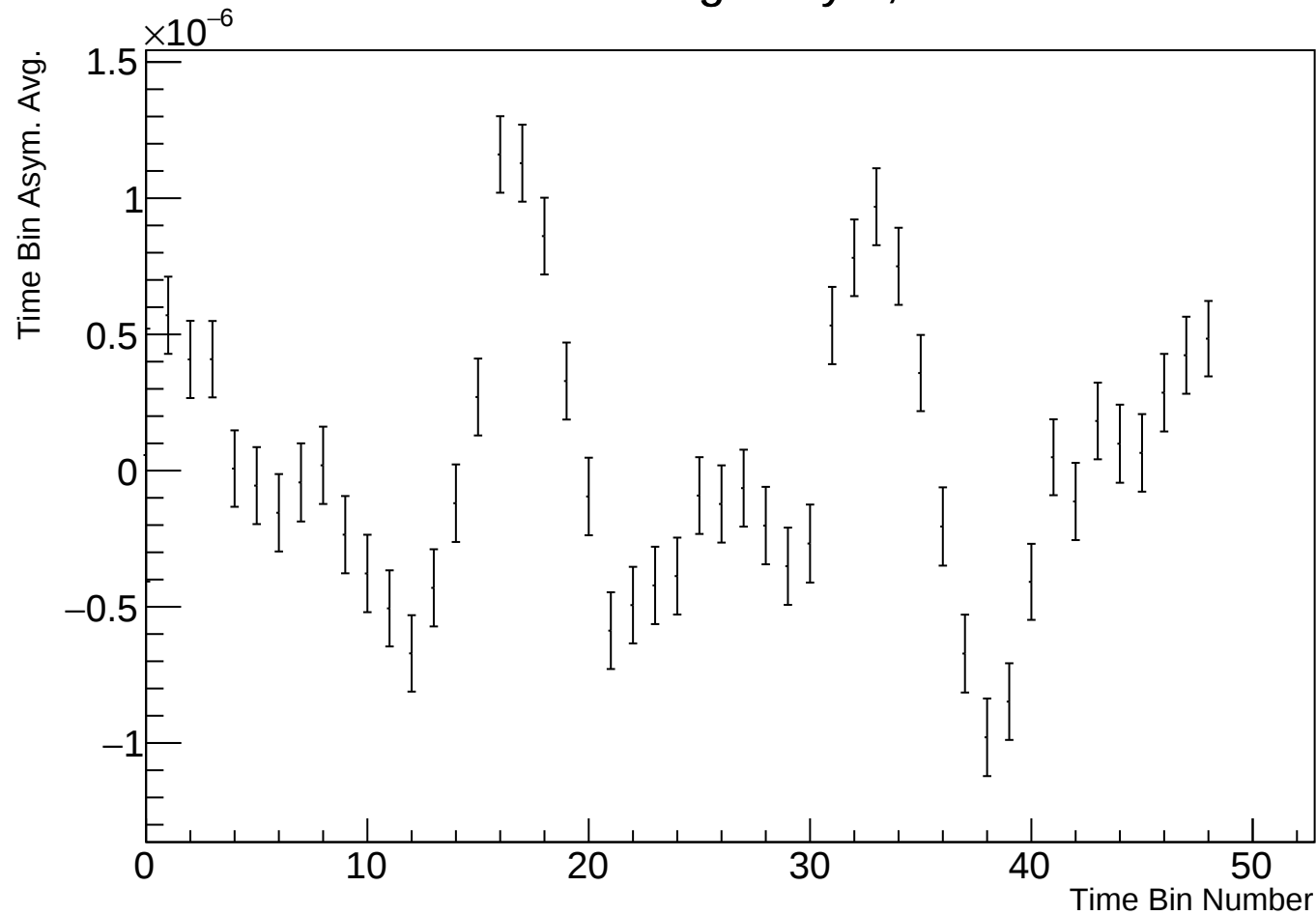
Time Bin Run Average Asym, r38314 w103
