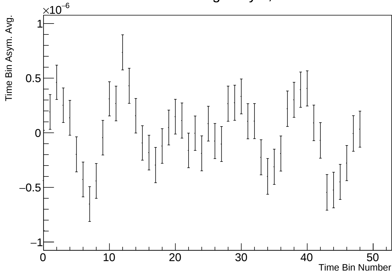
Time Bin Run Average Asym, r38314 w33
