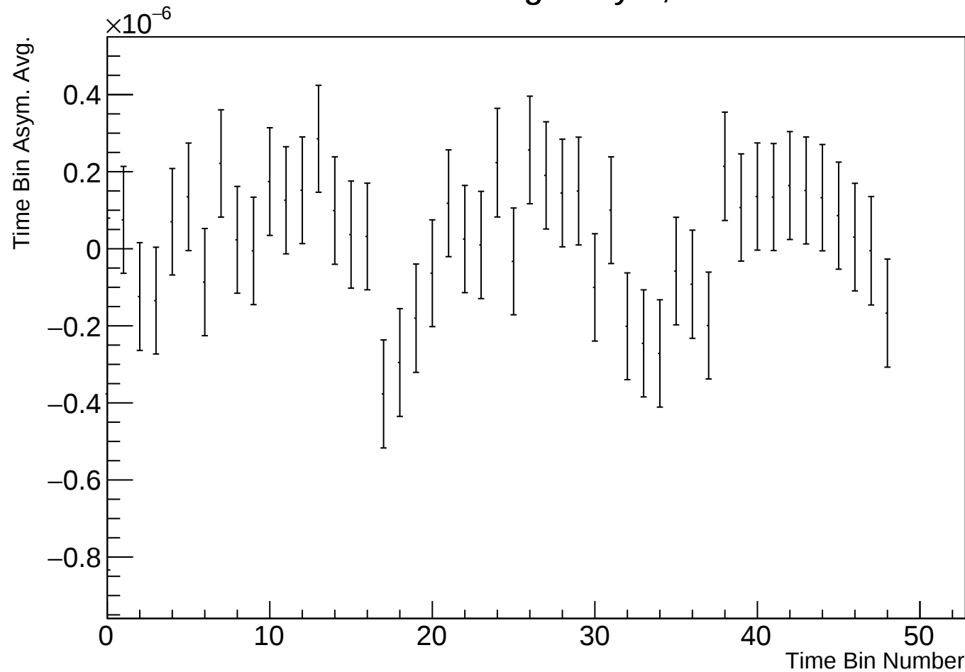
Time Bin Run Average Asym, r38314 w63
