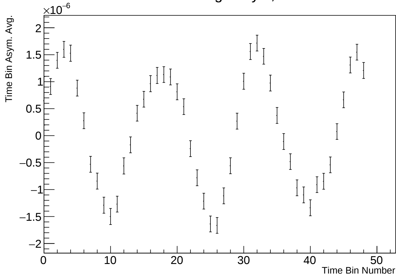
Time Bin Run Average Asym, r38314 w57
