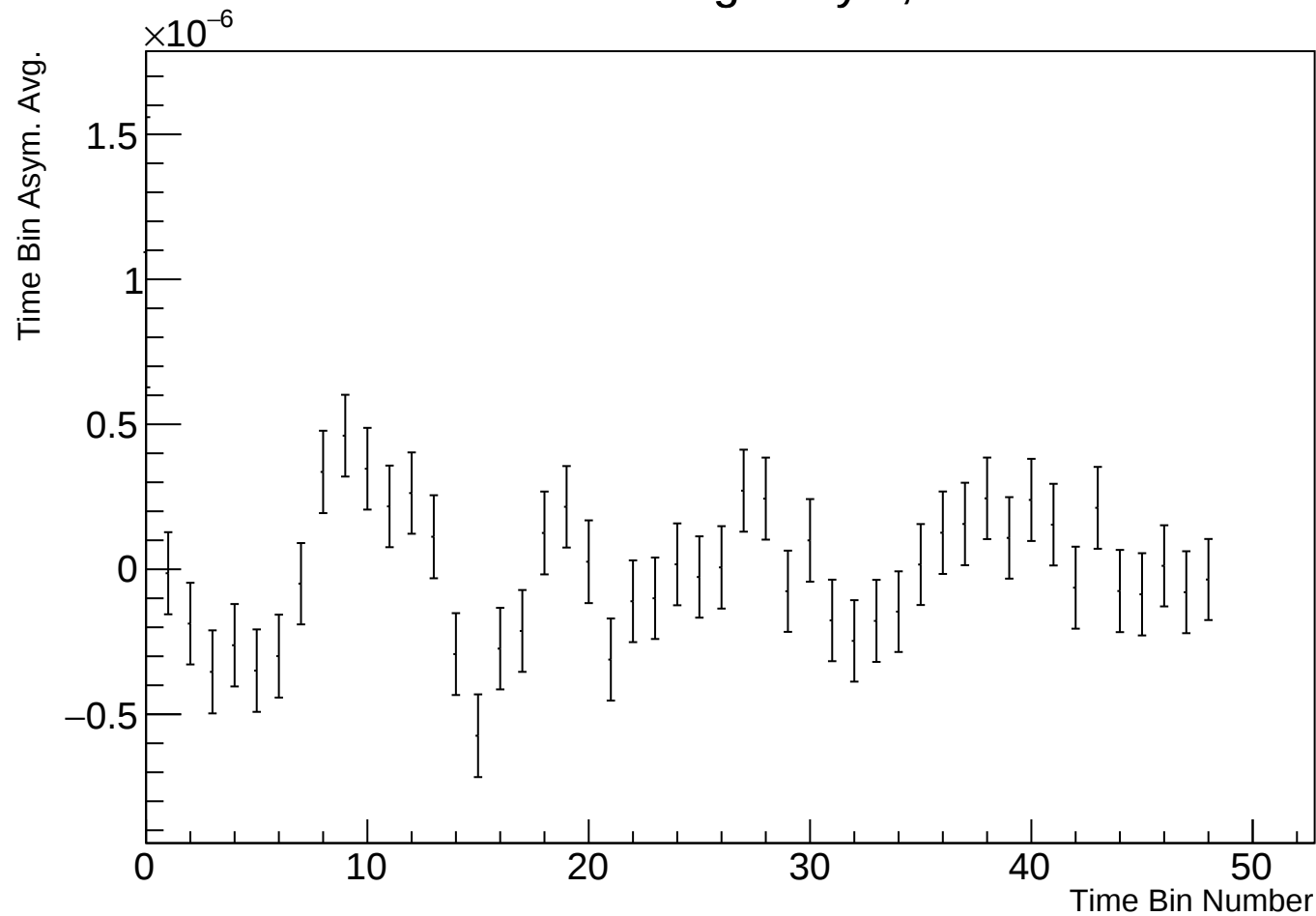
Time Bin Run Average Asym, r38314 w85
