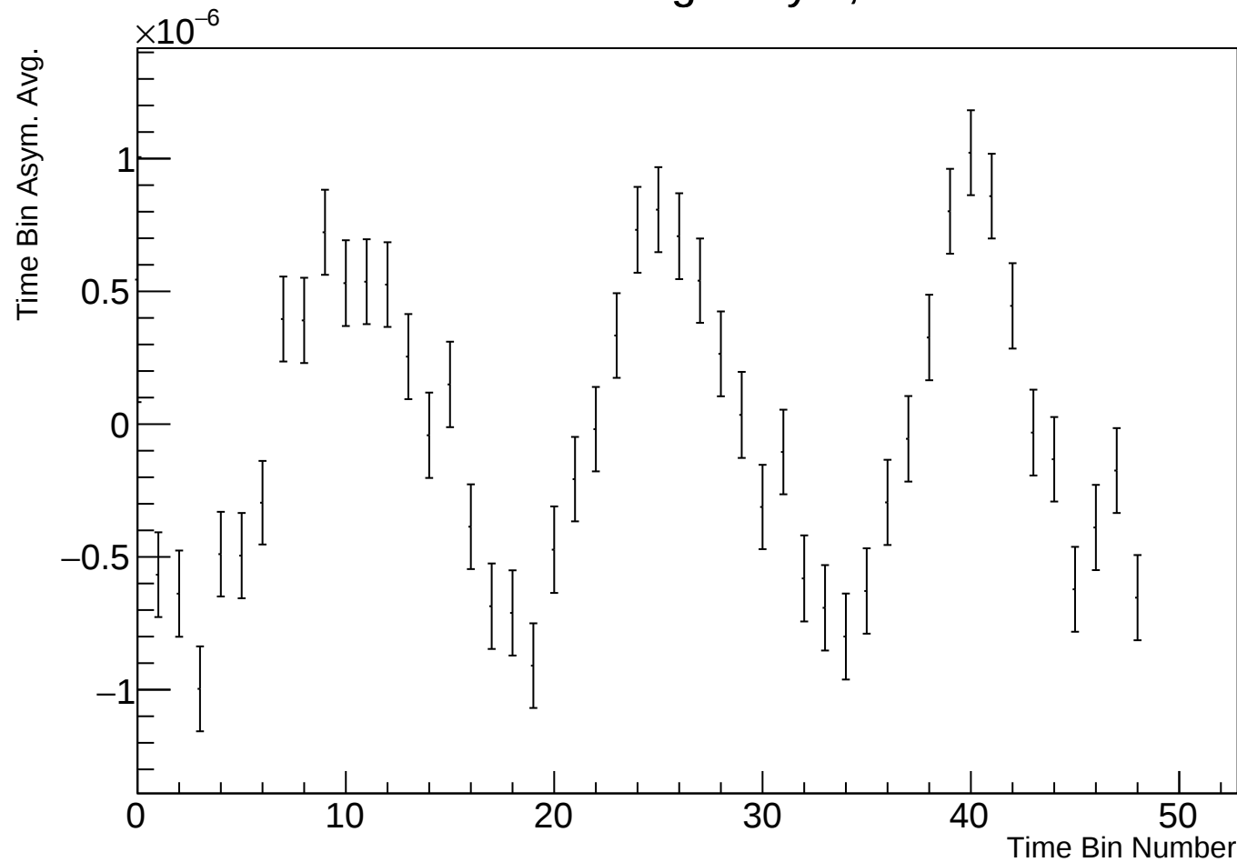
Time Bin Run Average Asym, r38314 w12
