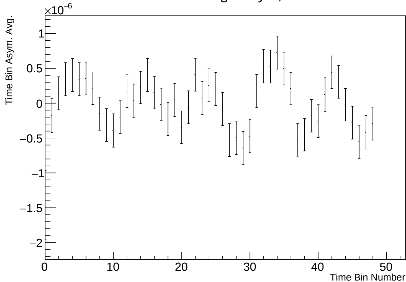
Time Bin Run Average Asym, r38314 w67
