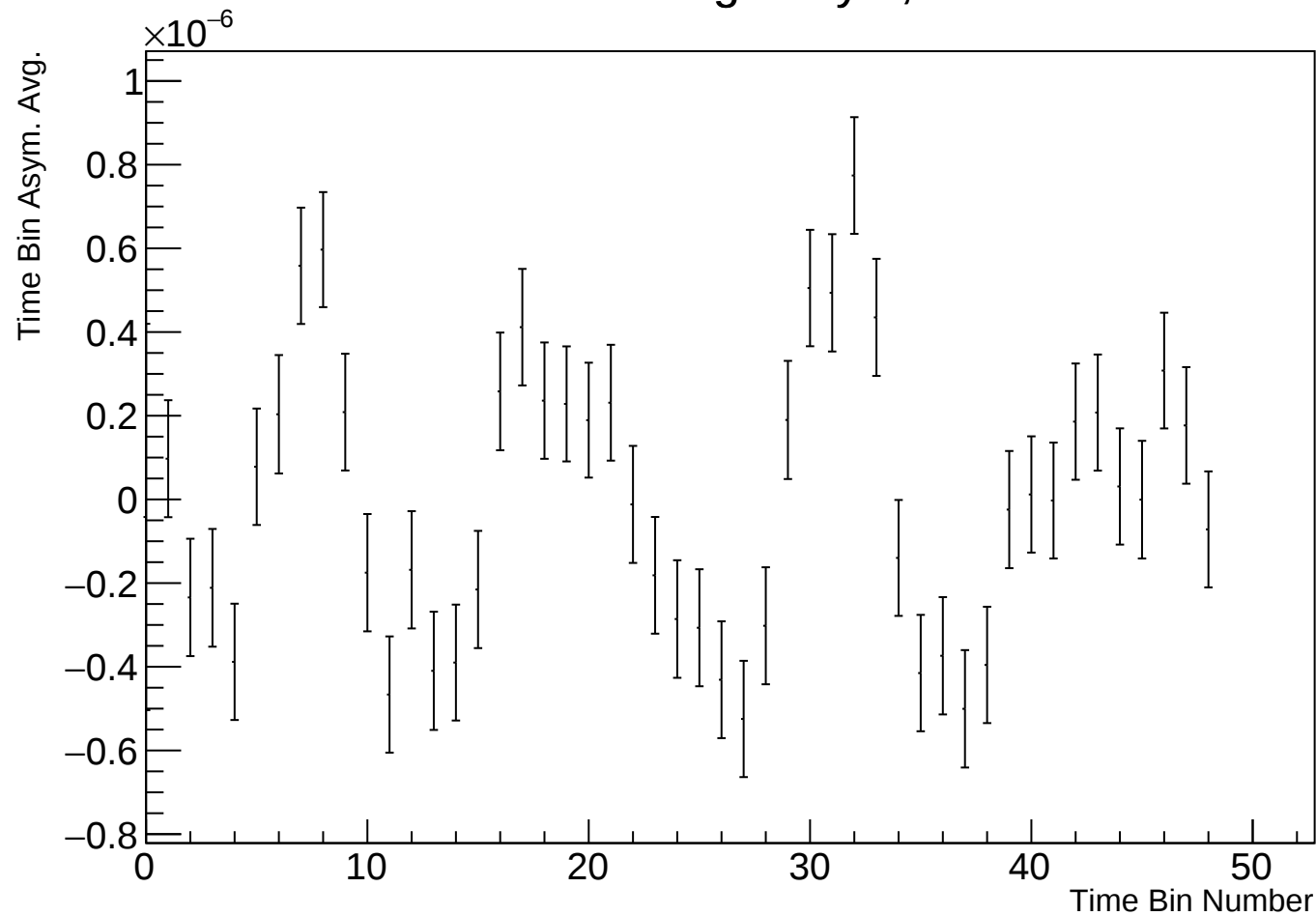
Time Bin Run Average Asym, r38314 w15
