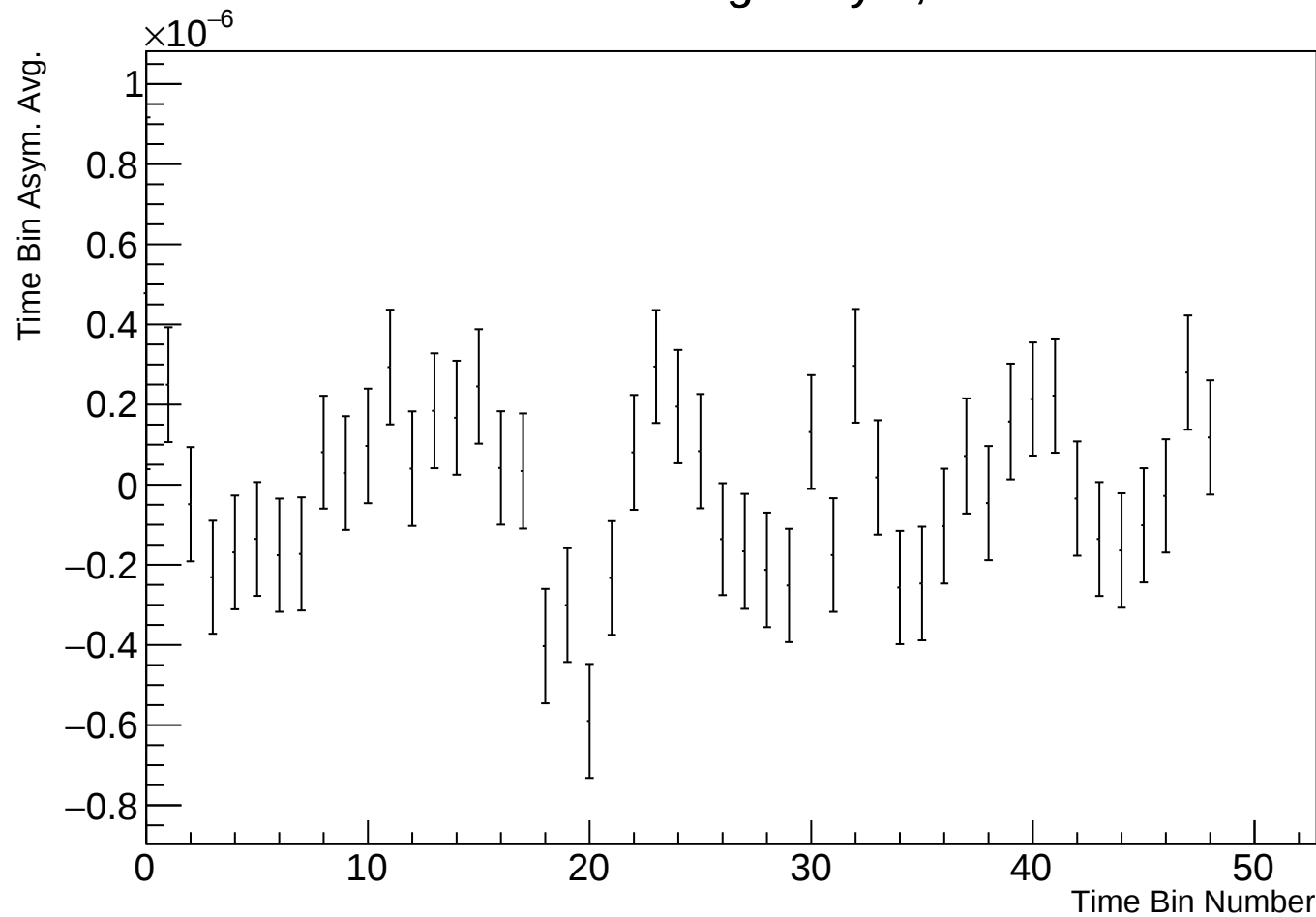
Time Bin Run Average Asym, r38314 w2
