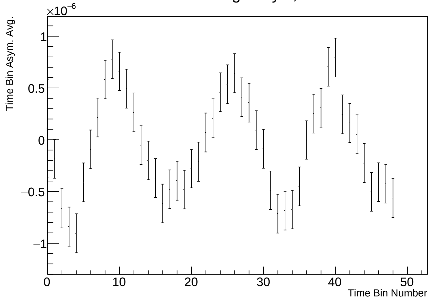
Time Bin Run Average Asym, r38314 w52
