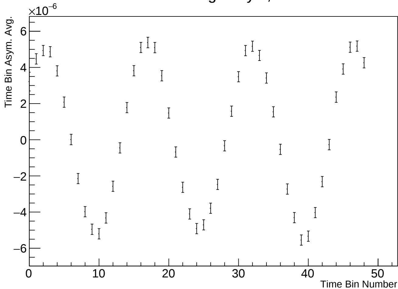
Time Bin Run Average Asym, r38314 w39
