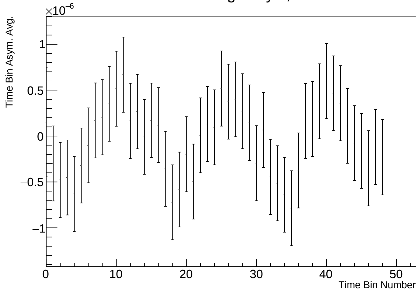
Time Bin Run Average Asym, r38314 w11
