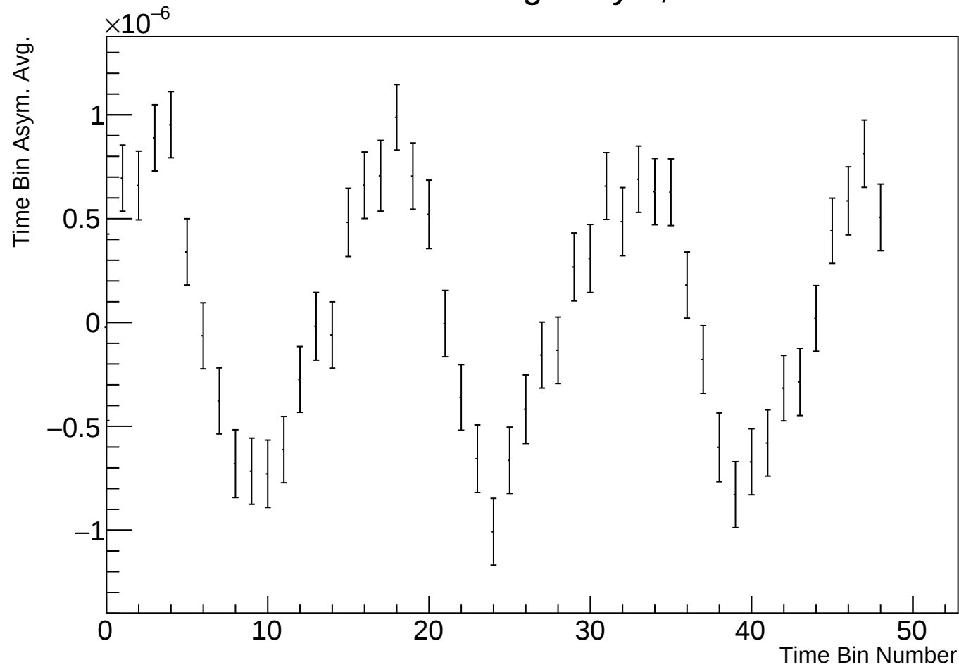
Time Bin Run Average Asym, r38314 w21
