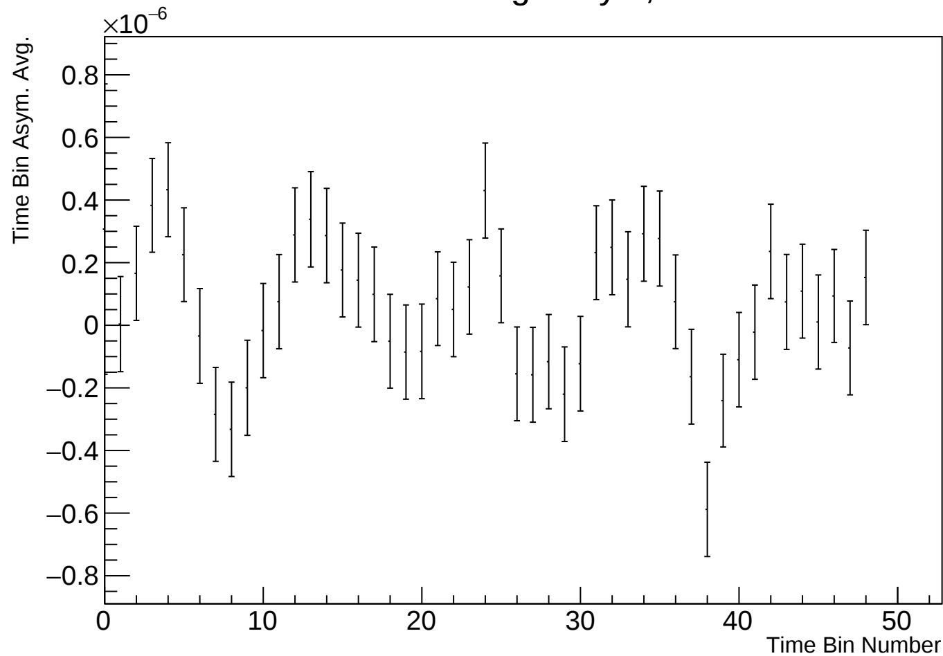
Time Bin Run Average Asym, r38314 w64
