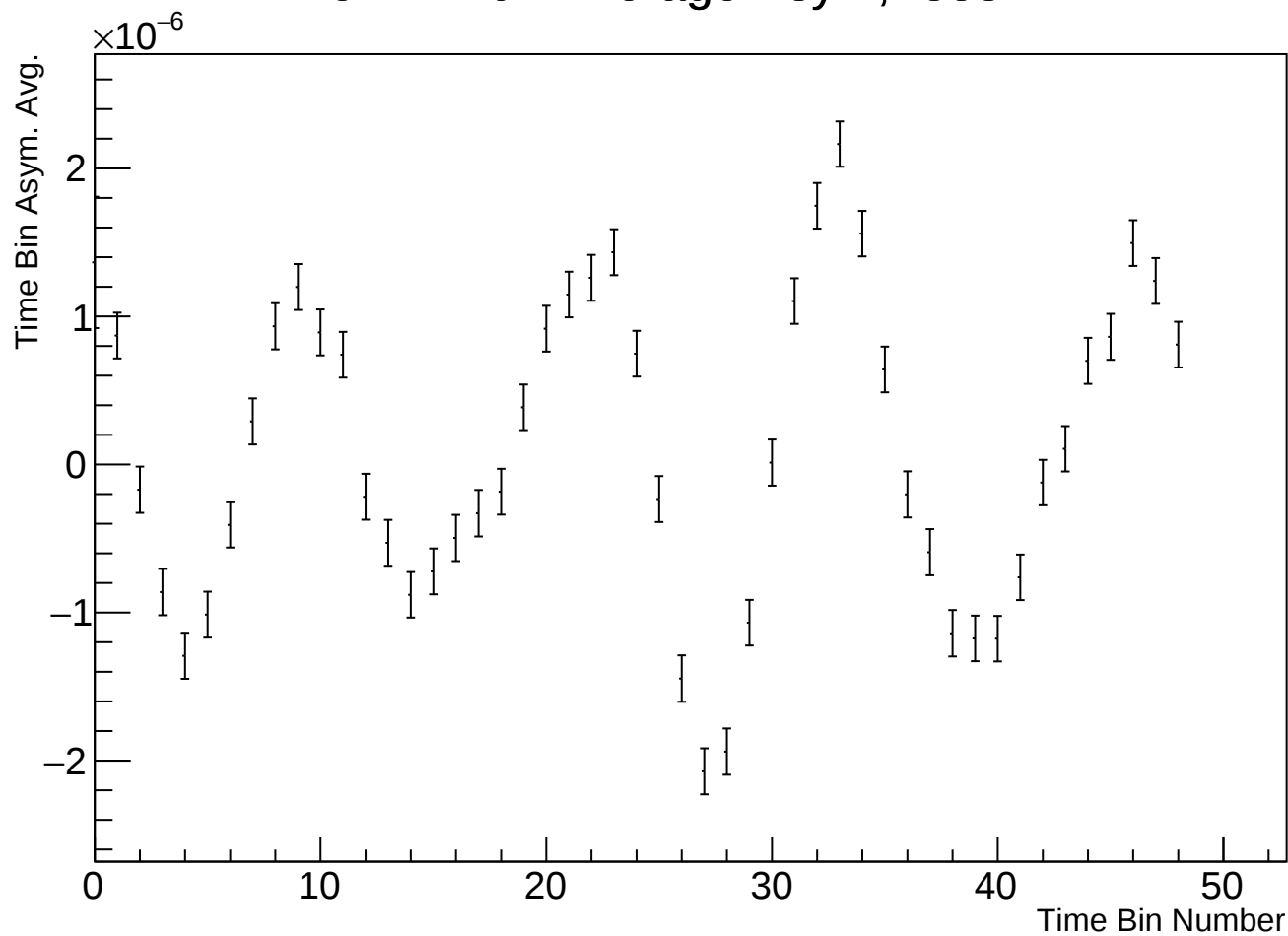
Time Bin Run Average Asym, r38314 w7
