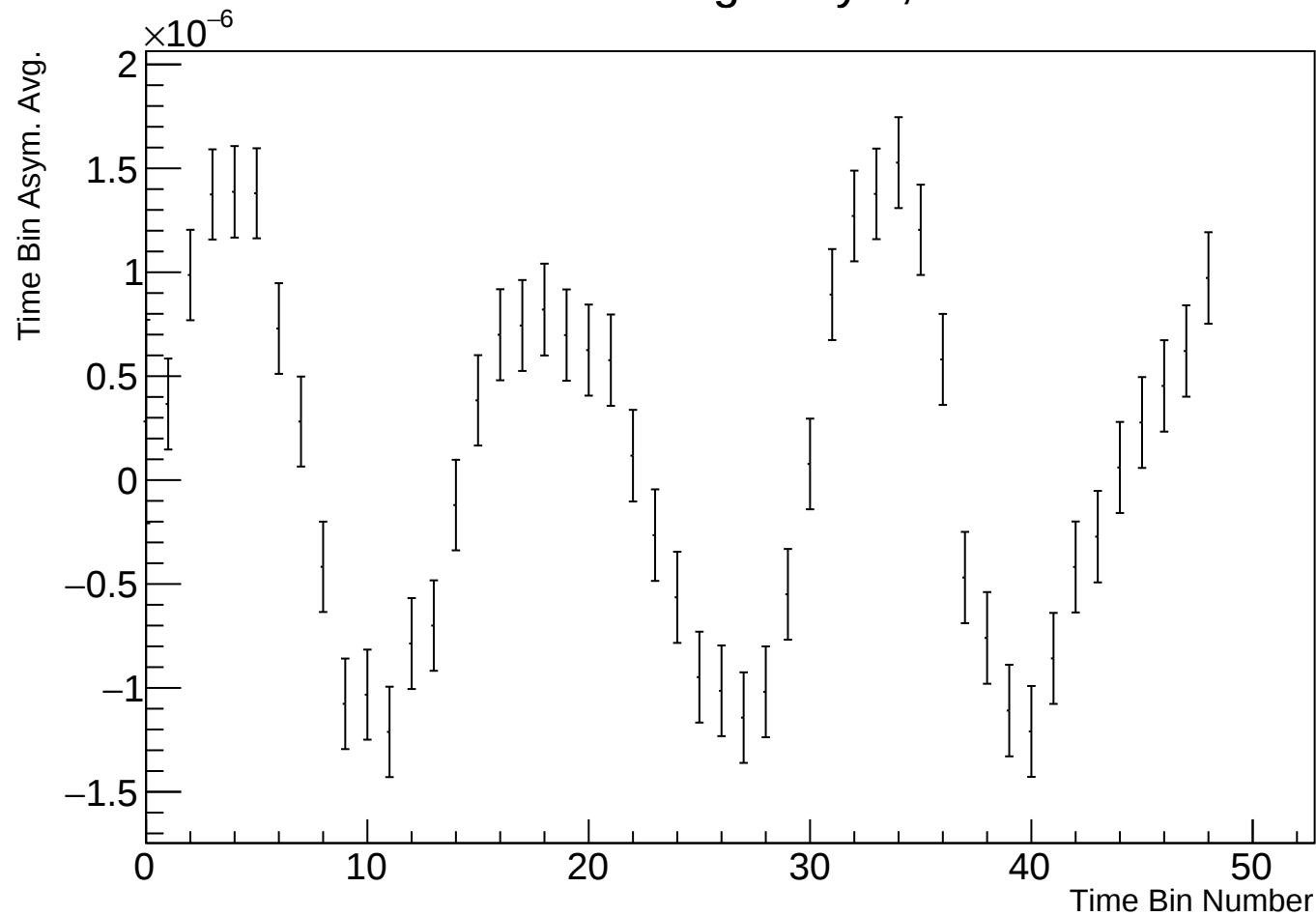
Time Bin Run Average Asym, r38314 w66
