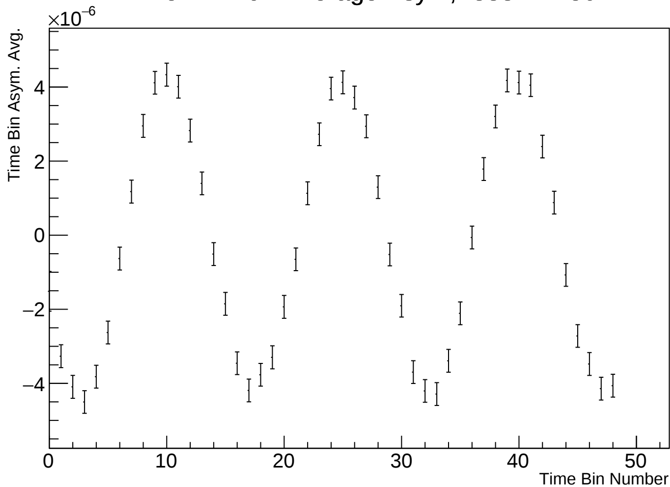
Time Bin Run Average Asym, r38314 w50
