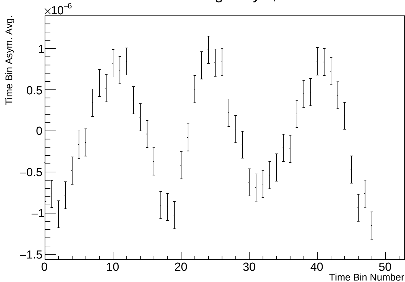
Time Bin Run Average Asym, r38314 w133
