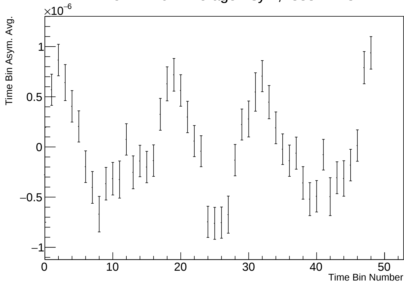
Time Bin Run Average Asym, r38314 w31
