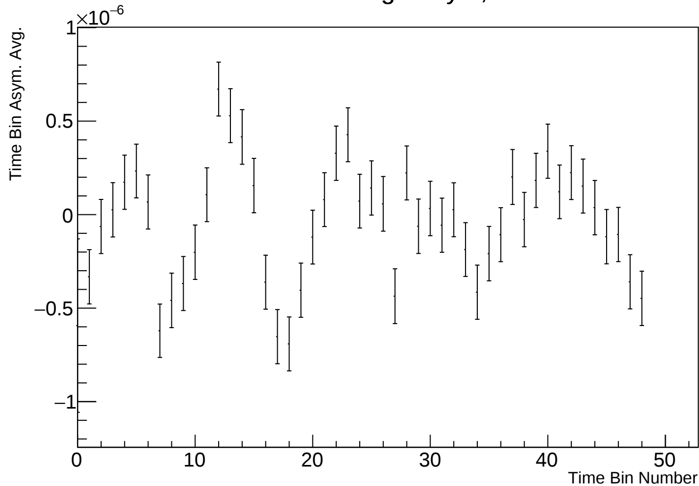
Time Bin Run Average Asym, r38314 w91
