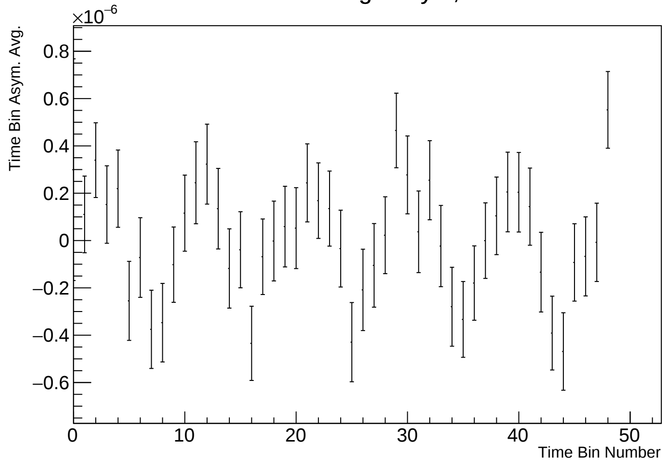
Time Bin Run Average Asym, r38314 w32
