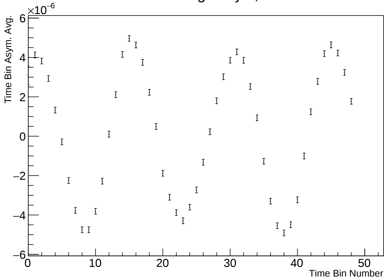
Time Bin Run Average Asym, r38314 w141
