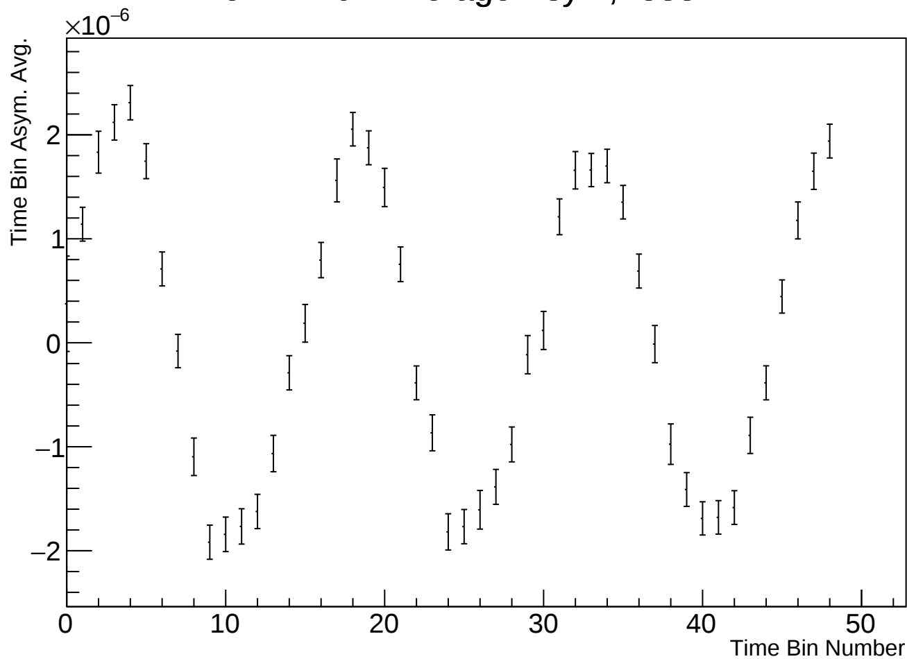
Time Bin Run Average Asym, r38314 w22
