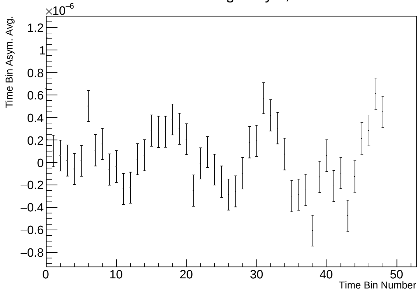
Time Bin Run Average Asym, r38314 w14
