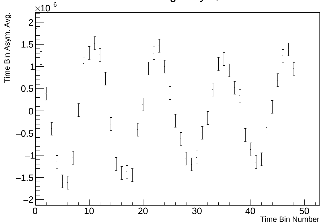
Time Bin Run Average Asym, r38314 w136
