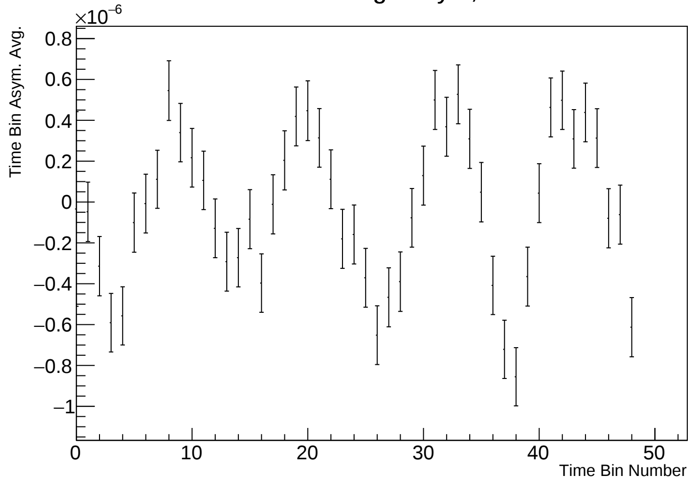
Time Bin Run Average Asym, r38314 w99
