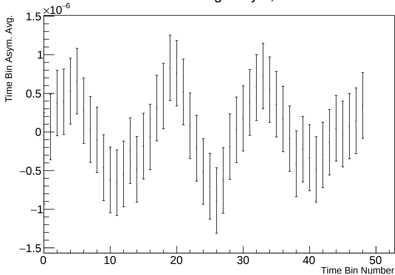
Time Bin Run Average Asym, r38314 w19
