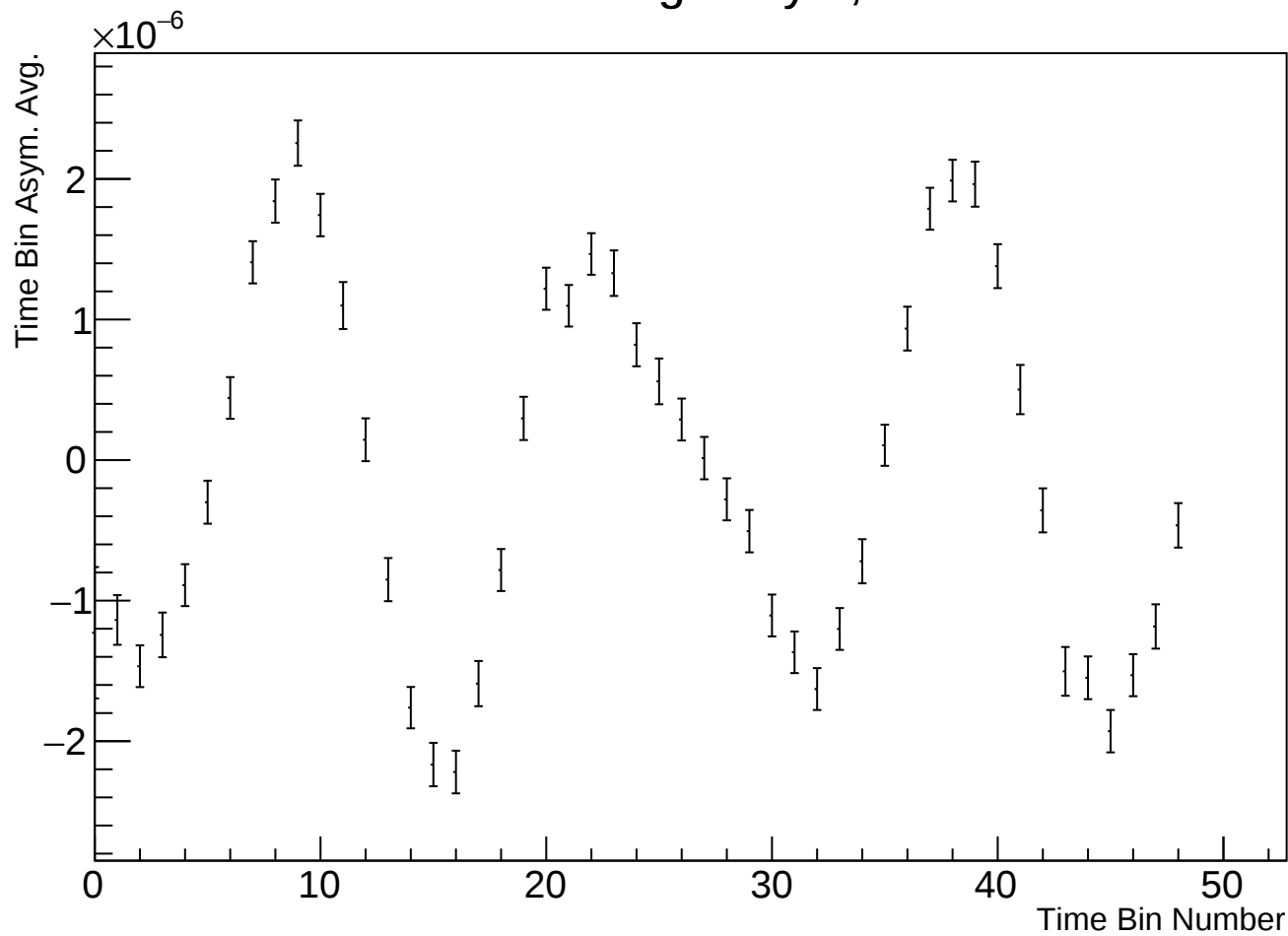
Time Bin Run Average Asym, r38314 w142
