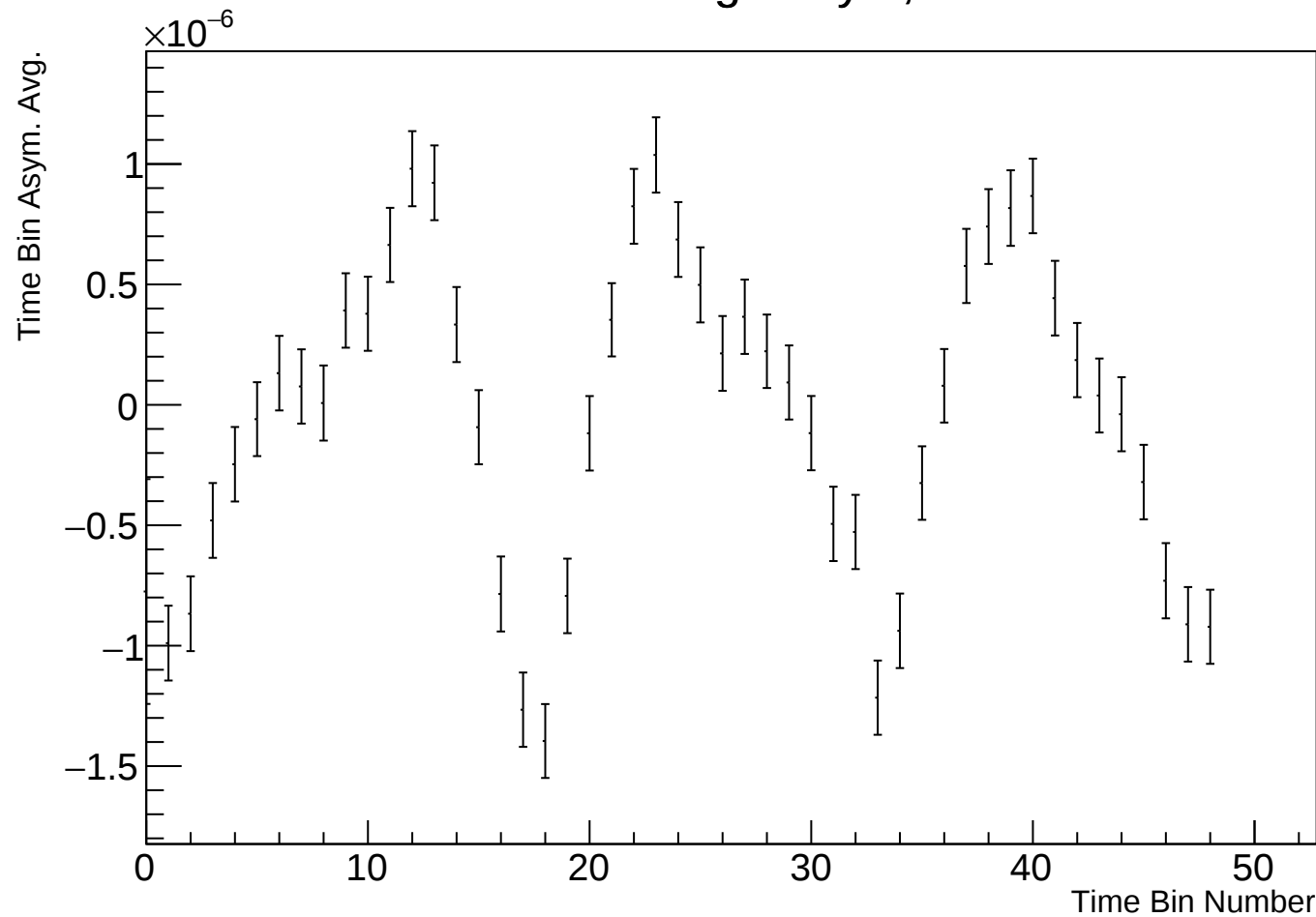
Time Bin Run Average Asym, r38314 w95
