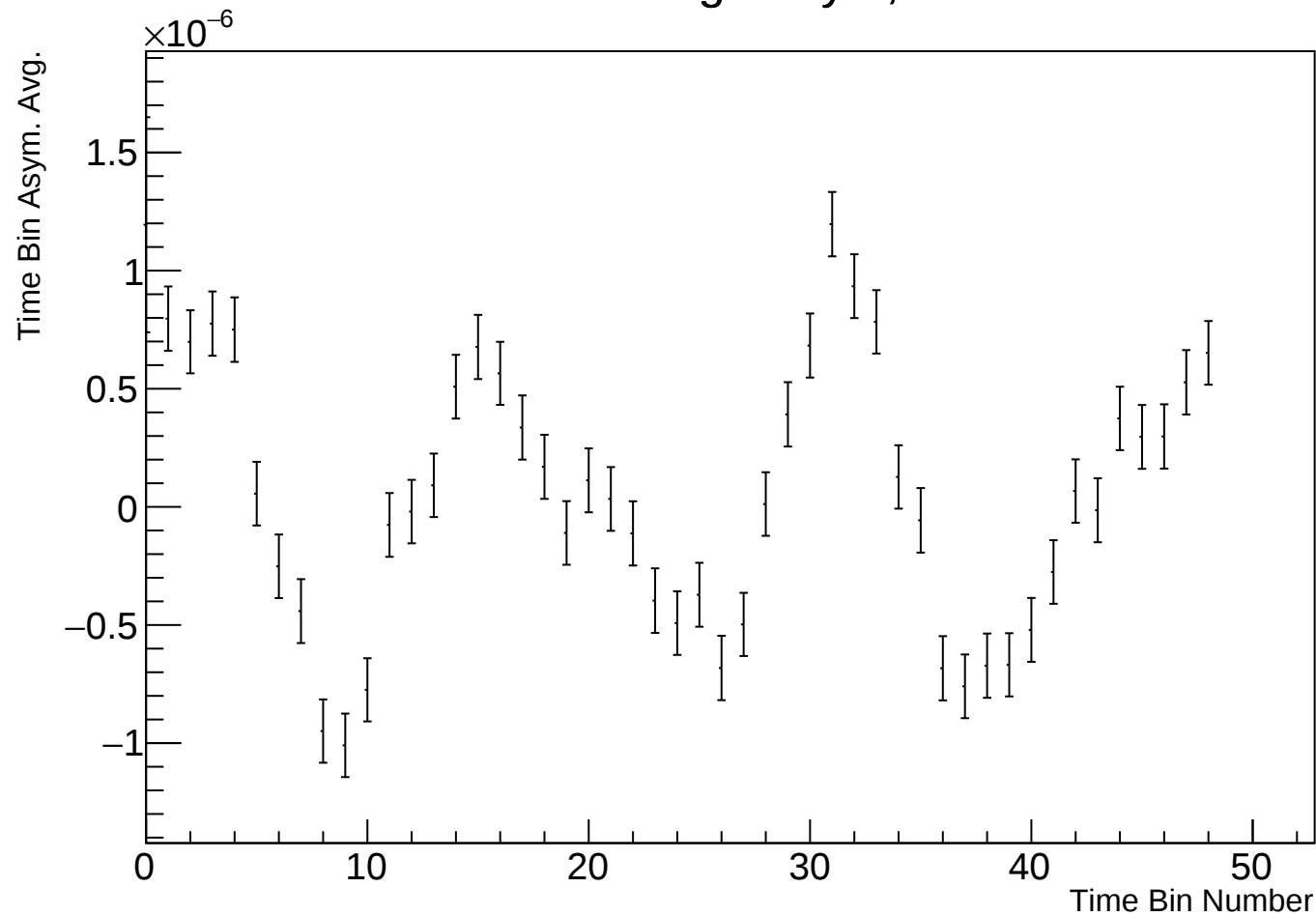
Time Bin Run Average Asym, r38314 w113
