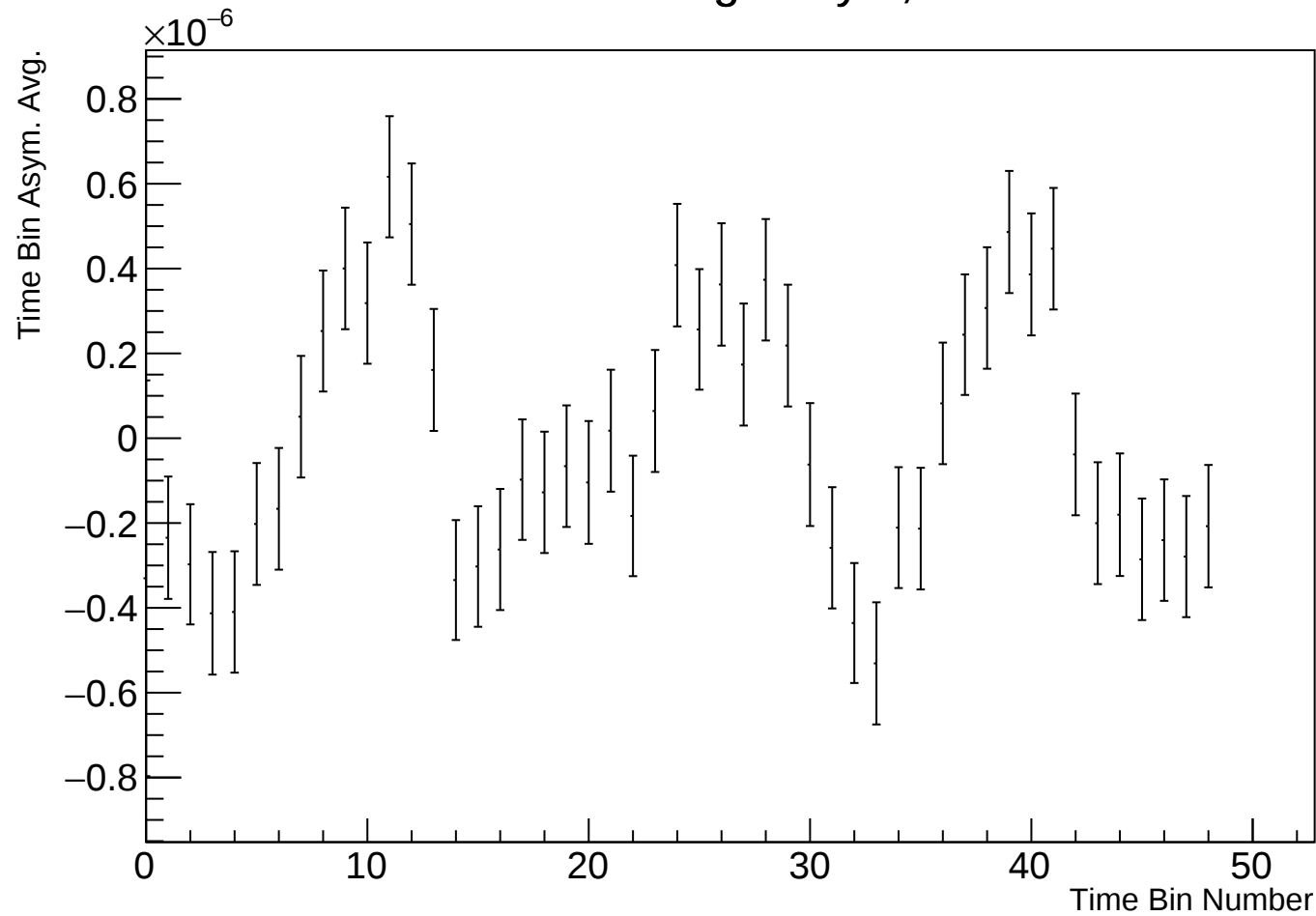
Time Bin Run Average Asym, r38314 w86
