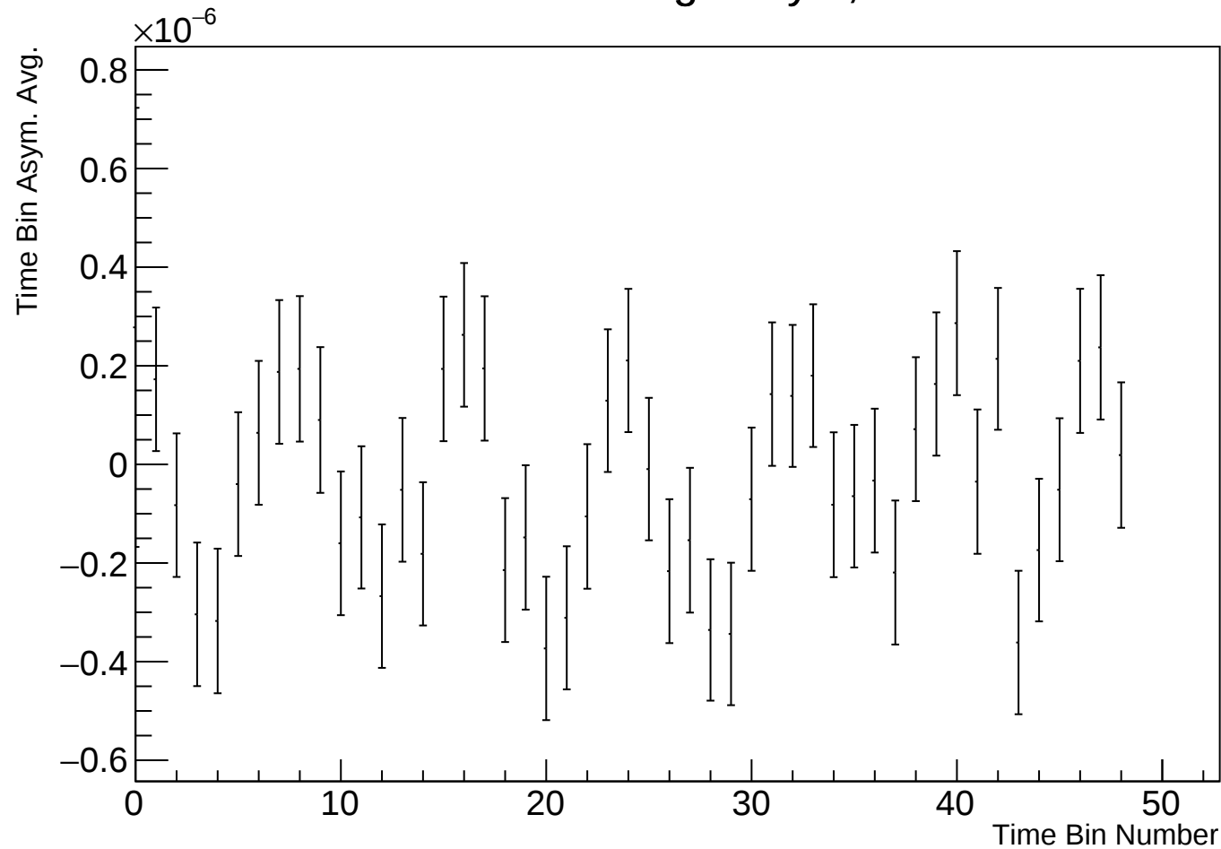
Time Bin Run Average Asym, r38314 w4
