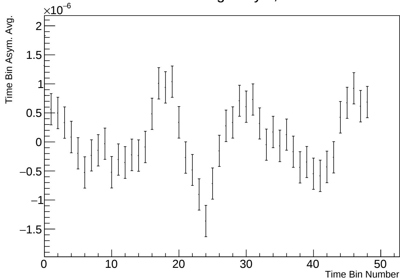
Time Bin Run Average Asym, r38314 w76
