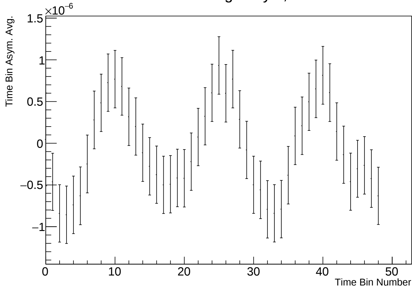
Time Bin Run Average Asym, r38314 w51
