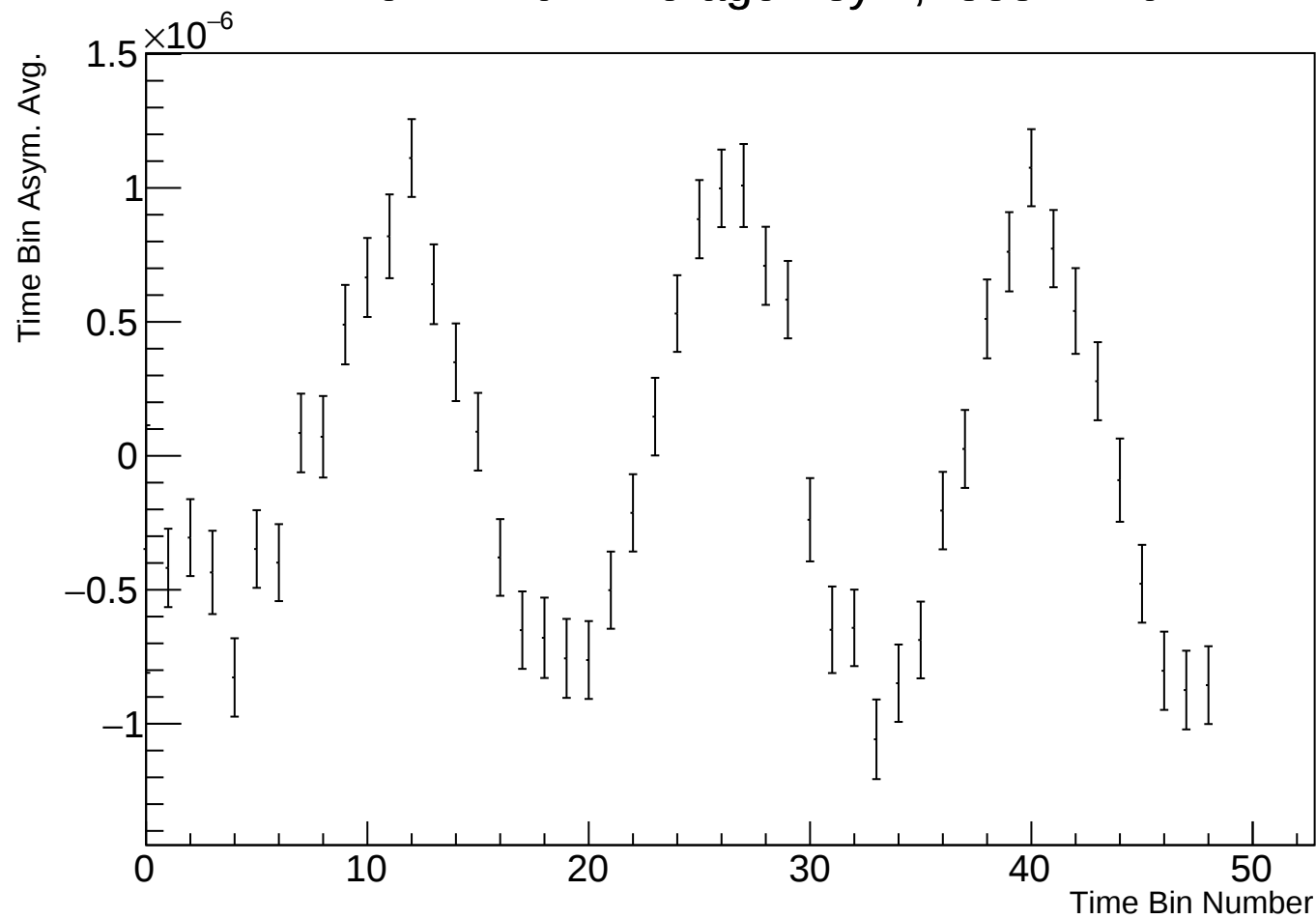
Time Bin Run Average Asym, r38314 w9
