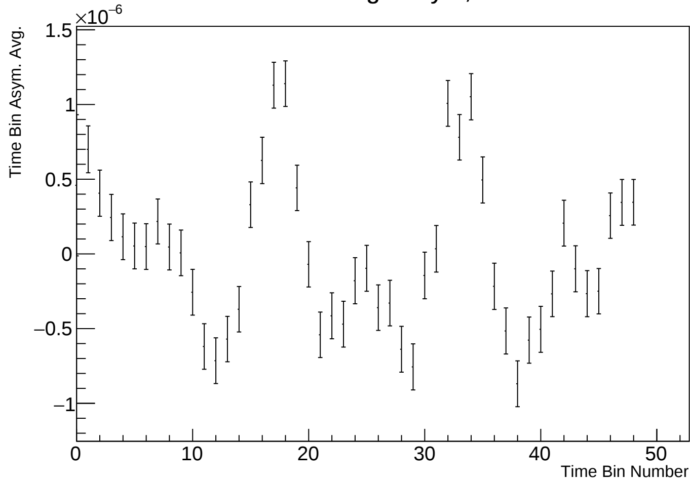
Time Bin Run Average Asym, r38314 w102
