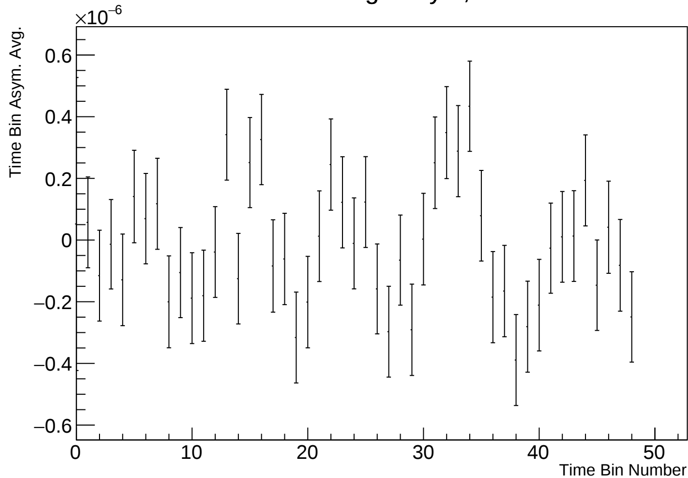
Time Bin Run Average Asym, r38314 w129
