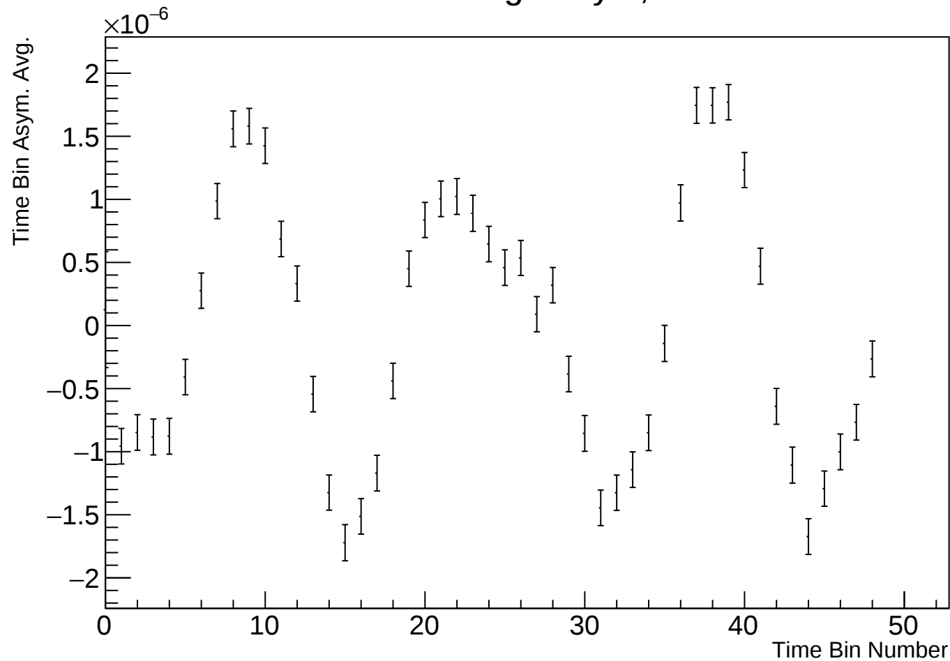
Time Bin Run Average Asym, r38314 w140
