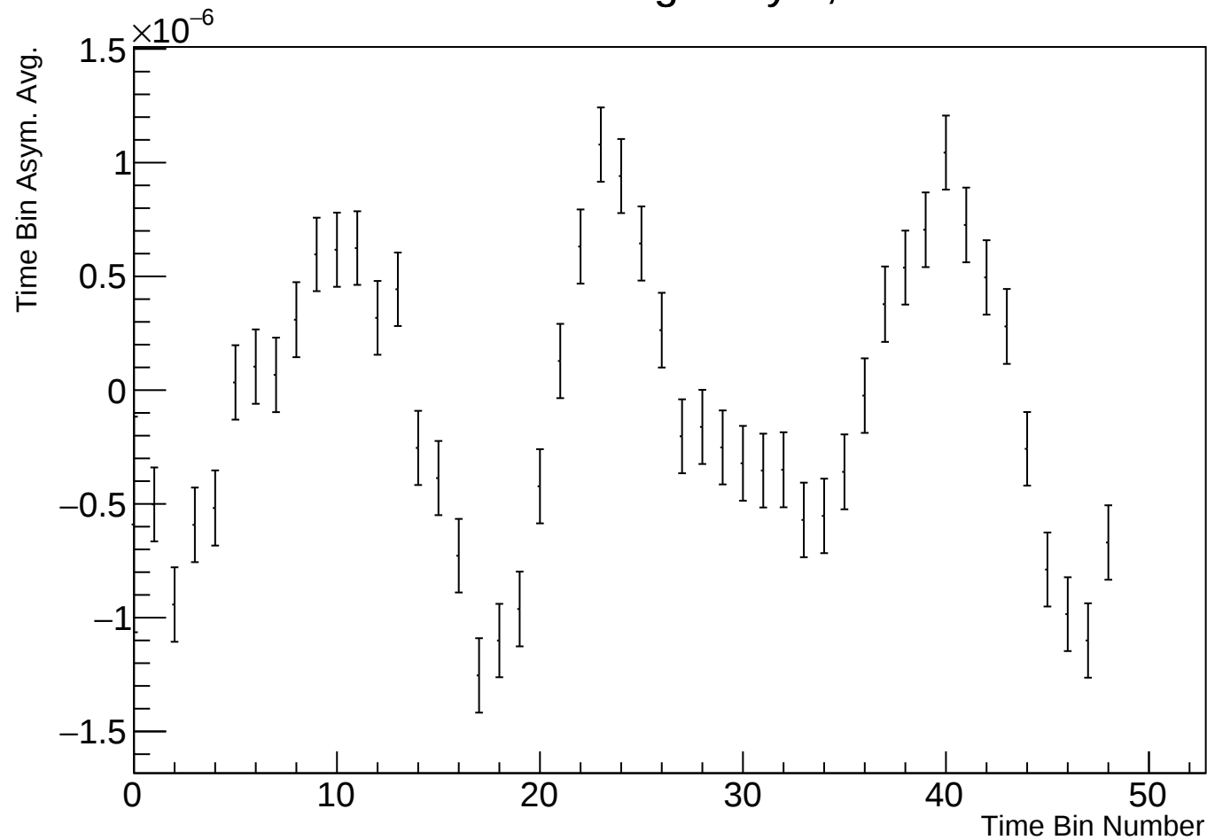
Time Bin Run Average Asym, r38314 w93
