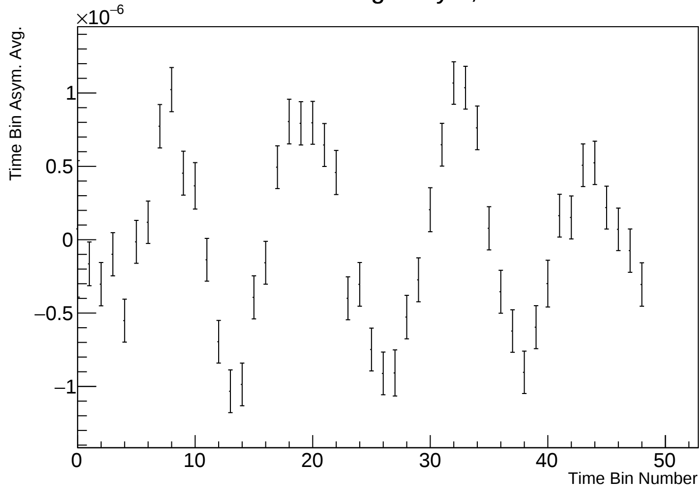
Time Bin Run Average Asym, r38314 w107
