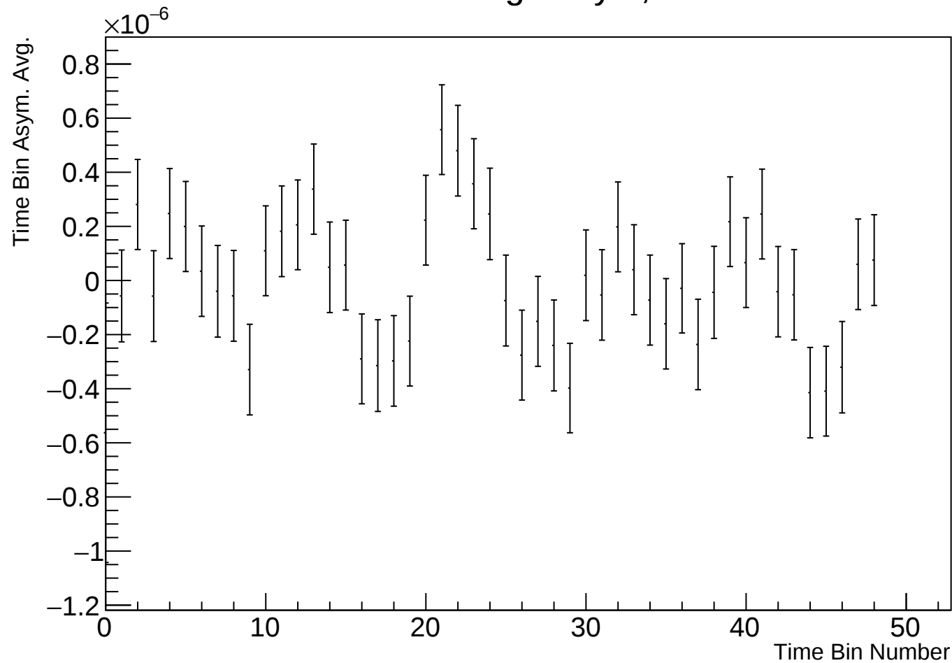
Time Bin Run Average Asym, r38314 w110
