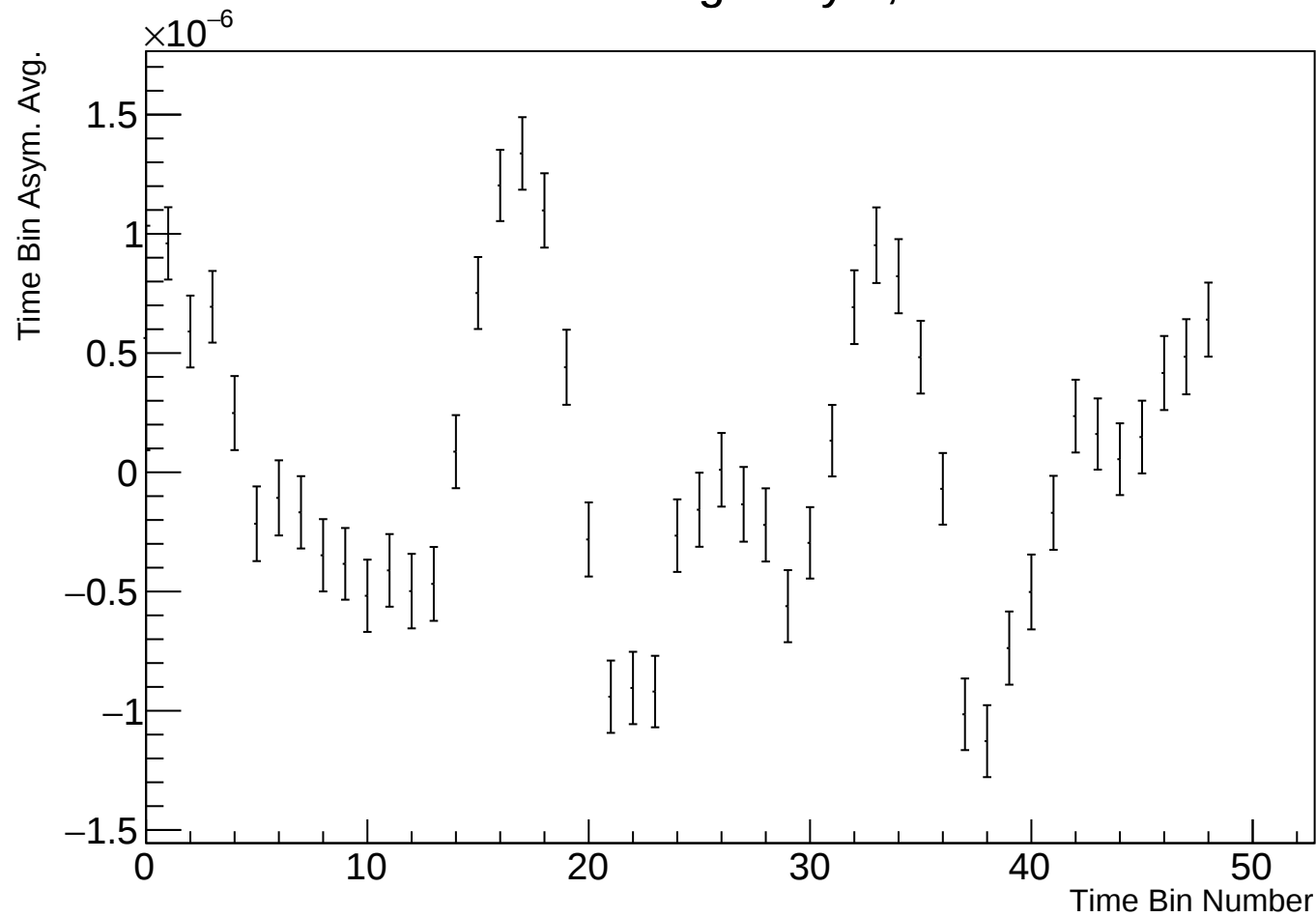
Time Bin Run Average Asym, r38314 w105
