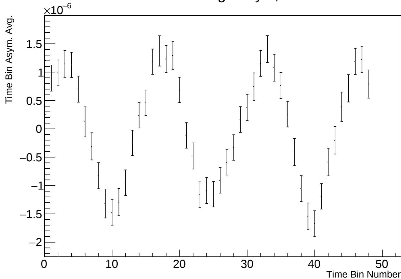
Time Bin Run Average Asym, r38314 w40
