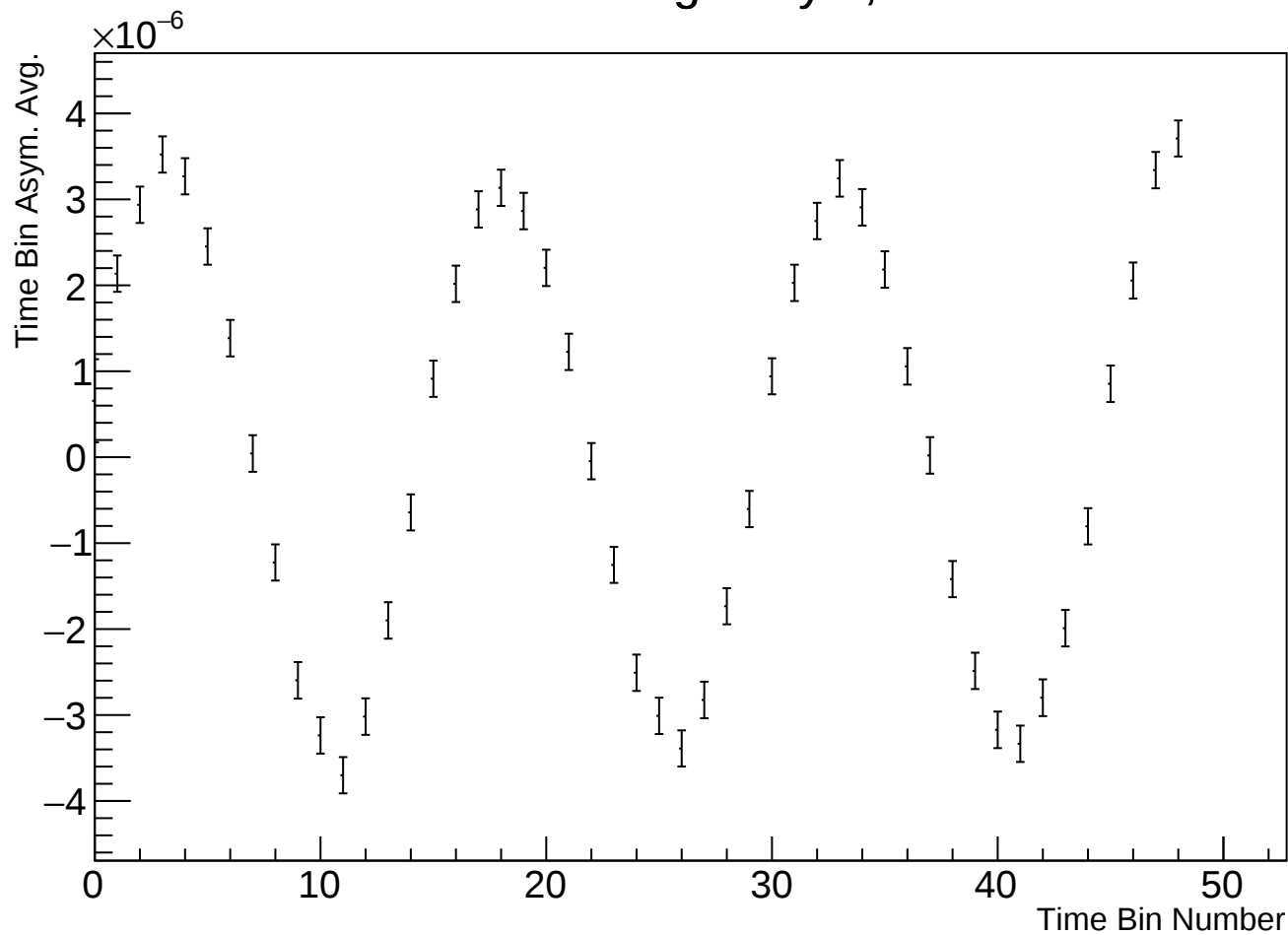
Time Bin Run Average Asym, r38314 w10
