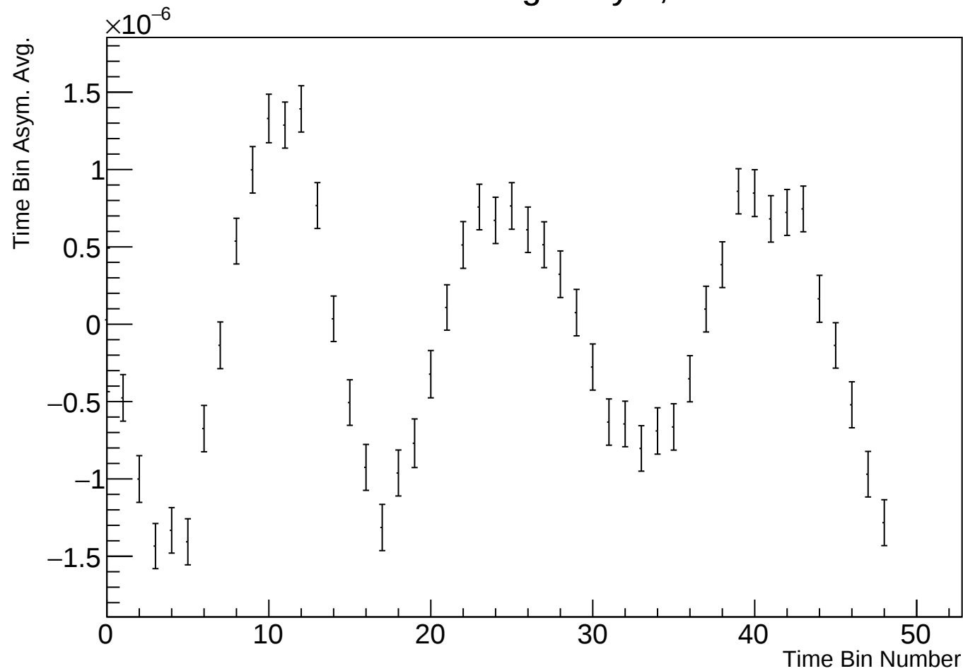
Time Bin Run Average Asym, r38314 w27
