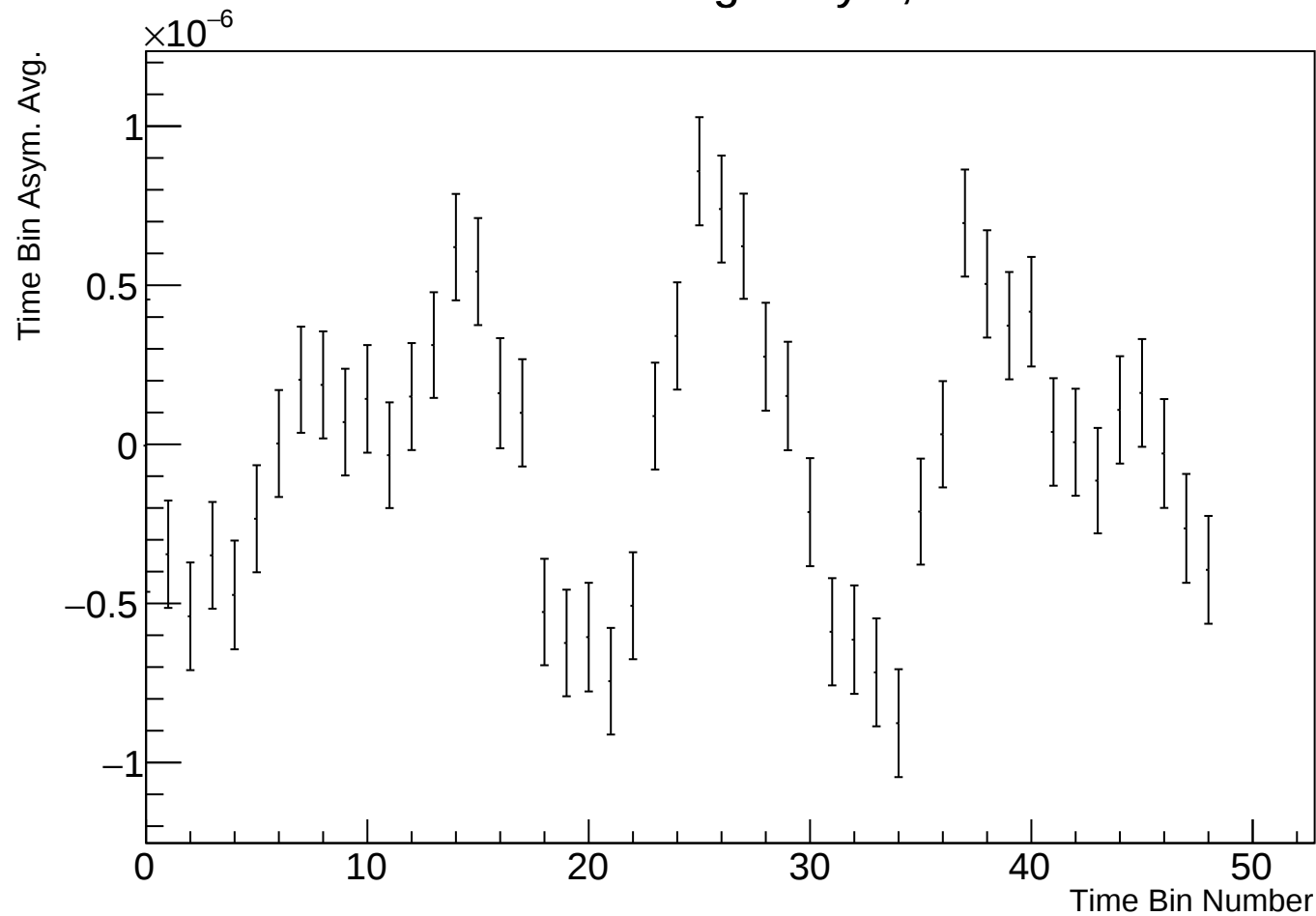
Time Bin Run Average Asym, r38314 w44
