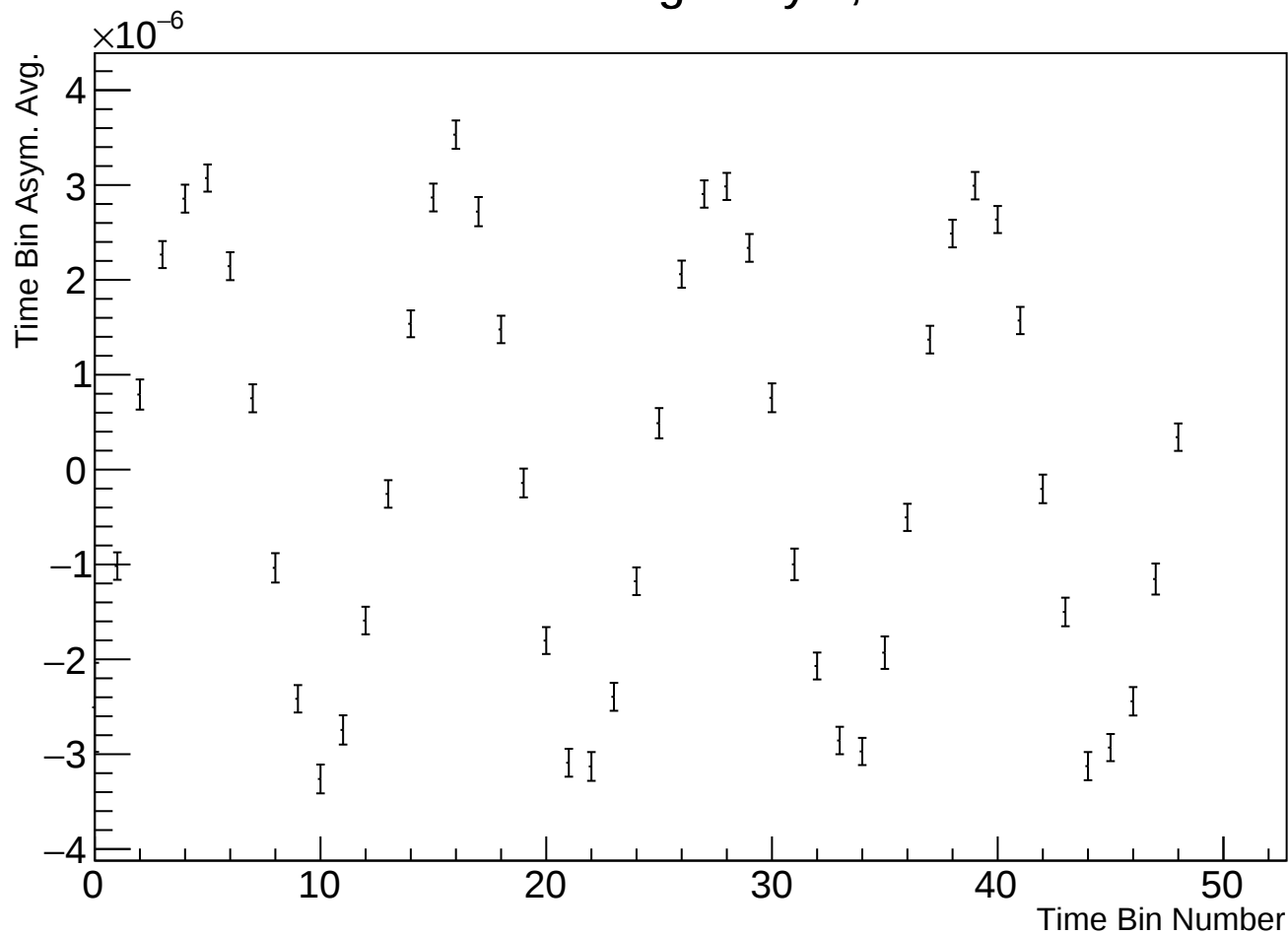
Time Bin Run Average Asym, r38314 w126
