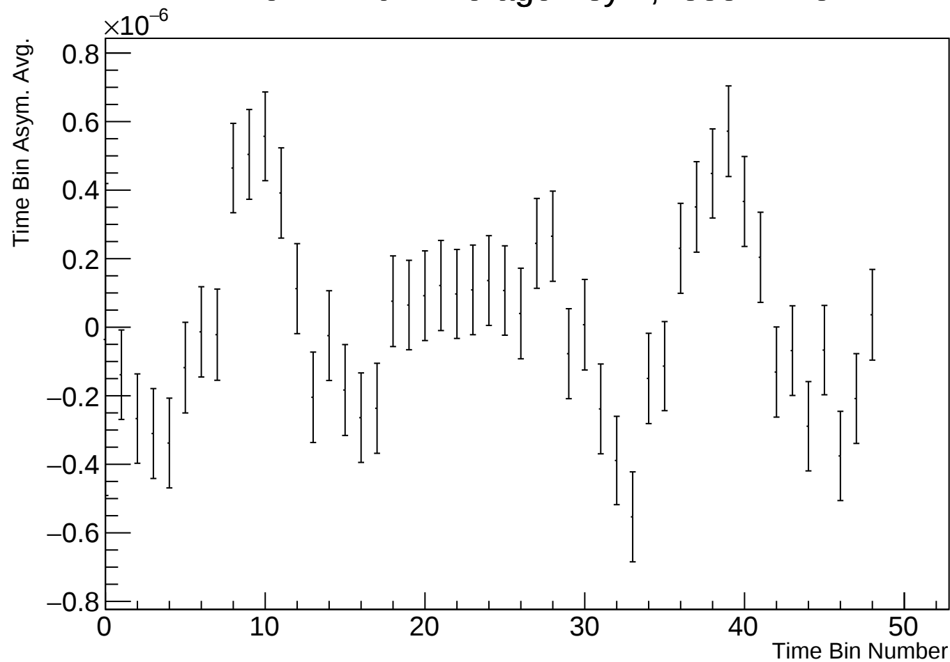
Time Bin Run Average Asym, r38314 w87
