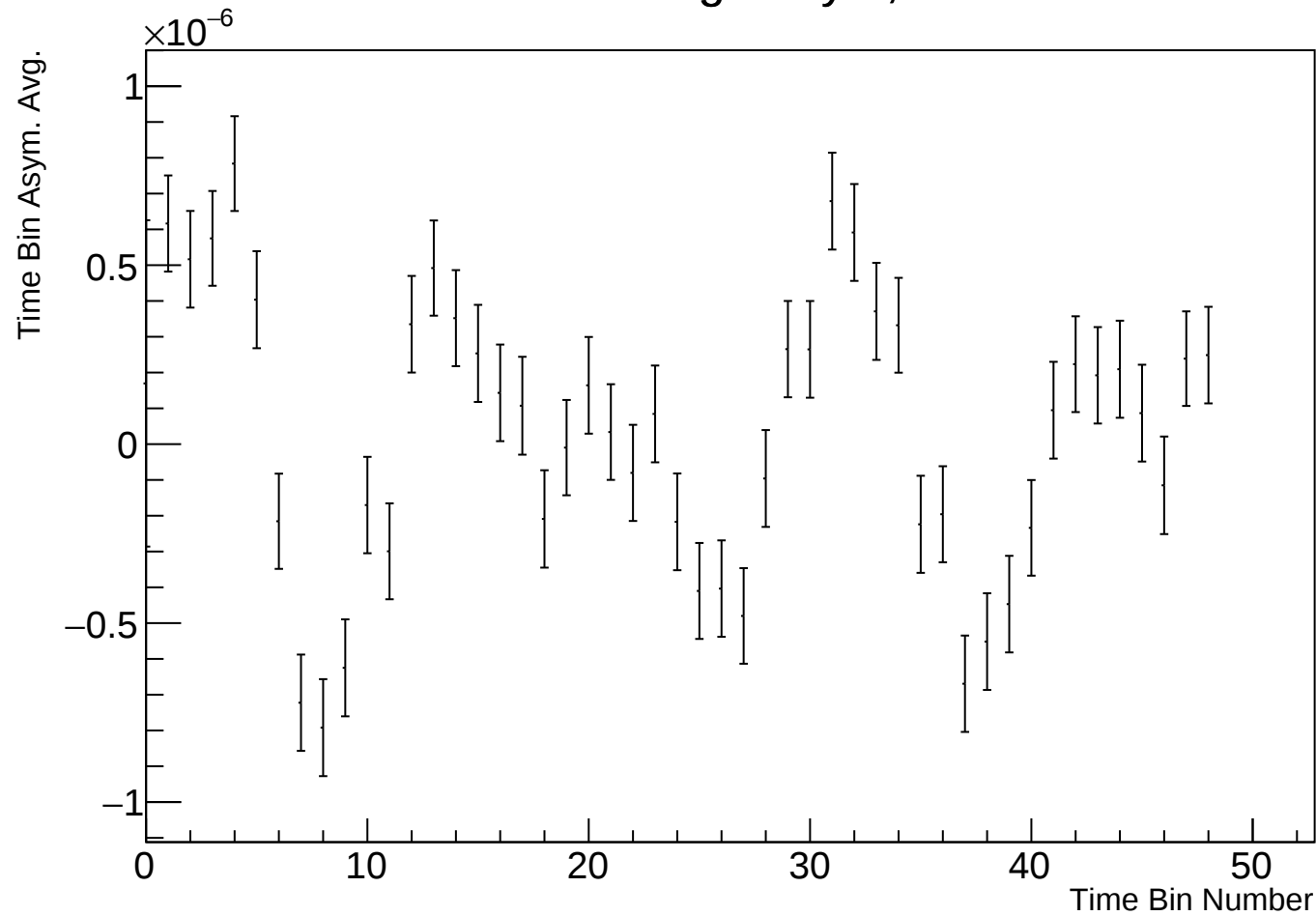
Time Bin Run Average Asym, r38314 w112
