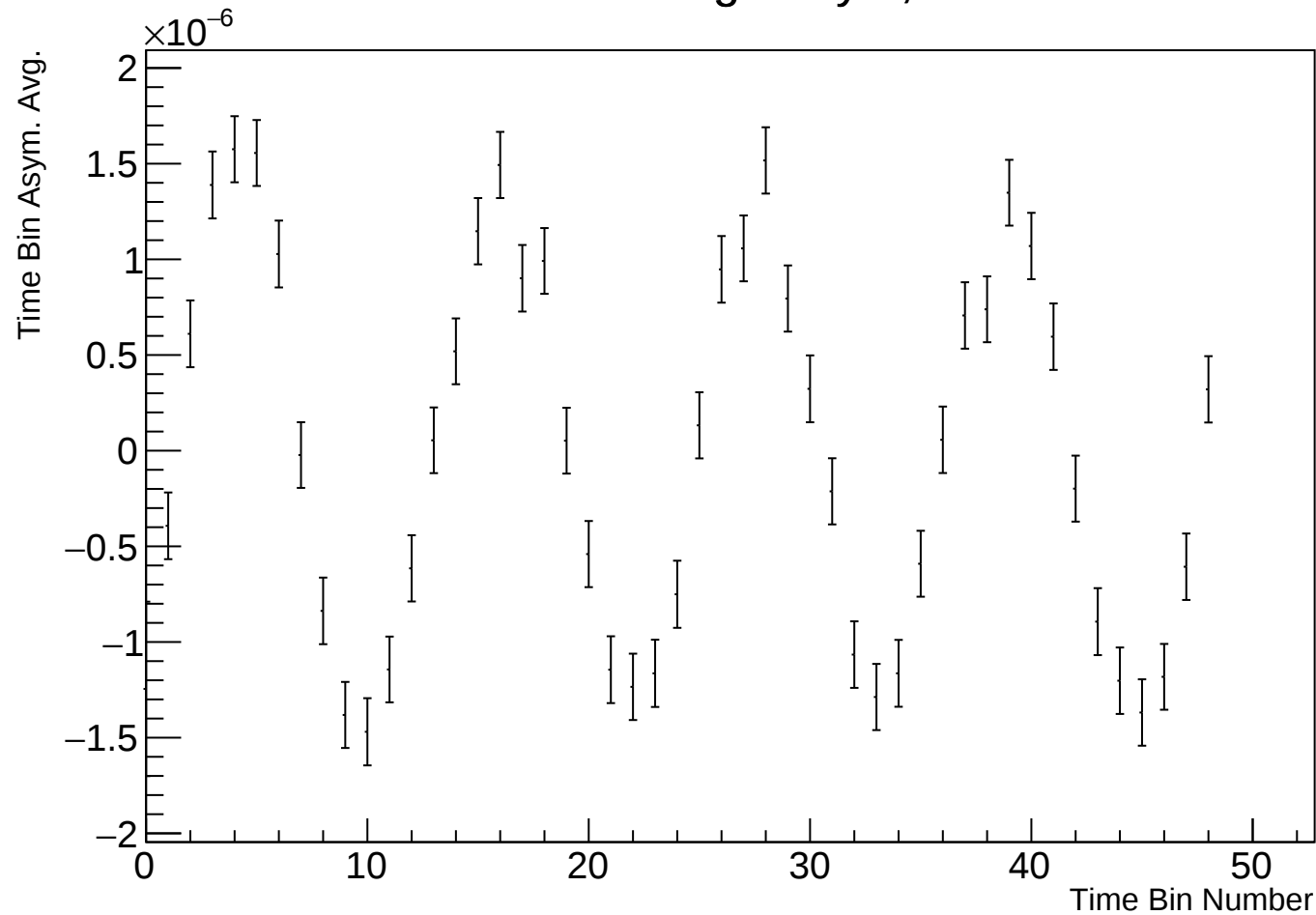
Time Bin Run Average Asym, r38314 w25
