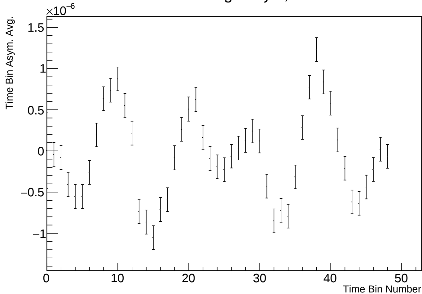
Time Bin Run Average Asym, r38314 w139
