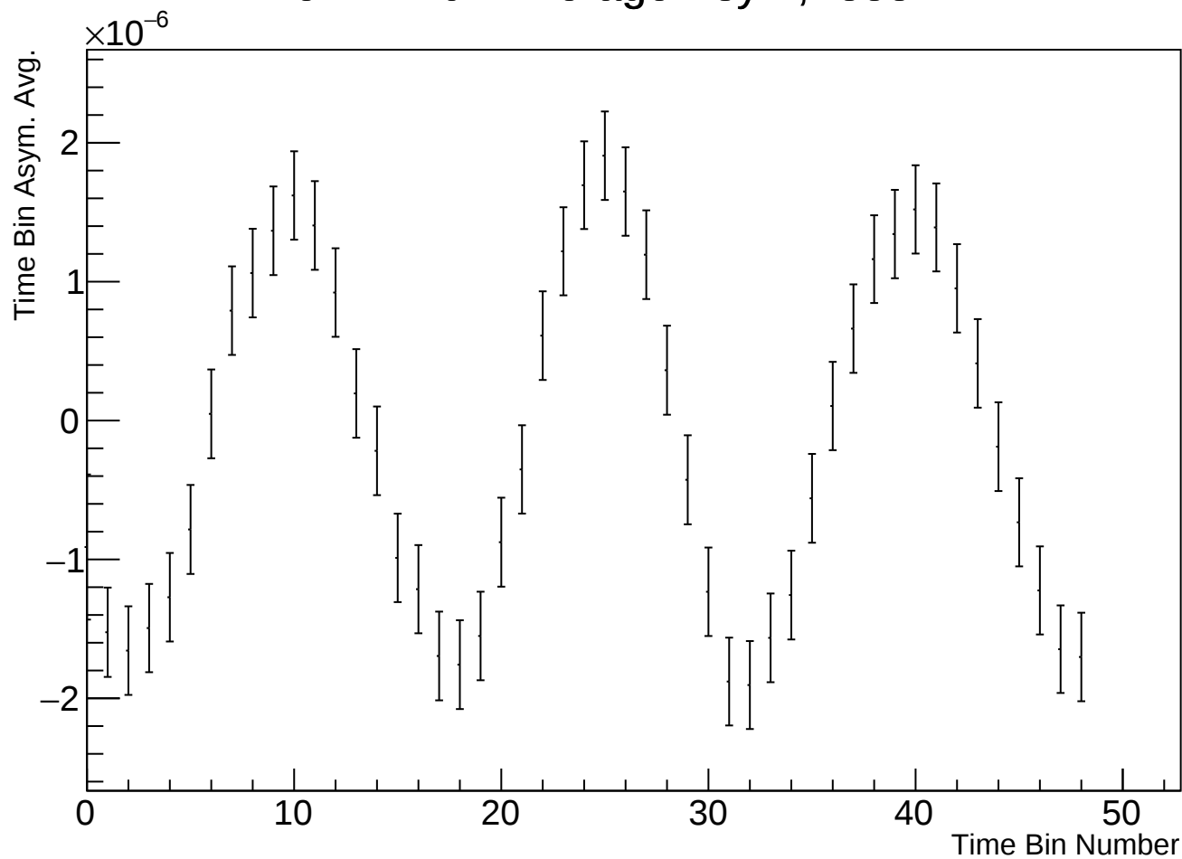
Time Bin Run Average Asym, r38314 w41
