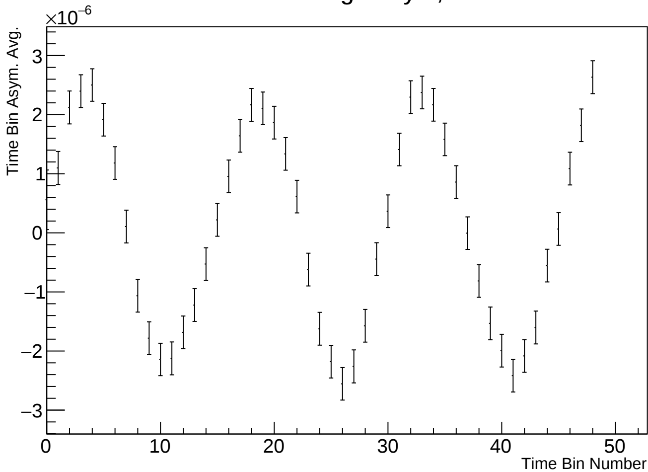
Time Bin Run Average Asym, r38314 w61
