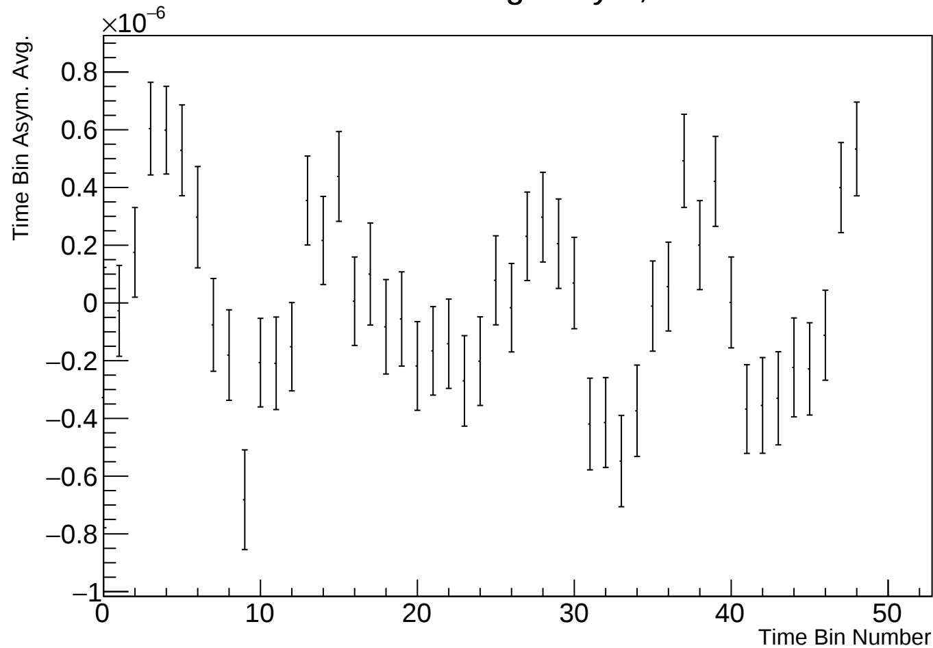
Time Bin Run Average Asym, r38314 w26
