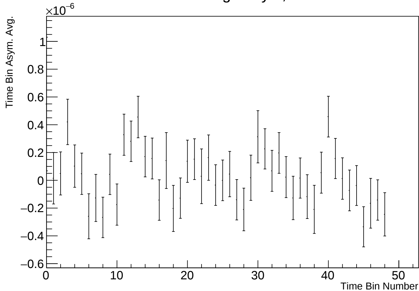
Time Bin Run Average Asym, r38314 w109
