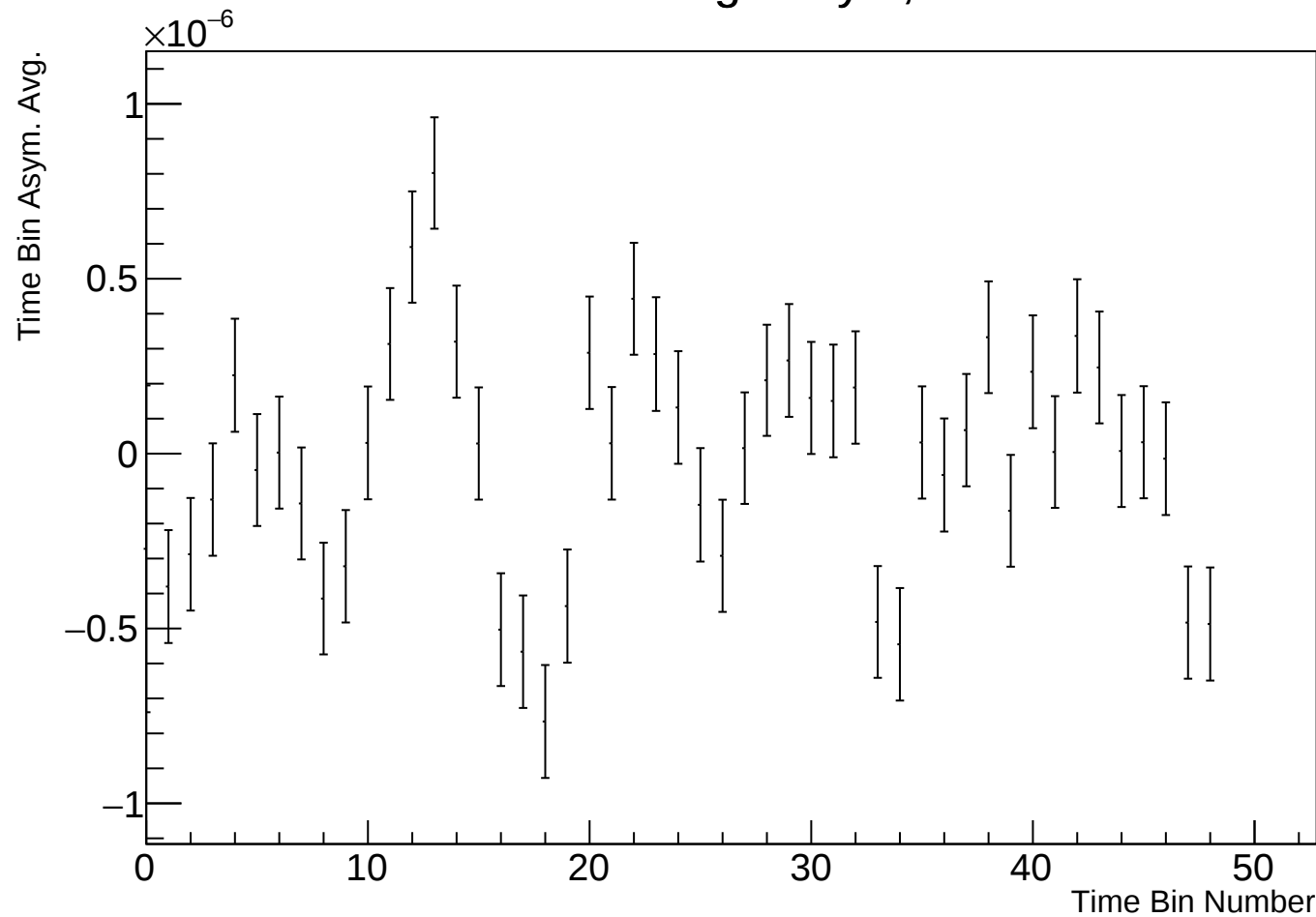
Time Bin Run Average Asym, r38314 w92
