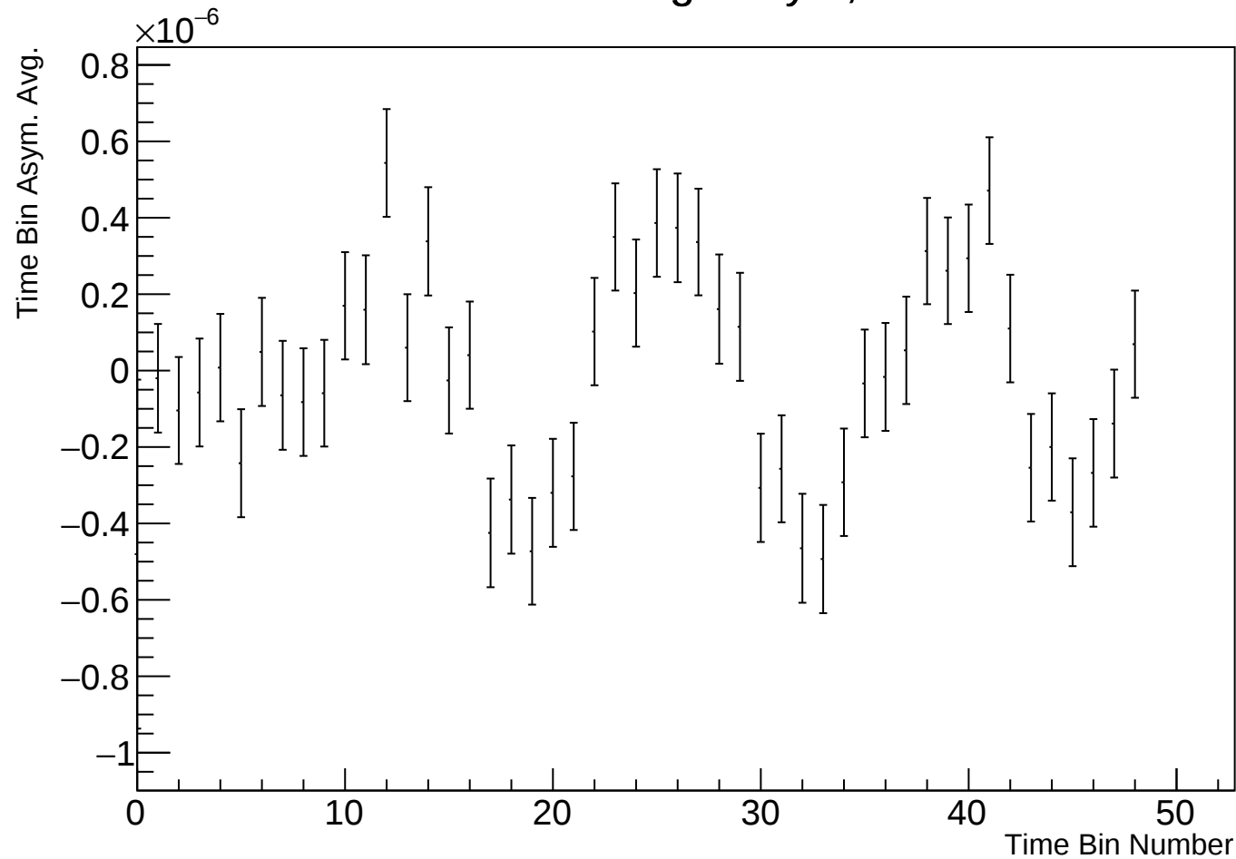
Time Bin Run Average Asym, r38314 w98
