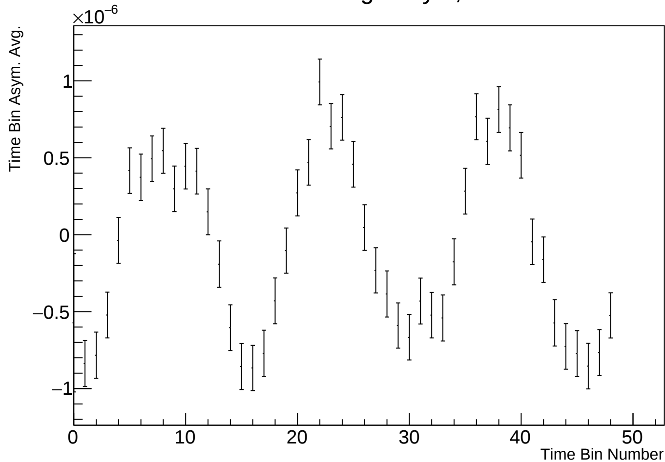
Time Bin Run Average Asym, r38314 w54
