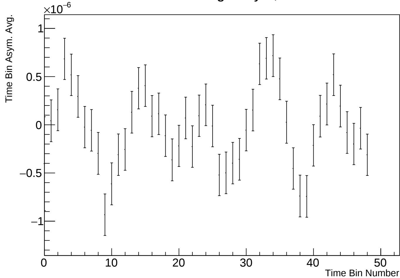
Time Bin Run Average Asym, r38314 w69
