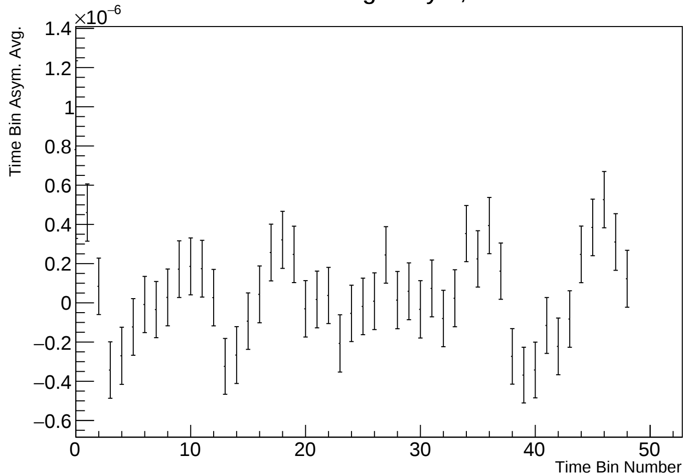
Time Bin Run Average Asym, r38314 w118
