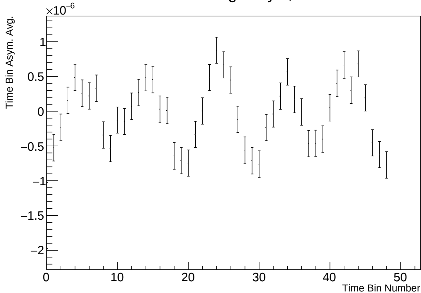
Time Bin Run Average Asym, r38314 w70
