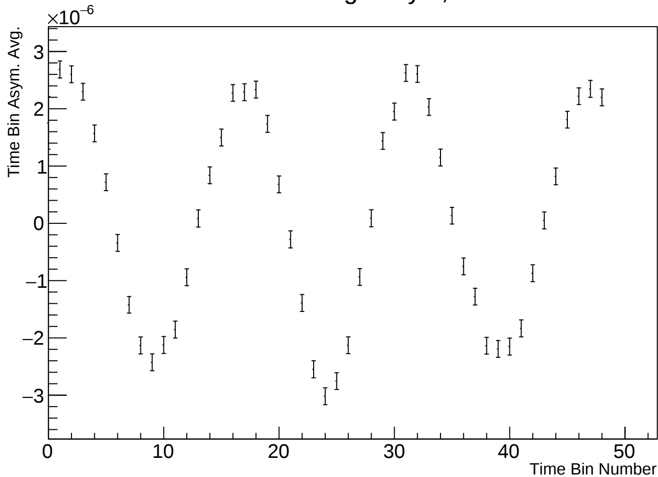
Time Bin Run Average Asym, r38314 w29
