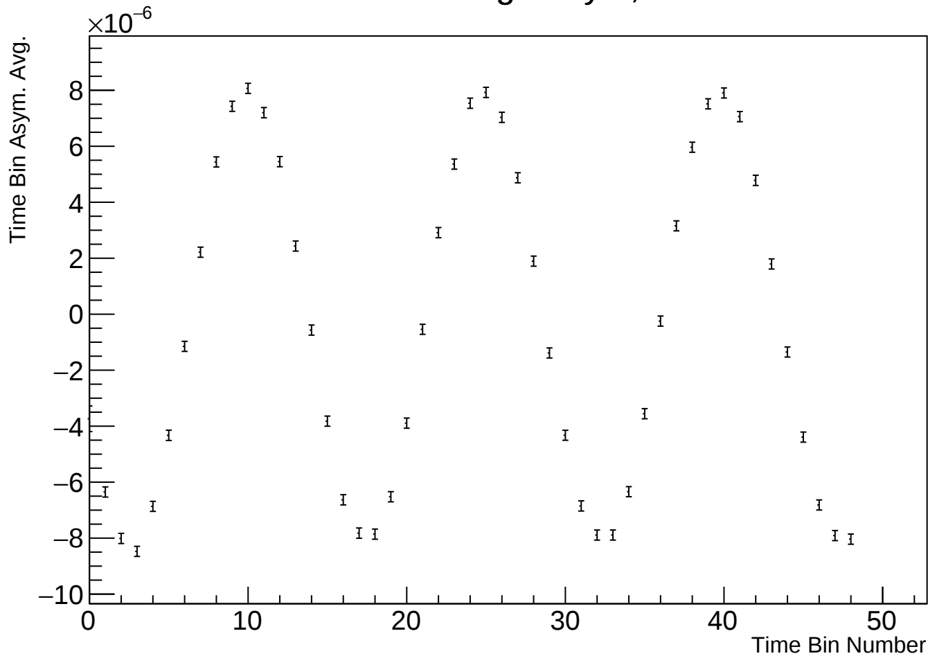
Time Bin Run Average Asym, r38314 w36
