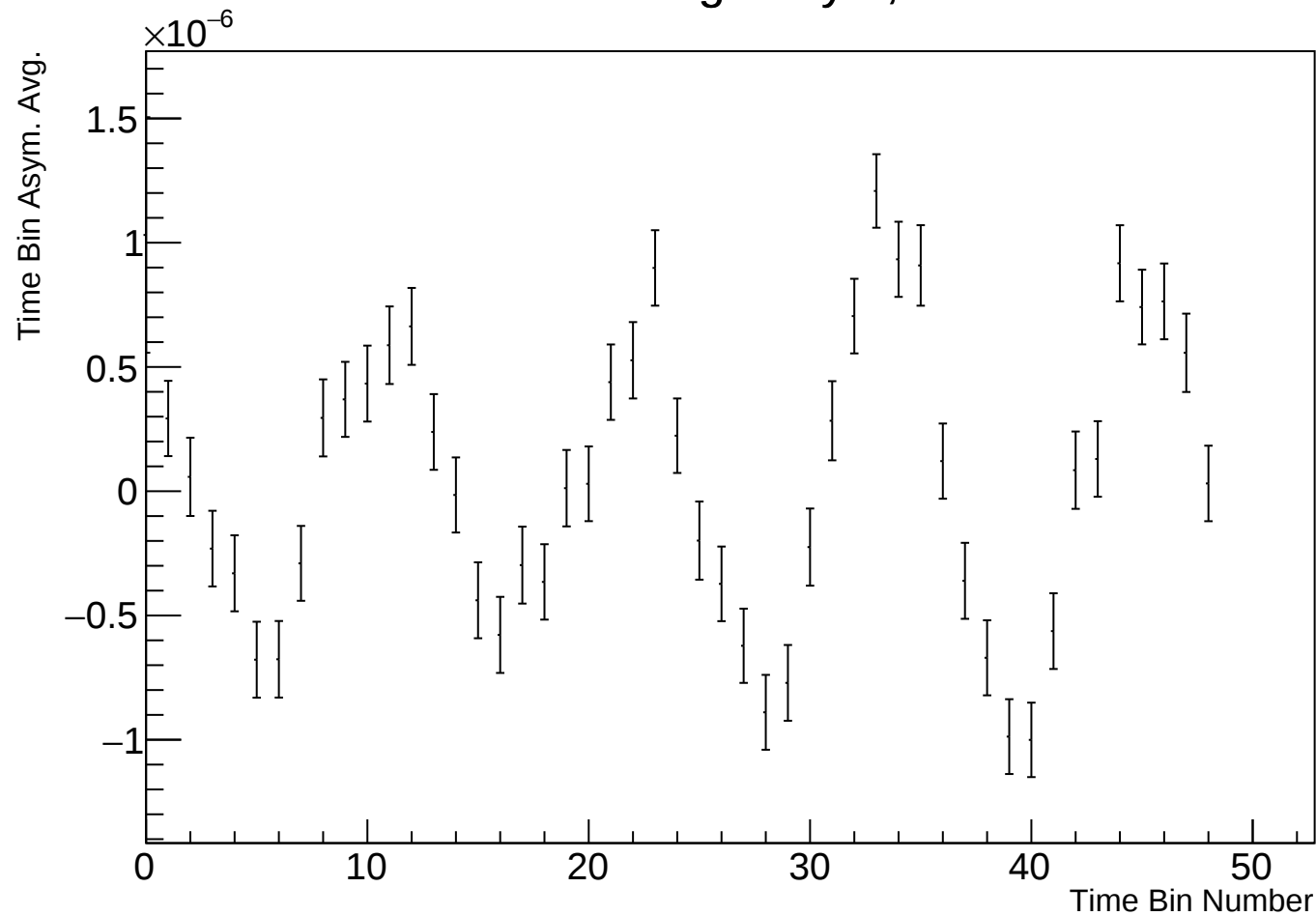
Time Bin Run Average Asym, r38314 w127
