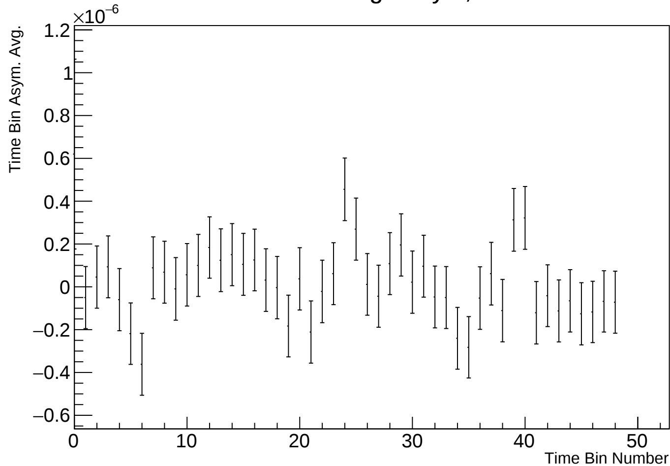
Time Bin Run Average Asym, r38314 w3
