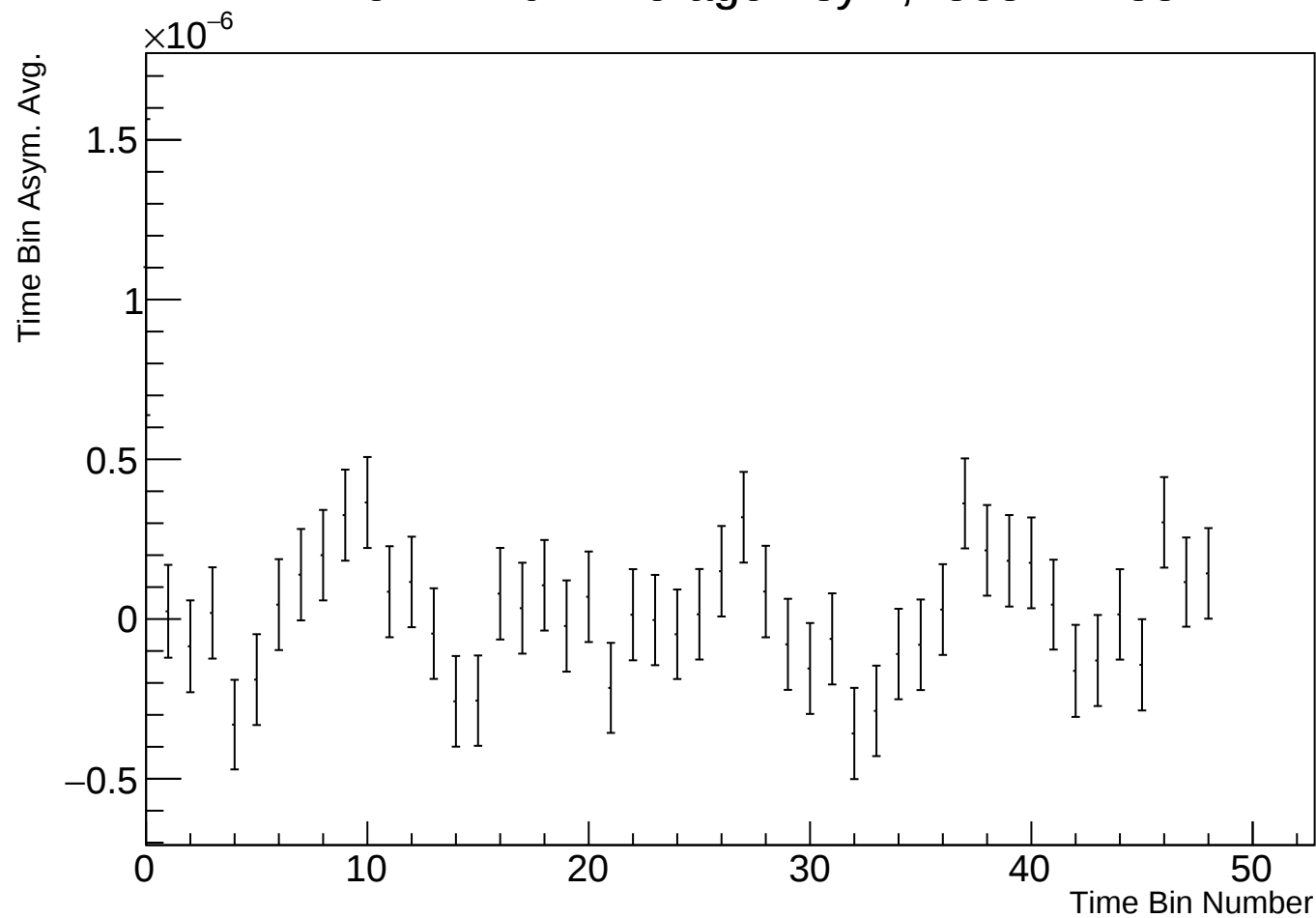
Time Bin Run Average Asym, r38314 w83
