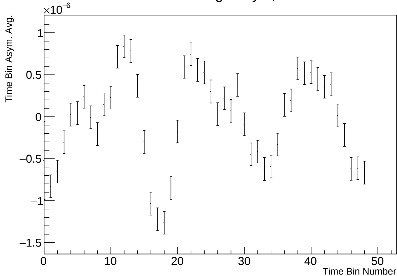
Time Bin Run Average Asym, r38314 w96
