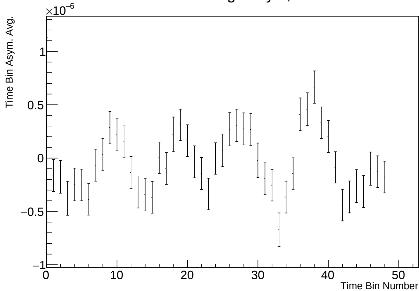
Time Bin Run Average Asym, r38314 w88
