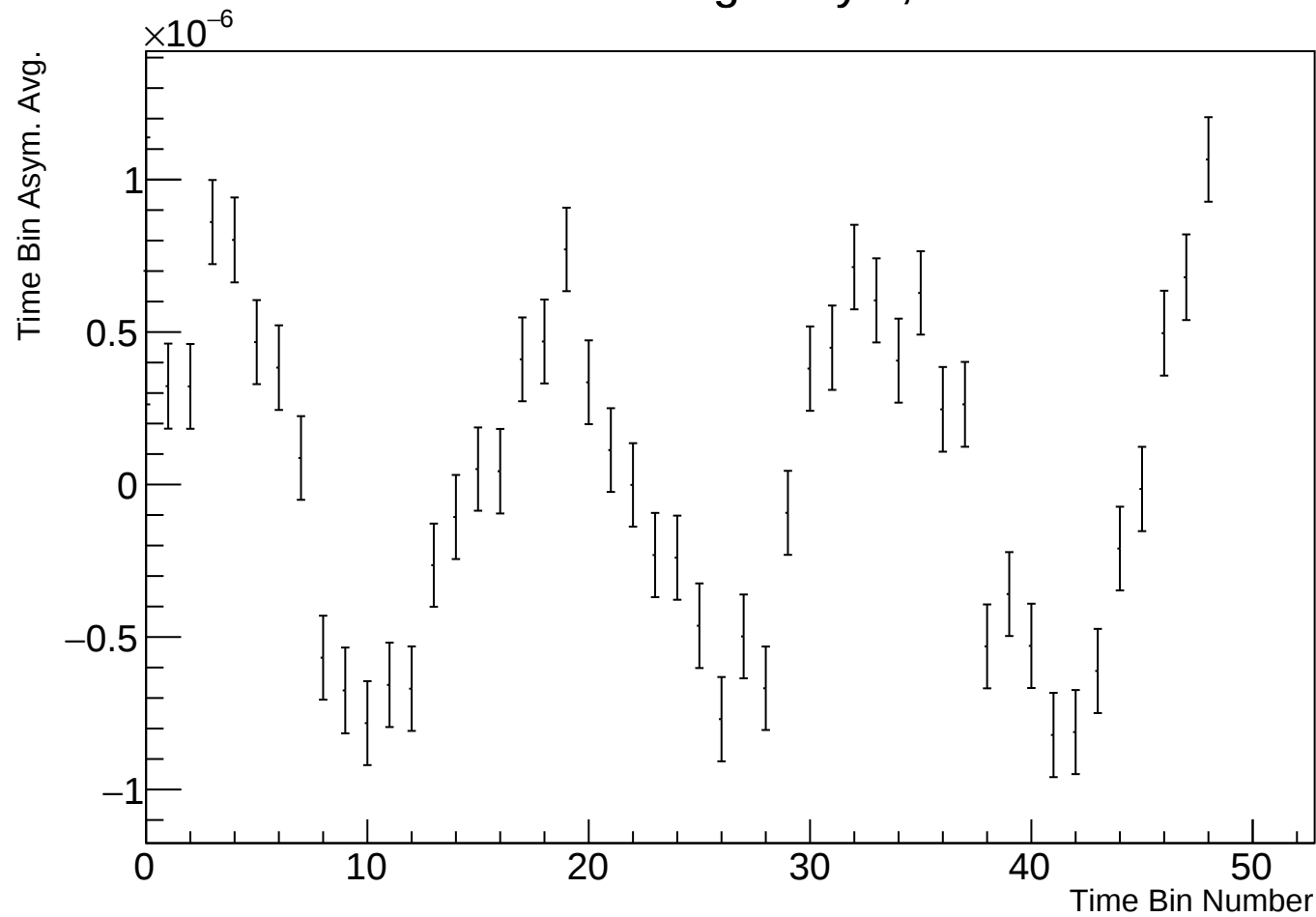
Time Bin Run Average Asym, r38314 w62
