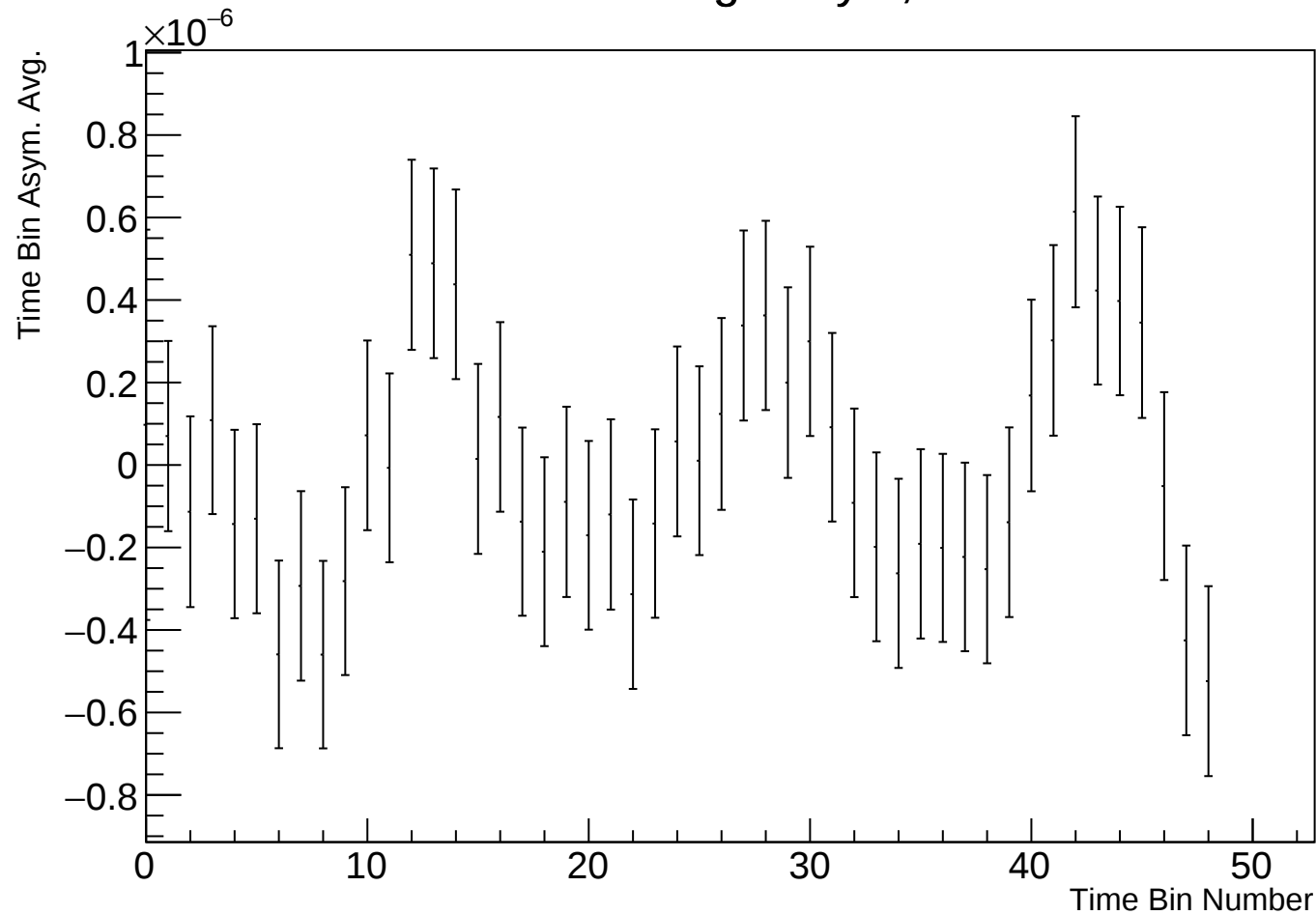
Time Bin Run Average Asym, r38314 w20
