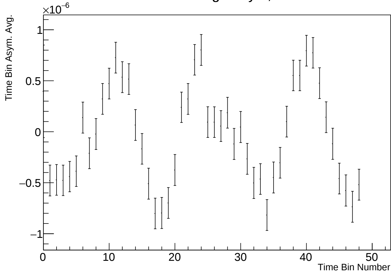
Time Bin Run Average Asym, r38314 w56
