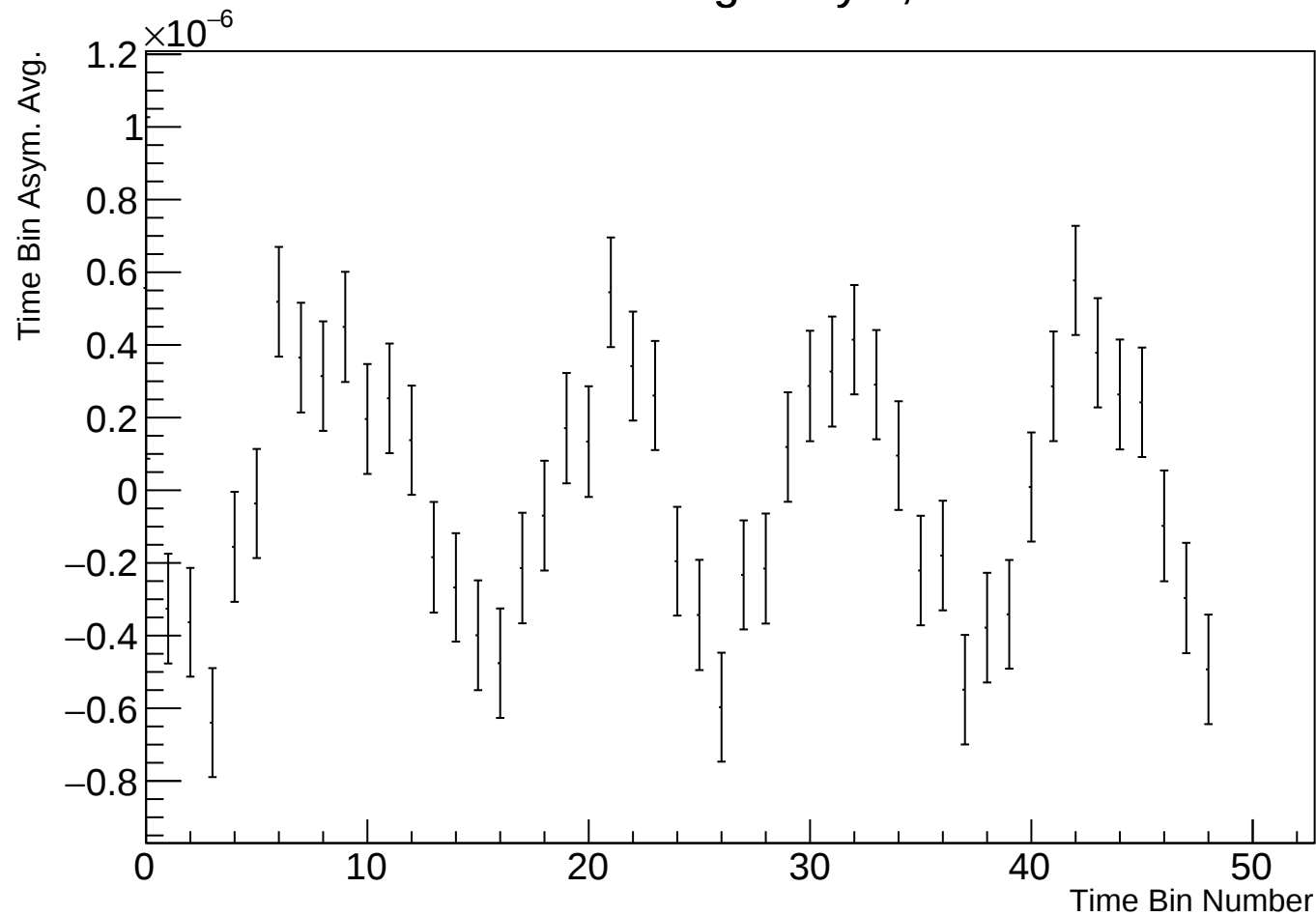
Time Bin Run Average Asym, r38314 w90
