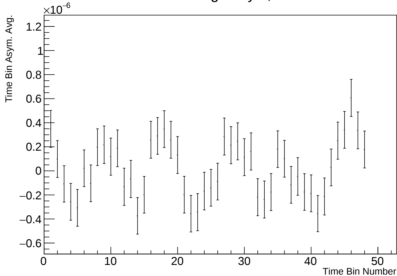
Time Bin Run Average Asym, r38314 w119
