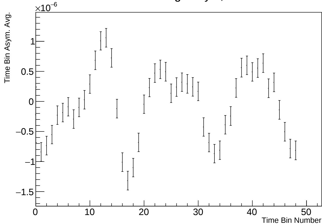
Time Bin Run Average Asym, r38314 w94
