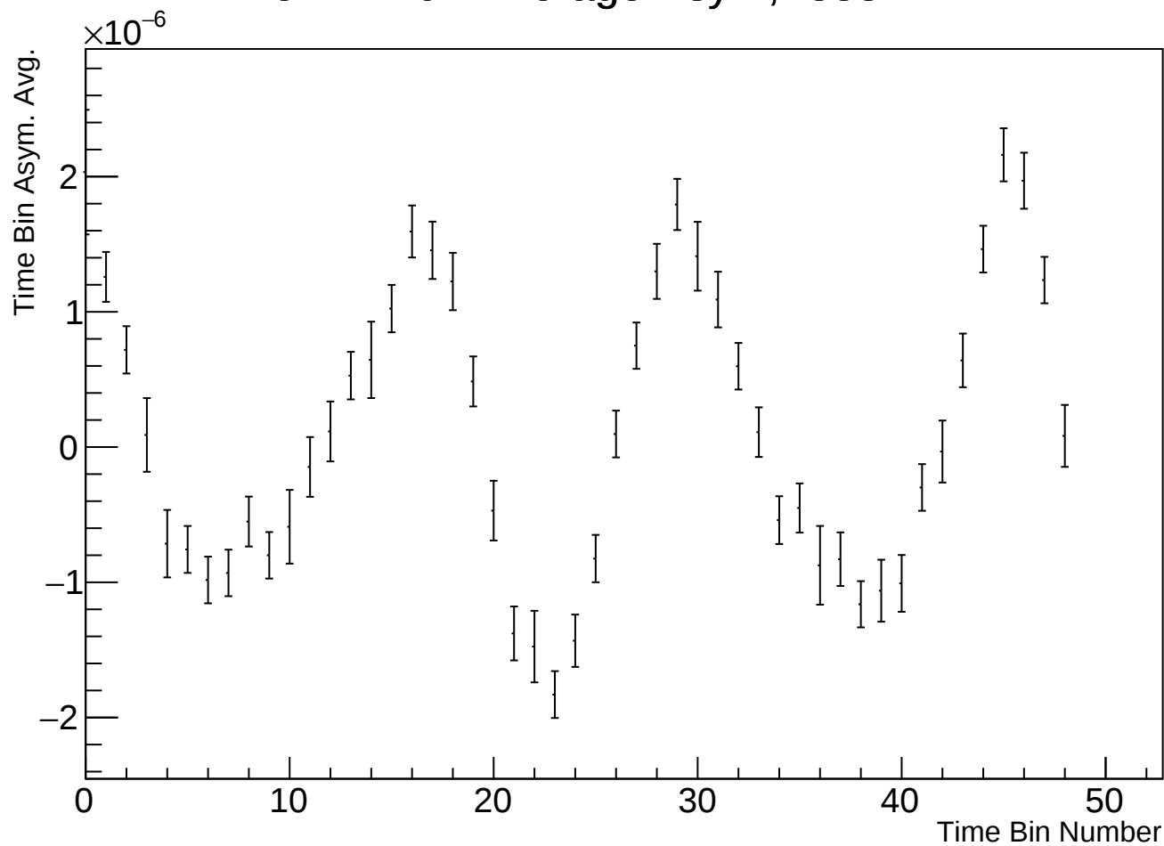
Time Bin Run Average Asym, r38314 w124
