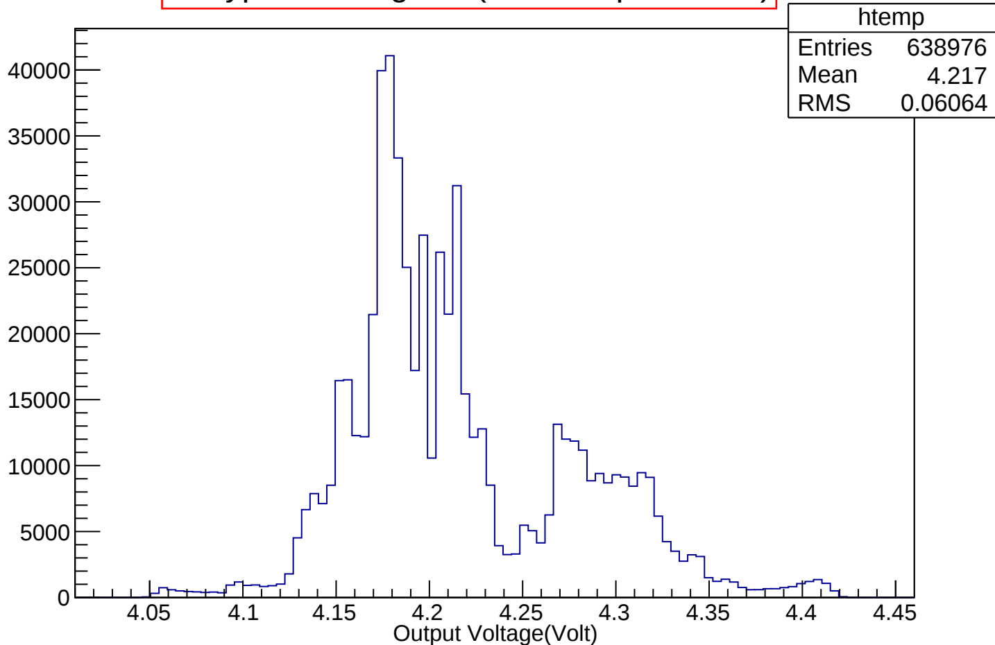
A typical histogram (Here for pin1 of J1)
