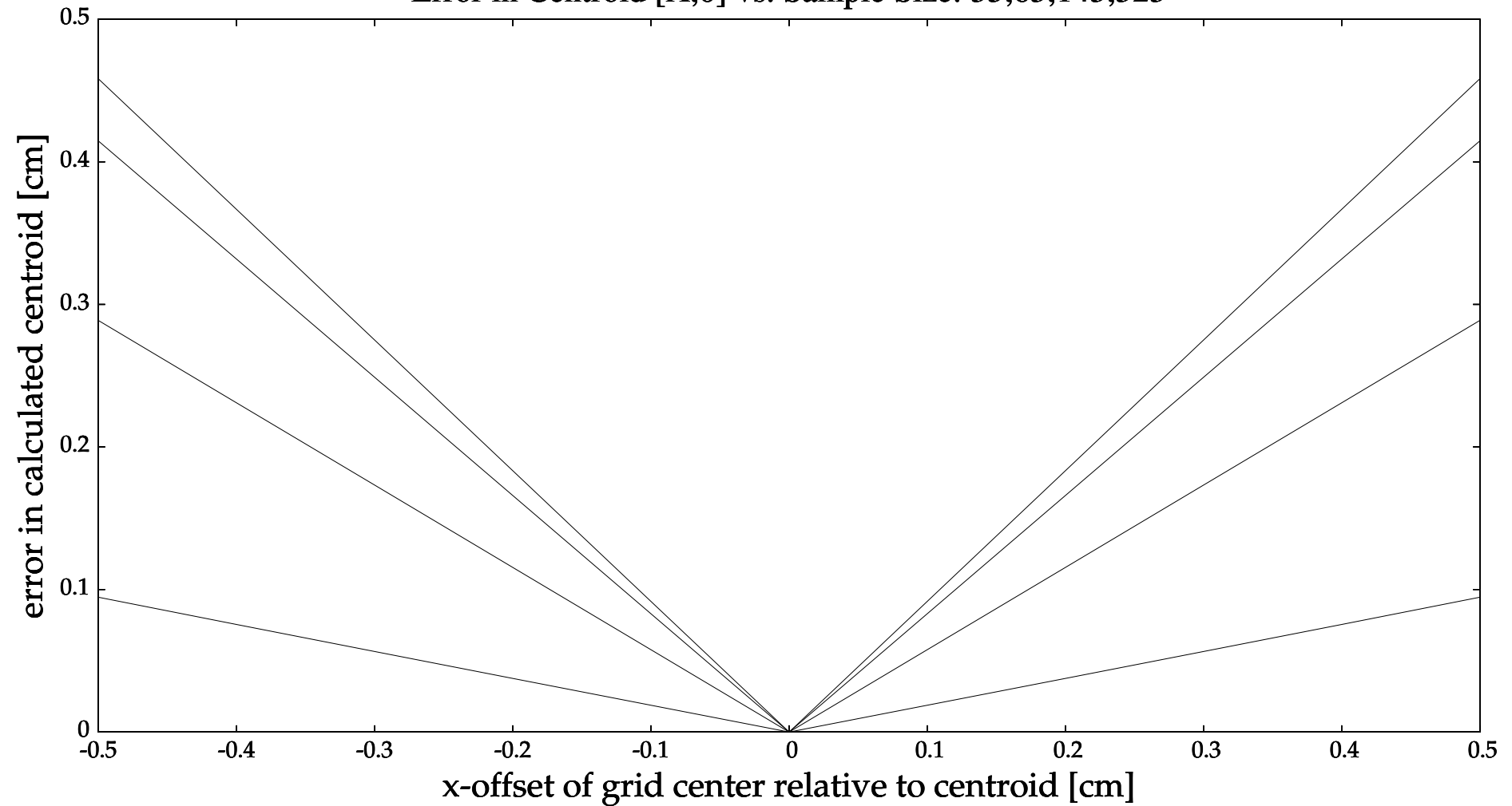
Error in Centroid [X,0] vs. Sample Size: 35,63,143,323
