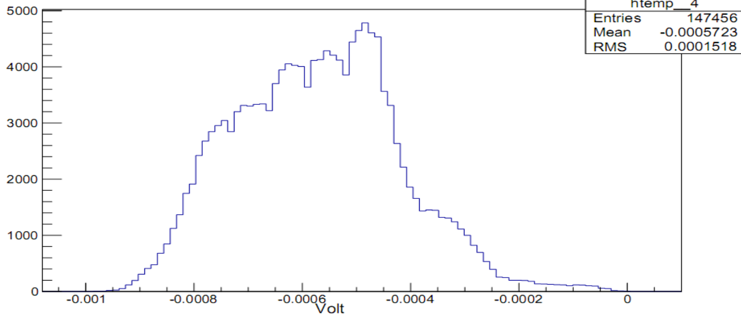
Noise measurement for Unshielded pre-amp (Output pin 1 & 2 of J1)
