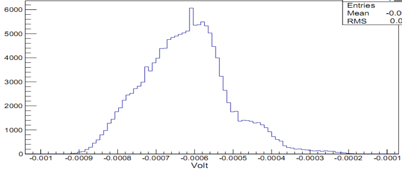
Noise measurement for Unshielded pre-amp (Output pin 16 & 17 of J10)
