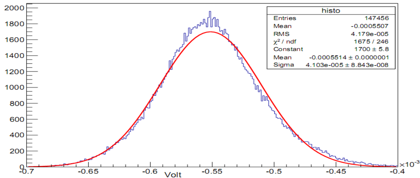
Noise measurement for shielded pre-amp with no input (Output pin 1 & 2)
