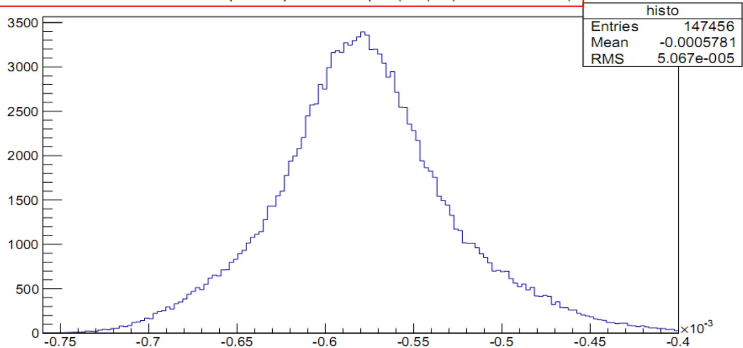
Noise measurement for shielded pre-amp with no input (Output pin 16 & 17 of J1)
