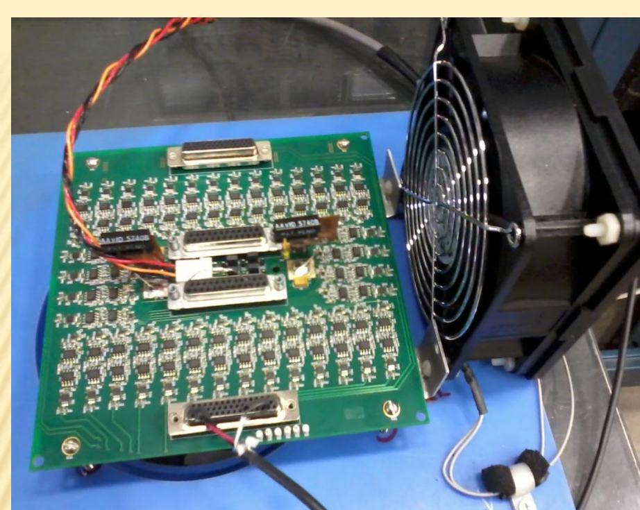
Unshielded pre-amp
