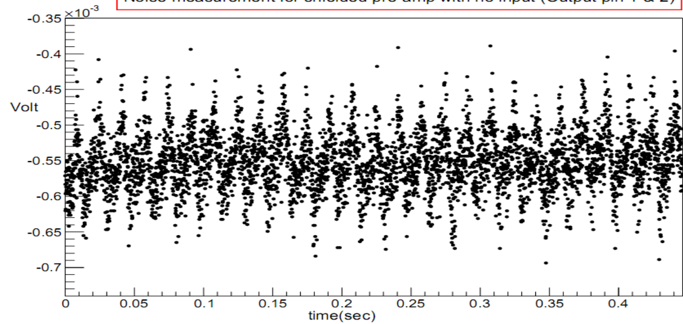
Noise measurement for shielded pre-amp with no input (Output pin 1 & 2)
