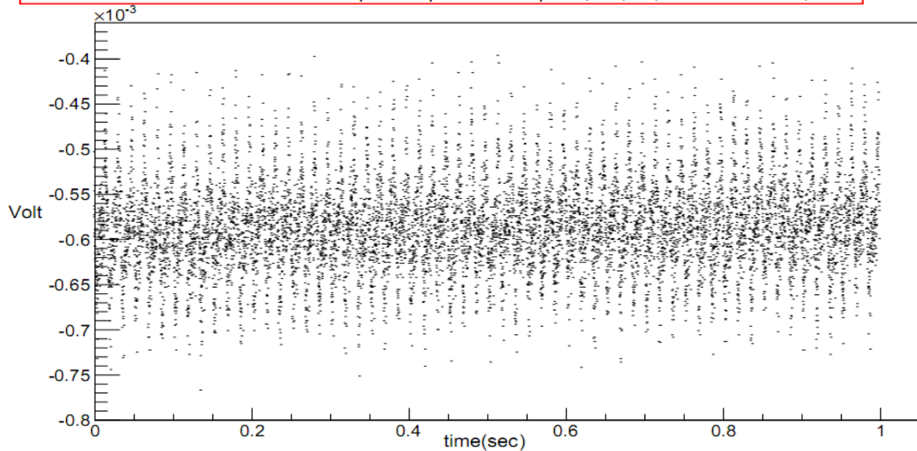
Noise measurement for shielded pre-amp with no input (Output pin 16 & 17 of J1)
