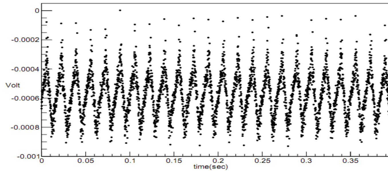
Noise measurement for unshielded pre-amp (Output channel 1&2 of J1)
