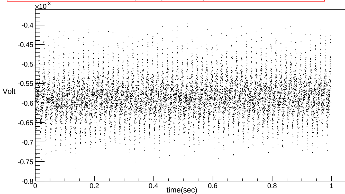
Noise measurement for shielded pre-amp with no input (Output pin 16 & 17 of J1)
