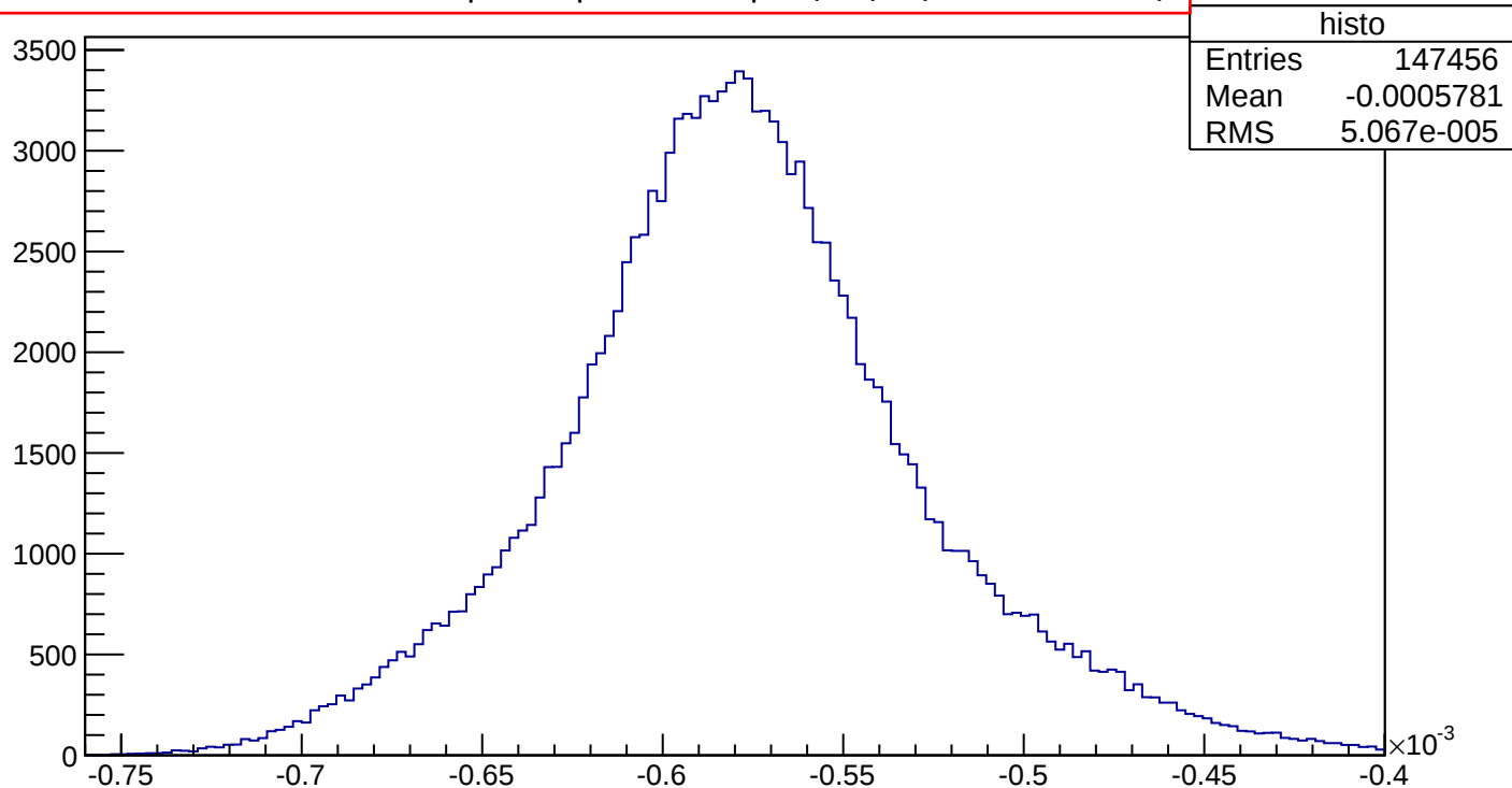
Noise measurement for shielded pre-amp with no input (Output pin 16 & 17 of J1)
