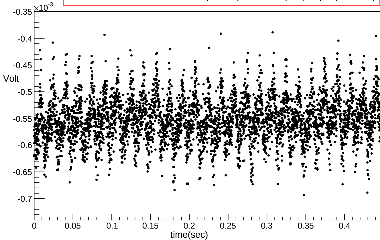
Noise measurement for shielded pre-amp with no input (Output pin 1 & 2)
