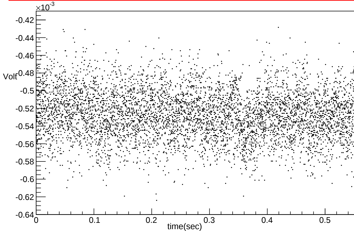
Pre-amp measurement with no input (with DAQ body and pre-amp body connected ground)
